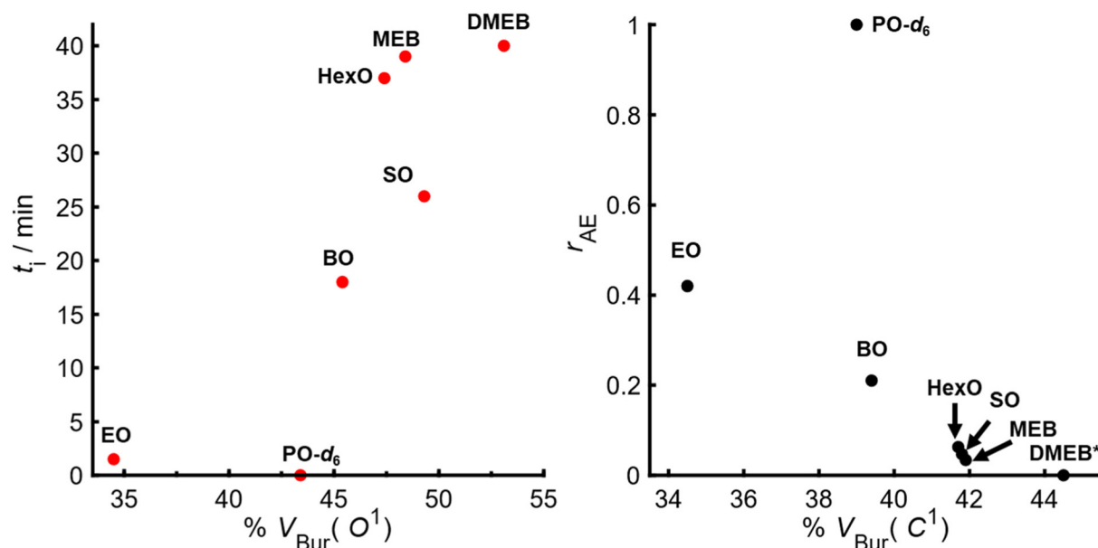
Fig. 5 Left: determined induction times for the experiment with the respective comonomer plotted vs. \%V_{Bur}(O^1) of the respective comonomer. Right: determined reactivity ratios of comonomers plotted vs. \%V_{Bur}(C^1) of the respective comonomer. *DMEB was included as a reference point with r_{DMEB} set to 0.
