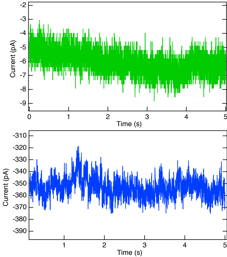
FIGURE 3.14. Leakage currents flowing through a well coated tip (top) and a bad coated tip (bottom). Recorded with the STM, at E_{sample}=0.65 V and E_{tip}=0.30 V in electrochemical mode, on a gold substrate in contact with 0.01M H_2SO_4 .
