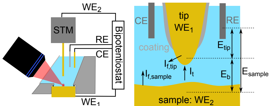
FIGURE 3.10. left: sketch of the EC-TERS configuration and electrodes. Reproduced with permission from Angewandte Chemie Int. Ed. , 88, 7108-7114 (2016); Copyright 2017 Wiley-VCH Verlag GmbH & Co. KGaA. [4] Right: zoom into the tip apex region, indicating Faraday currents ( I_f of tip and sample) and tunneling current ( I_t ); adapted from [34] .
