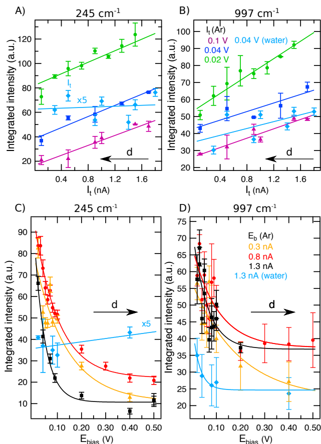
FIGURE 5.2. A: Integrated intensity of the 245\text{ cm}^{-1} mode (B: 997\text{ cm}^{-1} ) as a function of I_t at constant E_b values of 0.02 V (green), 0.04 V (dark blue), 0.1 V (purple) in Ar and 0.04 V in water (light blue). C: Integrated intensity of the 245\text{ cm}^{-1} mode (D: 997\text{ cm}^{-1} ) as a function of E_b at constant I_t values of 0.3 nA (orange), 0.8 nA (red), 1.3 nA (black) in Ar and 1.3 nA in water (light blue). Normalized to the same power and integration time. Averaged results from scans up and down are presented with standard deviation as error. Solid lines represent linear fittings (A and B) and exponential fittings (C and D) of the experimental data points. Reproduced with permission from Faraday discussions , 205, 233-243 (2017); published by the Royal Society of Chemistry. [3]
