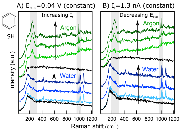
FIGURE 5.1. Raw spectra recorded in Ar (green) and in water (blue) for A: I_t ramp at constant E_b of 0.04 V, B: E_b ramp at constant I_t of 1.3 nA. For each series, 20 nm retraction spectra (far-field) are included in black. Gray rectangles indicate marker bands. Spectra are y-offset for clarity. Inset: PhS chemical structure. Reproduced with permission from Faraday discussions , 205, 233-243 (2017); published by the Royal Society of Chemistry. [3]
