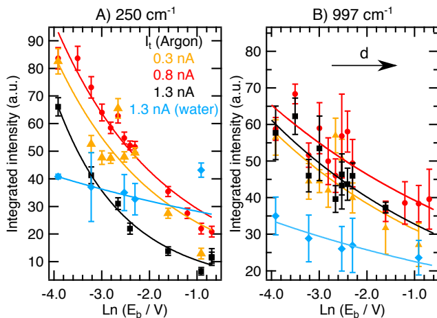
FIGURE 5.4. A: Integrated intensity of the 250\text{ cm}^{-1} mode (B: 997\text{ cm}^{-1} ) as a function of E_b at constant I_t values of 0.3\text{ nA} (orange triangles), 0.8\text{ nA} (red circles), 1.3\text{ nA} (black squares) in Ar and 1.3\text{ nA} in water (light blue diamonds). Averaged results from spectra taken in scans up and down are presented with standard deviation as error. Fittings to Eq. 5.3 are included (solid lines). Reproduced with permission from Faraday discussions , 205, 233-243 (2017); published by the Royal Society of Chemistry. [3]
