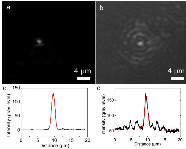
FIGURE 3.5. Images of the focus points taken with the CMOS camera in a: air at 127\ \mu\text{W} , exposure time 10\ \mu\text{s} , S/N=21 and b: water at 600\ \mu\text{W} (at the exit of the objective), exposure time 40\ \mu\text{s} , S/N=11 . c: Lateral profile of the focus (black) fitted to a Gaussian profile (red) in air (d: water). Reproduced with permission from Analytical Chemistry , 88, 7108-7114 (2016); Copyright 2016 American Chemical Society. [1]
