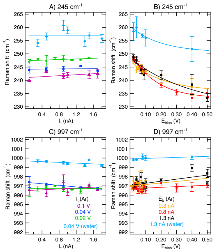
FIGURE 5.5. Raman shift of the 245 cm -1 as a function of I_t (A) for constant values of bias voltage in Ar (0.02 V green, 0.04 V dark blue, 0.1 V purple) and water (0.04 V, light blue), and as a function of E_b (B) for constant values of tunnelling current in Ar (0.3 nA orange, 0.8 nA red, 1.3 nA black) and water (1.3 nA, light blue). C and D show the equivalent shifts for the 997 cm -1 band. Averaged results from spectra taken in scans up and down are presented with standard deviation as error. Solid lines represent linear fittings (A, C and D) and exponential fittings (B) of the experimental data points. Reproduced with permission from Faraday discussions , 205, 233-243 (2017); published by the Royal Society of Chemistry. [3]
