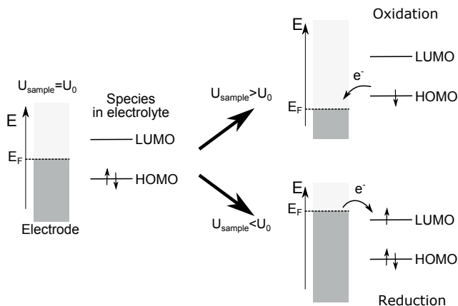
FIGURE 2.3. In electrochemistry, applying a potential to the electrode ( U_{\text{sample}} ) results in a ramp of Fermi energy ( E_F ) with respect to the equilibrium position, U_0 . Depending on the sign of the potential, oxidation or reduction of the species in the solution occurs. Left: At a given potential U_0 , the interface is at equilibrium with E_F of the electrode lying in between highest occupied molecular orbital (HOMO) and the lowest unoccupied molecular orbital (LUMO) of the electroactive species at the interface. Right: When U_{\text{sample}} is more positive than U_0 , E_F decreases to a level where the electrons in the HOMO flow to the electrode resulting in a oxidation process (reduction of the electroactive species happens when U_{\text{sample}} is more negative than U_0 , rising E_F of the electrode to a level where electrons can flow from the electrode into the LUMO of the species in solution).
