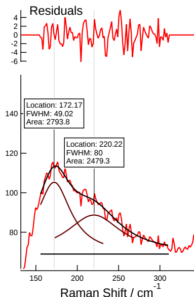
FIGURE A.3. Fitting of the far-field (20 nm tip retraction) spectrum of adenine/Au(111) in \text{H}_2\text{SO}_4 (0.01 M). Reproduced with permission from Angewandte Chemie Int. Ed. , 88, 7108-7114 (2016); Copyright 2017 Wiley-VCH Verlag GmbH & Co. KGaA. [4]
