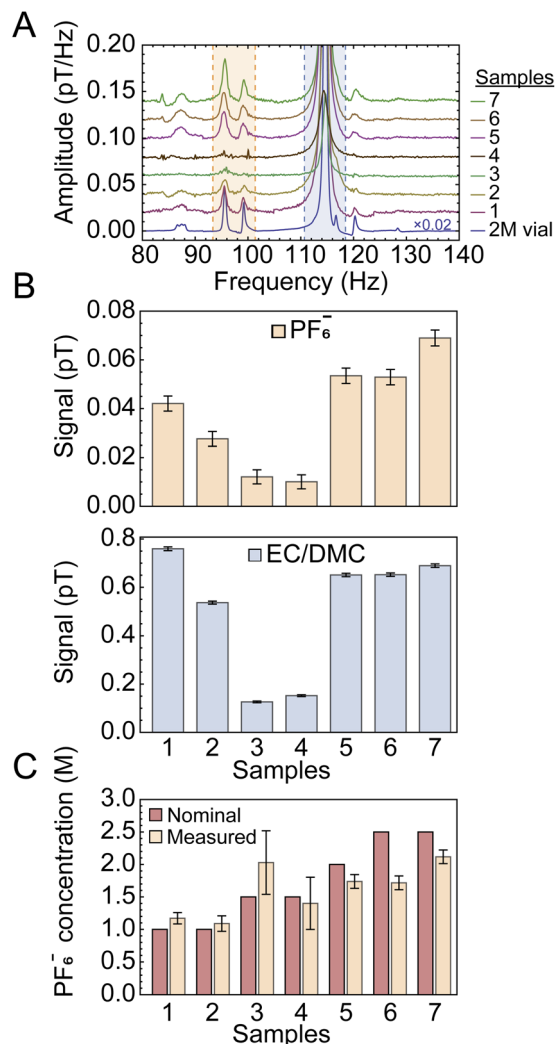
Fig. 3 (A) Stacked plots showing the measured electrolyte signals at a 2.7 \mu\text{T} background field from a series of sample cells filled with electrolyte of different nominal (prepared) \text{LiPF}_6 concentrations. All spectra were obtained with the setup and protocol in Fig. 1 from averages of 10 000 scans, apart from sample 1 and the calibration vial for which 8913 and 256 scans were collected, respectively; the large number of scans was selected to improve SNR of measured signals from the cells, as well as to suppress the power-line harmonic at 100 Hz. (B) Quantification of signals obtained from integration of the shaded areas indicated in (A) for the solute and solvent peaks (top and bottom panels, respectively). Error bars correspond to the standard errors obtained in Fig. 4 and their values as a fraction of the signal scale inversely with SNR, as explained in the text. (C) \text{LiPF}_6 concentrations obtained from the measurements in (B) and propagation of errors, according to the procedure outlined in the text.
