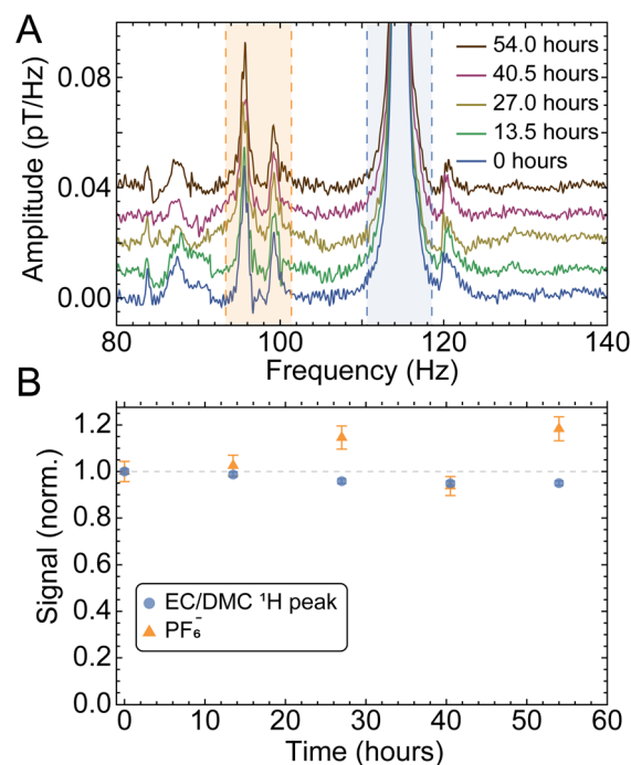
Fig. 4 Monitoring of the electrolyte peaks as a function of time, using five partitions or batches of 2000 scans (13.5 h each) from the cell with a nominal 2.5 M \text{LiPF}_6 concentration (sample 7 in Fig. 3). (A) Measured spectra, and (B) solute and solvent integrals normalized to the first data point. Error bars are calculated as standard error of the partitioned integrated signals (shaded regions). The error on the proton signal is smaller than that on the \text{PF}_6^- signal (relative errors of 4.4% and 1.1% for solute and solvent signals, respectively), as expected due to the smaller SNR of the latter. The electrolyte signals from this sample cell were found to be relatively stable not only over the course of the three-day measurement cycle (with minor fluctuations), but also in a second measurement taken two months later (Fig. S7).
