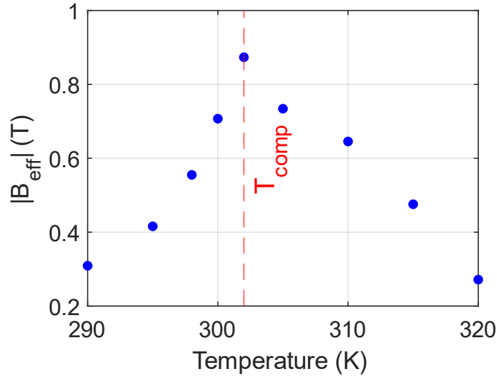
FIG. S3. Temperature dependence of the effective emergent field B_{eff} , estimated from \rho_{xy}^{THE} = R_H \cdot B_{eff} using the extracted topological Hall resistivity and ordinary Hall coefficient.
