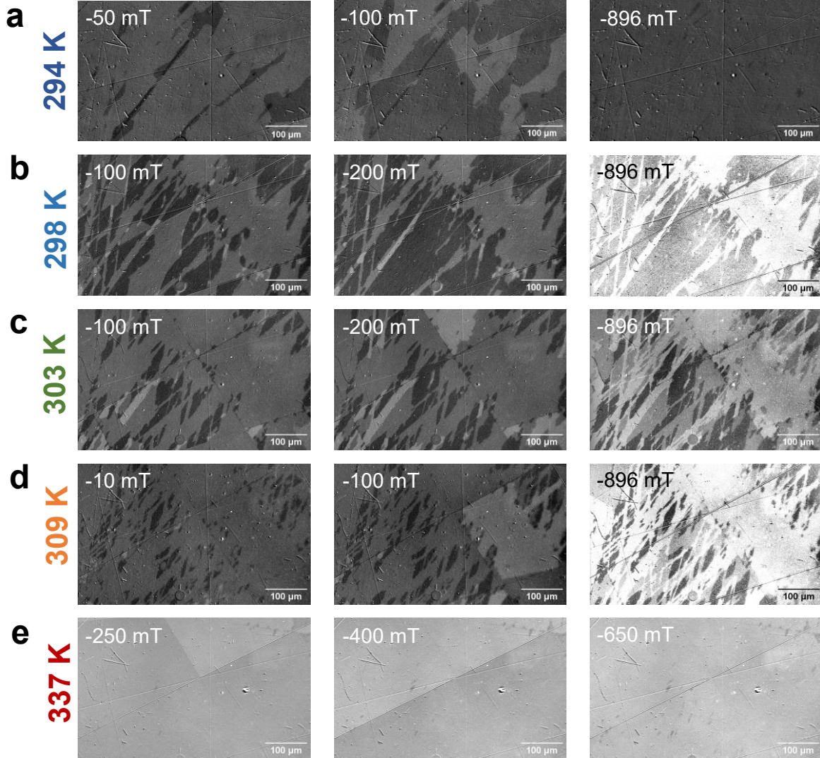
Fig. 3. Polar Kerr imaging across the compensation region. (a–e) Difference Kerr images (with respect to the +896 mT state) acquired at selected negative magnetic field strengths for five representative temperatures: 294 K (far below compensation), 298 K (below compensation), 303 K (near compensation), 309 K (above compensation), and 337 K (far above compensation). For 298–309 K, the film cannot be fully saturated within the 896 mT OOP, and the reversal proceeds through mixed multidomain states that correspond to the SH-AHE+SH-THE features seen in transport. Around the compensation (298 K, 303 K and 309 K), the domain pattern becomes irregular and multidomain, consistent with the non-collinear regime. At 294 K and 337 K, only SH-AHE is observed, the
