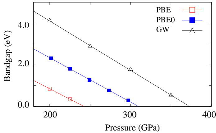
Figure 1. Band gap of the Cmca -12 crystal structure as a function of pressure as calculated using the PBE, PBE0 and GW approximations. The PBE, PBE0 and GW results show that the band gap of Cmca -12 vanishes at 245, 309 and 373 GPa, respectively.
