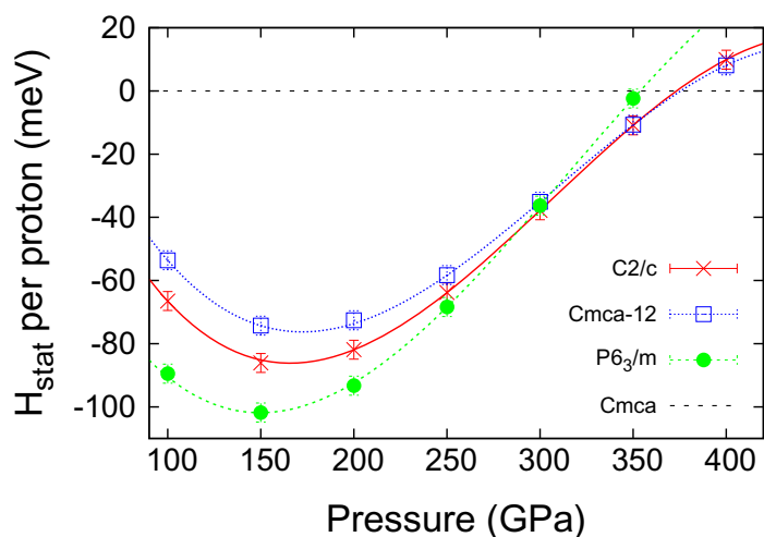
Figure 2. Enthalpy as a function of pressure calculated using the DMC-TABC method in the static approximation. The static lattice enthalpies of three different insulating crystal structures are reported relative to the enthalpy of the metallic Cmca structure. The metallization occurs via a transition from the zero band-gap Cmca-12 structure to the metallic Cmca structure at around 375 GPa.
