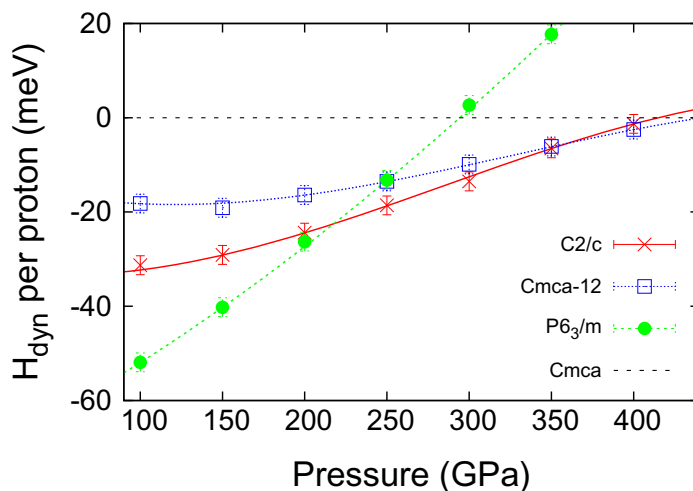
Figure 3. Enthalpy as a function of pressure calculated using the DMC-TABC method in the dynamic approximation. The quasi-harmonic proton ZPE was calculated using DFT. The dynamic lattice enthalpies of three different insulating crystal structures are reported relative to the enthalpy of the metallic Cmca structure. The P6 3 /m , C2/c , Cmca-12 and Cmca phases are stable in the pressure ranges <220, 220–360, 360–430 and >430 GPa, respectively
