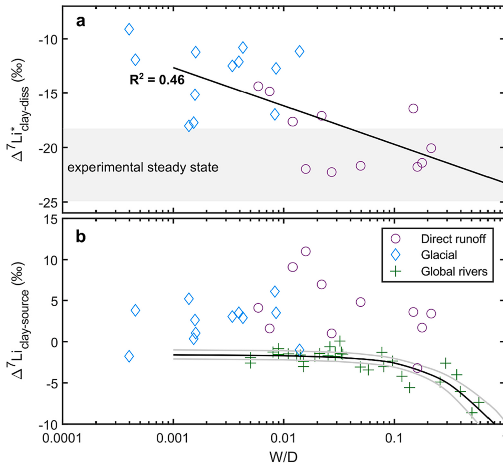
Fig. 9. (a) Relationship between the weathering intensity (W/D, where W = weathering, D = denudation) and the difference between the \delta^7\text{Li} values of the clay fraction and the dissolved fraction. The grey bar labelled ‘experimental steady-state’ is the equilibrium fractionation observed in basalt weathering experiments (Pogge von Strandmann et al., 2019b; Pogge von Strandmann et al., 2022). (b) Relationship between weathering intensity (W/D) and the difference between the \delta^7\text{Li} values of the clay fraction and the primary source rock (here, the calculated \delta^7\text{Li}_{\text{residue}} after leaching; see text for details). The green crosses represent fine-grained data ( <0.6 \mu\text{m} size fraction) from a global multi-lithological compilation, while the black line and its error margins represent their trend (Dellinger et al., 2017). Our Icelandic basalt clay Li isotope data are more similar to the boomerang-shaped relationship of the dissolved load Li isotopes than to the clay relationship seen by Dellinger et al. (2017). (For interpretation of the references to colour in this figure legend, the reader is referred to the web version of this article.)
