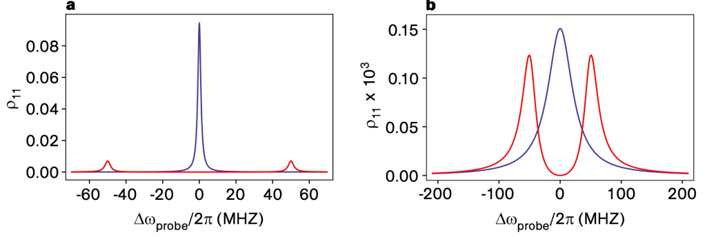
Figure 5.3: Probability of finding a photon in a bottle mode \rho_{11} , with ( g = 2\pi \cdot 50 MHz, red line) and without ( g = 0 , blue line) interaction between the bottle mode and the atom. In (a) the parameters are set to \varepsilon_0 = 2\pi \cdot 0.3 MHz, \kappa = 2\pi \cdot 0.98 MHz, \gamma_\perp = 2\pi \cdot 2.61 MHz. In (b) \kappa = 2\pi \cdot 24.4 is increased according to Q_{\text{crit}} = 7.2 \times 10^6 MHz which is a typical value for a bottle microresonator in add-drop configuration.
