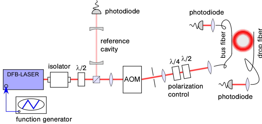
Figure 3.5: Schematic of the optical setup.
