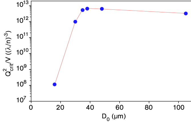
Figure 4.7: The ratio Q_{\text{crit}}^2/V for bottle microresonators of various diameter D_0 . This graph is based on the data from Fig. 3.18. The optimal ratio is obtained for resonators of diameters around 40 \mu\text{m} .
