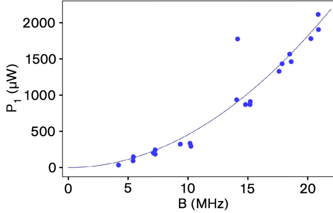
Figure 4.15: Variation of the switching threshold as a function of the resonator bandwidth. The solid line is a square-law fit ( P_1 = a_0 B^2 ) to the experimental data, confirming the quadratic dependency. This means that P_1/B^2 is constant at a value of a_0 = (4.75 \pm 0.20) \mu\text{W}/\text{MHz}^2 .
