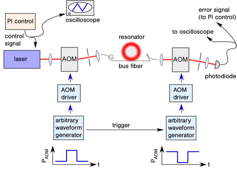
Figure 4.12: Setup for measuring the thermal relaxation time of a bottle mode. During the measurement, a sudden step in P_{\text{in}} is applied using an arbitrary waveform generator that controls the power modulation input of the AOM's driver unit ( P_{\text{AOM}} denotes the power of the radiofrequency signal sent to the AOM). During the modulation of P_{\text{in}} , the laser-resonator detuning \delta^\nu is kept constant by the side-of-fringe power lock technique described in section 4.2.4. The control signal sent from the PI control module to the laser current modulation input is then proportional to the resonance frequency shift and the change in the temperature of the mode volume induced by the sudden increase in the intracavity intensity. Due to the variation in P_{\text{in}} , the power measured directly behind the bus fiber output is no longer a suitable error signal for the lock because it not exclusively depends on \delta^\nu . Therefore, the step in P_{\text{in}} is compensated using a second AOM in front of the photodiode. This ensures that the signal detected at the photodiode is proportional to the transmission through the ultra-thin waist of the bus fiber U_{\text{PD}} \propto P_{\text{out}}^{\text{bus}}(t)/P_{\text{in}}(t) .
