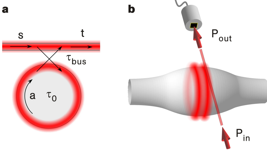
Figure 3.6: (a) The coupling junction between the bus fiber and the bottle microresonator can be described by a simple model using few parameters. The “mode amplitude” of the bottle microresonator is denoted by a . Whereas s and t are the “input field amplitude” and the “output field amplitude” of the waveguide. Characteristic time constants \tau_{\text{bus}} and \tau_0 describe the transfer of optical energy between both structures and the intrinsic resonator energy loss. (b) In the experimental characterization the power transmitted through the bus fiber P_{\text{bus}}^{\text{out}} = |t|^2 is measured for a given input power P_{\text{in}} = |s|^2 and varying width x of the coupling gap.
