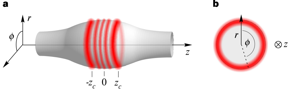
Figure 2.1: Sketch of the resonator geometry along (a) and in a plane perpendicular (b) to the resonator axis. The Helmholtz equation is solved in cylindrical coordinates. (b) The azimuthal coordinate is denoted by \phi . (a) The radial coordinate and the axial coordinate are denoted by r and z , respectively. A slowly varying parabolic profile of the resonator radius along the z axis is assumed (see Eq. (2.1)). The radial and axial (indicated in red) intensity distribution of the modes is derived. Each bottle mode is located between two caustics at \pm z_c . The caustic radius R_c can be understood as a cutoff for propagation along z due to the angular momentum of the bottle mode.
