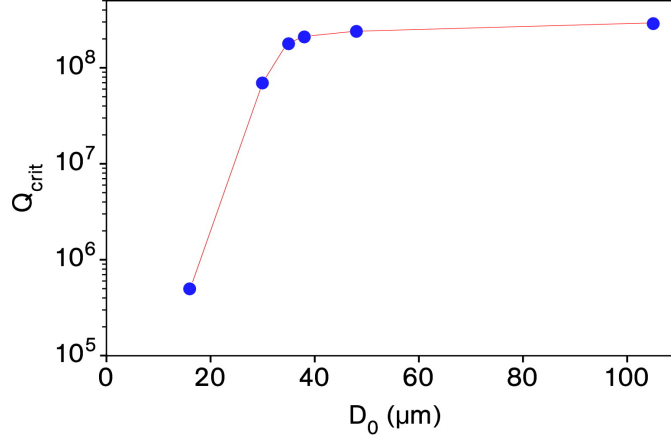
Figure 3.17: Quality factor Q_{\text{crit}} as a function of resonator diameter D_0 . For resonator diameters ranging from 30 – 105 \mu\text{m} , ultra-high quality factors are measured using a cavity-ringdown technique. Due to the small errors on the order of 0.5%, no error bars are shown. The quality factor of 4 \times 10^5 for D_0 = 16 \mu\text{m} is inferred from the linewidth of the mode. The red line is a guide to the eye. Modes with varying axial quantum numbers in resonators with different curvatures of the resonator profile were used. However, for a given resonator diameter, a dependency of the quality factor on the axial quantum number and on the curvature of the resonator profile is not observed.
