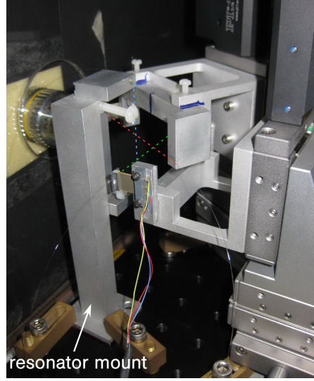
Figure 3.4: Mechanical setup used for operating a bottle microresonator in add-drop configuration. The bottle microresonator (indicated by the dashed blue line) is mounted vertically. The bus (dashed green line) and the drop fiber (dashed red line) are mounted in a plane perpendicular to the resonator axis. Each ultra-thin fiber can be manipulated using a positioning system as shown in Fig. 3.2. The picture shows a situation in which both ultra-thin fibers are moved away from the bottle microresonator.
