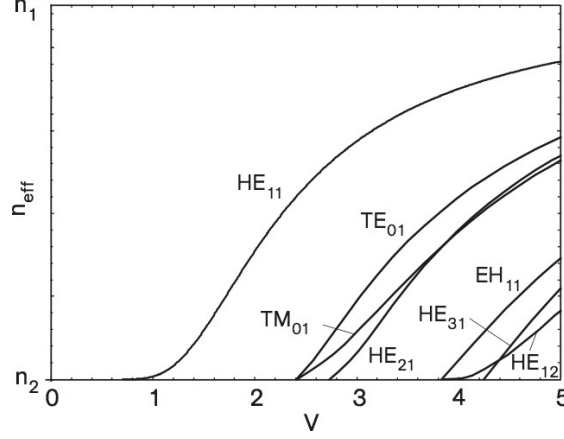
Figure 2.8: The normalized propagation constant \beta/k_0 = n_{\text{eff}} as a function of the V -parameter for various solutions of Eq. (2.44). The fundamental HE_{11} mode exists for all fiber radii. All other modes are only guided if the fiber radius is larger than a certain cutoff radius.
