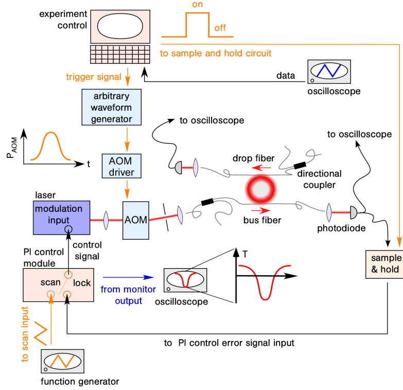
Figure 4.10: Measuring the nonlinear response in the transmission properties through two ultra-thin fibers coupled to a bottle mode in add-drop configuration, induced by a modulation of the input power P_{in} . An arbitrary waveform generator, triggered by the experiment control, sends an \sin^2 -shaped pulse to the modulation input of the AOM's driver unit which controls the power of the radiofrequency signal P_{AOM} that is sent to the AOM. The initial cold laser-resonator detuning \delta_0' is set using a side-of-fringe power lock technique, where the signal transmitted through the bus fiber is fed back to the current modulation input of the laser using a PI control loop. In the "scan mode" the laser frequency is constantly swept over the resonance. A monitor output of the PI control module allows one to choose a "set point". In the "lock mode", the PI control module controls the laser diode current in order to keep the error signal at this set-point. Its value is chosen corresponding to the desired value of the laser-resonator detuning. The PI control module allows one to change the sign of \delta_0' by inverting the input signal. A sample-and-hold circuit "freezes" the lock during the pulse. A directional coupler at the inputs of both ultra-thin fibers allows one to measure the losses in the fiber tapers in order to obtain the power levels P_{in} and P_{out} in the ultra-thin fiber waists.
