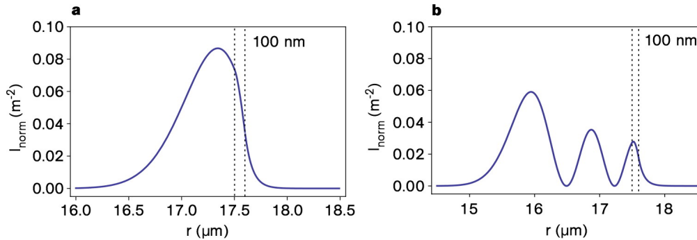
Figure 4.19: (a) Normalized radial intensity distribution of the fundamental radial mode for a wavelength around 850 nm in a silica WGM resonator with a diameter of 35 \mu\text{m} and a polymer coating of thickness d = 100 nm. At this wavelength the overlap of the radial intensity distribution with the polymer film is larger than for the same coating thickness and \lambda = 1080 nm (Fig. 4.18). (b) Higher order radial mode in the same resonator. The overlap of the radial intensity distribution with the polymer film is much smaller than for the fundamental radial mode. This results in both, less absorption and a smaller enhancement of the nonlinear refraction. Moreover, the intensity at the surface is about a factor of two smaller than for the fundamental mode.
