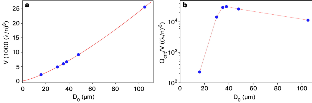
Figure 3.18: (a) Calculated mode volumes for different resonator diameters. The calculation assumed TE polarization, an axial quantum number of q = 1 and a curvature of \Delta k = 0.012 \mu\text{m}^{-1} . (b) Q_{\text{crit}}/V obtained from the calculated mode volumes shown in (a) and the radial dependency of Q_{\text{crit}} presented in Fig. 3.17.
