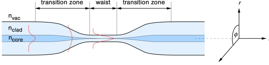
Figure 2.7: Schematic of an ultra-thin tapered optical fiber. The fiber is produced from a commercial step-index glass fiber using a heat-and-pull technique. In the thick fiber ends the mode is guided by total internal reflection induced by the weak refractive index contrast between core and cladding n_{\text{core}} - n_{\text{clad}} \ll 1 . The mode in the ultra-thin fiber waist is guided due to the refractive index contrast between the cladding and the surrounding medium n_{\text{clad}} - n_{\text{vac}} \approx 0.5 . Shaping the transition zone for optimal coupling between both modes is a prerequisite to obtain high transmission of optical power through the fiber taper [Lov86, War07].
