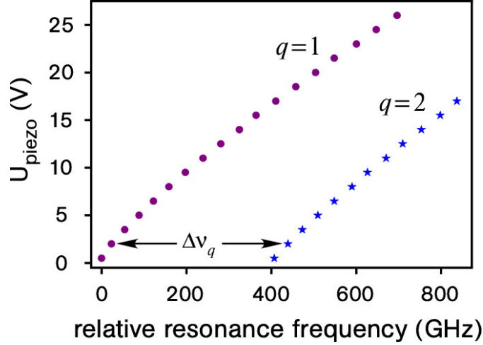
Figure 3.19: Tuning the bottle microresonator. Using a piezo-electric actuator to elastically elongate a bottle microresonator of 35\ \mu\text{m} diameter and \Delta k = 0.012\ \mu\text{m}^{-1} , the TE polarized q = 1 and q = 2 bottle modes are strain-tuned. The tuning range of 700 GHz of the q = 1 mode exceeds the observed axial FSR of \Delta\nu_q = 425 \pm 8\ \text{GHz} .
