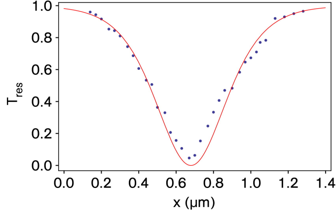
Figure 3.9: Transmission on resonance T_{\text{res}} for various values of the width x of the coupling gap. Critical coupling is achieved for x = 680 nm. The data shows close agreement with the theoretical prediction from the model. The measurement is taken for a q = 1 mode in a resonator with a diameter of 35 \mu\text{m} . The red line shows a fit to the data according to the model presented in previous section, assuming an exponential variation of \tau_{\text{bus}}(x) .
