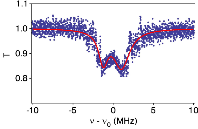
Figure 3.12: Modal coupling in a bottle microresonator. The measurement shows a q = 1 mode in a bottle microresonator with a diameter of 35 \mu\text{m} in the under-coupled regime. The fit (red line) is a superposition of two Lorentzian profiles with \Delta\nu of 1.4 MHz and 2.5 MHz and a spectral separation of 2.3 MHz. The observation of distinct linewidth can be explained by the fact that both eigenmodes are mutually orthogonal standing waves. For this reason they sense different parts of the resonator surface and thus experience different losses.
