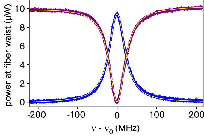
Figure 4.2: Resonant power transfer between two ultra-thin optical fibers coupled to the evanescent field of a bottle mode with ultra-high intrinsic quality factor. The plot shows the powers at the waists of the bus fiber P_{\text{out}}^{\text{bus}} (purple dots) and the drop fiber P_{\text{out}}^{\text{drop}} (blue dots) while the frequency of the probe laser is swept over the resonance. A loaded quality factor of Q_{\text{load}} = 7.2 \times 10^6 and a power transfer efficiency E = 0.93 is inferred by fitting a Lorentzian to both signals (yellow curves).
