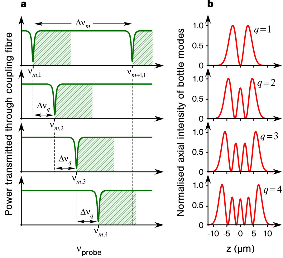
Figure 3.20: Bottle microresonator tuning scheme for the resonator with D_0 = 35 \mu\text{m} and \Delta k = 0.012 \mu\text{m}^{-1} , for which tuning over one axial FSR was demonstrated in Fig. 3.19. For this resonator dimensions \Delta\nu_m = 1.9 \text{ THz} is calculated to be five times larger than the measured value of \Delta\nu_q = 425 \text{ GHz} . (a) Assuming the measured tuning range (indicated by the green shaded areas) of 700 \text{ GHz} , the q = 1 - 4 bottle modes allow one to fully bridge the azimuthal FSR of the bottle microresonator. This makes any arbitrary frequency accessible by strain tuning the nearest mode with q = 1 - 4 and m properly chosen. (b) Calculated axial intensity distribution of the TE polarized q = 1 - 4 bottle modes for the resonator dimensions given above. These modes exhibit the smallest possible separation between the two caustics and thus yield the smallest mode volumes ranging from 1180 \mu\text{m}^3 to 1470 \mu\text{m}^3 for a wavelength of \lambda = 850 \text{ nm} .
