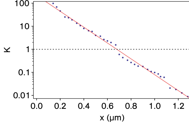
Figure 3.10: Spatial variation of the coupling parameter calculated from T_{\text{res}} . The solid line (red) is a fit of the form K_0 \cdot \exp(-x/\gamma_0) with \gamma_0 = 130 nm. A maximum value of K = 98 is obtained close to the resonator surface. The horizontal dashed line indicates the critical coupling point for which K = 1 .
