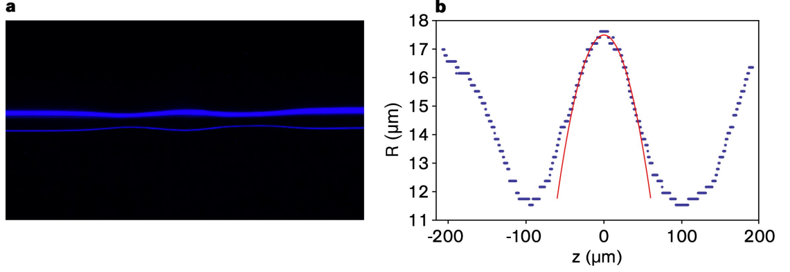
Figure 2.11: Reconstructing the diameter profile of a bottle microresonator. (a) Micrograph of a typical bottle microresonator taken after fabrication. Since the customized image analysis software uses only the information from the blue pixels all other pixels are deactivated. A flashlight mounted in the fiber pulling rig is used for illumination. (b) Reconstructed diameter profile with a parabolic fit (red). Only the data in the region z = \pm 35 \mu\text{m} have been considered for the fit. In the central zone where the mode is guided the resonator profile shows close agreement with a parabola of the form D(z) \approx D_0 \cdot [1 - 1/2 (\Delta k \cdot z)^2] . The fit yields D_0 = 35 \mu\text{m} and \Delta k = 0.0135 \mu\text{m}^{-1} .
