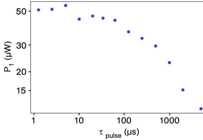
Figure 4.14: Dependency of the threshold power for optical bistability on the FWHM duration of the input pulses. This measurement is taken without the drop fiber. For pulse durations shorter than 100 \mu\text{s} , the quasi-instantaneous Kerr effect dominates the thermo-optical effect due to the finite thermal relaxation time ( \tau_{\text{therm}} \sim 15 \text{ ms} ) of the resonator mode. ON-OFF switching of the transmission through the bus fiber via the Kerr effect is achieved at a threshold power of 50 \mu\text{W} .
