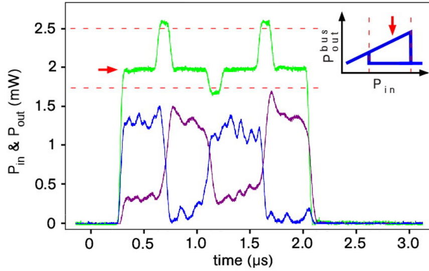
Figure 4.17: Demonstration of optical memory functionality in a bottle microresonator using the Kerr effect. For an input power level (green) in the bistable regime (as indicated by the arrow) the power at the outputs of the bus fiber (blue) and of the drop fiber (purple) exhibits two stable states. The output state is chosen by temporarily lowering (raising) P_{in} below (above) the bistable regime, which is schematically indicated by the dashed lines.
