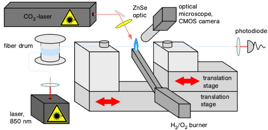
Figure 2.9: Schematic of the so-called “fiber pulling rig”, used to fabricate ultra-thin optical fibers and bottle microresonators. A commercial optical fiber is clamped to two translation stages. One stage is mounted on top of the other. The fiber is then heated by an oxygen-hydrogen flame with a width of 1 mm. The upper stage, called “stretcher”, elongates the heated fiber, while the “translator” moves it relative to the flame (“flame-brush technique”). Alternatively, a focused CO 2 -laser beam with a maximum power of 30 W (Synrad, Series 48-2) can be used as a heat source. The laser beam is focused by a ZnSe lens ( f = 48 \text{ mm} ) and only heats a 100 \mu\text{m} – 150 \mu\text{m} wide section of the fiber. A microscope connected to a CMOS camera allows one to take micrographs of processed fibers. Moreover, during the fabrication of ultra-thin optical fibers, the transmission of a diode laser emitting at a wavelength of 850 nm through the fiber is monitored.
