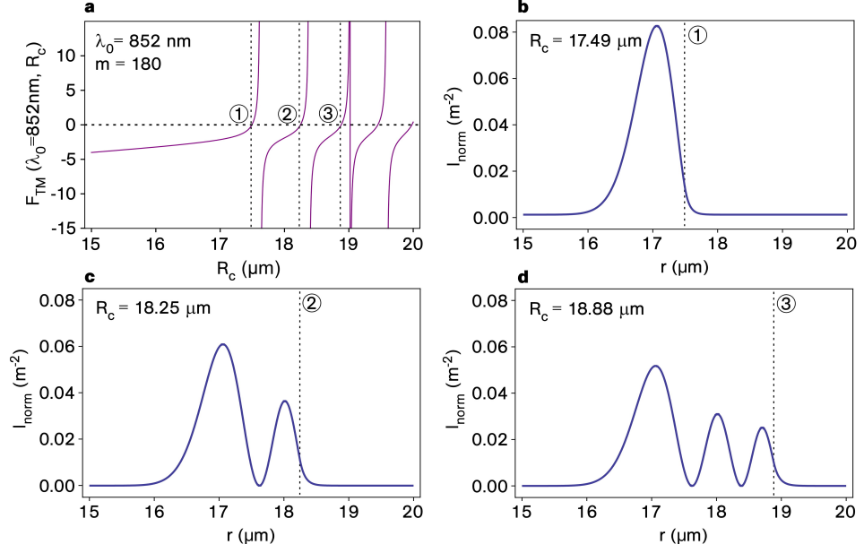
Figure 2.2: Solving the radial wave equation for TM polarization and m = 180 . (a) In order to identify resonant caustic radii, F_{TM}(\lambda_0 = 852 \text{ nm}, R_c) is plotted for R_c ranging from 15 \mu\text{m} to 20 \mu\text{m} and for a fixed wavelength of \lambda_0 = 852 \text{ nm} . The roots at R_c = 17.49 \mu\text{m} , R_c = 18.25 \mu\text{m} and R_c = 18.88 \mu\text{m} correspond to radii that fulfill the resonance condition. Radii R_c < 17.49 are not compatible with an angular momentum of L_z = 180\hbar . Plots (b–d) show the normalized radial intensity distribution I_{\text{norm}}(r) = |E_z(r)|^2 / \int |E_z(r)|^2 r dr for all three radii R_c obtained in (a). The intensity is normalized with respect to the radial power density in order to allow a comparison of the peak intensities of the different modes. For the smallest resonant radius, L_z = 180\hbar coincides with the maximum possible angular momentum L_{z,\text{max}} = \hbar m_{\text{max}} and the fundamental radial mode is obtained (b). This mode travels closest to the surface and offers the strongest confinement. For larger radii, m_{\text{max}} increases and the modes exhibit p = m_{\text{max}} - m nodes along the radial coordinate.
