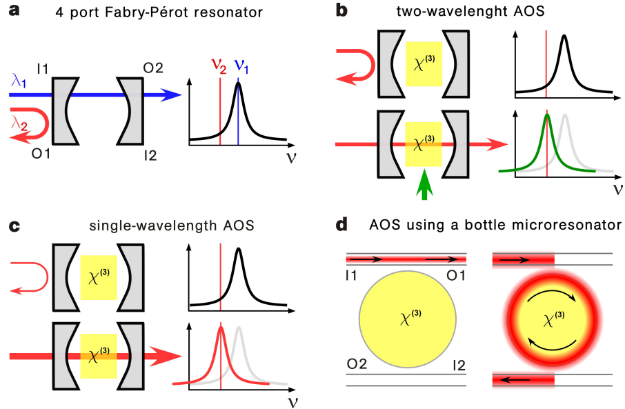
Figure 4.6: Different resonator enhanced all-optical switch schemes. (a) The schemes are illustrated for an FP resonator, which exhibits two input ports ( I1 and I2 ) and two output ports ( O1 and O2 ) and therefore forms an add-drop device comparable to a bottle microresonator coupled to two ultra-thin fibers. A resonant signal at frequency \nu_1 incident into I1 is transmitted through the resonator and thereby transferred to O2 . A signal detuned from resonance at frequency \nu_2 is reflected into O1 . (b–c) By introducing a Kerr material into the FP, a signal beam initially detuned from resonance can be switched between O1 and O2 , employing an intense pump beam or by modulation of the intensity of the signal beam itself. (d) Transfer of the single-wavelength all-optical switching scheme to a bottle microresonator, fabricated from a nonlinear material.
