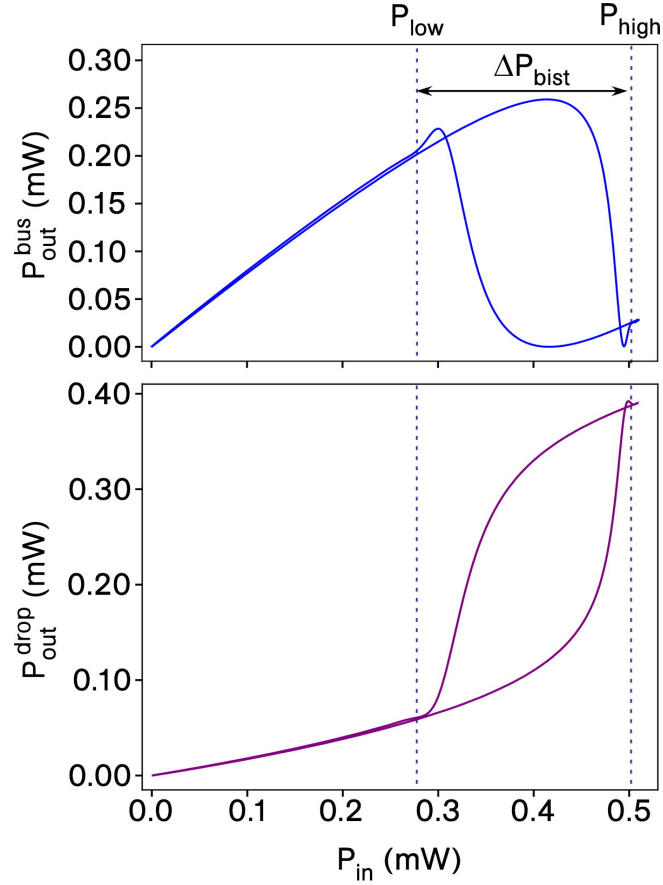
Figure 4.9: (a) P_{out}^{bus} and (b) P_{out}^{drop} as a function of P_{in} . The system shows a pronounced hysteretic behavior and, for a certain range of P_{in} , exhibits two stable states. The bistable regime is defined as the region between the powers P_{low} and P_{high} , where both, P_{out}^{bus} and (b) P_{out}^{drop} , show different values depending on the sign of dP_{in}/dt . Note that the threshold powers, P_1 and P_2 , do not coincide with the borders of the bistable region.
