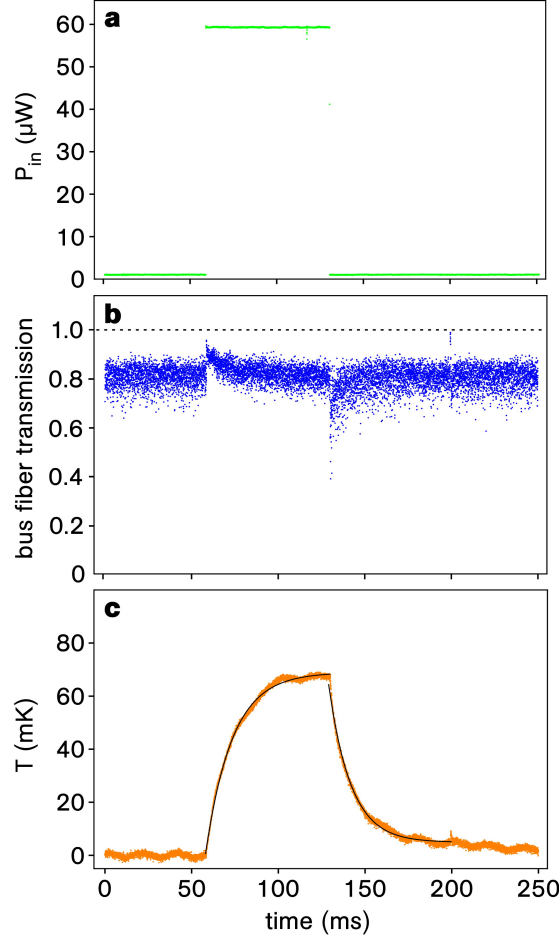
Figure 4.13: Measuring the thermal relaxation time of the mode volume of a q = 2 bottle mode with a linewidth of \Delta\nu_{\text{crit}} = 6.5 MHz. (a) A rectangular 70 ms pulse in P_{\text{in}} heats the mode volume of the bottle mode. This pulse is compensated using a second AOM behind the bus fiber output, so that the photodiode signal detected behind this AOM is proportional to the transmission T = P_{\text{out}}^{\text{bus}}(t)/P_{\text{in}}(t) through the ultra-thin bus fiber waist. This signal is used as the error signal for the PI control loop that keeps the resonator–laser detuning constant. (b) Bus fiber transmission during the measurement calculated from the photodiode signal. In order to obtain the bus fiber transmission, the signal is normalized to its value measured with the bus fiber pulled away from the resonator and the lock disabled. The set point of the lock corresponds to \delta\nu = \Delta\nu_{\text{crit}} and T = 0.8 . The maximum and minimum values of T = 0.95 and T = 0.4 observed reveal, that the PI control loop maintains a laser–resonator detuning between \delta\nu = 2.2 \times \Delta\nu_{\text{crit}} and \delta\nu = 0.4 \times \Delta\nu_{\text{crit}} during the measurement. (c) The temperature of the mode volume, T_{\text{mode}} , as calculated from the control signal fed from the PI control loop to the laser current modulation input. Exponential fits (black curves) yield relaxation time constants of \tau = (15.40 \pm 0.04) ms for the heating of the mode volume, when the pulse is applied, and of \tau = (12.78 \pm 0.05) ms for its cooling, after the pulse. The maximum relative temperature change of approximately 70 mK corresponds to a shift in \nu_0 of 34 \times \Delta\nu_{\text{crit}} .
