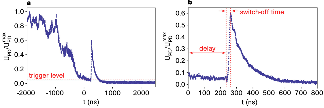
Figure 3.15: Typical cavity-ringdown measurement taken on a 38\text{-}\mu\text{m} diameter bottle microresonator. (a) and (b) show the signal from the photodiode measuring the power transmitted through the bus fiber with its maximum value normalized to unity for different time intervals. The frequency of the probe laser light \nu_{\text{probe}} is swept over a resonance. For t = 0 ns the transmission reaches a value corresponding to the trigger level of the oscilloscope, indicated by the dashed line in (a). The laser power is switched off within 35 ns, see dashed lines in (b), via a TTL pulse sent by the oscilloscope to the AOM driver. The time delay of 240 ns is due to the electronics of the oscilloscope and the AOM driver and the velocity of the acoustic wave travelling in the AOM crystal. After completely switching off the probe laser power, the transmission has partially recovered and then exponentially decays to zero. At critical coupling, the waveguide field and the “cavity leakage field” destructively interfere due to their identical amplitudes and the phase-shift of \pi (see section 3.2.1). After completely switching off the input field, the intracavity intensity can thus be monitored via the cavity leakage field.
