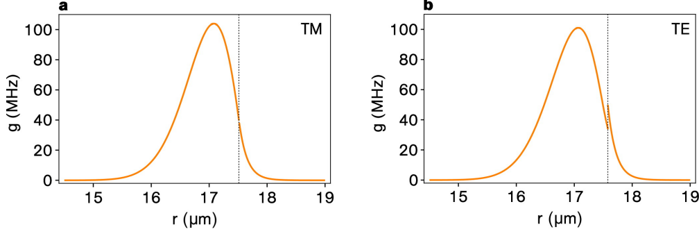
Figure 5.1: Calculated radial dependency of the coupling rate g for the fundamental TM (a) and TE (b) polarized q = 1 bottle modes in a 35- \mu\text{m} diameter resonator.
