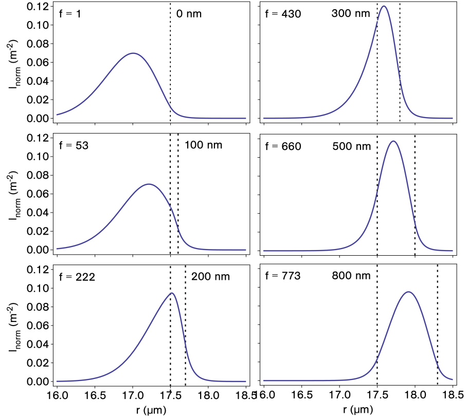
Figure 4.18: Normalized intensity distribution of the fundamental radial modes at wavelengths around 1080 nm in a 35- \mu\text{m} silica WGM resonator coated with a polymer exhibiting a nonlinear refractive index that is 815 times higher than that of the resonator material. The nonlinear refraction is enhanced by a factor f with respect to the uncoated silica resonator.
