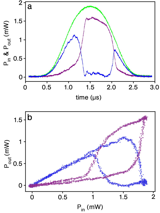
Figure 4.11: Optical bistability in a bottle microresonator. In order to characterize the bistable behavior of bottle modes, the input power is pulsed and the laser frequency is initially detuned from resonance by \delta'_0 = -1.2 \times \Delta\nu_{crit} . (a) Response of the system to a \sin^2 -shaped pulse with a FWHM duration of \tau_{pulse} = 1.25 \mu s (green). The plot shows P_{in} (green), P_{out}^{bus} (blue) and P_{out}^{drop} (purple). As soon as P_{in} exceeds a certain threshold, the light is resonantly switched to the drop fiber via the Kerr effect. (b) By plotting P_{out}^{bus} and P_{out}^{drop} versus P_{in} for the data shown in Fig. 4.11 (a) (identical color coding), bistable behavior is apparent for P_{in} ranging from P_{low} \approx 1.0 mW to P_{high} \approx 1.8 mW.
