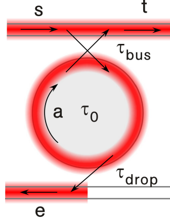
Figure 4.1: A bottle microresonator, coupled to two ultra-thin fibers. The model described in section 3.2.1 is extended by introducing two parameters accounting for the influence of the drop fiber. Its “output field amplitude” is denoted by e and the time constant of the energy transfer between the resonator mode and the drop fiber is \tau_{\text{drop}} .
