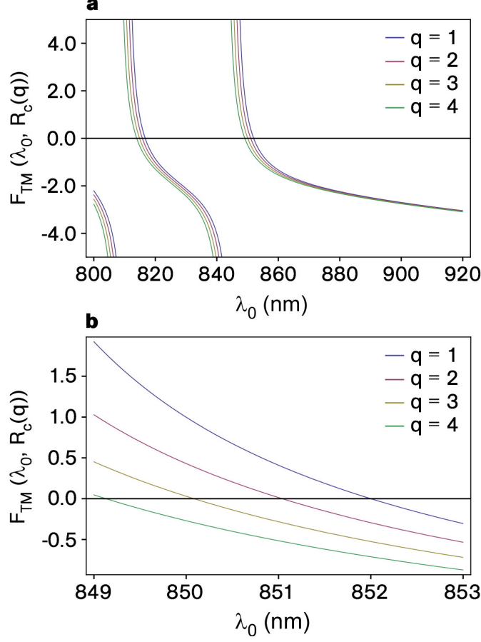
Figure 2.6: Identifying the resonant wavelengths for the four lowest order, TM polarized axial bottle modes. In (a) F_{TM}(\lambda_0, R_c(q)) from Eq. (2.22) is plotted with a fixed radius R_c(q) for each mode. (b) shows a smaller range of \lambda . The roots of each curve mark \lambda_q . The spectral mode spacing \Delta\nu_q is found to be 397 GHz between the two lowest order modes. For the higher order modes, it slightly decreases by approximately 0.1%. This slight deviation from the equidistant mode spacing, expected from the radius profile given in Eq. (2.27) that is used for solving the axial wave equation, is ascribed to the approximation of c_r when solving Eq. (2.34) for R_c(q) .
