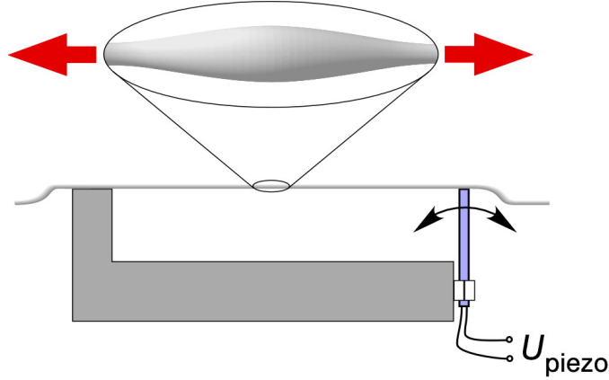
Figure 3.1: Schematic of the fiber holder design used to manipulate both, the ultra-thin fibers and the resonator fiber. The picture illustrates the application of mechanical strain to a bottle microresonator using an integrated piezo-electric bending actuator controlled by a voltage U_{\text{piezo}} . This design enables the tuning of bottle modes and the reduction of the vibration amplitude of the ultra-thin fiber waists.
