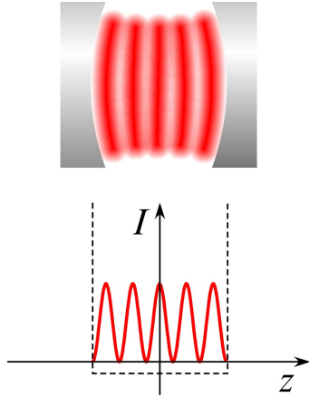
Figure 1.1: Basic principle of a Fabry-Pérot resonator consisting of two highly reflecting mirrors. The cavity mode is a Gaussian beam exhibiting a standing wave structure.
