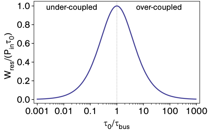
Figure 3.7: Energy stored inside a bottle mode on resonance W_{\text{res}} = |a(\omega = \omega_0)|^2 as a function of \tau_0/\tau_{\text{bus}} . A maximum value of P_{\text{in}} \cdot \tau_0 is reached at critical coupling. This value corresponds to the power incident through the bus fiber integrated during the intrinsic energy storage time \tau_0 .
