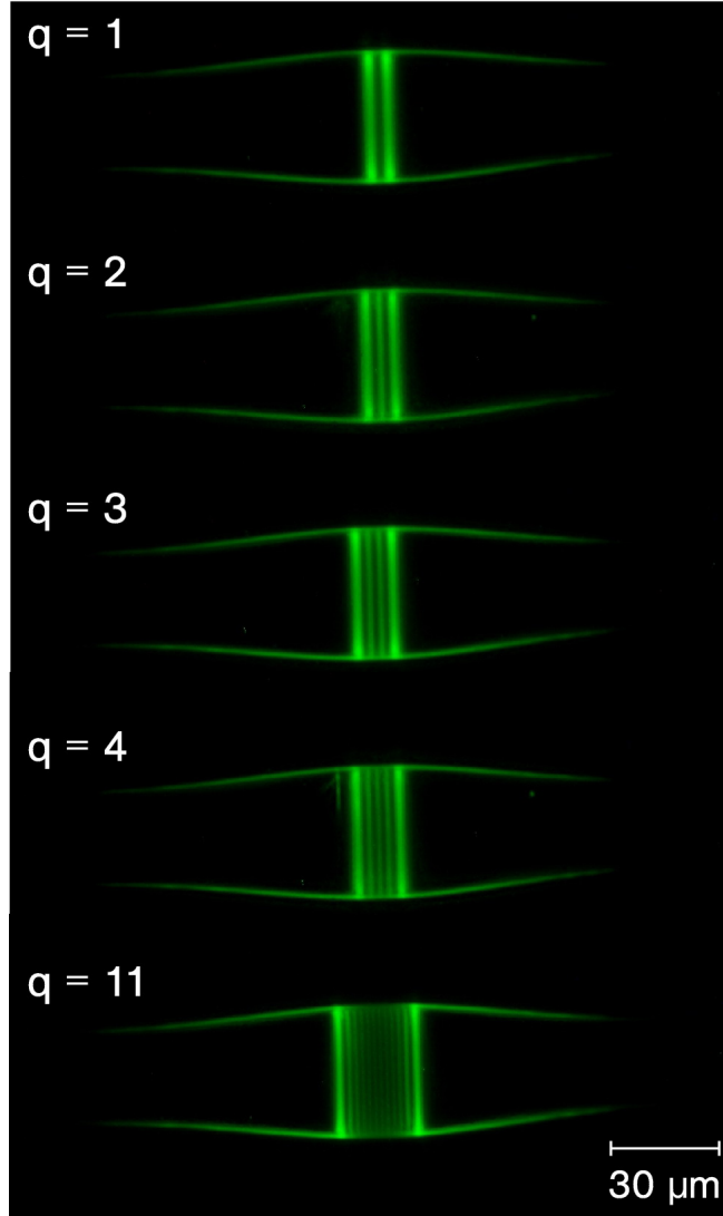
Figure 3.13: Experimental micrographs of the q = 1 – 4 and q = 11 bottle modes visualized via the up-converted green fluorescence of dopant erbium ions in a 36\text{-}\mu\text{m} diameter bottle microresonator.
