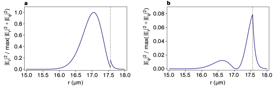
Figure 2.3: |E_r|^2 / \max(|E_r|^2 + |E_\phi|^2) (a) and |E_\phi|^2 / \max(|E_r|^2 + |E_\phi|^2) (b) for the fundamental radial, TE polarized mode. For a wavelength of \lambda_0 = 852 \text{ nm} and m = 180 the resonance condition is fulfilled for a radius of R_c = 17.56 \mu\text{m} . Note the discontinuity of |E_r|^2 at the surface (dashed line). The radial intensity distribution is proportional to |\vec{E}|^2 = |E_r|^2 + |E_\phi|^2 . Both field components, E_r and E_\phi are normalized by dividing them by the maximum value of |\vec{E}| .
