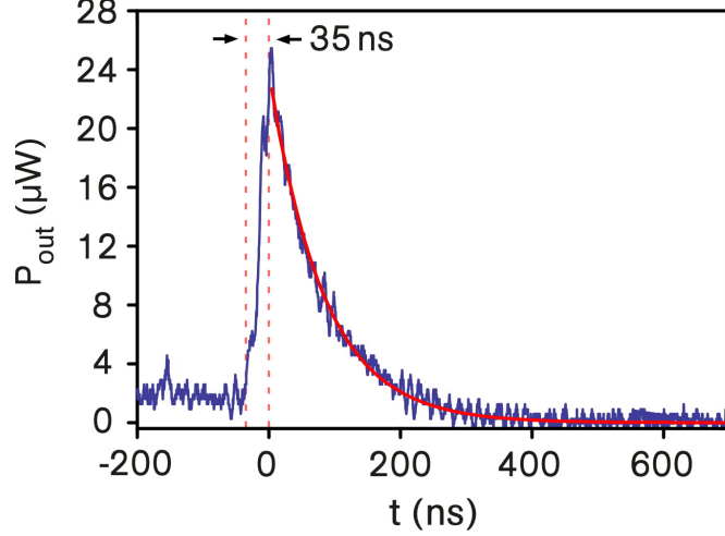
Figure 3.16: Cavity-ringdown measurement of the q = 1 bottle mode in a bottle microresonator with a diameter of 35 \mu\text{m} and a curvature of \Delta k = 0.012 \mu\text{m}^{-1} . The measurement was performed at critical coupling for a wavelength near 850 \text{ nm} and transverse electric (TE) polarization. The exponential fit (red line) according to Eq. (3.36) yields \tau_{\text{crit}} = (82 \pm 0.45) \text{ ns} .
