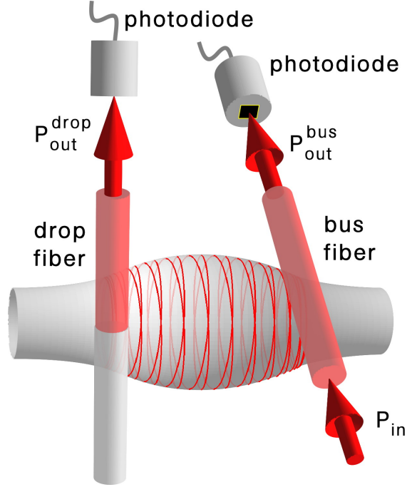
Figure 3.3: Schematic of the coupling setup in add-drop configuration. Two ultra-thin fiber couplers are placed at both caustics of the bottle microresonator. Depending on its frequency, light propagating in the bus fiber is selectively coupled into the resonator mode and exits the resonator through a second ultra-thin fiber, referred to as the drop fiber. The optical powers at the output of the bus fiber P_{\text{out}}^{\text{bus}} and the drop fiber P_{\text{out}}^{\text{drop}} are measured using two photodiodes. The red line indicates a possible path of a light ray in the bottle microresonator.
