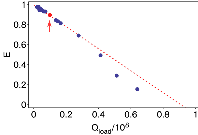
Figure 4.3: Power transfer efficiency between both fiber waists at the critical coupling point as a function of Q_{\text{load}} . The data shows close agreement with the theoretical linear prediction, however, for high loaded quality factors, a slight modal splitting is observed, leading to an underestimation of the quality factor. Excluding the three rightmost data points, a fit of Eq. (4.7) (blue line) yields an intrinsic quality factor of Q_0 = 1.8 \times 10^8 . The red arrow indicates the data point extracted from the measurement shown in Fig. 4.2.
