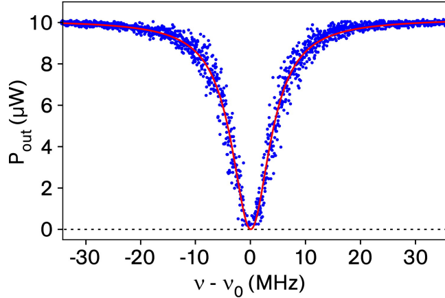
Figure 3.8: Spectrum of a bottle mode with q = 2 in a 36\text{-}\mu\text{m} diameter resonator. A Lorentzian fit (red line) shows close agreement with the measured line shape. From the fit one obtains \Delta\nu = 8.5 MHz and T_{\text{res}} < 1\% . The measured line shape corresponds to a quality factor of Q_{\text{crit}} = 4.1 \times 10^7 .
