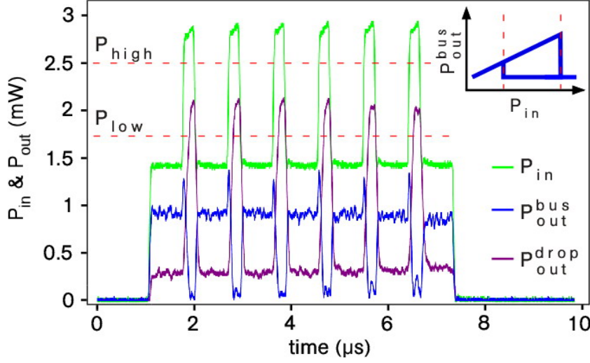
Figure 4.16: Demonstration of all-optical routing using the optical Kerr bistability in a bottle microresonator. P_{in} is varied between two levels which are located below and above the bistable regime, delimited by P_{low} and P_{high} , (schematically indicated by the dashed lines) as shown in the inset. At the same time, the power at the outputs of the bus fiber and the drop fiber is monitored. As soon as the input power exceeds P_{high} , 70% of the incident light is transferred to the output of the drop fiber. Lowering the input power below P_{low} , again reverses the situation at the outputs.
