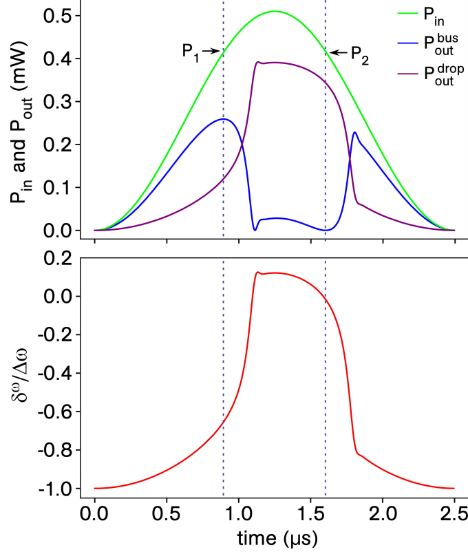
Figure 4.8: (a) P_{\text{out}}^{\text{bus}} and P_{\text{out}}^{\text{drop}} modelled for a \sin^2 -shaped pulse of the input power P_{\text{in}} . A resonator with parameters Q_0 = 1.8 \times 10^8 , Q_{\text{load}} = 1.7 \times 10^7 and V = 1000 \mu\text{m}^3 is assumed. (b) Evolution of the laser-resonator detuning \delta\omega . The cold laser-resonator detuning at t = 0 has a value of \delta_0^\omega = -\Delta\omega_{\text{crit}} . When P_{\text{in}} exceeds a threshold P_1 , d\delta\omega/dP_{\text{in}} reaches a critical value and the Kerr effect “pulls” the resonator mode into resonance with the laser frequency. At the peak value of P_{\text{in}} , the detuning reaches positive values. When P_{\text{in}} decreases again, at a power P_2 , the intracavity intensity ( \propto P_{\text{out}}^{\text{drop}} ) has sufficiently decreased to reach zero detuning. From this point onward, the resonator rapidly returns to the initial situation. The exact values of the threshold powers are defined by dP_{\text{out}}^{\text{bus}}/dP_{\text{in}} = 0 . Between the two switching events, the transmission through the bus fiber is strongly reduced due to critical coupling. At the same time, due to the near-zero values of \delta\omega , the intracavity power is high and a large fraction of P_{\text{in}} is transferred to the drop fiber output.
