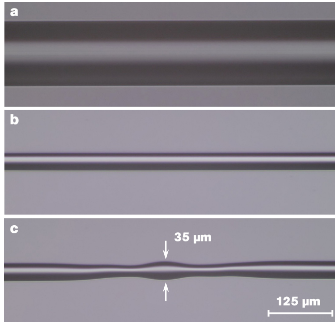
Figure 2.10: Micrographs showing the fabrication of a typical bottle microresonator in 2 steps, starting from a commercial 125- \mu\text{m} diameter optical step-index fiber (a). (b) First, a section with a homogeneous diameter of 35 \mu\text{m} is created by simultaneously heating and stretching the fiber. (c) Next, local heating by a focused \text{CO}_2 -laser beam and simultaneous elongation creates two microtapers on the fiber waist separated by approximately 150 \mu\text{m} . The bulge between the microtapers forms a bottle microresonator of radius D_0 = 35 \mu\text{m} .
