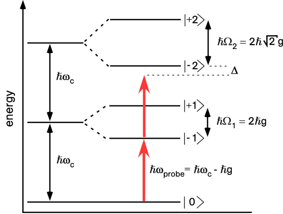
Figure 5.5: Ladder of eigenstates of a strongly coupled atom-cavity system, as predicted by the Jaynes-Cummings model in the case of \omega_c = \omega_a = \omega . The ground state corresponds to the bare atom-cavity system. By absorbing one/two photons the system is transferred to the first/second excited state. The Rabi splitting \hbar\Omega_n = 2\hbar\sqrt{n}g of the excited states depends on the photon number n . In contrast to a bare cavity with a constant energy spacing of \hbar\omega_c between adjacent modes, the energy levels of the coupled system exhibit distinct spacings, giving rise to single-photon nonlinearities. For a probe beam with frequency \omega_{\text{probe}} = \omega_c - g , absorption of one photon leads to a detuning of \Delta from the next resonance of the coupled atom-cavity system.
