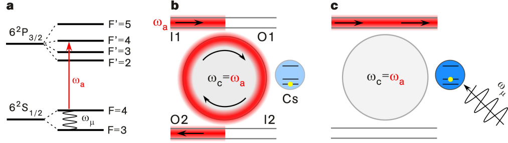
Figure 5.4: Schematic of the “single-atom beamsplitter”. (a) Simplified energy level scheme of ^{133}\text{Cs} . The cesium atom can be switched between the F = 3 and F = 4 hyperfine ground states using microwave radiation at a frequency of \omega_\mu = 2\pi \times 9.2 GHz. Exposure of the atom, originally in the F = 3 state, to a resonant microwave \pi pulse, transfers the atom into the F = 4 state which then couples to a light field (red arrow) with frequency \omega_a , resonant with the ( F = 4 \rightarrow F' = 4 ) transition. (b-c) A weak light field with frequency \omega_a is coupled into one of the input ports (I1) of the bottle microresonator in add-drop configuration. The resonance frequency \omega_c of the bottle mode is also stabilized to the frequency of the atomic transition \omega_a . The possibility of on- and off-switching of the interaction between the bottle mode and the atom by a microwave pulse enables routing of the input light field between both fiber outputs (O1 and O2). (b) If the atom is in the F = 3 state, the coupling rate between the atom and the resonator mode is zero. In this case, the input light field is resonantly coupled to the resonator mode and is thus transferred to output O2. (c) As soon as the atom is excited to the F = 4 state, it strongly couples to the bottle mode. The resonance frequencies of the eigenmodes of the strongly coupled atom-cavity system are now detuned from \omega_a , see Fig. 5.3 (b). The input light field can no longer enter the cavity and is transmitted through the bus fiber.
