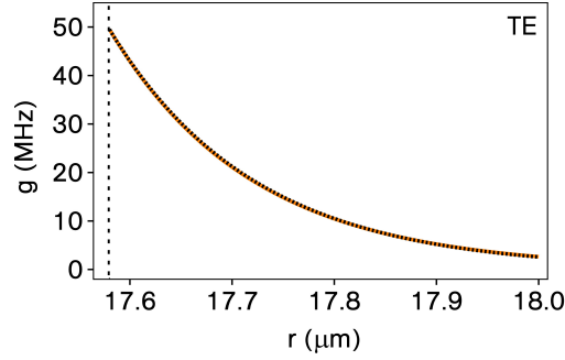
Figure 5.2: Spatial variation of the coupling rate close to the resonator surface for the TE polarized mode from Fig. 5.1 (b). At the surface, (vertical, dashed line) g has a maximum value of g_{\text{surf}} = 2\pi \cdot 50.0 MHz which decreases with the distance from the surface d . For the given parameters, an exponential decay, according to g(d) = g_{\text{surf}} \cdot \exp(-d/d_0) , with spatial decay length d_0 = 142 nm (dashed, black line) is a good approximation of the result of the rigorous calculation in the region of interest given by a Bessel function.
