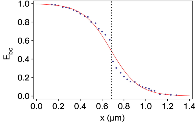
Figure 3.11: Dependency of E_{bc} on the width x of the coupling gap. In the under-coupled regime almost all of the light stored inside the mode is dissipated and E_{bc} exhibits values close to zero. For critical coupling (indicated by the vertical dashed line) a value of E_{bc} = 0.5 is reached. In the over-coupled regime, \kappa_{bus} becomes much larger than \kappa_0 and \kappa_{para} and a maximum value of E_{bc} = 0.99 is measured. The red line corresponds to the values obtained for K from the fit in Fig. 3.10.
