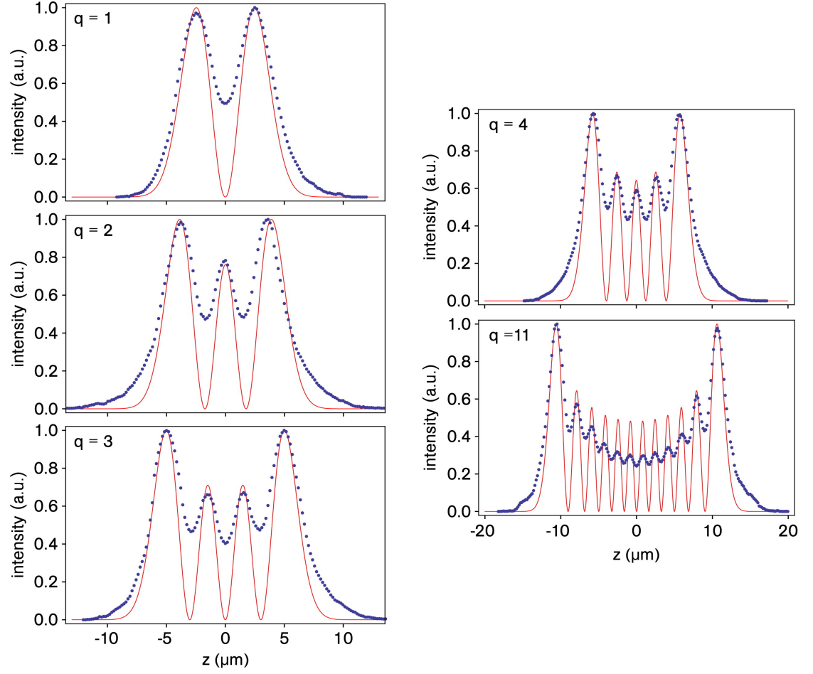
Figure 3.14: Fluorescence intensity along resonator axis (blue dots), extracted from Fig. 3.13, plotted together with the calculated intensity distribution of the mode guiding the pump light at a wavelength of 850 nm (red lines). Both intensities are normalized to unity for better comparability.
