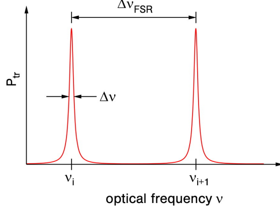
Figure 1.2: Mode spectrum of a Fabry-Pérot resonator. The power transmitted through the cavity P_{tr} as a function of the optical frequency of the input light field is given by an Airy function. The signal transmitted through the cavity is proportional to the intracavity intensity. The individual peaks of FWHM \Delta\nu , corresponding to the modes of the resonator, are separated by the free spectral range \Delta\nu_{FSR} .
