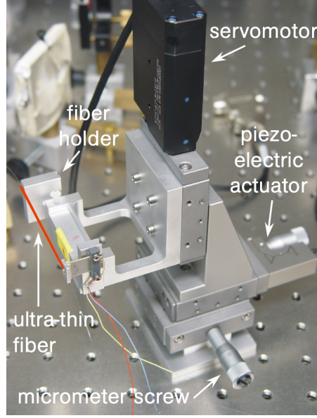
Figure 3.2: Mechanical system used for positioning an ultra-thin optical fiber (indicated by the red line). Three orthogonally oriented stages driven by a piezo-electric actuator, a servomotor and a micrometer screw are used to place the ultra-thin fiber at one of the caustics of the bottle microresonator.
