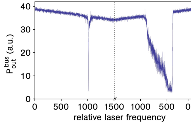
Figure 4.4: Thermal bistability in a bottle microresonator. Depending on the sign of d\nu_{\text{probe}}/dt , the transmission T(\nu_{\text{probe}}) shows two distinct values for a given frequency \nu_{\text{probe}} . For d\nu_{\text{probe}}/dt < 0 (right side of the graph) the resonance frequency shift due to heating of the mode volume by absorption has the same sign as the change of the laser frequency. The resonance frequency is therefore pulled along with the laser frequency scan causing a broadening of the line shape. In contrast, a scan over the same frequency range with d\nu_{\text{probe}}/dt > 0 (left side of the graph) shows a reduction of the linewidth with respect to the line shape measured for powers P_{\text{in}} below the threshold of thermal bistability.
