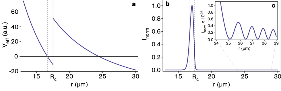
Figure 2.4: (a) Considering the form of the radial wave equation one can define an effective potential for the light confined in a resonator mode. The plot shows V_{\text{eff}} for m_{\text{max}} = 180 in a bottle microresonator with R_c \approx 17.49 \mu\text{m} for a wavelength of 852 nm. (b) Normalized radial intensity distribution I_{\text{norm}} = |E_z|^2 / \max(|E_z|^2) of the corresponding TM mode. The mode is located in the region V_{\text{eff}} \leq 0 , whereas for V_{\text{eff}} > 0 the fields are purely evanescent. (c) For larger radii of approximately 25 \mu\text{m} , V_{\text{eff}} again becomes positive and gives rise to an unbound, propagating light field. Note the scaling factor of 10^{26} between (b) and (c). Due the rapid exponential decay of the intensity outside of the silica resonator structure the losses due to coupling of the confined fields to the radiating modes are negligible in this case.
