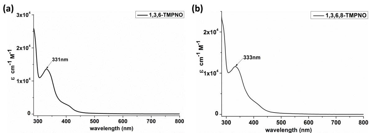
Figure 5.16: UV-Vis spectrum of 1,3,6-TMPNO and 1,3,6,8-TMPNO.
