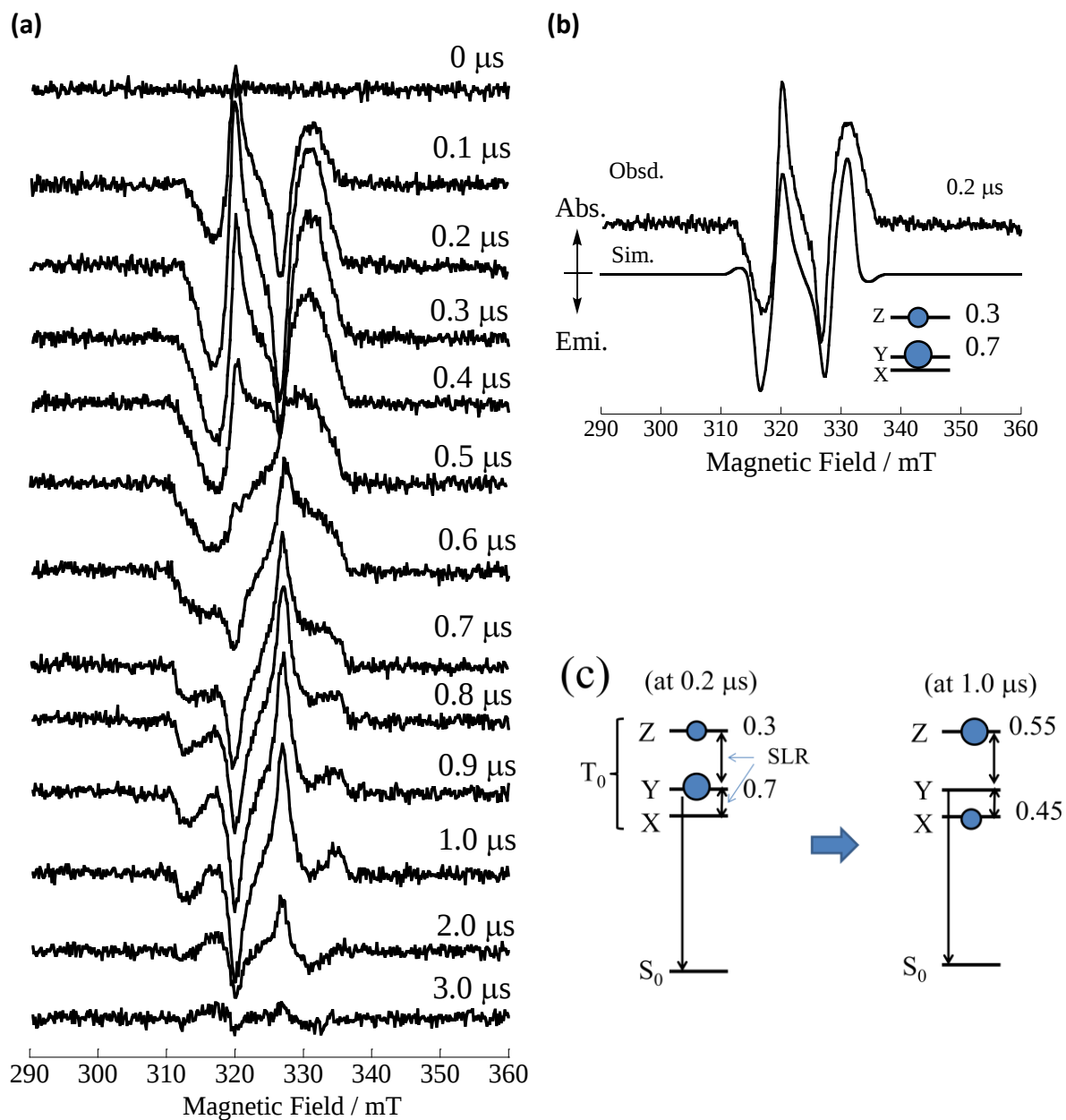
Figure 6.15: (a) Time dependence of TREPR spectra of 2,7-TMPNO (b) observed and simulated TREPR spectra at 30 K on 0.2 \mu s after photo-excitation, (c) relative population change. The relative populations to give the spectral simulation have changed to 0.45, 0 and 0.55 at 1.0 \mu s, which indicates the Y spin-sublevels being more allowed to the S_0 state.
