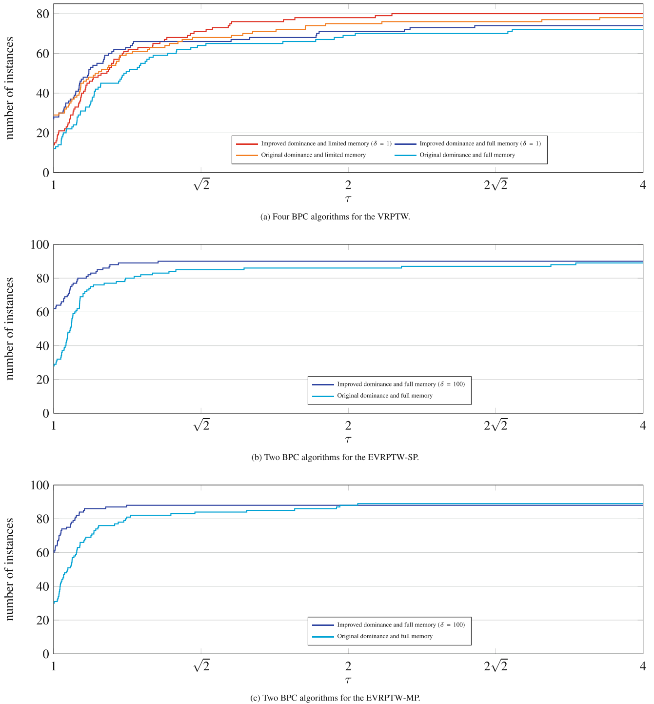
FIGURE 4 | Performance profiles of BPC algorithms using either the original or improved dominance.
