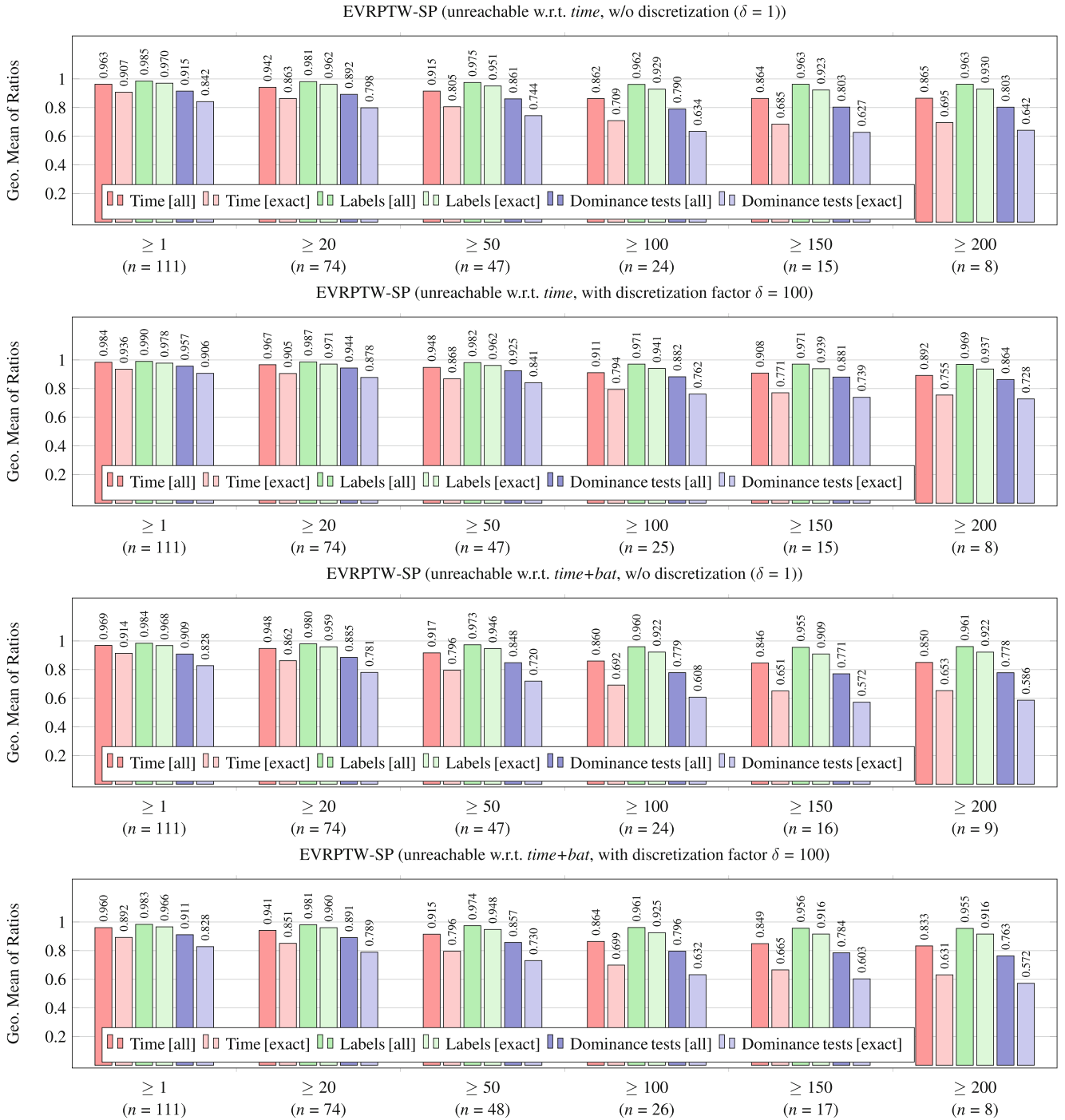
FIGURE 2 | Geometric mean of the computation time ratios, number of generated labels, and number of dominance tests performed; we distinguish between all pricing iterations (partial and exact: [all]) and iterations with exact pricing using the complete network ([exact]); results are grouped by \geq n_{SRI} where only instances for which the total number of added SRIs is at least n_{SRI} are considered. The four diagrams show results using attributes time and time+bat to define unreachable customers as well as results without discretization and with discretization using the factor \delta = 100 .
