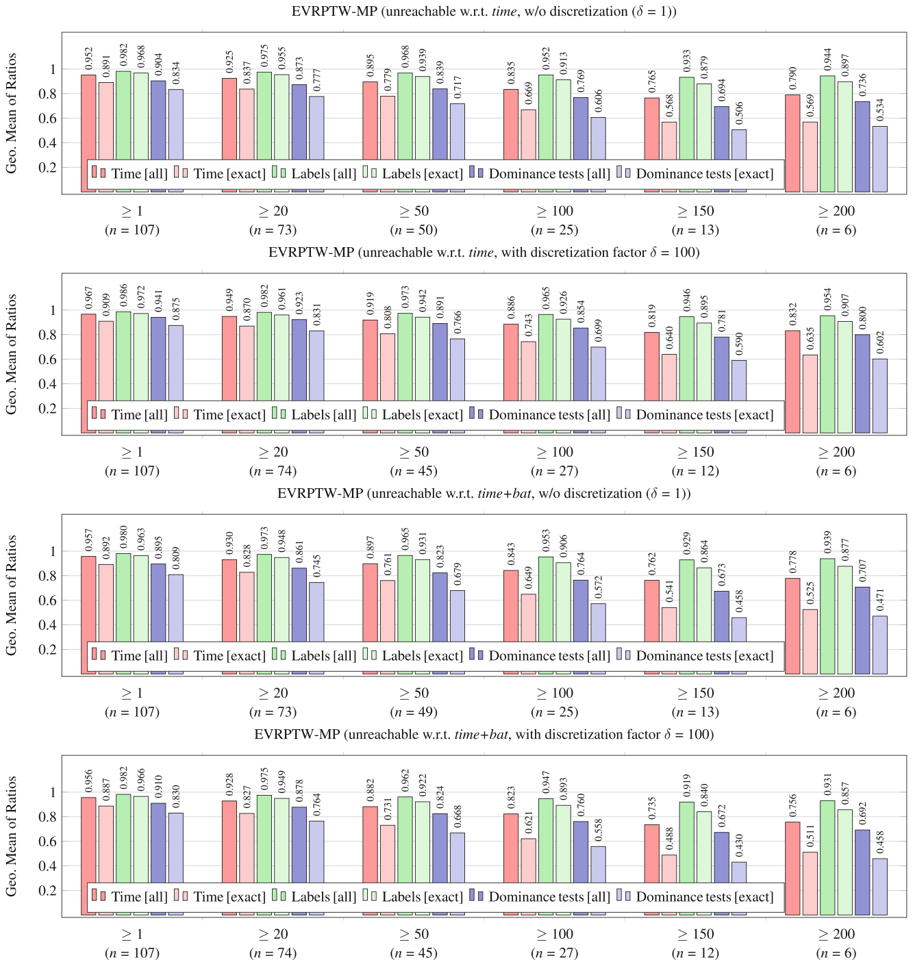
FIGURE 3 | Geometric mean of the computation time ratios, number of generated labels, and number of dominance tests performed; we distinguish between all pricing iterations (partial and exact: [all]) and iterations with exact pricing using the complete network ([exact]); results are grouped by \geq n_{SRI} where only instances for which the total number of added SRIs is at least n_{SRI} are considered. The four diagrams show results using attributes time and time+bat to define unreachable customers as well as results without discretization and with discretization using the factor \delta = 100 .
