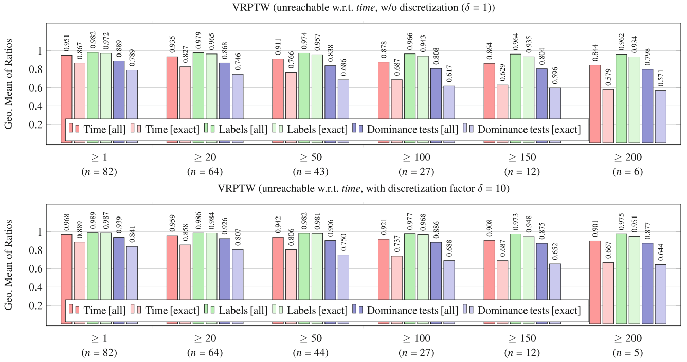
FIGURE 1 | Geometric mean of the computation time ratios, number of generated labels, and number of dominance tests performed; we distinguish between all pricing iterations (partial and exact: [all]) and iterations with exact pricing using the complete network ([exact]); results are grouped by \geq n_{SRI} where only instances for which the total number of added SRIs is at least n_{SRI} are considered. The upper and lower diagrams show results without discretization and with discretization using the factor \delta = 10 , respectively.
