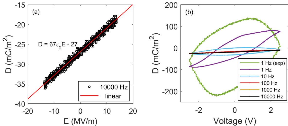
Figure 6.7. (a) Experimental electric displacement of the MAPbI 3 -based capacitor as a function of electric field at frequency of 10 kHz. (b) D - V characteristics calculated with the high frequency apparent dielectric constant of 67\epsilon_0 . Also shown is the experimental displacement loop at 1 Hz for comparison (green symbols).
