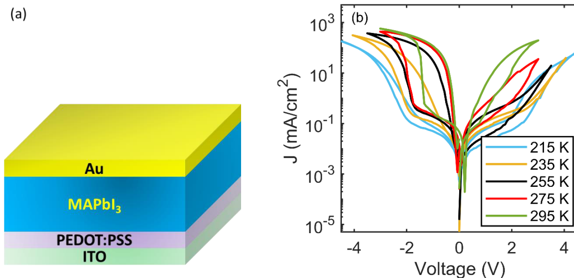
Figure 2.16. (a) Device structure and (b) temperature dependence of hole current in ITO/PEDOT:PSS/MAPbI 3 /Au hole-only device.
