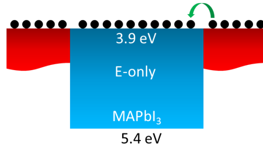
Figure 2.6. Schematic of a MAPbI 3 electron-only device. The schematic exhibits that for efficient electron injection the E_f ( E_c ) of the conductive (semiconductor) injecting contact has to be close the E_c of MAPbI 3 (-3.9 eV).
