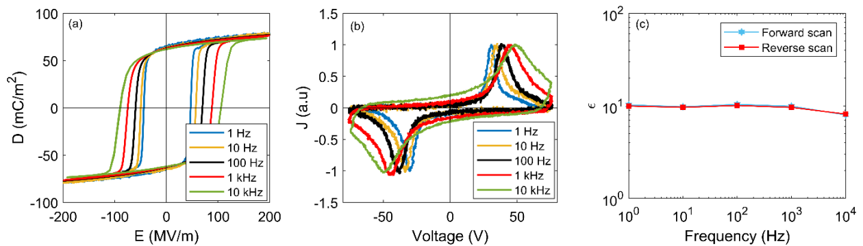
Figure 4.1. (a) D-E and (b) J-V loops of a P(VDF-TrFE) ferroelectric capacitor at different frequencies ranging from 1 Hz to 10 kHz. (c) Dielectric constant of P(VDF-TrFE) obtained from D-E loops as a function of frequency.
