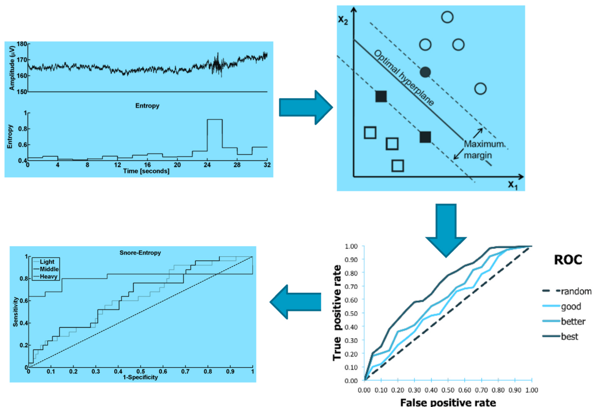
Fig. 1. Analysis Pipeline of data extraction and SVM analysis; ROC= Receiver Operating Curve.
