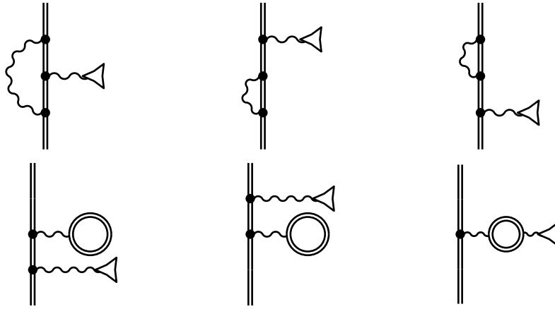
Figure 2.3: Feynman diagrams of BS-QED in first order of \alpha . The double line depicts the BS-QED electron propagator. Additional to the direct analogons to the free electron g -factor, 4 causal permutations have to be considered that were already included in the mass and charge renormalization of the electron propagator for the free electron.
