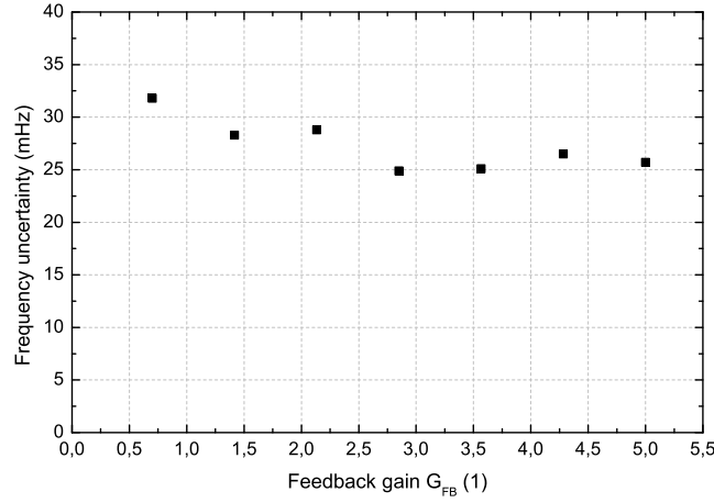
Figure 5.3: The linesplitting performance is roughly independent of the feedback gain, as the increase in the SNR is mostly canceled by the simultaneously increasing linewidth. This demonstrates that the particle can be cooled with noise feedback without sacrificing linesplitting precision.
