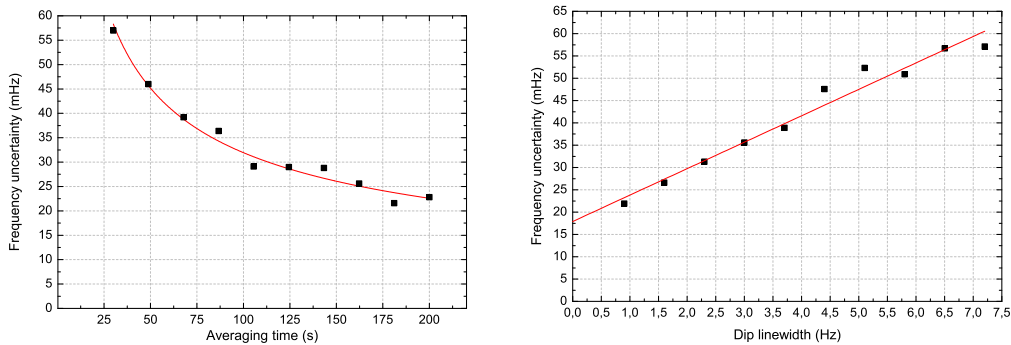
Figure 5.2: Standard deviation of the frequency value determined by a fit to artificially generated Monte Carlo spectra using typical parameters of a ^{28}\text{Si}^{13+} ion in the PT. The determinability improves with \frac{1}{\sqrt{T}} (left) and directly reflects the entropy of the incoherent signal. For averaging durations up to 60 s this line-splitting determines entirely the axial frequency resolution. The precision can be improved by decreasing the linewidth of the dip (right) for example via decoupling the ion from the tank circuit.
