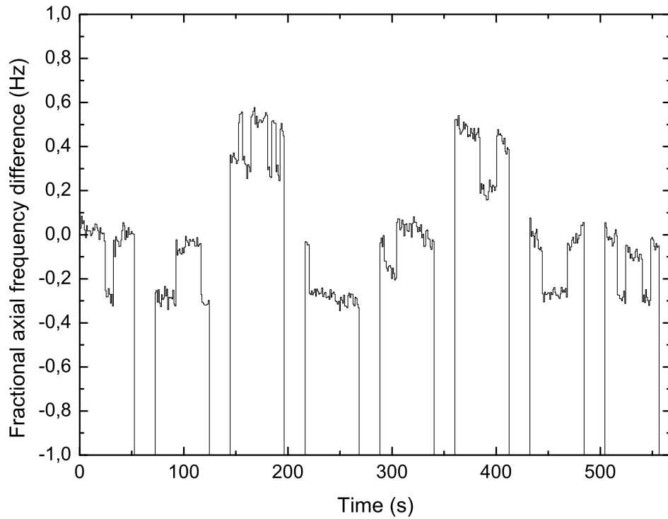
Figure 5.18: Spin state detection in the AT with intermittent transports to the PT, where the narrow spin transition is probed with a microwave excitation. Spinflips can be detected by observing the spin state before and after the stay in the PT. The random frequency offset between successive AT measurements originates from the Boltzmann distribution of cyclotron energies after sideband cooling.
