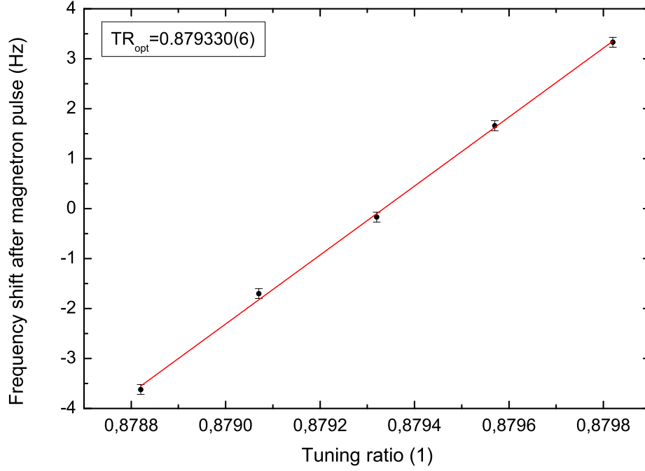
Figure 4.5: Optimization of the tuning ratio with the magnetron burst technique. The linear dependence of the frequency shift between hot and cold ions is clearly visible. The tuning ratio can be deduced with a linear regression, yielding T_{\text{opt}} = 0.879330(6) .
