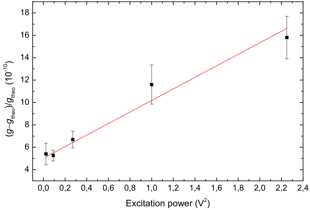
Figure 6.8: Individual g -factor values determined from the centroids of the eight recorded resonances. For centroids with identical excitation energy, the weighted average value is plotted.
