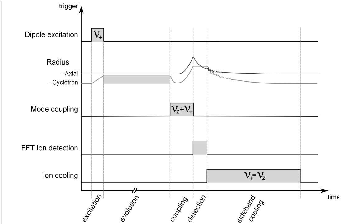
Figure 5.7: Pulse diagram for the PnA cyclotron frequency detection technique. The phase is determined by coupling the motion of two modes, in this case the axial and cyclotron mode, with a pulse on the blue cyclotron sideband. This causes both coupled mode radii to increase exponentially, encoding the initial cyclotron phase in the axial motion. After the amplification pulse, the axial signal can be read out with an arbitrary SNR.
