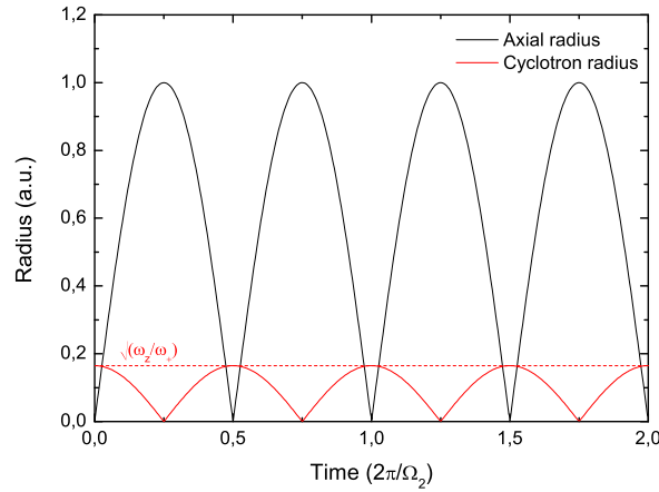
Figure 3.7: Exemplarily evolution of the mode radii with resonant excitation at the lower cyclotron sideband \omega_2 . The behavior is a classical analog to Rabi oscillations between the two coupled modes.
