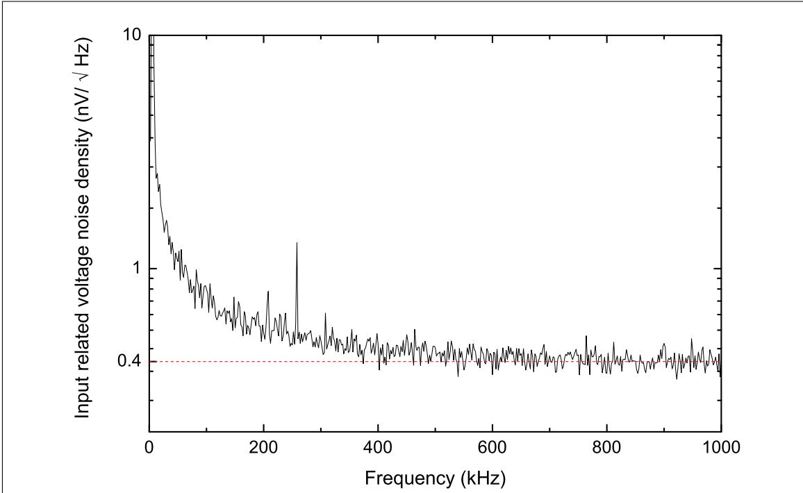
Figure 4.12: Voltage-noise density of the cryogenic amplifier, measured with shorted input at liquid helium temperature. The flicker noise corner is at roughly 350 kHz, below the lowest detected frequency in the current experiment.
