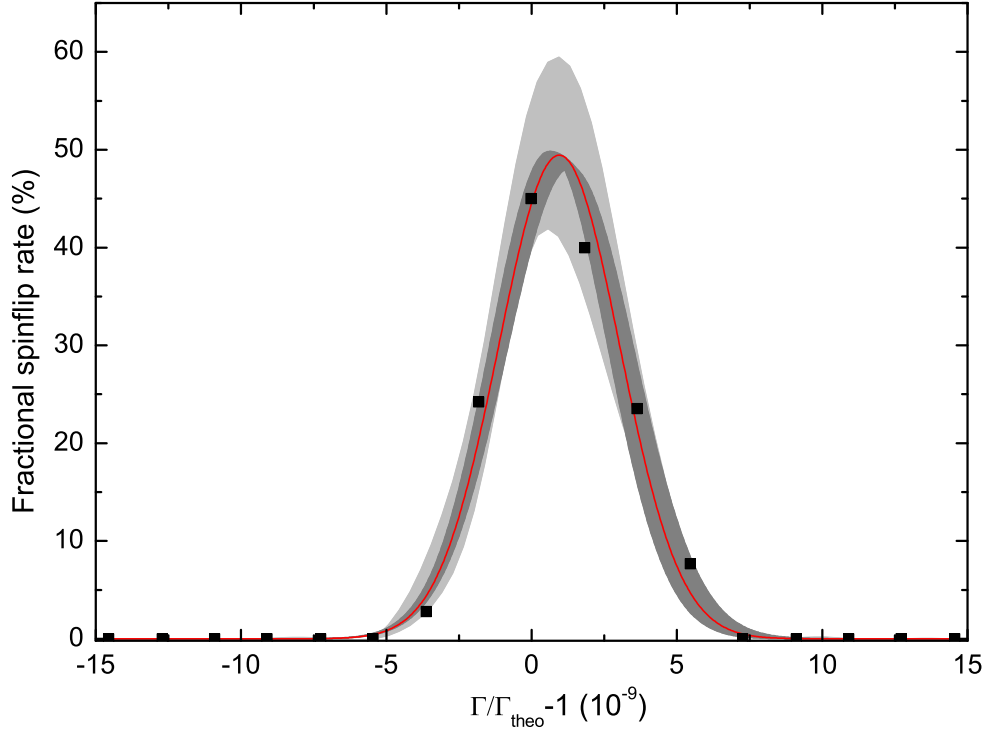
Figure 6.1: One of the 6 recorded resonances with the double-dip detection technique. Compared to previous g -factor experiments the linewidth is significantly smaller and the resonance shows no asymmetry. The relative precision obtainable from this resonance is about \delta g/g = 0.4 ppb. Corrections for systematic shifts arising from the interaction with the cavity are not included in the resonance. The dark gray area represents the 1\text{-}\sigma prediction band for the measurements, while the dark gray region displays the confidence band of the fit with respect to the centroid parameter. The data points are merely plotted for visualization and do not enter the fitting procedure.
