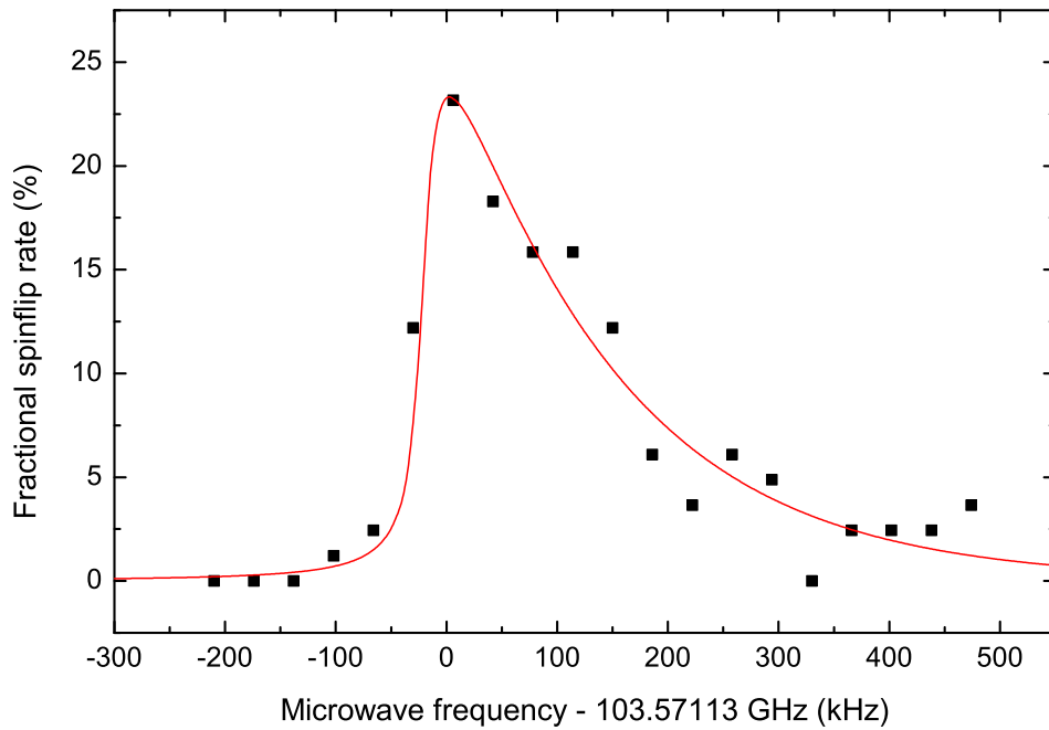
Figure 5.17: Resonance of the spin transition recorded in the strong magnetic bottle of the analysis trap. The red line is the theoretical prediction according to the line-shape model taken from the Ph.D. thesis of J. Verdú [34], with only the microwave power and the centroid as free parameters. The asymmetry due to the Boltzmann distribution of axial energies in the magnetic bottle is clearly visible, yielding a fractional linewidth of roughly 1 ppm. In combination with feedback cooling and appropriate cyclotron frequency detection a measurement of the g -factor directly in the AT with a fractional uncertainty of roughly 10 ppb becomes possible.
