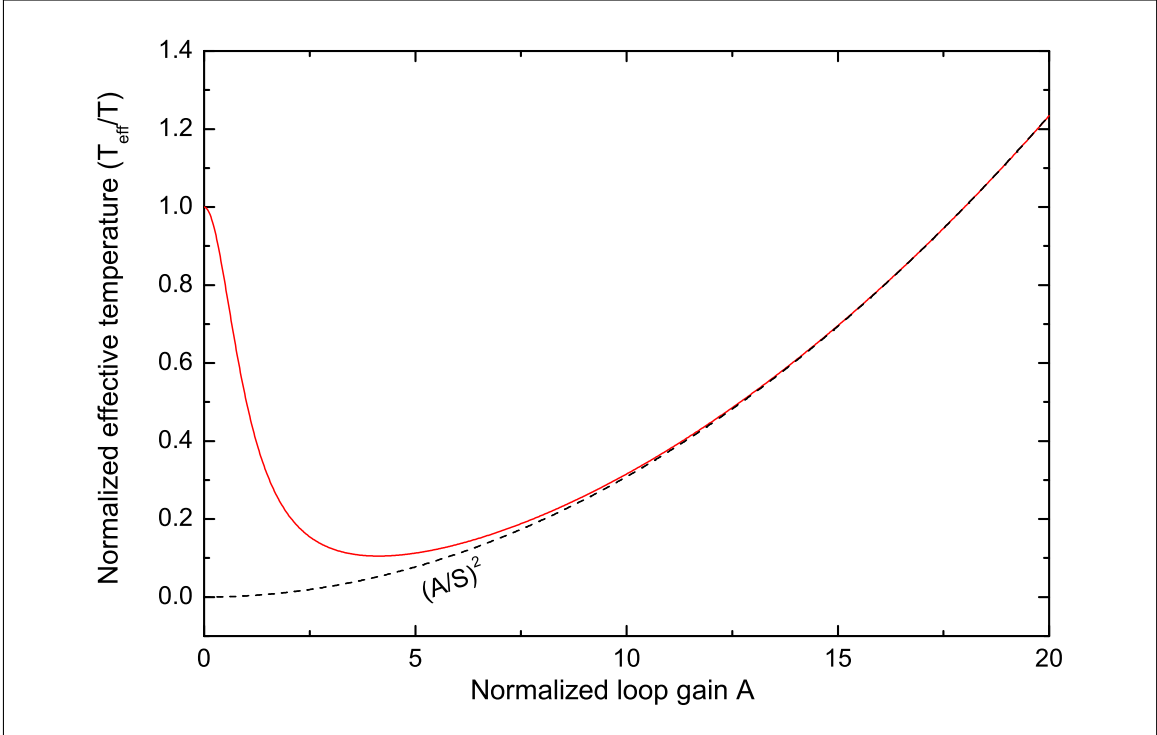
Figure 4.15: Normalized temperature of the ion in thermal equilibrium with the tank circuit with negative electronic feedback. The temperature decreases monotonically with increasing feedback gain, until a minimum value, depending only on the initial SNR, is reached. If the feedback is increased beyond that point only electronic noise is added and the temperature rises.
