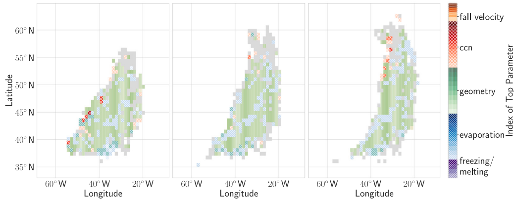
Fig. 11. The top parameters for specific humidity at 900 hPa ≤ p < 1000 hPa, between 1 h ≤ t < 2 h, 7 h ≤ t < 8 h, and between 13 h ≤ t < 14 h (from left to right) after the first trajectory started its ascent. Cells are colored according to the parameter that most frequently occurs within the leading order of magnitude in the given bin, where the magnitude is calculated for each trajectory. The gray outline shows the total area covered by our simulation within these time periods.
