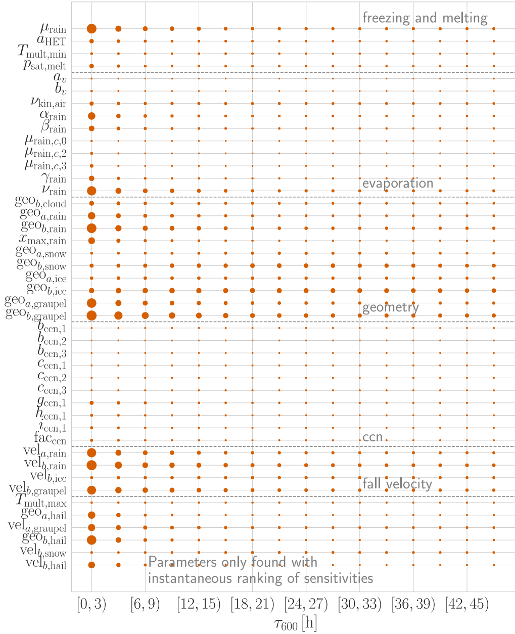
Fig. 13. Mean gradients \overline{|\zeta_{r,j,h}^2|} for latent heating with different ascent timescales ( \tau_{600} ) of the trajectories. The size of the markers is proportional to the mean of each gradient.
