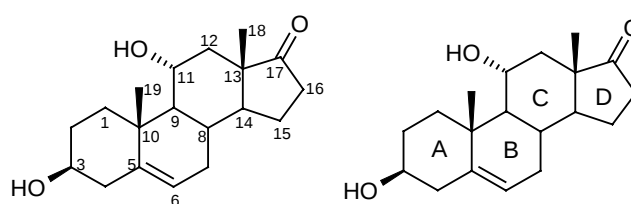
Steroid 131
