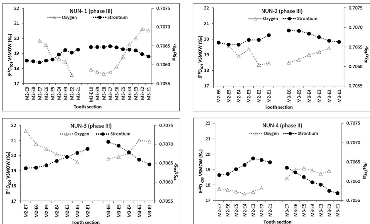
Fig. 6. Plots a–d demonstrate intra-tooth isotope values of ^{87}\text{Sr}/^{86}\text{Sr} (solid circles) and \delta^{18}\text{O}_{\text{Co}3} (open triangles) for M2 and M3s of each of the caribou analysed. Plot a, b and c represent the phase III individuals NUN-1, -2 and -3, respectively. Plot d represents the phase II individual NUN-4. Analytical error for strontium measurements is within the symbol markers.
