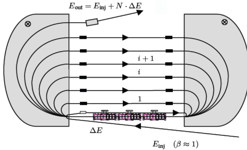
Figure 3.2: Schematic of a racetrack microtron (RTM) [74].
