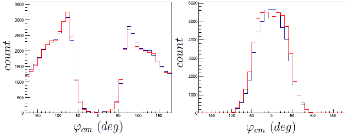
Figure 4.24: (Left) setting LOW \varphi_{cm} distributions from VCSSIM (blue) and from the experiment (red) with fixed normalizations at q'_{cm} = 37.5 \text{ (MeV}/c) . (Right) setting INP \varphi_{cm} distributions, at q'_{cm} = 112.5 \text{ (MeV}/c) , when one considers a GP effect in VCSSIM (blue).
