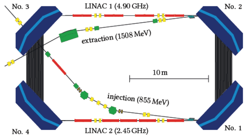
Figure 3.3: Schematic of a harmonic double-sided microtron (HDSM) [74].
