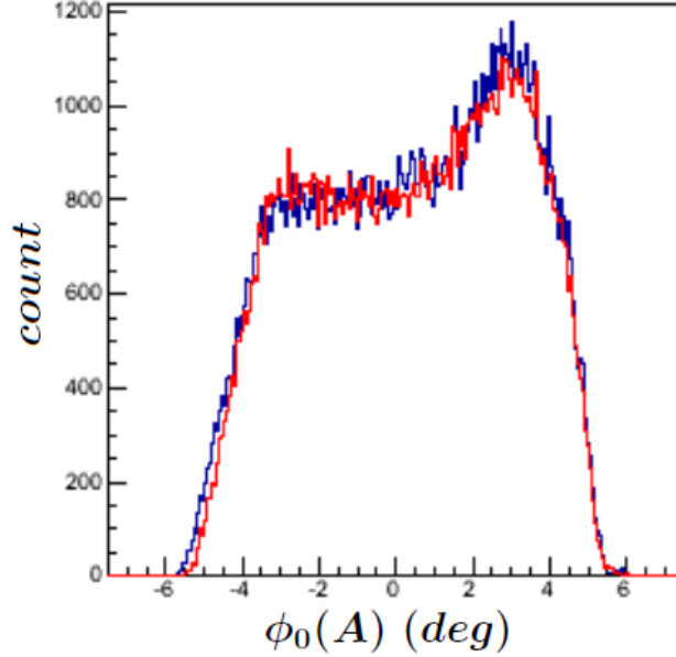
Figure 4.22: \phi_0 angle reconstructed by spectrometer A at q'_{cm} = 87.5 \text{ MeV}/c for the INP setting. A small disagreement is found on the left edge of the distributions.
