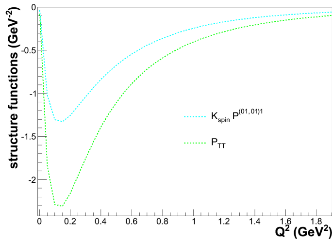
Figure B.1: DR model predicted value of K_{spin} P^{(01,01)1}(q_{cm}) and P_{TT} .
