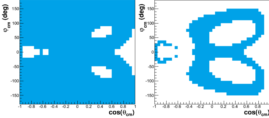
Figure 5.16: Bins (in blue) that satisfy the mask selection in the (\varphi_{cm}, \cos(\theta_{cm})) -plane when K_{thr} = 2.5\% , P_{LL} - P_{TT}/\epsilon = 17.9 ( GeV^{-2} ) and P_{LT} = -3.7 ( GeV^{-2} ) at q'_{cm} = 87.5 MeV/c (left) and q'_{cm} = 112.5 MeV/c (right).
