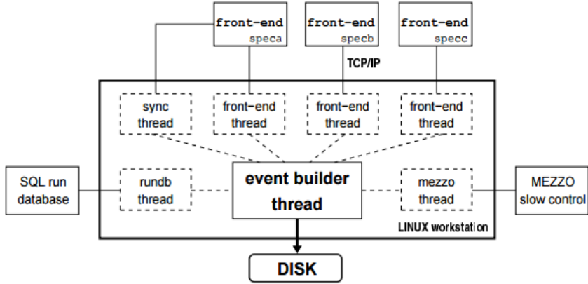
Figure 3.9: Schematic view of the Aqua++ event builder threads, from [79].
