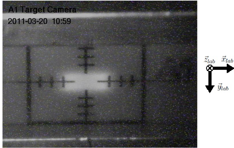
Figure 4.7: Snapshot of the aluminum screen hit by the beam. The composition of the screen makes it glow where the electrons strike it. The bright rectangle shows the wobbler size in horizontal ( x ) and vertical ( y ); here (\pm 2 \text{ mm})(\pm 1 \text{ mm}) .
