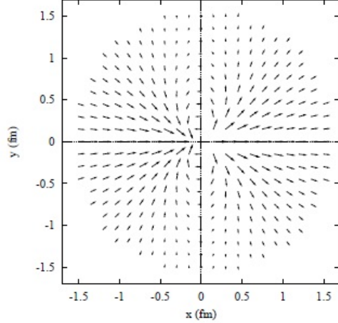
Figure 1.4: Nucleon polarization induced by an electric field along the x axis, calculated in the framework of HB \chi PT O(p^3) . Figure taken from [29].
