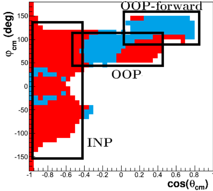
Figure 5.17: Bins, in blue, that satisfy the mask selection in the (\varphi_{cm}, \cos(\theta_{cm})) -plane at q'_{cm} = 112.5 MeV/c . The bins in red contain data that are rejected by this selection.
