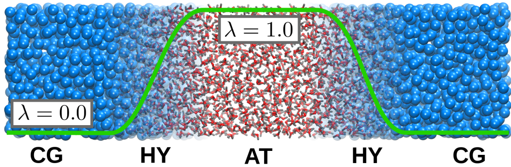
Figure 1.5.: Snapshot from an adaptive resolution simulation coupling 3-site atomistic water to a single-site CG model. The green line represents the resolution function. When molecules diffuse through the system and cross the hybrid region, they change their resolution accordingly.
