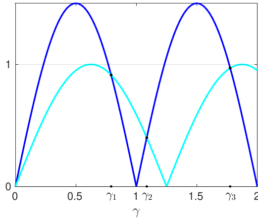
Figure 1. The graphs of the two functions of \gamma in (2.3): The lighter curve corresponds to the function on the left-hand side, the darker one is the graph of the function on the right-hand side. The marked abscissae of the three intersection points of the two graphs are the solutions of (2.3) in the interval (0, 2] .
