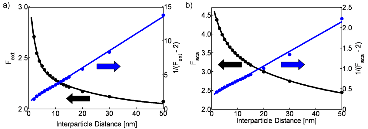
Figure 2.17: The optical response of a dimer depends on the interparticle distance for the extinction (a) as well as for the amount of scattered light (b). In the limit of a large interparticle distance the optical response of a dimer consisting of two spherical particles is twice as much compared to a single sphere of the same diameter. The figures show the ratio F of the optical response of a dimer compared to a single sphere. Calculations are based on BEM simulations with gold spheres with 60 nm in diameter in water. The fit functions of the factor F (equation 2.67) and 1/(F - 2) are given in equations 2.68 - 2.70.
