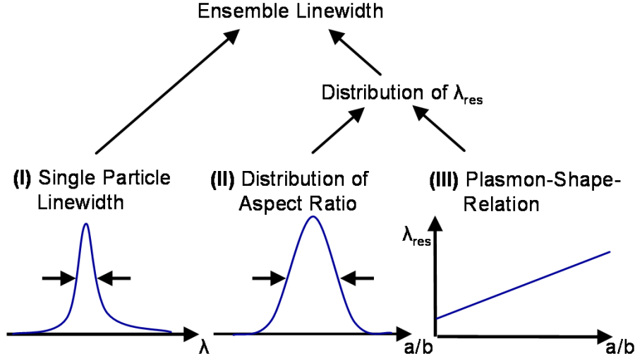
Figure 10.1: The three factors contributing to the ensemble plasmon linewidth: (I) the single particle linewidth, (II) the width of the distribution in aspect ratios ( a/b ) in the sample, and (III) the slope of the plasmon-shape relation connecting aspect ratio ( a/b ) to resonance wavelength ( \lambda_{\text{res}} ). A change in the slope of the plasmon-shape relation (III) is responsible for the ensemble linewidth narrowing of gold nanorods after silver coating. (Image taken from reference [Becker et al., 2008].)
