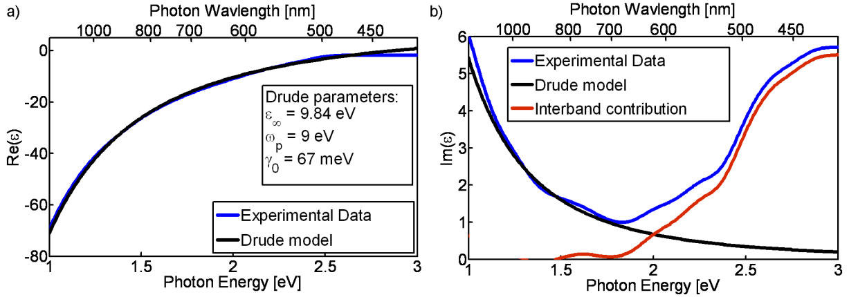
Figure 8.6: Real and imaginary part of the dielectric function of gold (a and b, respectively). Experimental data are taken from Johnson and Christy [Johnson & Christy, 1972] and compared to calculated values using the Drude model (equation 8.8) with the given Drude parameters for gold [Sönnichsen, 2001]. The difference between measurement and theory in the imaginary part of the dielectric function is due to the interband contribution, which is not explained by the Drude model. (Image taken from Reference [Becker et al., 2010].)
