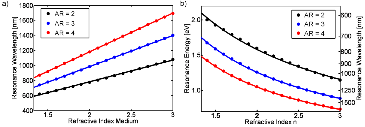
Figure 2.8: The dependency of the (scattering) resonance-wavelength (a) and -energy (b) on the refractive index of the environmental solution is shown for rods with different aspect ratios. The calculation was performed using the boundary element method (BEM), assuming gold nanorods having a diameter of 20 nm and spherical shaped endcaps. Obtained resonances were fitted by the functions given in equations 2.52 - 2.54.
