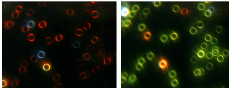
Figure 6.8: In situ particle growth observation of gold nanorods exposed to a growth solution using the RotPOL setup with a consumer digital camera. Starting with rod-shaped nanoparticles with light scattering mostly in the red (left panel), the resonance wavelength decreases over time until the particles scatter light mostly in the green (right panel). (Image taken from reference [Schubert et al., 2008].)
