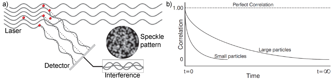
Figure 4.4: (a) Scheme of an approach using the dynamic light scattering process. The particles in the sample scatter the propagating waves which leads to a speckle pattern on the detector (inset). (b) Correlation function for large and small particles. As can be seen, the rate of decay for the correlation function depends on the particle size. (Image taken from reference [Malvern Instruments Ltd., 2005].)
