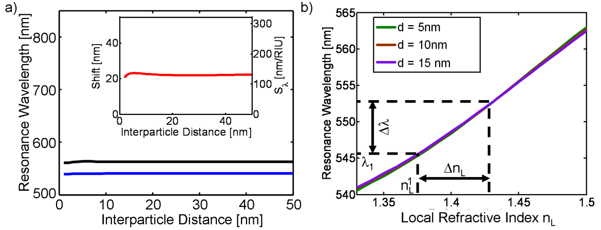
Figure 11.2: a) For the transversal plasmon mode the resonance wavelength is nearly independent of the interparticle distance in water (blue line) as well as in a medium with refractive index n = 1.5 (black line). An increase of the refractive index leads to a redshift, which is therefore also constant in respect to the interparticle distance (inset). b) Relationship of the plasmon resonance and the refractive index for different interparticle distances. The overlapping of the lines emphasizes the independency of the resonance wavelength from the interparticle distance. By measuring the transversal resonance wavelength \lambda_1 the local effective refractive index n_L^1 can be calculated. An occurring shift \Delta\lambda corresponds therefore in a change of \Delta n_L .
