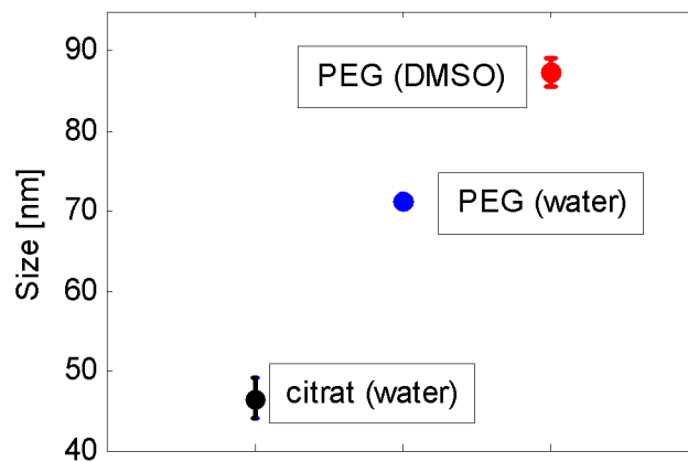
Figure 11.7: Dynamic light scattering (DLS) measurements of nominally 40 nm spherical particles in water initially stabilized with citrate reveals a hydrodynamic diameter of 46.5 \pm 2.6 nm. After coating the particles with methoxy-Polyethyleneglycol-thiol (mPEG) molecules the hydrodynamic diameter (also in water) is increased to 71.3 \pm 0.8 nm. After transfer of these particles into DMSO the hydrodynamic diameter amounts to 87.4 \pm 1.7 nm, which proves the hypothesis that the PEG molecule is more stretched in DMSO than in water.
