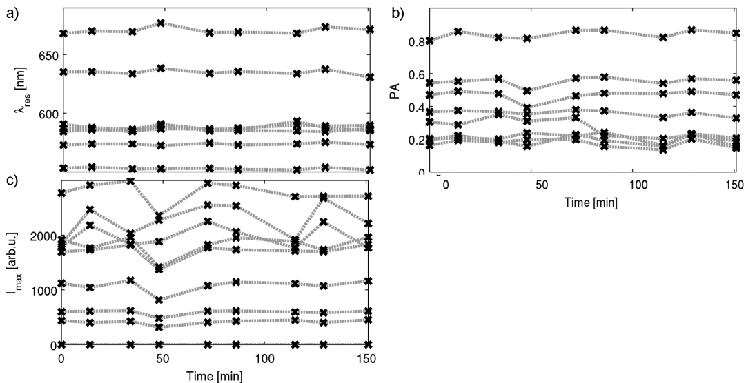
Figure 5.8: Stability of the setup. The same particles were measured repeatedly for more than two hours. The standard deviation is below 1%, about 6% and about 10% for the resonance energy, PA and maximum intensity, respectively. (Image taken from reference [Schubert et al., 2008].)
