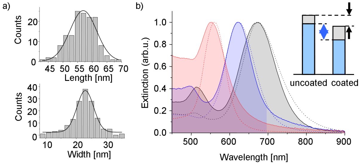
Figure 10.5: (a) Length and width distribution of a sample of uncoated gold nanorods as determined from TEM images of 145 particles. The length and width show a mean of 56.4 \pm 4.4 and 22.8 \pm 3.4 nm, respectively. (b) Ensemble extinction spectra of this gold nanoparticle sample (black) with a thin (2.3 nm) silver coating (blue) and a thick coating (6.9 nm, red): solid lines measured, dashed lines calculated. Only one free parameter enters all three calculations: the eccentricity e used to calculate the geometrical “L factor” [Prescott & Mulvaney, 2006], here e = 0.95 . All other parameters are determined by TEM. The calculated spectra show good agreement to the measurement in both resonance position and linewidth. The inset illustrates the (calculated) linewidth for the uncoated and thinly coated nanorods, in black/gray including the single particle contribution and in blue without this contribution (i.e., pure plasmonic focusing). (Image taken from reference [Becker et al., 2008].)
