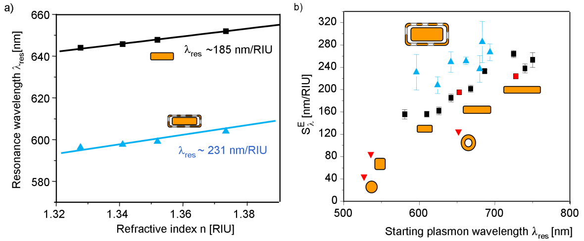
Figure 9.4: (a) Position of the longitudinal plasmon resonance wavelength vs refractive index of the surrounding medium for gold nanorods and nanorattles (as indicated). The slopes show different sensitivities S_\lambda^E [nm/RIU] toward changes in the dielectric environment for both particles. (b) Overview of the S_\lambda^E values of different gold nanostructures: spheres, cubes, rods, shells, and rod-shaped nanorattles. Since the sensitivity S_\lambda^E depends not only on shape but also on the position of the resonance wavelength, we show the S_\lambda^E values as a function of the plasmon wavelength in water. The values for spheres, cubes, shells, and some rod samples are taken from the literature ([Raschke et al., 2003, Raschke et al., 2004, Chen et al., 2008]). Our data for ensemble measurements on different samples of solid gold nanorods (black labels) show lower values for plasmon sensitivity than those of rod-shaped gold nanorattles, produced from these rods (blue labels). (Image taken from Reference [Khalavka et al., 2009].)
