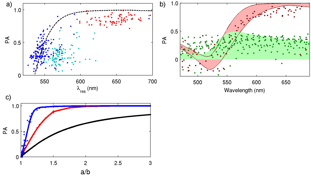
Figure 5.10: (a) The polarization anisotropy PA(\lambda_{\text{res}}) = (I_a - I_b)/(I_a + I_b) at the longitudinal plasmon resonance wavelength \lambda_{\text{res}} is shown as a function of the resonance wavelength for three different gold particle samples (blue dots: nominally spherical gold particles with 60 nm diameter; teal dots: 87 nm diameter; and red dots: gold nanorods). We extract each point from a full wavelength and polarization dependent single particle scattering spectrum I(\lambda, \theta) . The dashed black line is a theoretical prediction from simulations of gold rods of different aspect ratios and sizes embedded in water (refractive index n = 1.34 ). The polarization anisotropy PA(\lambda) for a given particle varies as a function of wavelength \lambda , which we show in (b) for gold rods (red dots) and spheres (green dots). The shaded red and green areas correspond to theoretical predictions for particles with aspect ratios ( a/b ) of 2 < a/b < 3 and a/b < 1.2 , respectively. The theoretical prediction of polarization anisotropy PA at the resonance wavelength as a function of aspect ratio ( a/b ) for silver (blue dots), gold (red dots) and \text{SiO}_2 (black dots) particles is shown in (c). Dots correspond to DDA-simulations, the lines are fits. The simulations do not perfectly follow a common trend due to a small influence of particle volume on the polarization anisotropy. (Image taken from reference [Schubert et al., 2008].)
