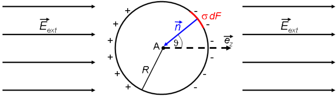
Figure 2.1: To calculate the total local electric field \vec{E}_{loc} at the position of one single lattice atom A the electric field \vec{E}_L due to the polarization of the remaining atoms in the particle has to be added to the external electric field \vec{E}_{ext} . For this purpose a spherical volume with radius R around A is examined, which contains no other atoms except the selected one. \vec{E}_L creates a surface charge \sigma dF on the surface of the spherical volume with the normal vector \vec{n} .
