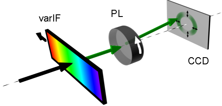
Figure 5.4: Schematics of the rotPOL setup. One wavelength is selected by a linear variable interference filter (varIF), then the light is dispersed into the different polarization directions by a wedge-shaped rotating polarizer (PL), resulting in ring-shaped intensity profiles of a pointlike light source on the digital camera. (Image taken from reference [Schubert et al., 2008].)
