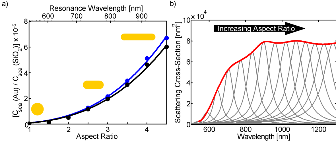
Figure 2.14: a) Comparisons of the scattering cross-section of gold nanorods C_{sca}(Au) with a silica sphere (blue) or silica rods (black) C_{sca}(SiO_2) at the resonance of the rod in water. The volume of the particles was kept constant (i.e. equal to a sphere with 60 nm diameter) by choosing the appropriate rods' length and width to allow a direct comparison. The ratio of the cross-sections compared to the silica sphere and the silica rods in respect to the aspect ratio can be fitted by equation 2.63 and 2.64, respectively. b) Scattering spectra of the gold nanorods with constant volume, but different aspect ratios. The amount of scattered light increases up to an aspect ratio of AR \approx 4 due the associated resonance shift to larger wavelengths, where the interband damping gets less. For even higher aspect ratios, the interband damping is not existing at all and therefore the scattering cross-sections are more or less constant.
