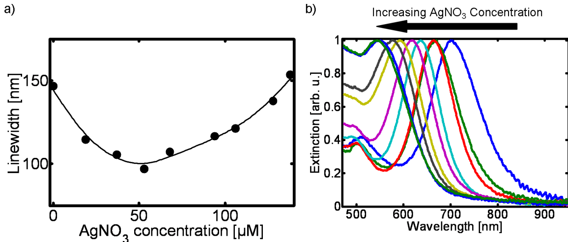
Figure 10.2: (a) Ensemble linewidth as a function of silver concentration in the coating solution for a gold nanorod sample with an initial linewidth of 148 nm. The linewidth is the full width at half-maximum (FWHM) as determined directly from the spectra (shown in (b)). It shows a minimum at 53 \mu\text{M} , where it is reduced to 97 nm from the initial 148 nm (thin line is a guide to the eye). (Image taken from reference [Becker et al., 2008].)
