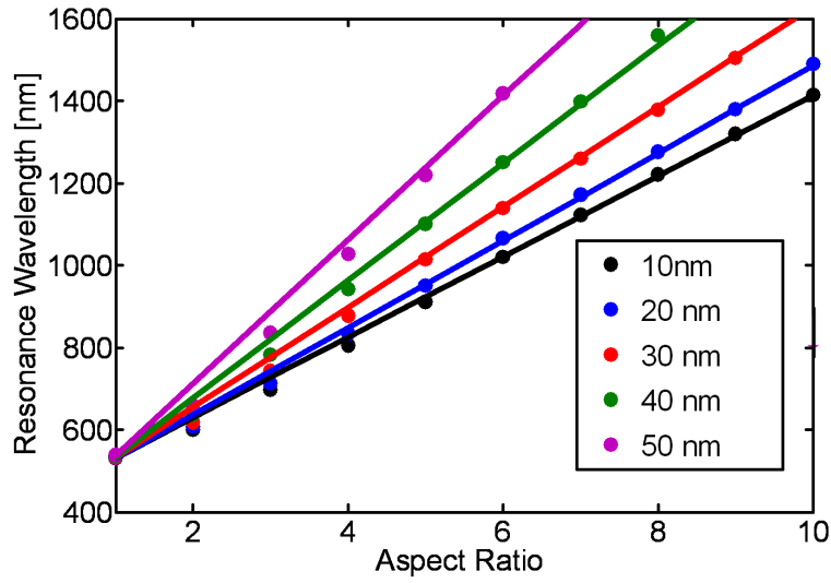
Figure 2.6: Resonance dependency on aspect ratio for gold nanorods with different diameters. Spectra are simulated using the boundary element method assuming rods with spherical endcaps and water as embedding medium ( n = 1.33 ).
