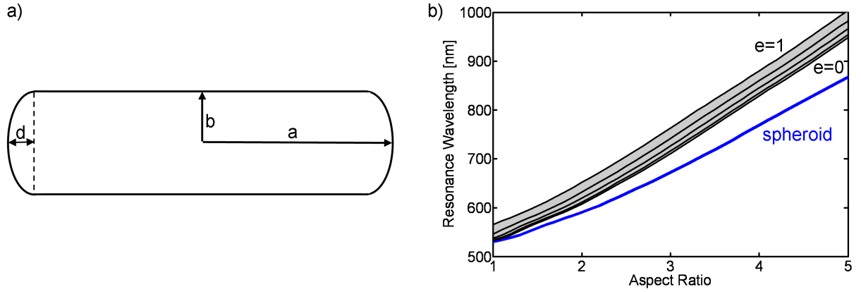
Figure 2.3: a) Scheme of the particle morphology for a rod with an ellipsoidally shaped capped cylinder. The eccentricity e is calculated by: e^2 = 1 - d^2/b^2 , with the limits of a rod with spherical endcaps ( e = 0 ) and no endcaps (i.e. just a cylinder, with e \rightarrow 1 ). b) The resonance wavelength in respect to the aspect ratio for spheroidal gold nanoparticles is represented by the blue line. For gold nanorods having endcaps with an eccentricity 0 < e < 1 the resonance wavelength is displayed by the grayish area. The solid black lines represents resonances for eccentricity values of ( e = 0, 0.5, 0.8, 0.95, 1 ) according to table 2.1.
