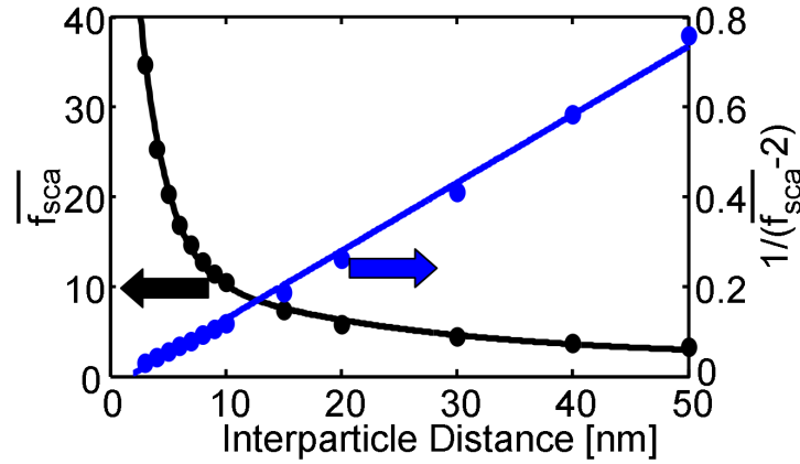
Figure 2.19: Comparisson of the scattering cross-sections of the monomer and the dimer at the dimer's resonance ( C_M^D and C_D , respectively according to Figure 2.18a). The fit functions of the factor \overline{f_{sca}} (equation 2.74) and 1/(\overline{f_{sca}} - 2) shown are given in equation 2.75 and equation 2.76, respectively. The calculations are based on BEM simulations with gold spheres with 60 nm in diameter in aqueous solution.
