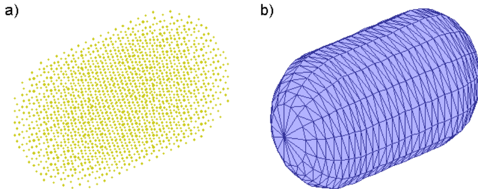
Figure 2.5: Scheme how a particle is discretized within the (a) discrete-dipole approximation (DDA) and (b) the boundary element method (BEM). While in DDA the whole particle is described by an array of N polarizable dipolar elements, in BEM the surface of the particle is discretized into N' surface elements.
