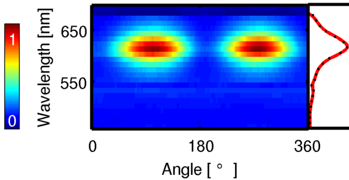
Figure 5.6: By inserting a variable wavelength interference filter the polarization profile is determined for a single wavelength. Repeating this procedure for a wavelength regime (by moving the interference filter with a stepper motor) produces intensity values as a function of wavelength and polarization angle I(\lambda, \theta) , which is shown here color-coded. (Image taken from reference [Schubert et al., 2008].)
