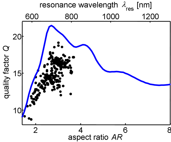
Figure 8.7: The quality factor Q (see equation 8.15) shows a maximum for rods with an aspect ratio of approximately AR = 3 and decreases for larger aspect ratios. The blue line represents the results obtained by BEM calculations, while the black dots correspond to measurements on single gold nanorods. (Image taken from Reference [Becker et al., 2010].)
