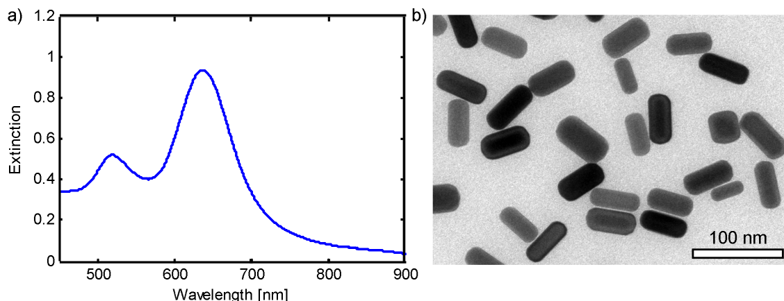
Figure 3.1: a) Extinction spectra and (b) transmission electron microscope image (TEM) of a typical gold nanorod sample.
