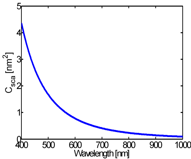
Figure 2.15: The scattering cross-section of a silica sphere with 60 nm in diameter in aqueous solution follows Rayleigh's law and decreases for larger wavelengths. Therefore, the scattering ratio between gold nanorods and \text{SiO}_2 spheres increases continuously, although the maximal scattering cross-section is constant for aspect ratios of the gold nanorods larger than 4 (Figure 2.14a and b).
