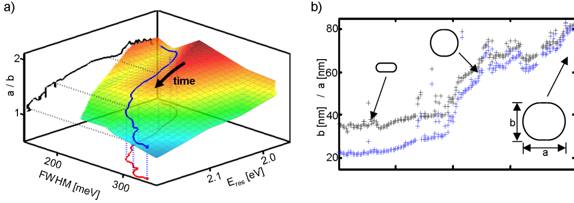
Figure 6.6: (a) The particle geometry (given by the long and short axes a and b , or the aspect ratio a/b and the volume V ) are related to the measured spectral quantities resonance position ( E_{res} ) and linewidth ( FWHM ) by a bijective function F (shown as colored surface area). The function F was calculated by interpolation between values obtained by DDA simulations and Mie calculations. We have indicated a measured trajectory of E_{res} and the FWHM (red line) and the corresponding trajectory of the aspect ratio (blue line). (b) Time development of the long (black)/short (blue) axis of one single nanorod as a function of time (respectively) as determined by the function F . The insets indicate the size of the rod at three moments in time. (Image taken from Reference [Becker et al., 2007].)
