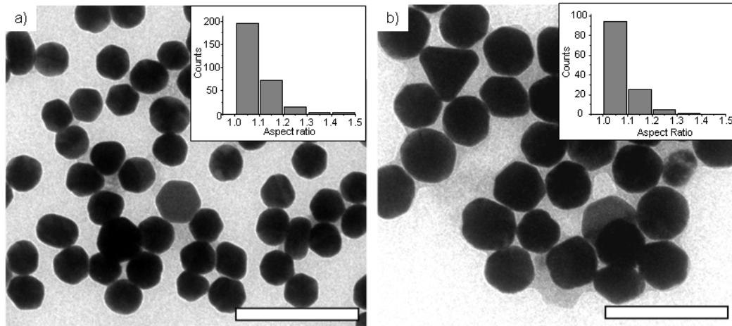
Figure 5.11: Shape of gold nanospheres (BBI Inc. UK.) determined from TEM images for 60 nm particles (a) and 80 nm particles (b) (scalebars 200 nm). Histograms of the aspect ratio determined from such TEM images for more than 100 particles per sample are shown in the appropriate insets. The nominally round particles have a mean aspect ratio (shape anisotropy) of about 1.1 for both samples, which is enough to induce strongly polarized light scattering. (Image taken from reference [Schubert et al., 2008].)
