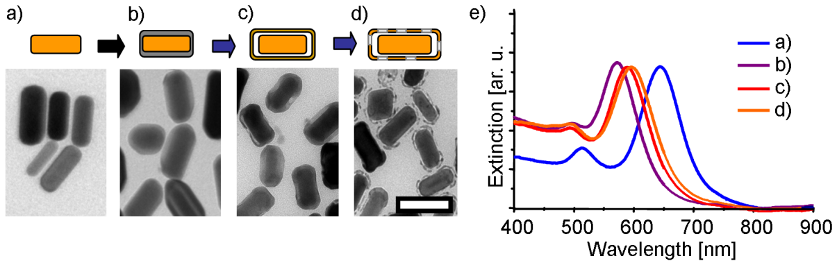
Figure 3.3: Growth of gold nanorattles. Starting with gold nanorods (a), a silver layer is deposited (b). By means of reaction with Au ions (blue arrows), a shell of Ag-Au grows and then transforms into a cage with the dealloying of silver leading to a closed (c) or porous shell (d), depending on the amount of gold added. Representative TEM images corresponding to all the steps are shown on the bottom (scalebar is 50 nm). (e) Extinction spectra corresponding to each step. While the silver coating leads to a blue-shift of the resonance wavelength, the replacement of the silver shell with a gold cage red-shifts the resonance wavelength. (Image taken from reference [Khalavka et al., 2009].)
