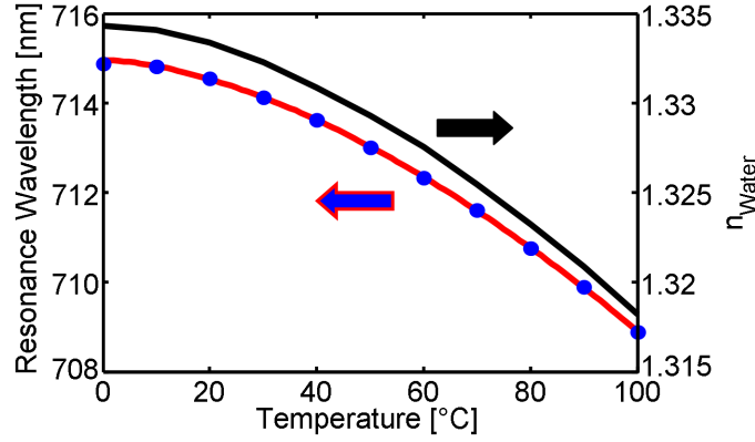
Figure 2.10: Since the refractive index of water depends on its temperature (right axis), the plasmon resonance wavelength changes upon temperature variations of the aqueous solution. On the left axis the plasmon resonance wavelength calculated with the BEM of a gold nanorod with a diameter of 20 nm and an aspect ratio of AR = 3 is plotted. The red line is a fit according to equation 2.57.
