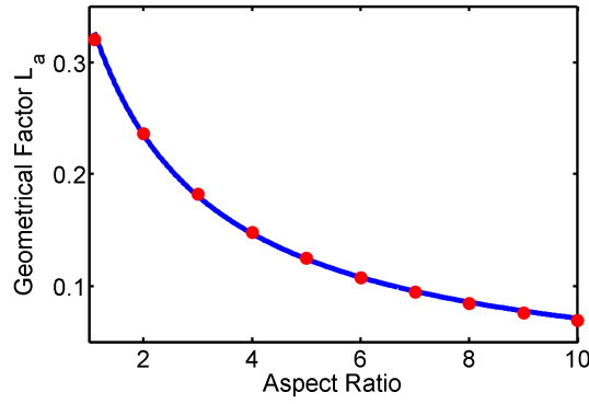
Figure 2.2: The geometrical factor L_a and L_b of the long axis of a oblate shaped spheroid can be described by the simple approximation of equation 2.30 (blue line). The red dots mark the exact values calculated by equation 2.27.
