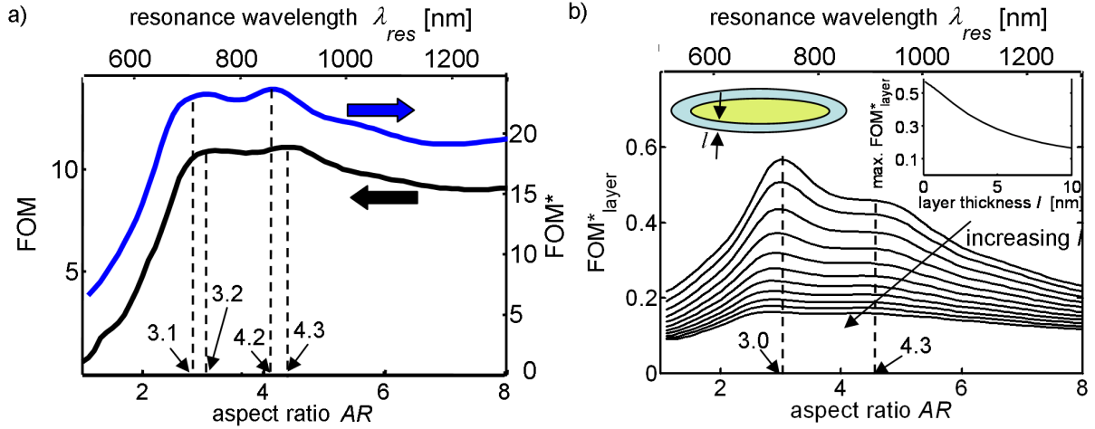
Figure 8.3: To identify the optimal aspect ratio for plasmon sensing, various “figure of merits” (FOM) are calculated a) The classical FOM defined as plasmon sensitivity S divided by plasmon linewidth \Gamma (left axis) is compared to a generalized FOM^* defined as the maximal relative intensity change |\Delta I|/I for a small refractive index change \Delta n (right axis). While the “classical” figure of merit FOM has a maximum for an aspect ratio of AR = 4.3 and a second maximum at AR = 3.2 , the generalized FOM^* has its maximum at AR = 4.2 with its second local maximum at AR = 3.1 . b) The FOM_{layer}^* takes into account the sensing volume by considering the plasmon change induced by a small layer around the particle normalized to the layer thickness ( 0.01\text{ nm} < l < 10\text{ nm} in 1\text{ nm} steps). The plasmon sensing quality FOM_{layer}^* decreases with increasing layer thickness (inset) and shows a maximal value of FOM_{layer}^* = 0.55 for l \rightarrow 0 at an aspect ratio AR = 3.0 . (Data for a) are calculated by BEM for gold nanorods with spherical end-caps and 20\text{ nm} diameter, data for b) within the QSA for spheroids.) (Image taken from Reference [Becker et al., 2010].)
