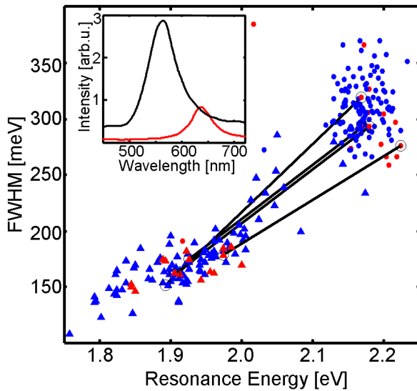
Figure 6.3: Optical single-particle spectra of particles before (triangles) and after (dots) rinsing them with growth solution for about 180 min. For each spectrum, the full width at half-maximum (FWHM) is plotted against its resonance energy. The particles corresponding to the red markers are continuously measured. Red dots represent 16 of the particles investigated continuously during rinsing with growth solution. The inset shows an example of a single particle spectrum before (red) and after (black) rinsing with growth solution. The increase of absolute intensity is caused by the increased particle volume. (Image taken from reference [Becker et al., 2007]).
