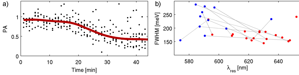
Figure 6.9: (a) The initial rod-shaped nanoparticles have a high degree of polarization anisotropy PA which decreases over time due to the additional growth until nearly all particles show a much lower anisotropy. The red line is an average over six particles. Before and after the growth process, detailed polarization-dependent scattering spectra I(\lambda, \theta) are obtained. (b) The linewidth FWHM and resonance wavelength \lambda_{\text{res}} extracted from these measurements are shown in (red dots at start of growth process, blue dots afterward). Dashed lines connect dots corresponding to the same particle. For most particles, the resonance wavelength decreases and the linewidth increases. The decrease of polarization anisotropy over time, the simultaneous decrease in resonance wavelength, and the increase in linewidth suggest that the rod-shaped particles grow mainly along the short axis, resulting in particles that are more spherical. (Image taken from reference [Schubert et al., 2008].)
