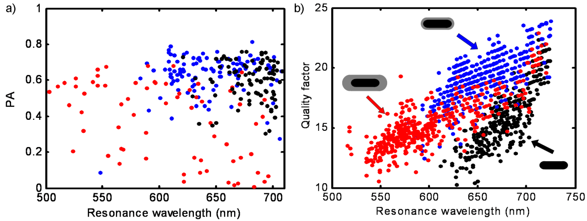
Figure 9.3: (a) Polarization anisotropy ( PA ) for pure gold nanorods (black dots), with a thin silver coating (blue dots), and with a thick silver coating (red dots). PA is a measure for the degree of rod-like shape: it is expected to be close to 1 for perfect rods and close to 0 for perfect spheres. Clearly, the PA decreases for particles with thick coating. (b) The quality factor extracted from single particle scattering spectra are shown here for pure gold nanorods (black dots), those rods with a thin silver coating (blue dots) and thick silver coating (red dots). The silver coating increases the quality factor up to 2 fold. (Image taken from Reference [Becker et al., 2008].)
