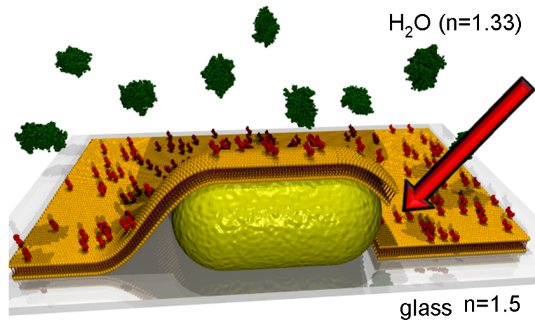
Figure 7.4: Schematics of a gold nanorod (yellow) coated with a partly biotinylated (red) membrane (orange) and exposed to streptavidin (green). In contrast to Figure 7.1 the scheme here presents the case of a incomplete membrane coverage (see red arrow) which can lead to a non-specific binding of streptavidin to the rodsurface.
