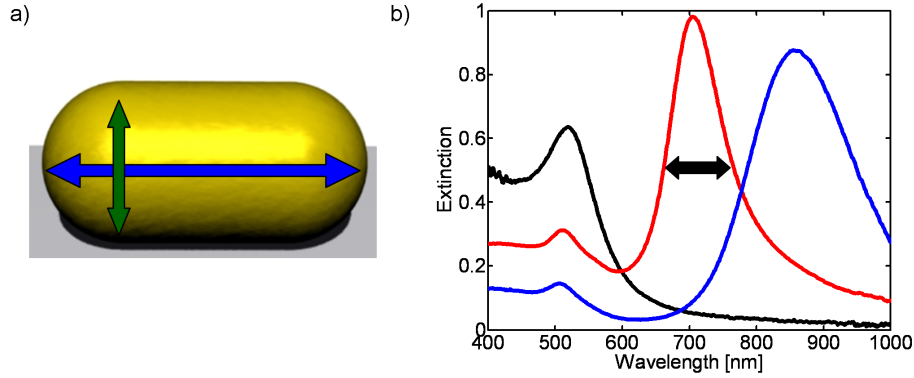
Figure 4.1: (a) Rodshaped particles show a longitudinal (blue arrow) as well as a transversal (green arrow) resonance due to their non-isotropic shape. (b) Ensemble extinction spectra of gold spheres (black) and gold rods with different aspect ratio ( AR=3 and AR=4 , red and blue lines, respectively). While spherical particles have only one resonance peak, rods show two peaks resulting from the transversal and the longitudinal resonance mode. Thereby the position of the longitudinal peak strongly depends on the aspect ratio of the particles. The arrow indicates the linewidth (FWHM) of the ensemble spectrum, which is connected to the polydispersity of the sample.
