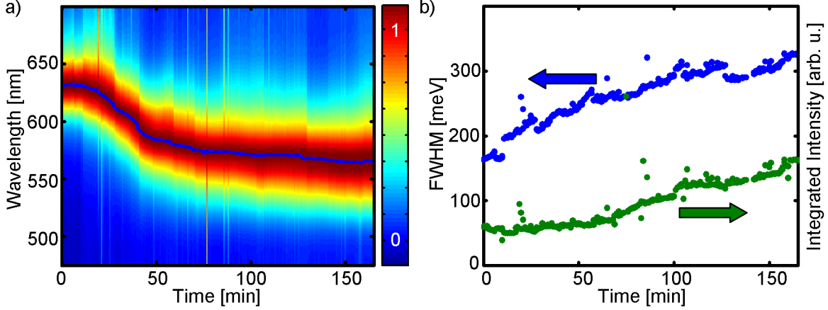
Figure 6.4: (a) Normalized scattering spectra of one single particle during rinsing with growth solution shown color-coded as a function of time. During the first 10 min, the particle is incubated in pure CTAB solution (0.1 M). For the same measurement, the time development of the FWHM (blue dots) and the integral of intensity over the wavelengths (green dots) are shown in (b). (Image taken from reference [Becker et al., 2007].)
