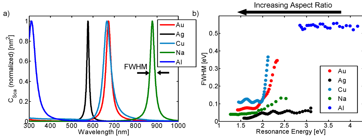
Figure 2.7: a) To obtain the “best” (smallest possible spectral linewidth) plasmonic particles, the scattering spectra in aqueous solution of nanoparticles consisting of different materials were simulated. From an array of dielectric functions only 5 materials show a plasmon peak in the visible spectrum: gold (Au), silver (Ag), copper (Cu), sodium (Na), and aluminum (Al). The graph shows the normalized scattering spectra of the long axis of spheroidal prolates with an aspect ratio of AR = 3 calculated within the quasi-static approximation. b) The quality of a plasmon peak can be determined by the FWHM of the peak. Better than gold are silver and sodium ellipsoidal prolates. However, due to its violent reactivity with water, sodium is not practicable for usage. Since silver is not as inert as gold (e.g. oxygen, ions, light) gold nanoparticles are the most appropriate plasmonic particles in the visible range of light. For higher energies probably aluminum particles could be a candidate for applications, but synthesis methods for rodshaped nanoparticles are still missing.
