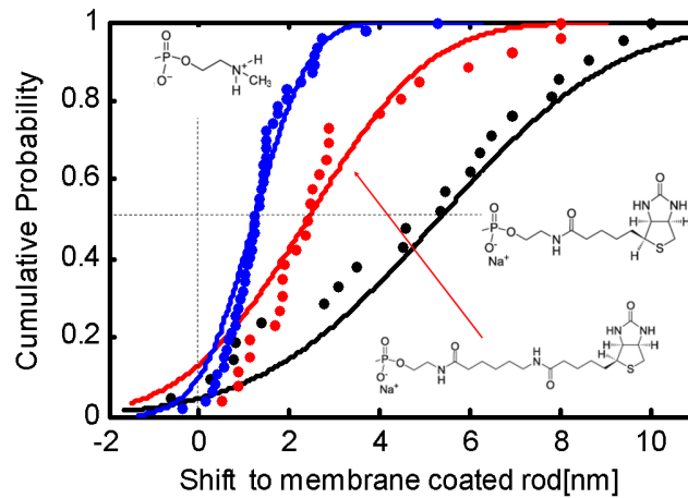
Figure 7.6: Cumulative probability of the spectral shifts due to attachment of streptavidin to gold nanorods coated with different lipids. Attaching streptavidin to rods coated with lipids including biotin leads to a shift of \Delta_s = 5.3 \pm 3.1 nm (block dots). Using instead lipids with biotin including a spacer the spectral shift is smaller and results in \Delta_s = 2.4 \pm 2.1 nm (red dots). A lipid without any biotin leads to a small shift of \Delta_s = 1.2 \pm 1.0 nm due to a nonspecific binding to the gold rod surface (blue dots). The solid lines show the cumulative probability for a Gaussian distribution with the listed median values and standard-deviations. (Image taken from reference [Baciu et al., 2008].)
