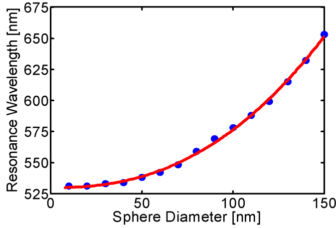
Figure 2.4: The resonance wavelength of gold nanospheres depends on the particles' diameter due to retardation. This effect occurs since the speed of light is finite, and changes in one particles end leads to a reaction in the opposite end with a certain phase delay, which leads to a redshift of the resonance wavelength. The spectra are calculated using Mie's theory and can be fitted by equation 2.36.
