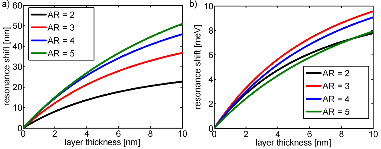
Figure 8.4: Resonance shift in respect to the layer thickness for gold nanorods with different aspect ratios in wavelength units (a) and energy units (b). The calculation was performed within the QSA for spheroids with a fixed diameter of 20 nm embedded in aqueous solution and assuming a refractive index of n = 1.5 for the coating layer.
