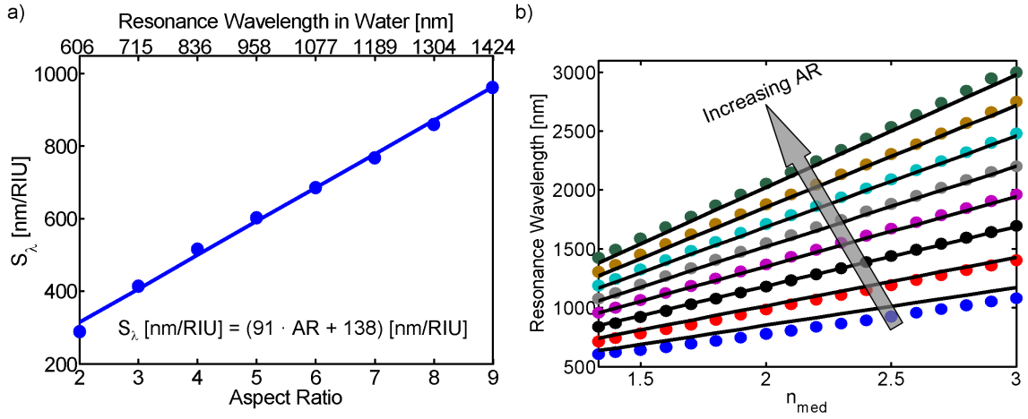
Figure 2.9: (a) The steepness of the lines in equations 2.52 - 2.54 represents the sensitivity S_\lambda [nm/RIU], which can be fitted with respect to the aspect ratio by the shown equation. This function can be extended to a fit-function describing the resonance in dependency to the aspect ratio and the refractive index of the embedding medium (equation 2.55). (b) The resonances calculated with BEM are shown as dots and the values obtained by the presented fit-function are plotted as black lines.
