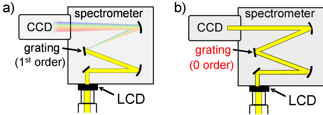
Figure 5.1: (a) Scheme of the spectrometer of the fastSPS setup, where the entrance slit of the spectrometer is replaced by an electronically addressable liquid crystal device (LCD) placed in the microscope's image plane. (b) To take an image of the sample the grating is moved to zero's order and operates then as a mirror.
