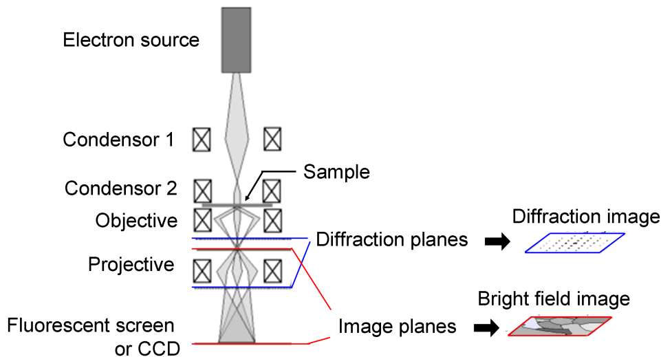
Figure 4.3: Scheme of a transmission electron microscope. A TEM can in principle be compared to a light microscope, if photons are substituted for electrons. The bright field image plane is used to image the sample, while the diffraction image plane reveals the elemental composition of the sample. (Image taken from reference [Wikipedia, 2009].)
