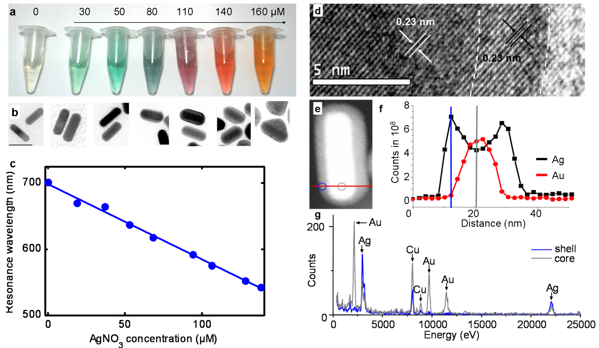
Figure 3.2: (a) True color photograph showing the color change of the pure gold nanorods (mean dimensions 51 \times 18 nm, left sample) upon increasing silver concentration in the coating solution (indicated by the number above each vial). (b) Representative TEM images corresponding to the samples shown above. Images show the increasing thickness of the silver shell with higher silver concentration. At very high silver concentrations the shell becomes inhomogeneous (scalebar for all images 50 nm). (c) Resonance wavelength as a function of silver concentration in the coating solution for a gold nanorod sample with a starting resonance wavelength of 700 nm. The shift in the resonance wavelength is approximately linearly dependent on the amount of silver present with a slope of -1.15 nm/ \mu\text{M} (dashed line). (d) High-resolution TEM image of a silver-coated gold nanorod. Dashed lines indicate the borders of the silver shell. Equal lattice spacing (0.23 nm) in the Au core and the Ag shell confirms epitaxial growth ([111] planes). (e) Scanning TEM image of a silver-coated gold nanorod with the position of the EDX linescan (red line). (f) Profile of the Au and Ag elemental distributions. (g) Two representative EDX spectra (at the positions indicated in (e) and (f)). (Image from reference [Becker et al., 2008].)
