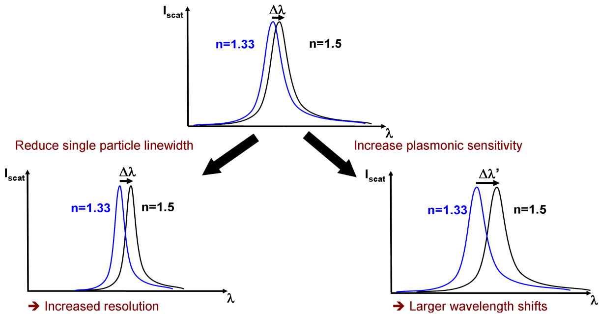
Figure 9.1: An increase in the refractive index of the local environment of a nanoparticle shifts its resonance wavelength into the red. To increase the sensitivity there are two possibilities: a reduction of the single particle linewidth (while the size of the shift stays the same) increases the resolution and therefore also the sensitivity of the sensor (left part of the image). Another possibility is to increase the size of the shift by increasing the plasmonic sensitivity on changes in the refractive index, which is shown in the right part of the image.
