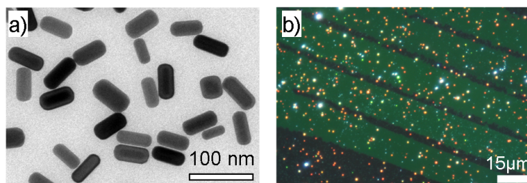
Figure 7.2: (a) Transmission electron microscope (TEM) image of gold nanorods used in this work (mean length 56 \pm 5 nm, width 26 \pm 5 nm, aspect ratio 2.2 \pm 0.4 nm, determined from 100 particles). (b) Darkfield image of gold nanorods (bright spots) covered by a lipid membrane. The membrane (greenish background) is structured on this substrate by a micromolding in capillaries [Janshoff & Kunneke, 2000]. (Image taken from reference [Baciu et al., 2008].)
