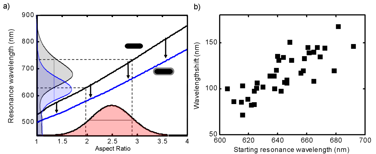
Figure 10.4: (a) The plasmon-shape relation shows how the resonance wavelength depends on aspect ratio. Values derived theoretically within the quasi-static approximation are shown for gold rods in water (black line, n = 1.33 ) and with a 2.3 nm silver coating (blue line). The plasmon-shape relation converts an ensemble of particles with a distribution of aspect ratios (indicated by pink shading) into a distribution of resonance wavelengths (indicated by the gray shaded spectrum). The plasmon-shape relations are almost linear, i.e. a distribution of aspect ratios with a given width (polydispersity) gives a certain linewidth regardless of the mean aspect ratio. The shallower slope of the plasmon-shape relation for the silver-coated rods results therefore in a smaller spectral linewidth (blue shaded spectrum). An alternative way to look at the effect of coating is to observe the vertical differences between the two plasmon-shape relations (indicated by black arrows). Hence, rods with higher aspect ratio shift more on silver coating than those with a smaller aspect ratio. (b) Experimental data for the wavelength shifts of gold nanorods upon coating with silver as a function of the starting resonance wavelength. Each data point is extracted from two single particle measurements of the same particle before and after coating. Higher starting resonance wavelengths (i.e. rods with higher aspect ratio), result in larger wavelength shifts. (Image taken from reference [Becker et al., 2008].)
