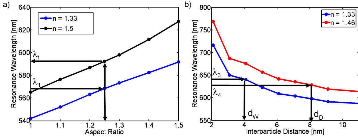
Figure 11.6: a) DDA simulation of the resonance wavelength of the transversal mode of dimers consisting of spheroidal particles with varying aspect ratio in water (blue) and n = 1.5 (black). Comparison with the measured transversal resonance \lambda_1 of the dimer in water reveals an aspect ratio of AR \approx 1.25 . The plasmonic sensitivity S_\lambda of the transversal mode is calculated using additionally the resonance wavelength \lambda_t in n = 1.5 . In combination with the measured resonance wavelength \lambda_2 of the transversal mode in the second solvent (DMSO) the local refractive index n_L could be estimated to n_L = 1.46 . b) DDA simulations of the longitudinal mode of a dimer consisting of two spheroidal particles with aspect ratio AR = 1.25 in water and in n_L = 1.46 . The measured resonances \lambda_3 and \lambda_4 reveal a interparticle distance of d_W \approx 4 nm in water and d_D \approx 8 nm in DMSO, respectively. This means an increase in the interparticle distance of \Delta d \approx 4 nm, due to the exchange of the solvent from water to DMSO.
