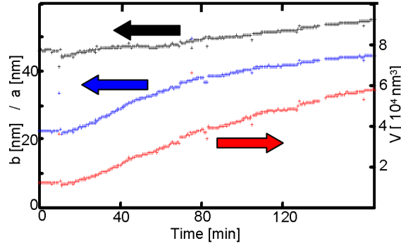
Figure 6.7: Average shape development of 12 particles calculated from E_{res} and the measured scattering intensity I_{sca} by the simplified function G . (Image taken from Reference [Becker et al., 2007].)
