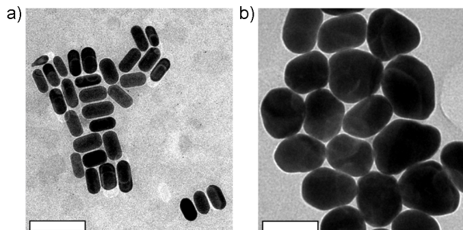
Figure 6.1: (a) TEM image of original gold nanorod sample. (b) TEM image of the sample after 2.5 hours incubation in growth solution in a batch experiment. The particles are considerably larger and more spherical. Scalebars are 100 nm. (Image taken from reference [Becker et al., 2007]).
