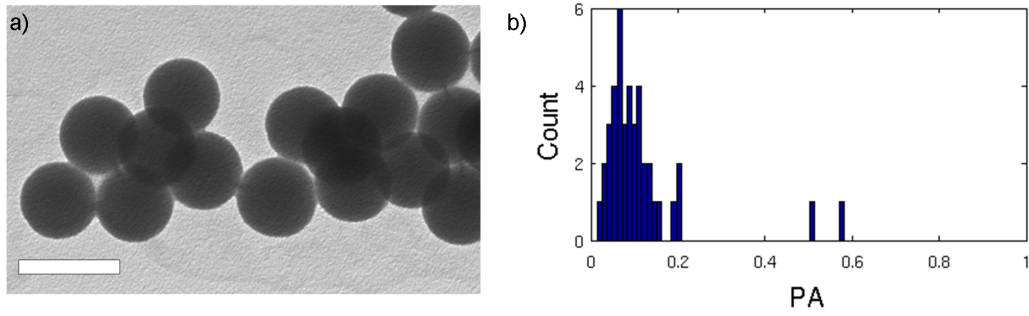
Figure 5.7: (a) TEM-image (scalebar: 500 nm) of \text{SiO}_2 -spheres and (b) results of a measurement of these perfectly spherical particles, using the rotPOL-setup. The imperfections of the optical components induce an error of about 0.1 in the polarization anisotropy (PA). (Image taken from reference [Schubert et al., 2008].)
