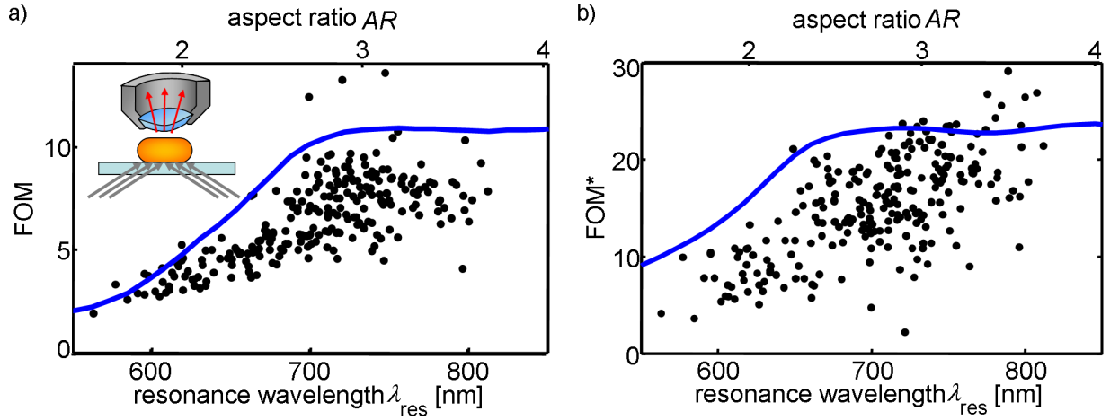
Figure 8.5: Experimental data (each black dot represents one single particle) for the figures of merit FOM (a) and FOM^* (b) obtained by single particle spectroscopy in a dark-field microscope (inset). The absolute values are slightly lower than the theoretical prediction (blue line, see also Figure 8.3a) due to the attachment of the gold rods to a glass substrate which limits the accessible surface (inset). (Image taken from Reference [Becker et al., 2010].)
