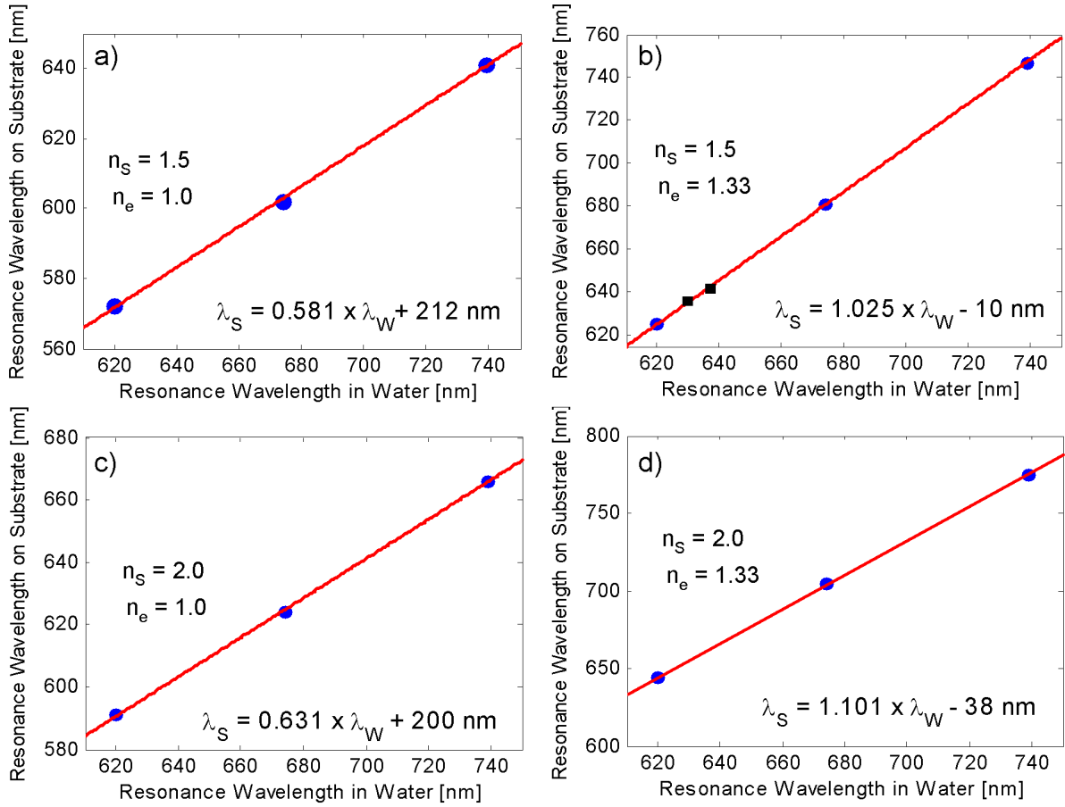
Figure 2.12: The resonance wavelength of gold nanorods is simulated with DDA in aqueous solution and on a different substrates ( n_S ) and environments ( n_m ). If the resonance on a specific substrate and environment \lambda_S is plotted versus the resonance wavelength in water \lambda_W , the data points of particles with different aspect ratios ( AR = 2, 2.5, 3 , blue dots) can be fitted by a linear function. The black dots in b) indicate two measured samples, where the resonance wavelength in water of the ensemble was measured as well as the mean resonance wavelength on a glass substrate ( n_S = 1.5 ) of many single particles with water ( n_m = 1.33 ) as environment. The measured data fit nicely to the simulated results.
