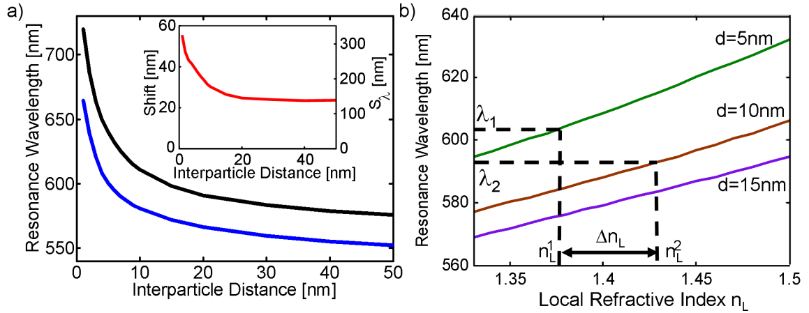
Figure 11.3: a) The resonance wavelength of the longitudinal plasmon mode shows a dependency on the interparticle distance in water (blue line) as well as in a medium with refractive index n = 1.5 (black line). An increase of the refractive index leads to a redshift, but in this plasmon mode the shift (i.e. also the sensitivity S_\lambda ) is not independent of the interparticle distance (inset). b) If the local effective refractive index n_L^1 was estimated from the transversal mode (Figure 11.2), the measured resonance wavelength \lambda_1 reveals the interparticle distance. In the case the interparticle distance stays constant for an increase of n_L (5 nm (green), 10 nm (brown) and 15 nm (purple) lines), the corresponding resonance wavelength is redshifted. However, if the local refractive index is increased up to n_L^2 and the interparticle distance enlarges (e.g. from 5 to 10 nm), the appropriate resonance wavelength \lambda_2 can even be blueshifted.
