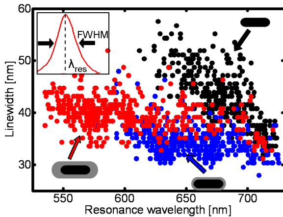
Figure 9.2: Linewidth of gold nanorods (without coating (black dots), with a thin (blue dots) and thick (red dots) silver shell) plotted against their resonance wavelength, both extracted directly from scattering spectra (inset). On average, the linewidth (FWHM) of particles with silver coating is smaller than the linewidth of pure gold nanorods with similar resonance wavelength. The thicker silver shell shows a higher linewidth than the thin shell due to an anisotropic shell thickness. (Image taken from Reference [Becker et al., 2008].)
