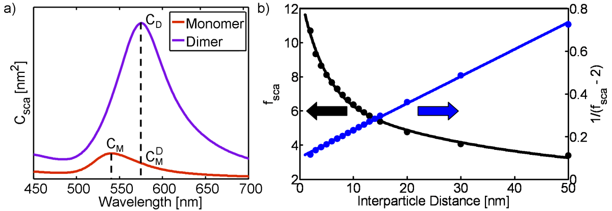
Figure 2.18: a) For single particle measurements it is often interesting to compare the ratio of the scattering cross-sections of the longitudinal mode of a dimer with the one of a single particle. The scattering cross-sections of a single nanosphere (red line) and a dimer (purple line) can be compared at each maximum ( C_M and C_D , respectively), or at a specific resonance wavelength (e.g. maximal scattering cross-section of the dimer) with the cross-sections C_M^D for the monomer and C_D for the dimer. b) Ratio of the maximal scattering cross-sections of the monomer ( C_M ) and the dimer ( C_D ). The fit functions of the factor f_{sca} (equation 2.71) and 1/(f_{sca} - 2) shown are given in equation 2.72 and equation 2.73, respectively. The calculations are based on BEM simulations with gold spheres with 60 nm in diameter in aqueous solution.
