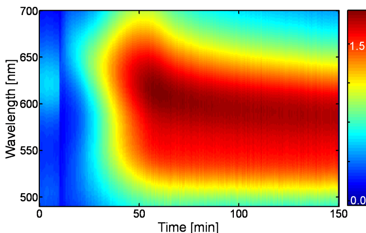
Figure 6.2: Continuous ensemble extinction spectra (color coded) of previously grown gold nanorods. After 10 min. a growth solution is added to achieve a further nanoparticle growth. The peak shifts to smaller wavelengths and increases in intensity due to the nanoparticle growth process. (Image taken from reference [Becker et al., 2007]).
