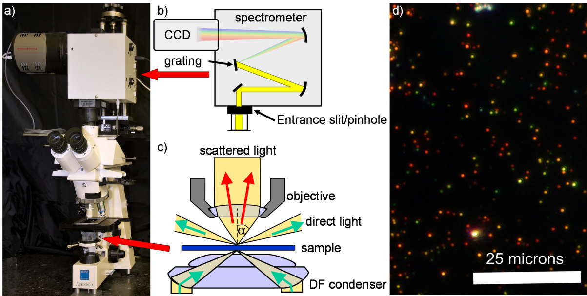
Figure 4.2: a) Picture of a conventional light microscope in darkfield mode, which is used to image gold nanorods and investigate them spectrally by a spectrometer and a coupled CCD camera (b). Illumination of the sample is through a darkfield oil immersion condenser (c), and therefore the direct light does not enter the objective and only the scattered light of the nanoparticles is collected. d) The resulting image shows bright spots on a black background, each spot representing the scattered light of one single nanoparticle.
