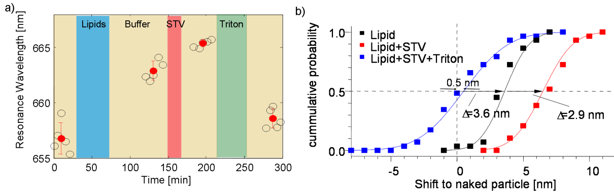
Figure 7.3: (a) The resonance wavelengths extracted from single particle spectra of one individual particle measured over the course of the experiment (black circles, mean in red with standard deviations). Shadings indicate the experimental steps: initially naked, then covered by a biotinylated membrane, followed by a layer of streptavidin, and finally after washing with Triton x-100 to remove the entire membrane coating (b) Cumulative probability of spectral shifts derived from observing 29 particles parallel to the particle in b. We observe a median shift of \Delta_m = 3.6 \pm 1.5 nm (black dots) after covering the particles with a membrane. Addition of streptavidin leads to a second shift of \Delta_s = 2.9 \pm 1.8 nm. After rinsing with protease and Triton x-100 (to remove the proteins and the membrane), the resonance wavelength is \Delta_t = 0.5 \pm 2.7 nm shifted compared to the beginning of the experiment. The solid lines show the cumulative probability for a Gaussian distribution with the listed median values and standard deviations. (Image taken from reference [Baciu et al., 2008].)
