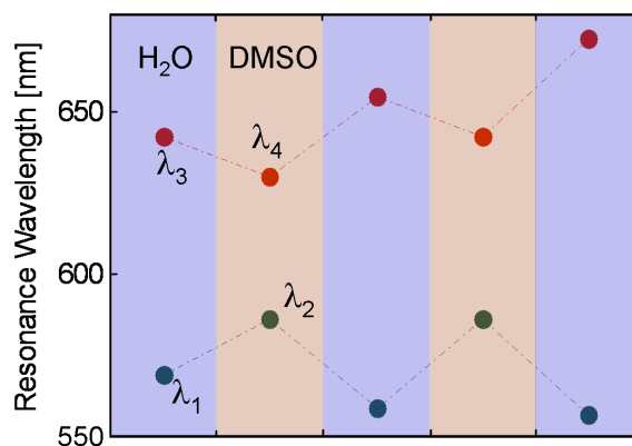
Figure 11.4: Investigation of the resonances of a single dimer in different refractive indices. Initially the dimer is immobilized on glass substrate and immersed in water n = 1.33 . Rinsing the flowcell with dimethyl sulfoxide (DMSO) with a refractive index of n = 1.47 leads to the expected redshift of the transversal plasmon mode (blue dots and line, with \lambda_1 = 568 nm and \lambda_2 = 586 nm). The resonance of the longitudinal plasmon mode (red dots and line, with \lambda_3 = 642 nm and \lambda_4 = 630 nm) shows a blueshift, which can only be explained by an increase of the interparticle distance. The reversibility was proved by rinsing the flowcell again with water, which results in an opposite shifts of the two modes compared to the initial ones.
