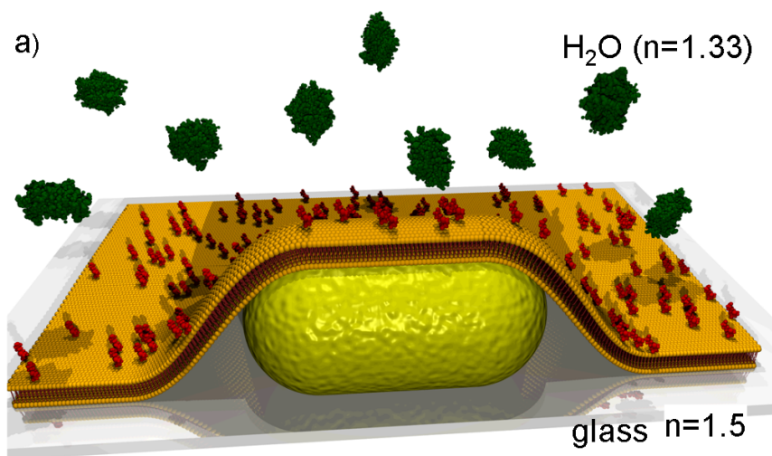
Figure 7.1: Schematics of a gold nanorod (yellow) coated with a partly biotinylated (red) membrane (orange) and exposed to streptavidin (green). The scheme presents the ideal case of a complete membrane coverage without any defects. The glass support has a refractive index of n = 1.5 , the aqueous buffer of n = 1.33 . (Image taken from reference [Baciu et al., 2008].)
