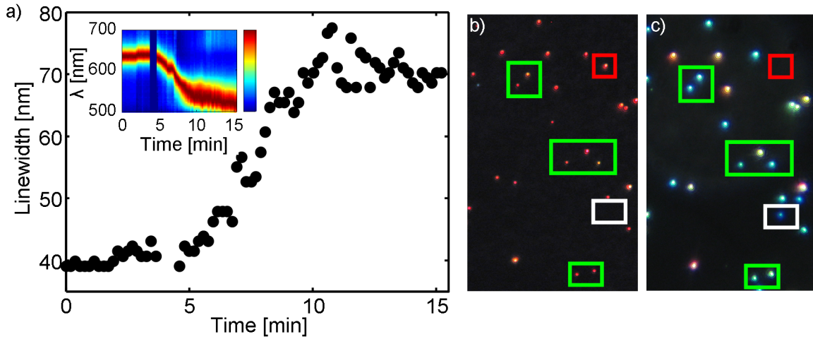
Figure 10.3: (a) Observation of the linewidth change over time of a single gold nanorod exposed to the silver-coating solution. The inset shows the full spectra (color coded) over time (image taken from reference [Becker et al., 2008]). True color photograph of the same particles in the dark-field microscope before (b) and after coating (c). Green boxes show particles which get coated, while the white box indicates the emersion of a blue particle, which is probably a silver sphere. Due to adding and mixing solutions during the growth process some particles can vanish (red box).
