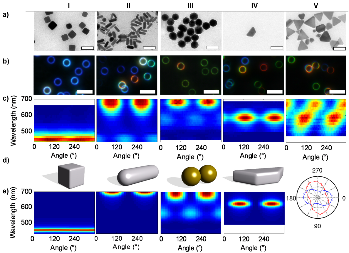
Figure 5.9: Typical plasmon polarization results for simple gold and silver plasmonic nanostructures. (a) TEM images of samples containing silver (I,II,IV,V) and gold (III) nanoparticles (scale bar: 100 nm). In line (b), typical real-color microscopic images of those samples are shown (scale bar: 15 \mu\text{m} ). The polarization dependent single-particle-scattering-spectra I(\lambda, \theta) of representative particles are shown in (c) color-coded as in Figure 5.6. These results can be compared to simulations by discrete dipole approximation shown in (e) with the model sketched in (d). For the triangular particle in column V, a polar graph of the intensity I(\theta) at the two particle resonances visible in Vc is shown in the bottom panel. Two loops with the expected 60° offset are clearly visible. (Image taken from reference [Schubert et al., 2008].)
