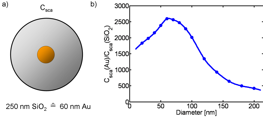
Figure 2.13: a) A gold (Au) sphere with 60 nm in diameter embedded in water scatters as much light as a 250 nm sized silica (SiO 2 ) sphere, compared at the resonance wavelength of the gold sphere ( \lambda_{res} = 548 nm). b) Comparing the scattering cross-sections of a Au and a SiO 2 sphere in respect to the particle size reveals a maximum at approximately 60 nm with an approximately 2500 higher scattering efficiency for the Au sphere.
