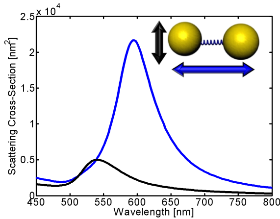
Figure 11.1: A dimer of nanospheres (particle diameter = 60 nm, interparticle distance = 5 nm) has two scattering modes, which are perpendicular to each other. Since the longitudinal (blue) mode is overlayed with the transversal mode (black) a polarizer is needed to investigate both modes independently.
