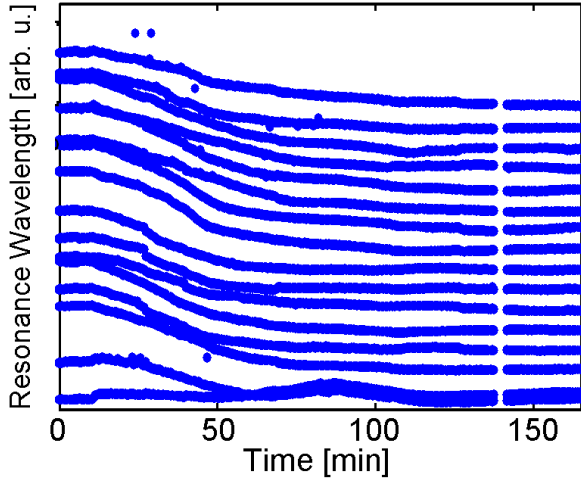
Figure 6.5: The resonance wavelength of 16 particles from one experimental run (arbitrary offset) decreases as a function of time for 14 particles (upper lines), while it stays nearly constant for two particles. The gap after 140 min is due to refocusing. (Image taken from reference [Becker et al., 2007]).
