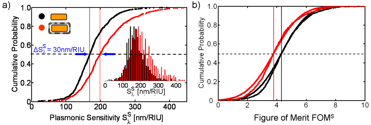
Figure 9.5: (a) Cumulative probability distribution of S_{\lambda}^S values derived from measuring single particle spectra of 1567 gold nanorods and 803 gold nanorattles. The median S_{\lambda}^S = 169 \pm 1.3 nm/RIU and S_{\lambda}^S = 199 \pm 2.5 nm/RIU for the rods (black) and cages (red), respectively. The inset shows the corresponding normalized histograms. (b) Cumulative probability distribution of the figure of merit (FOM) derived from the measured single particle spectra. The median value is FOM^S = 4.3 \pm 1.4 and FOM^S = 3.8 \pm 1.5 for the rods (black) and cages (red), respectively. Although the rattles have a higher S_{\lambda}^S value compared to the rods, they show a smaller FOM^S value due to the larger FWHM as a result of the stronger plasmon damping in rattles, which increases the linewidth. (Image taken from reference [Khalavka et al., 2009].)
