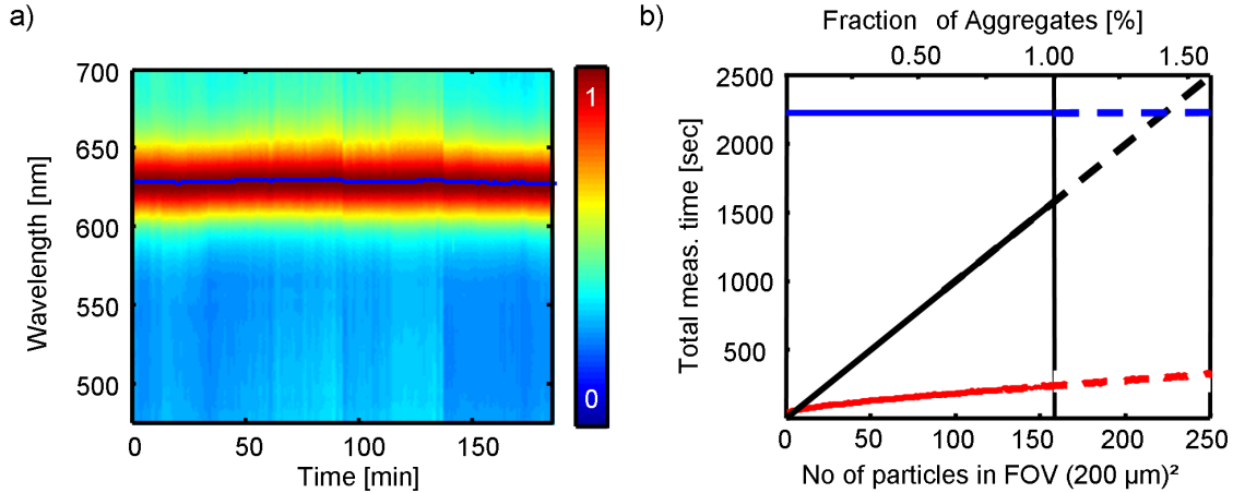
Figure 5.3: (a) Continuous measurement of the same particle with the fastSPS setup to test its stability. The spectra have a mean of 628.6 nm, a standard deviation of 0.65 nm and a maximal deviation of 1.58 nm. Refocusing (after about 90 and 140 minutes) leads to a maximal change of 1.47 nm (stripes in the image). The maximal deviation between two consecutive measurements is 0.58 nm. (b) For randomly deposited particles, higher particle densities on the sample (lower horizontal axis) lead to a higher percentage of more than one particle in a diffraction limited spot (particle aggregates, upper horizontal axis). The total measurement time for all particles in the field of view increases linearly for a serial method (black line) and is independent for all spectral imaging methods, which determine the spectra of all points in the field of view (blue line). The fastSPS method (red line) is by far the fastest method for realistic particle densities around 160 particles in the field of view ( \text{FOV} = 200 \mu\text{m}^2 ) corresponding to roughly 1% of particle aggregates. (Images taken from reference [Becker et al., 2007].)
