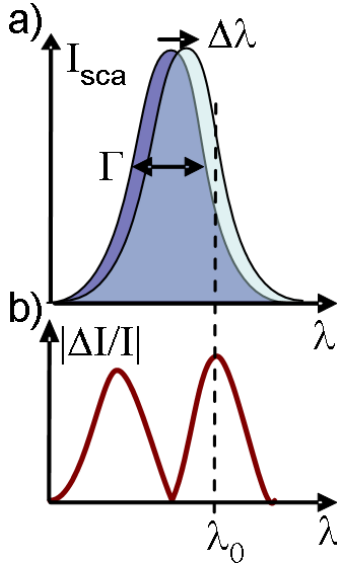
Figure 8.1: a) The plasmon resonance shifts ( \Delta\lambda ) upon changing the refractive index of the surrounding medium by \Delta n . To detect such changes, the sensitivity S_\lambda = \Delta\lambda/\Delta n needs to be large. Other important parameters that characterize plasmonic sensors are the plasmon linewidth \Gamma and b) the wavelength position \lambda_0 where the relative intensity change |\Delta I/I| is largest (see text). (Image taken from Reference [Becker et al., 2010].)
