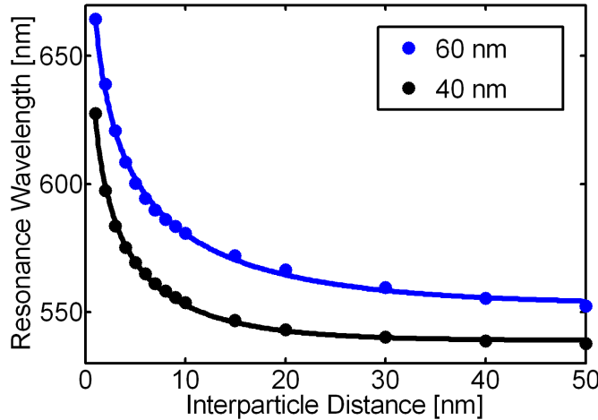
Figure 2.16: For a dimer, the resonance wavelength of the longitudinal axis depends on the interparticle distance. Here, the dependency is plotted for dimers consisting of 40 nm and 60 nm spheres in diameter simulated using the boundary element method (dots). Appropriate fit functions (solid lines) are given in equations 2.65 and 2.66 for both sizes.
