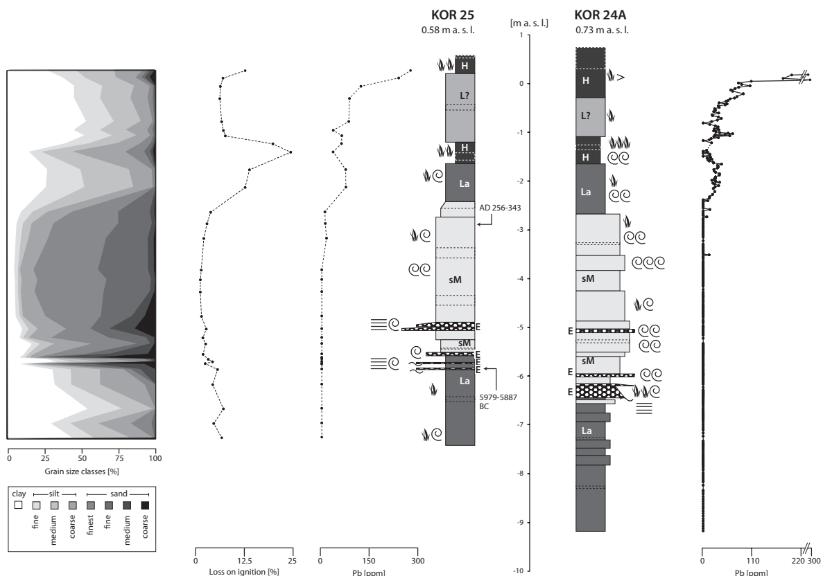
Figure 2.7: Facies classification, sedimentary features, selected geochemical parameters and grain size data of vibracores KOR 25 (left) and KOR 24A (right). For location of vibracoring sites see Figure 2.1; for explanations see text; legend according to Figure 2.2. Pb content of vibracore KOR 24A (right) was measured in situ with an average resolution of 2 cm while Pb content of vibracore KOR 25 (left) was measured with lower resolution at selected samples. In contrast to the lower lagoonal unit, the upper lagoonal mud shows distinct peaks in anthropogenic Pb content associated with high values in LOI.
