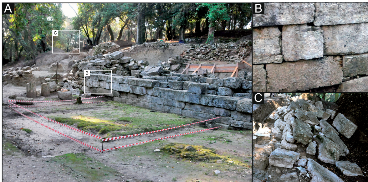
Figure 3.11: Northern retaining wall of the temple of Hera showing typical archaeoseismological features, which indicate damage by an earthquake: (A) Parts of the wall have been shifted forward, (B) single ashlars show triangle-shaped corner breakouts and (C) large wall sections imply earthquake-related dislocation in a slopeward direction. (Photos by A. Vött, 2012).
