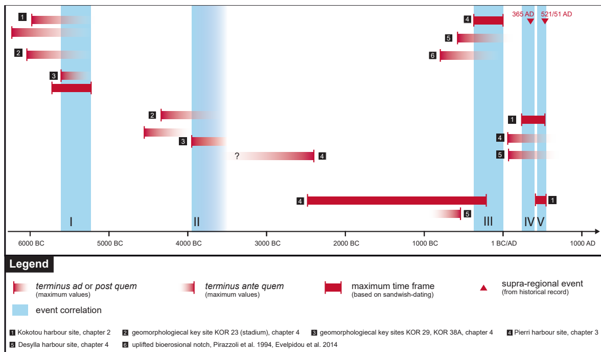
Figure 5.3: Seismic events trapped in the local geoarchives of ancient Corcyra.
