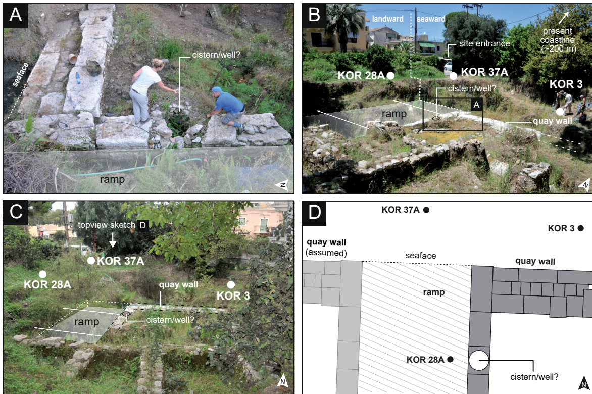
Figure 3.3: Photographic overview of the Pierri site. (A) Detailed view of the quay wall segment and vertical wall section, excavated at the Pierri site. View to the east. (B), (C) Location of vibracoring sites in relation to the Pierri quay wall and the associated ramp. View to the northwest and north, respectively. Vibracore KOR 28A was drilled on the landward side of the quay, covering the area of the assumed ramp, while vibracore KOR 3 is situated seaward right in front of the quay wall. Vibracoring site KOR 37A was drilled right in front of the assumed ramp. (D) Simplified sketch (top view, not true to scale) of the Pierri Site quay wall segment with associated ramp. (Photos by A. Vött 2012, 2013, 2014).
