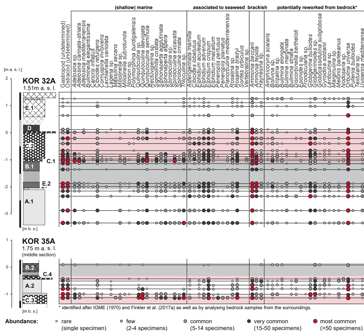
Figure 4.5: Results from microfaunal studies of selected samples collected from vibracores KOR 32A (top) and KOR 35A (bottom). Species were determined after LOEBLICH & TAPPAN (1988) and CIMERMAN & LANGER (1991) and classified according to their ecological preferences after SEN GUPTA (1999) and MURRAY (2006). Potentially reworked species of the local Neogene bedrock identified after IGME (1970) and FINKLER et al. (2016) were depicted separately. Microfaunal analysis of core KOR 32A indicates an open-marine sublittoral to littoral system with marine salinity that slightly changed into a brackish milieu in the upper part of the harbour sediments. High-energy layers C.1 and C.2 mirror the entry of first reworked harbour mud and then sublittoral sands. Moreover, microfaunal studies on KOR 35A show a clear difference between marine high-energy layer C.3 and the overlying A.2 sands, indicating the establishment of protected and brackish conditions due to protective constructions by man.
