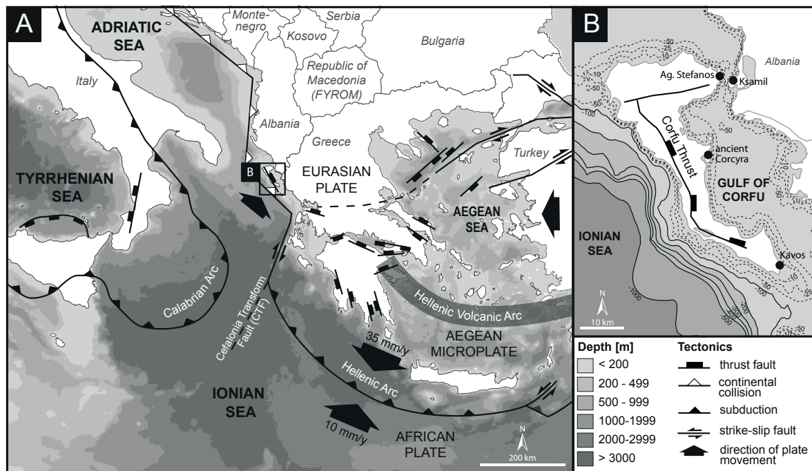
Figure 3.1: Tectonic structures and bathymetric conditions in the eastern Mediterranean. (A) Simplified tectonic map of the Ionian, Adriatic and Aegean Seas. Corfu Island (black box) is exposed to the Adriatic continental collision belt in the north, the subduction zones of the Hellenic and Calabrian Arc in the South and the Cefalonia Transform fault (CTF) right southwest of the island. Owing to compressional tectonics, the Corfu thrust as thrust fault runs across the island.
