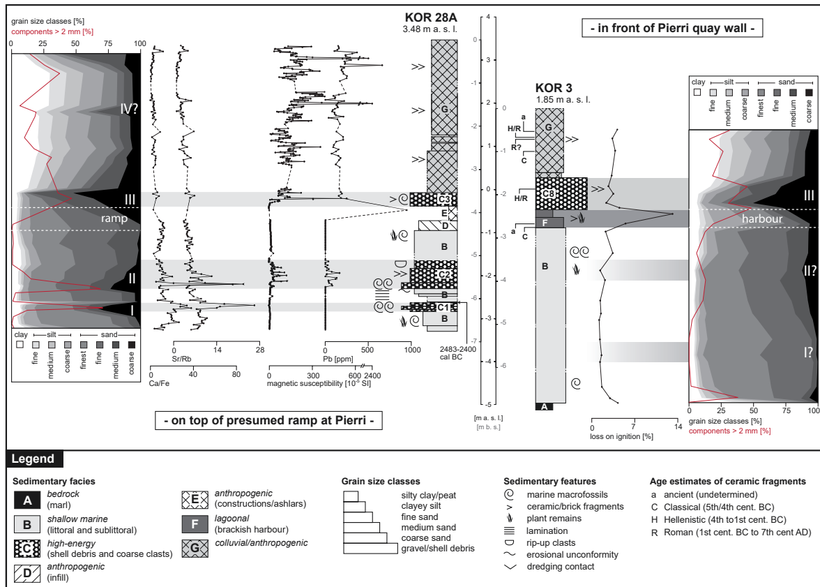
Figure 3.5: Results from grain size analysis, magnetic susceptibility measurements and selected geochemical proxies of vibracores KOR 28A (left) and KOR 3 (right). Lagoon-type harbour deposits (highlighted by dark grey colour) in vibracore KOR 3 were found in a stratigraphical position consistent with anthropogenic deposits marking most likely the base of a ramp. High-energy layers (highlighted by light grey colour) are characterised by increased amounts of medium to coarse sand but show different geochemical fingerprints.
