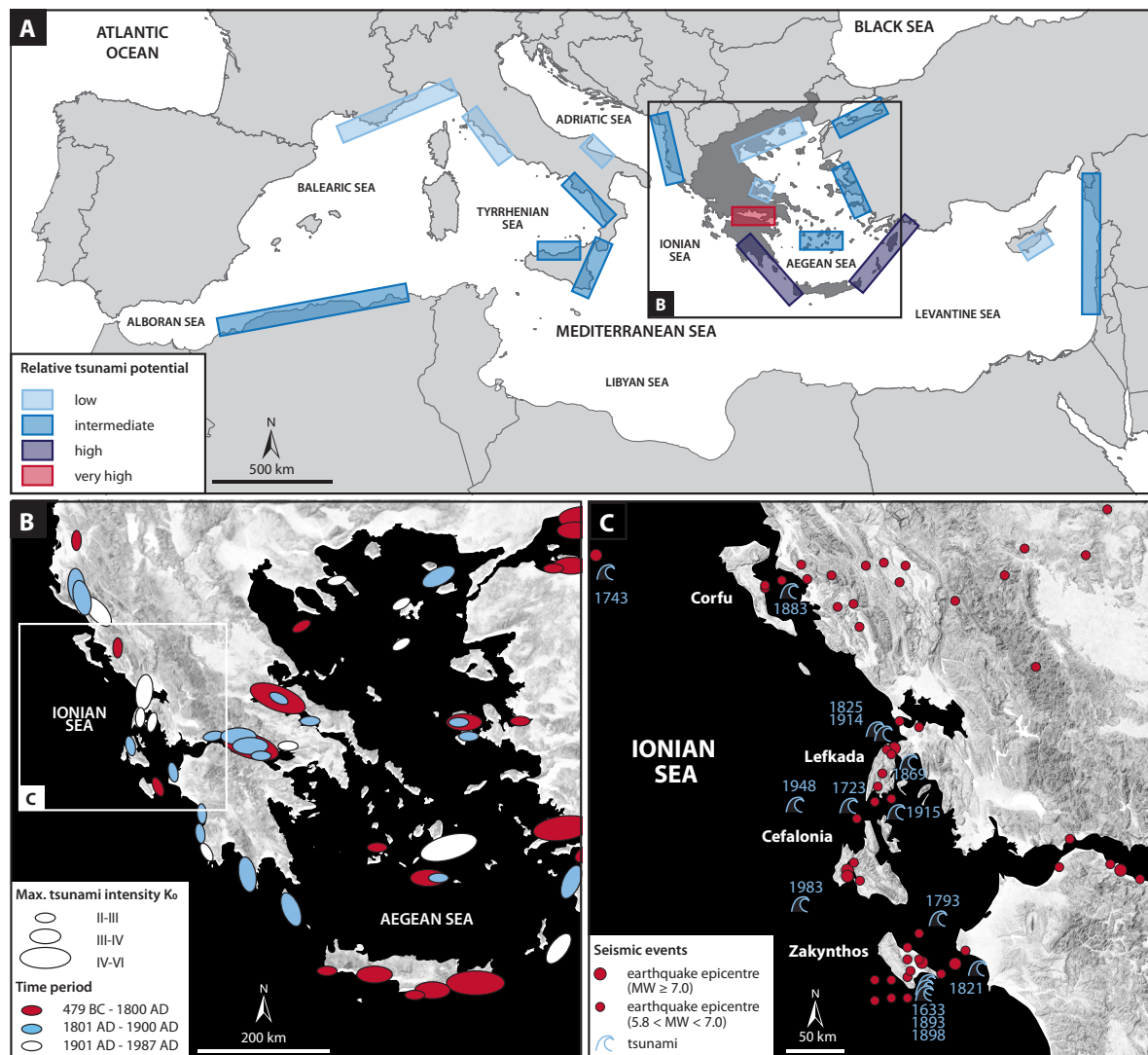
Figure 1.2: Tsunamigenic zones and tsunami events in the Mediterranean (A) Relative potential for tsunami events in the Mediterranean Sea according to documentary records showing highest tsunami risk in the Gulf of Corinth and along the Hellenic Arc (map modified after PAPADOPOULOS & PAPAGEORGIOU 2014). (B) Known and Inferred tsunamigenic zones in the Ionian and Aegean Seas compiled by PAPAZACHOS & DIMITRIU (1991). The elliptic form is orientated along the corresponding seismic fracture zone, while the size of the ellipses is proportional to the estimated maximum tsunami intensity. Colours refer to the time period, the tsunami event took place. Noticeable is the lack of pre-1800 events in the northern Ionian Sea. (C) Known tsunami events in the northern Ionian Sea as reported by modern tsunami catalogues supplemented by earthquake epicentres (red dots) from seismic events that occurred between 1000 and 1899 AD and featured moment magnitudes > 5.8 . (map adapted and modified after HADLER et al. 2012, tsunami events after PARTSCH 1887, SOLOVIEV et al. 2000, AMBRASEYS & SYNOLAKIS 2010; earthquake epicentres after STUCCHI et al. 2013)
