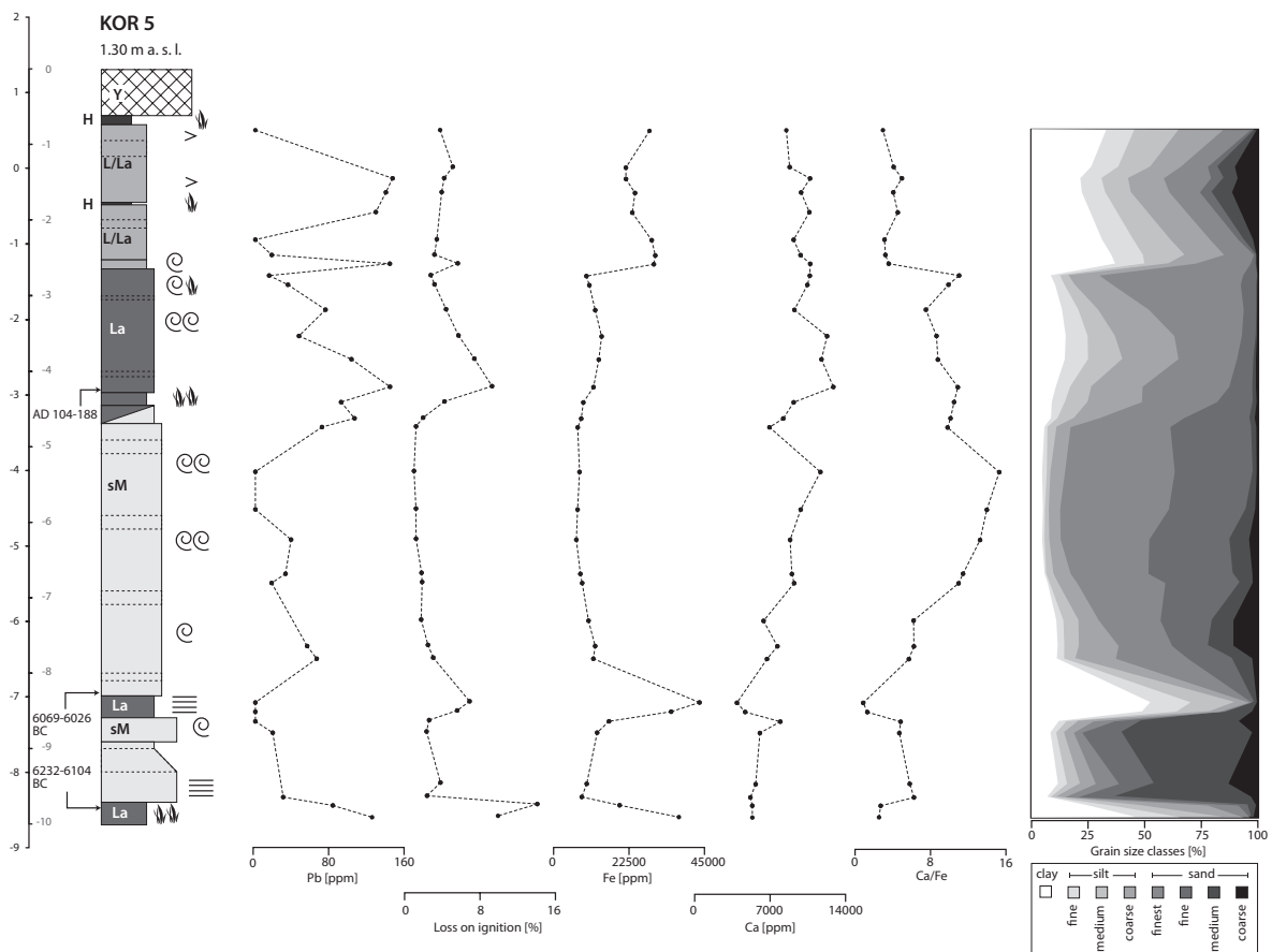
Figure 2.6: Sedimentary units and features, grain size data and selected geochemical parameters of vibracore KOR 5 from the western part of the Alkinoos Harbour basin. For location of vibracoring site see Figure 2.1, for explanations see text, legend according to Figure 2.2.
