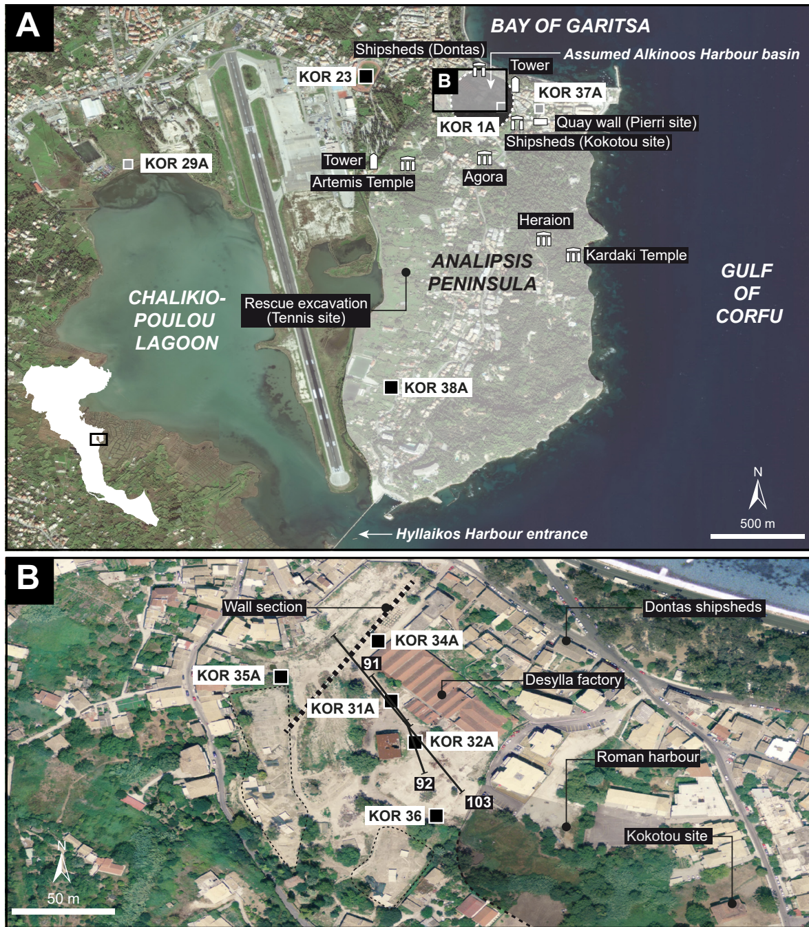
Figure 4.2: Geographical overview of the study sites on Corfu. (A) Physical setting of ancient Corcyra with main archaeological remains after BAIKA (2013a, 2015). The localisation of the Alkinoos Harbour is based on historical sources and archaeological findings. (B) Overview of the Desylla site. Vibracores of the present study are marked by black boxes, supplementary vibracores from studies by FISCHER et al. (2016a) and FINKLER et al. (2017a, 2017b) by grey boxes. Black bold lines in inlay map B refer to Electrical Resistivity Tomography (ERT) transects depicted in Figure 4.6. Maps modified after Bing aerial image of the year 2006 and NCMA S. A. (2014).
