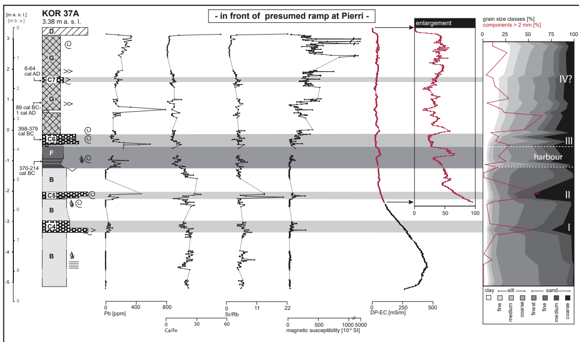
Figure 3.8: Results of grain size analysis, magnetic susceptibility measurements, Direct Push EC logging and selected geochemical proxies for vibracore KOR 37A. High-energy layers are highlighted by light grey colour and are characterised by coarser grain size and distinct peaks of Pb concentration, magnetic susceptibility values and marine ratios.
