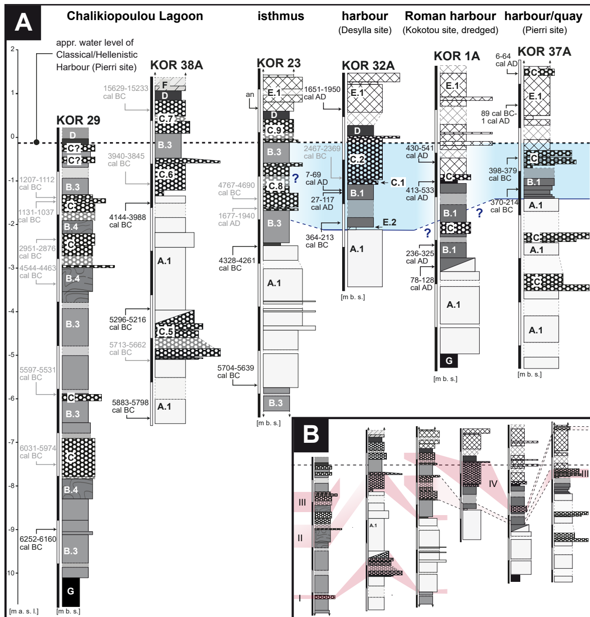
Figure 4.14: (A) Cross-section of selected vibracores from the surroundings of ancient Corcyra. Vibracores KOR 23, 32A and KOR 38A are complemented by vibracores from the Roman Alkinoos Harbour (FINKLER et al. 2017a), the Pierri quay wall site (FINKLER et al. 2017b) and the northern fringe of the Chalikiopoulou Lagoon (FISCHER et al. 2016a). Radiocarbon ages not considered for interpretation are depicted in grey (see section 4.5.3 for further explanations). Harbour sediments dating to Classical and younger times (shaded in blue) can be traced from the Pierri quay wall in the east to the Desylla site in the west. Dredging contacts (solid blue lines) document the efforts to keep the harbour navigable. (B) Impact of a pre-historical teletsunamis, a locally triggered Classical-Hellenistic tsunami and the 365 AD teletsunami can be traced all over the area. Consistent stratigraphic layers are shaded in pink colour.
