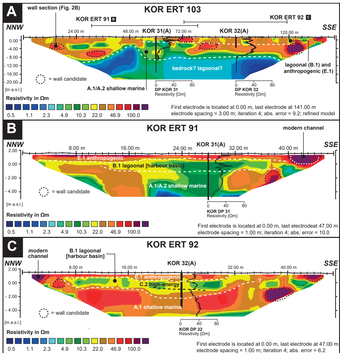
Figure 4.6: Depth sections of Electrical Resistivity Tomography (ERT) transects KOR ERT 103 (A), KOR ERT 91 (B) and KOR ERT 92 (C) carried out at the Desylla site. Electrical conductivity measurements by DP EC logging at sites KOR DP 31 and KOR DP 32 were transformed into resistivity logs and integrated into the profiles. Both, resistivity logs and ERT depth sections, clearly show a fine-grained harbour basin, thinning out towards drilling site KOR 31A. Furthermore, several distinctly delimited structures of high resistivity indicate wall structures in the subsurface, most likely related to man-made subdivisions.
