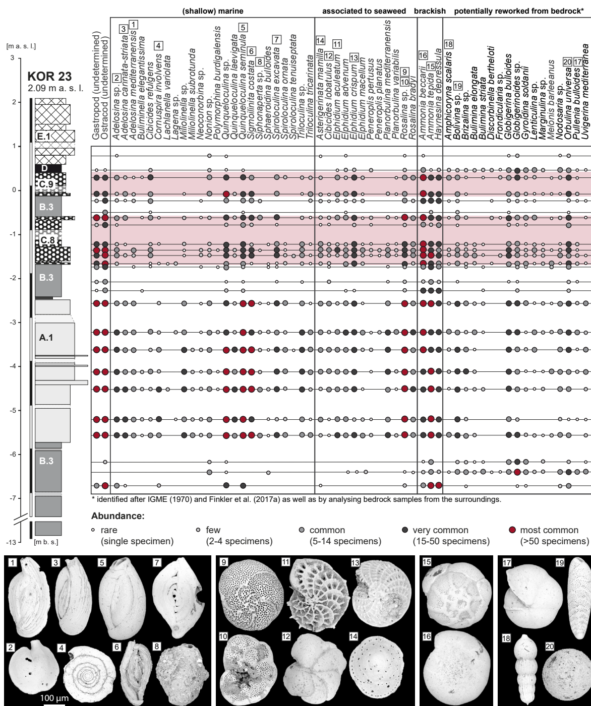
Figure 4.12: Results from microfaunal analysis of vibracore KOR 23 supplemented by SEM photographs of indicative specimens. Species were determined after LOEBLICH & TAPPAN (1988) and CIMERMAN & LANGER (1991) and classified according to their ecological preferences after SEN GUPTA (1999) and MURRAY (2006). Potentially reworked species of the local Neogene bedrock identified after IGME (1970) and FINKLER et al. (2016) were depicted separately. Foraminiferal studies prove the marine character of intersected A.1 sands. Furthermore the foraminiferal signal of both high-energy layers differs strongly from local lagoonal foraminiferal assemblages.
