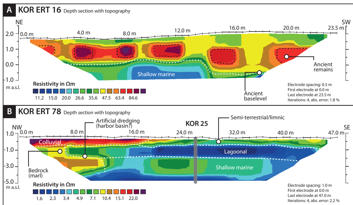
Figure 2.9: Results from Electrical Resistivity Tomography measured along transects KOR ERT 16 (A) and KOR ERT 78 (B). For location of ERT transects see Figure 2.1.
