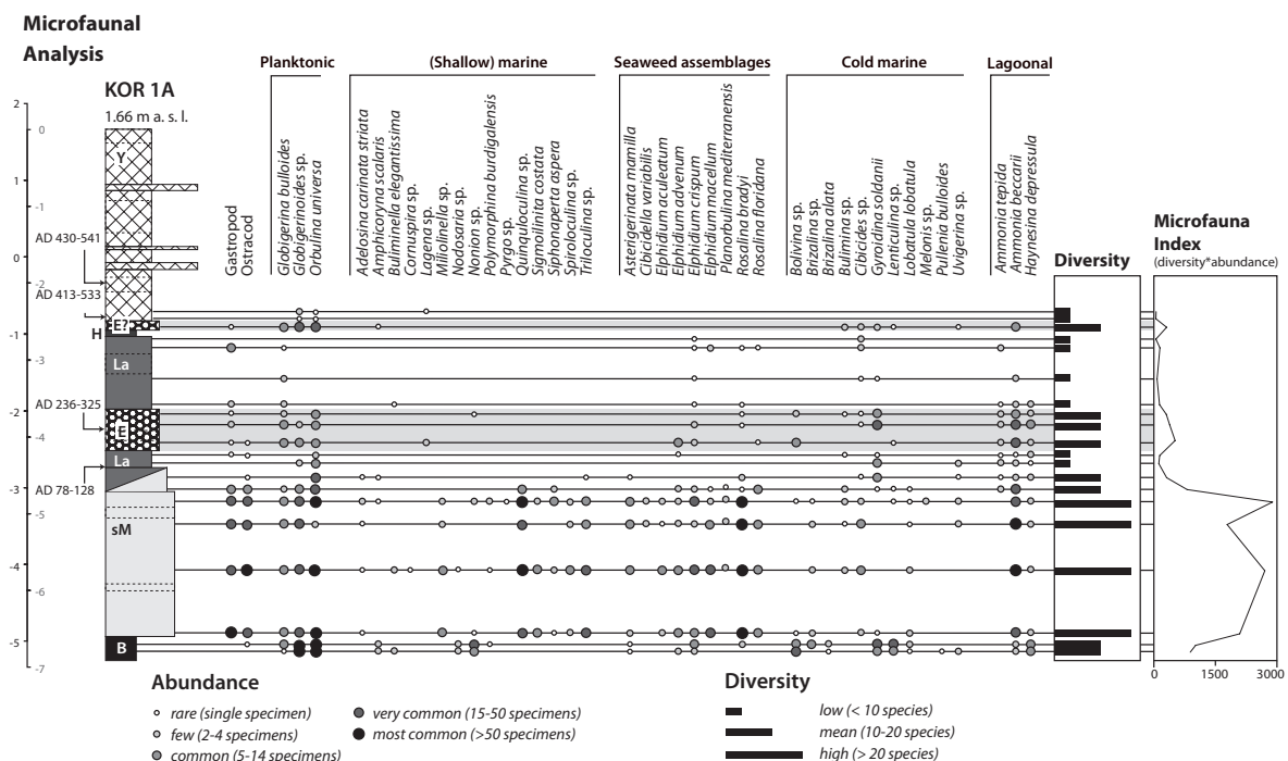
Figure 2.5: Results of microfaunal studies of selected samples from vibracore KOR 1A. For location of vibracoring site see Figure 2.1; for explanations see text and Figure 2.2. Foraminifera were determined after LOEBLICH & TAPPAN (1988) and CIMERMAN & LANGER (1991) and are classified according to their ecological preferences after MURRAY (2006) and SEN GUPTA (1999). Note the difference in abundance, diversity and species between the autochthonous lagoonal deposits and the intersecting high-energy layers.
