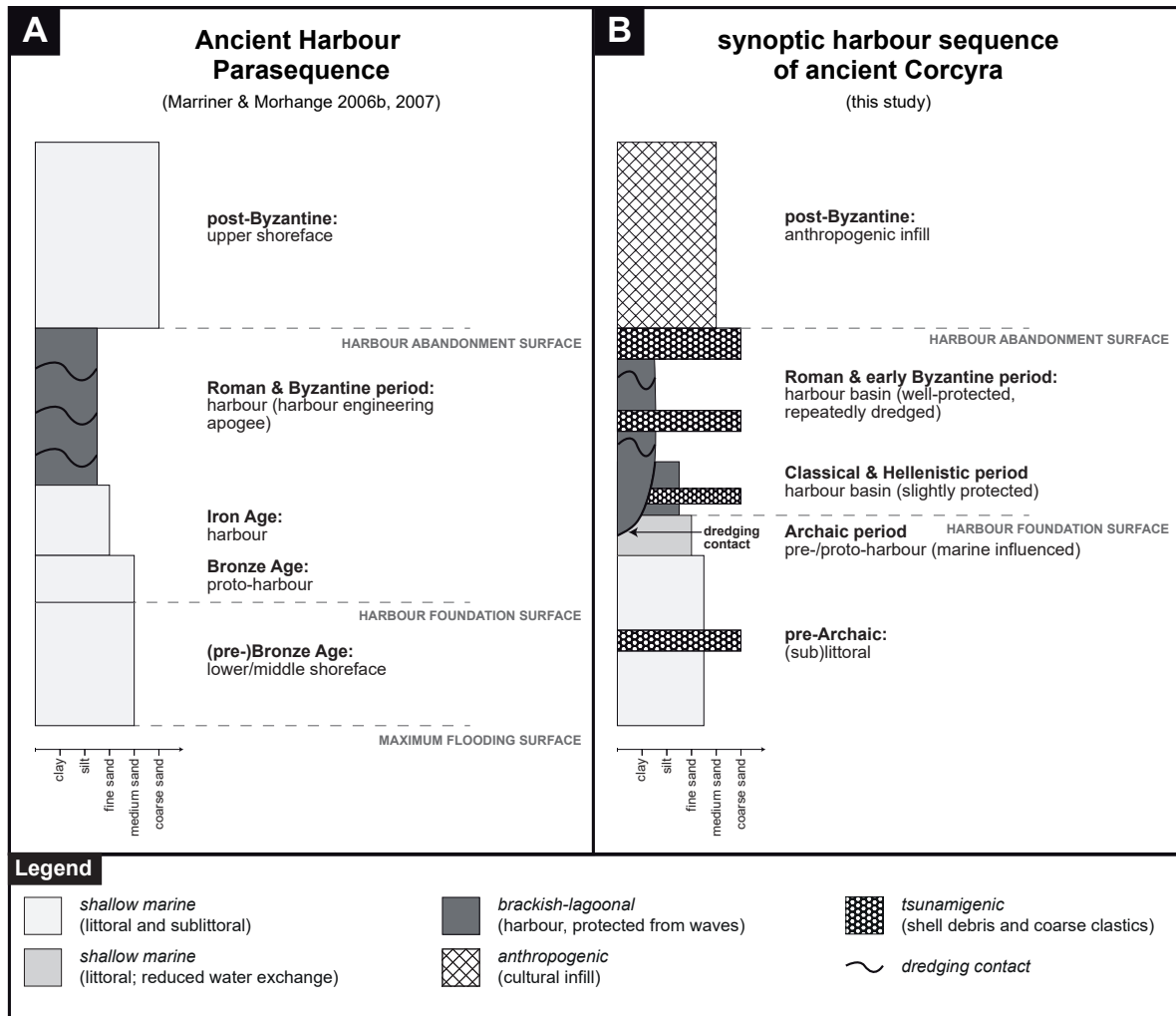
Figure 5.1: The harbour sequence of Corcyra in the Mediterranean context. (A) Lithostratigraphical features of the Ancient Harbour Parasequence deduced from general observed stratigraphic patterns in ancient Mediterranean harbours by Marriner & Morhange (2006b, 2007). (B) Synoptic and summarised harbour sequence of the ancient harbours of Corcyra based on the findings presented in this study.
