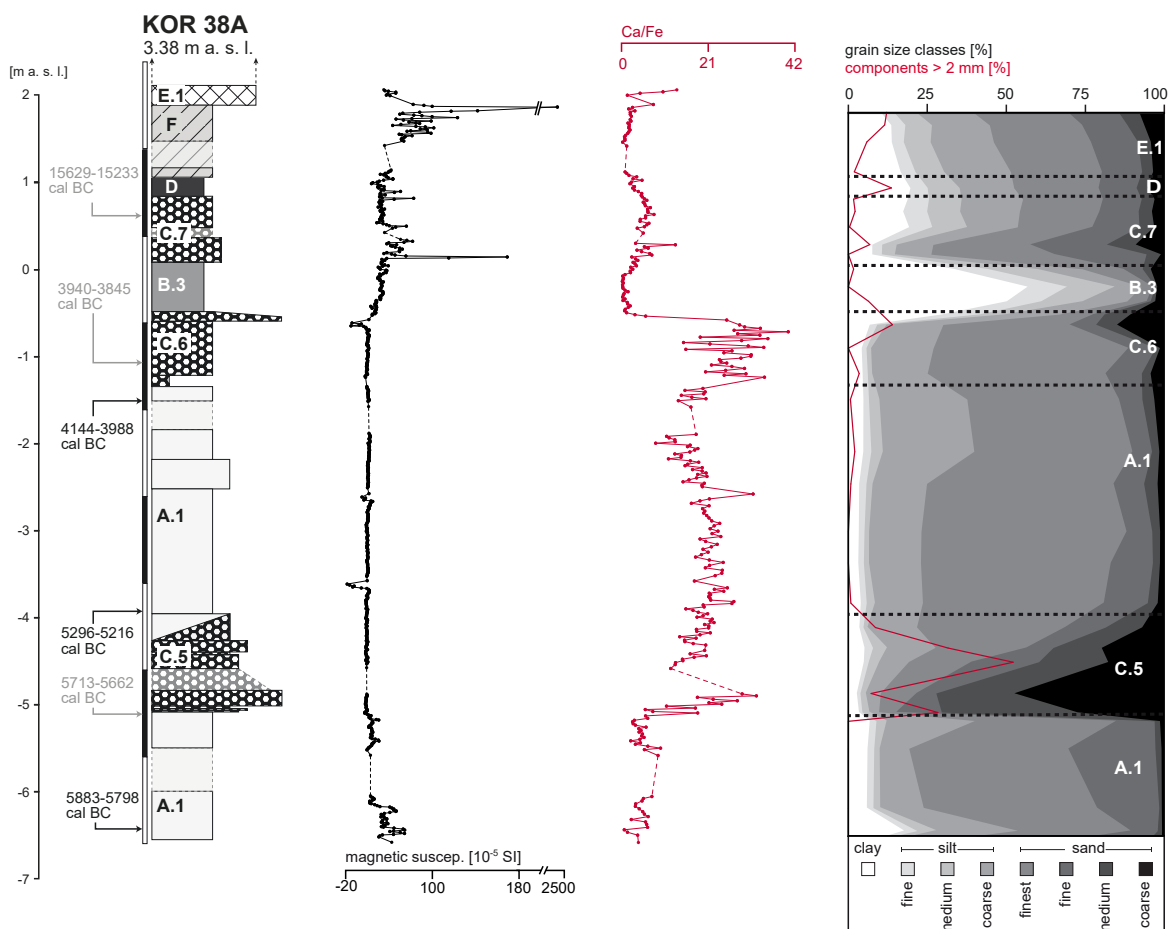
Figure 4.8: Results from multi-proxy analyses of samples from vibracores KOR 38A. Legend according to Figure 4.4. Intersected high-energy layers C.5 to C.7 distinctly differ from under- and overlying shallow marine sands due to the entry of coarse and medium sand as well as increased Ca/Fe values.
