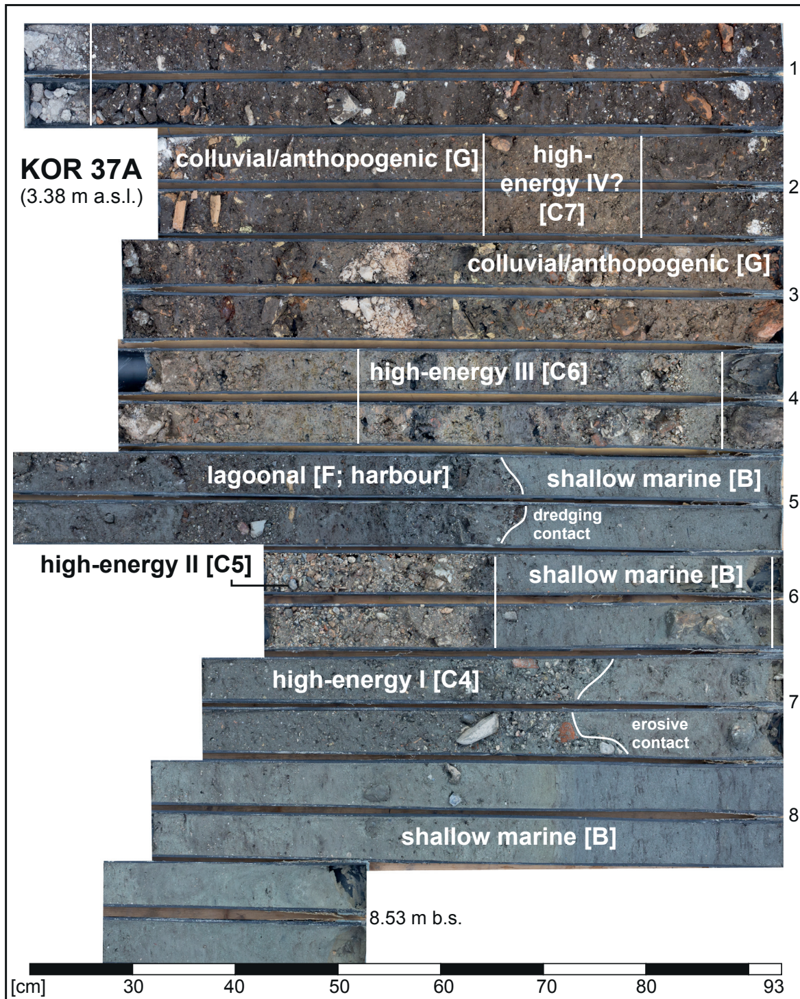
Figure 3.7: Stratigraphical record of vibracore KOR 37A. Shallow marine sands show intersected high-energy layers and are followed by thick colluvial to anthropogenic deposits. Harbour deposits (4.63–4.17 m b.s.) are characterised by an abrupt increase of silt content and contain stones, ceramic fragments and organic material. Capital letters B–G represent associated stratigraphical units described in the results chapter.
