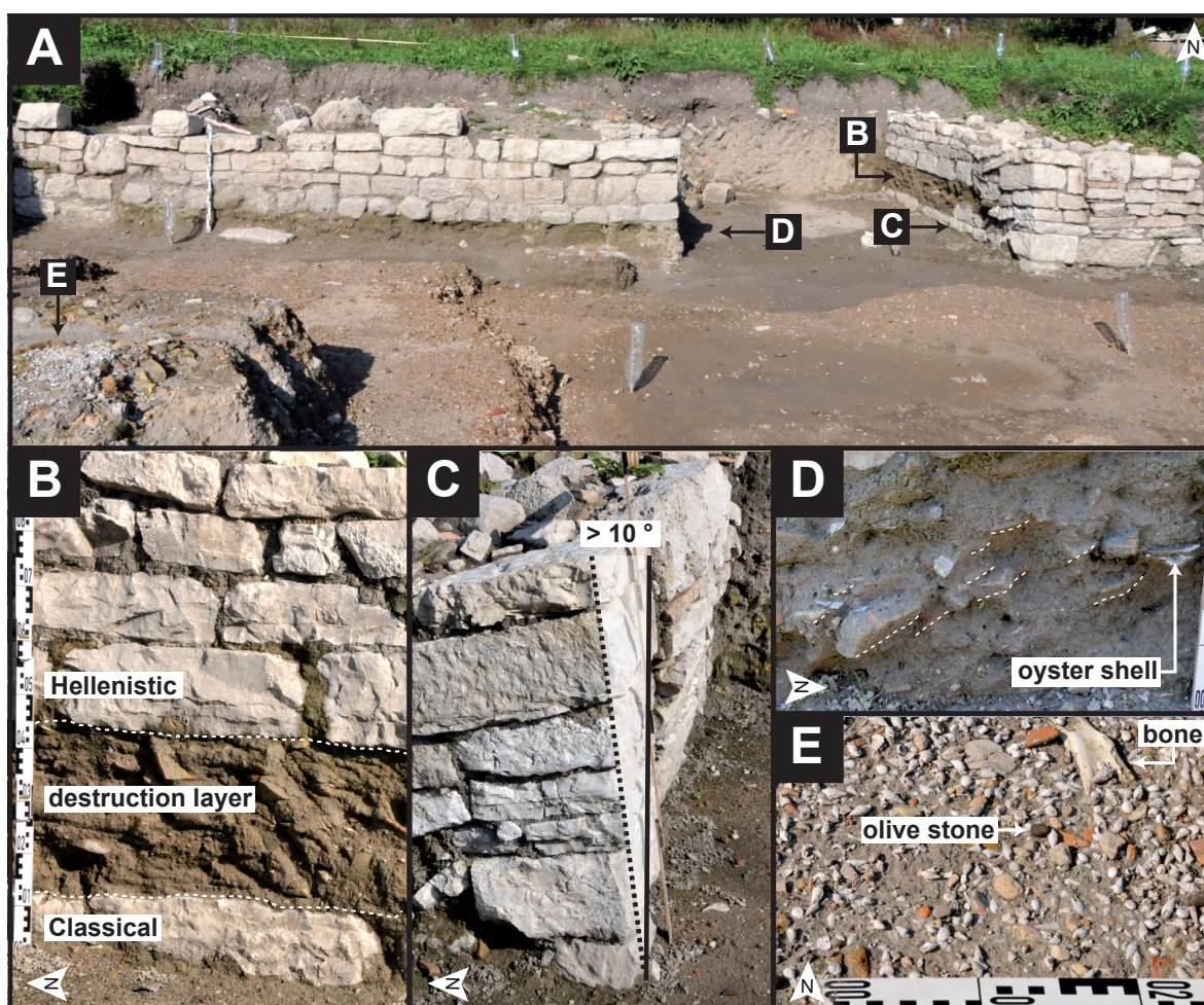
Figure 4.9: Rescue excavation site on the eastern shore of the Chalikiopoulou Lagoon. (A) Archaeoseismical traces of a strong local seismic event at a rescue excavation, situated on the eastern coast of the Chalikiopoulou Lagoon. A destruction layer, made of reworked lagoonal mud with embedded marine specimens and cultural debris (E) was found on top of a Classical foundation. After the event the building was rebuilt in Hellenistic times (B). Furthermore, strong tilted walls (C) and imbrication of ceramic sherds and oyster shells (D) indicated an abrupt seismic impulse and subsequent flooding of the site.
