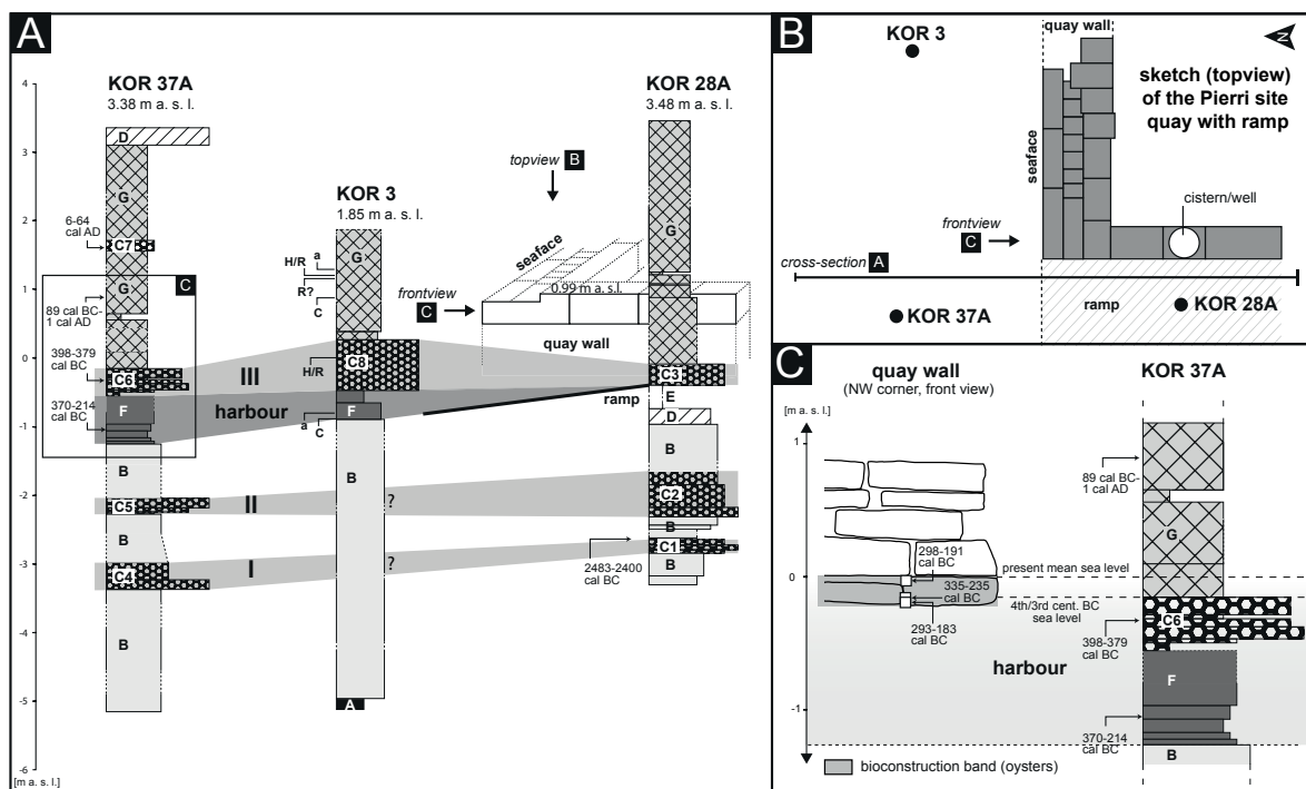
Figure 3.10: (A) Cross-section of all vibracores retrieved at the Pierri site with simplified facies pattern and ^{14}\text{C} ages. Note the location of the Pierri quay wall (only true to scale in vertical direction) with associated harbour sediments and ramp. (B) Simplified sketch (top view) of the Pierri site quay and locations of the vibracores depicted in A. (C) Sketch of the northwestern corner of the quay wall segment (front view) compared to the associated stratigraphy of vibracore KOR 37A (please see A for detailed section). Oyster bioconstruction band adhesive to the lower Pierri quay wall ashlar is depicted by grey colour, oyster samples that were radiocarbon dated are marked by white rectangles. The overall time span when oysters were alive was found to be 335-183 cal BC which is in accordance with the archaeological age of the harbour, dated to Classical-Hellenistic times (RIGINOS et al. 2000). Legend according to Figure 3.5.
