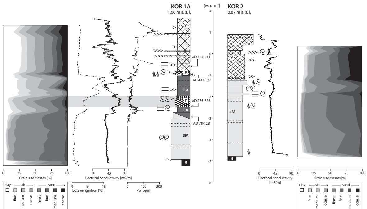
Figure 2.4: Results of multi-proxy analyses of vibracores retrieved from the Alkinoos Harbour showing facies classifications, sedimentary features, electrical conductivity, selected geochemical parameters and grain size data of vibracores KOR 1A (left) and KOR 2 (right). For location of vibracoring sites see Figure 2.1; legend according to Figure 2.2; see text for further explanation.
