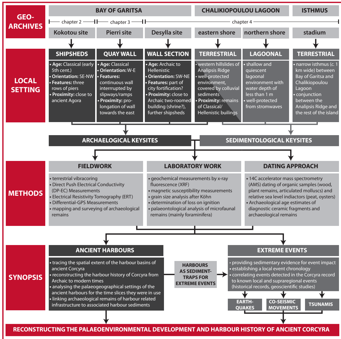
Figure 1.5: Conceptual framework and research design of the present study. Depicted are the main study areas with their local archaeological or geomorphological settings, the general methodological approach as well as the content-related key aspects.
