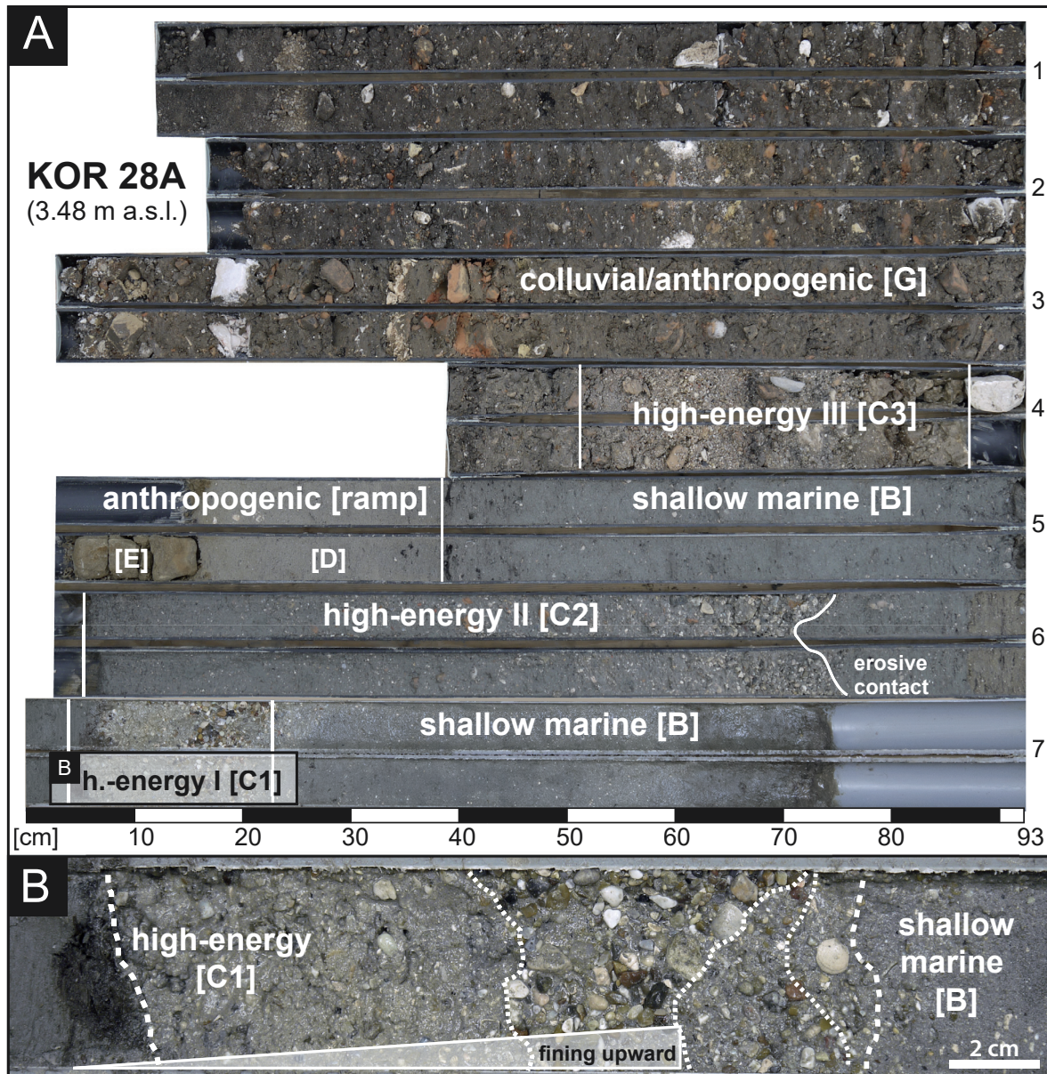
Figure 3.4: Stratigraphical record of vibracore KOR 28A. (A) On top of a thick unit of shallow marine sand, intersected by two high-energy layers (I and II), a solid ashlar out of calcareous sandstone and underlying homogeneous fine sand mark the base of the ramp at the Pierri site. It is covered by sediments of a high-energy facies (event III) and subsequent sediments of colluvial to anthropogenic origin. Capital letters B-G represent associated stratigraphical units; see text for explanation. (B) Detailed photo of high-energy deposits (event I, 6.61-6.06 m b.s) intersecting shallow marine sands. Mark the fining upward tendency in grain size and the peat-like sediments on top.
