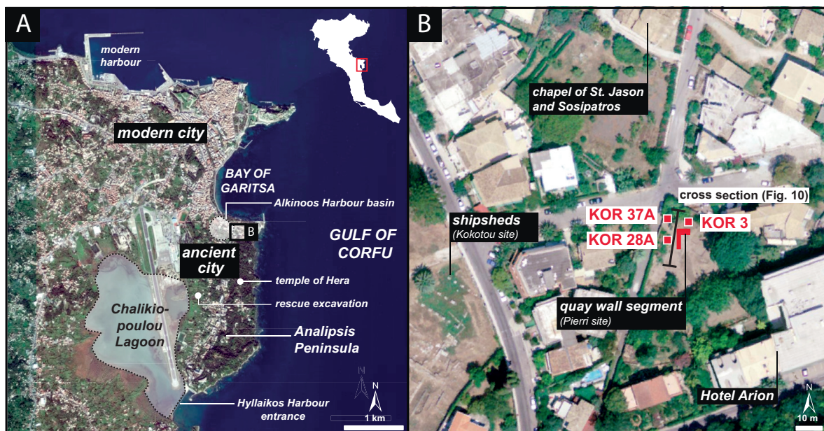
Figure 3.2: Topographic overview and detailed map of the study area. (A) Corfu city is situated at the eastern shore of the island and separated from the Greek and Albanian mainland by the Gulf of Corfu. Ancient Corcyra was built on the Analipsis Peninsula between the Chalikiopoulou Lagoon in the southwest and the Bay of Garitsa in the north. (B) The area associated with the ancient Alkinoos Harbour, traced by archaeological remains of shipsheds (Kokotou site), lies c. 200 m distant to the present coastline. At the Pierri site, remains of a quay wall document the use as a harbour (BAIKA 2013a). Vibracoring sites are marked by red rectangles. Map modified after BING AERIAL (2016) and NCMA S.A. (2014).
