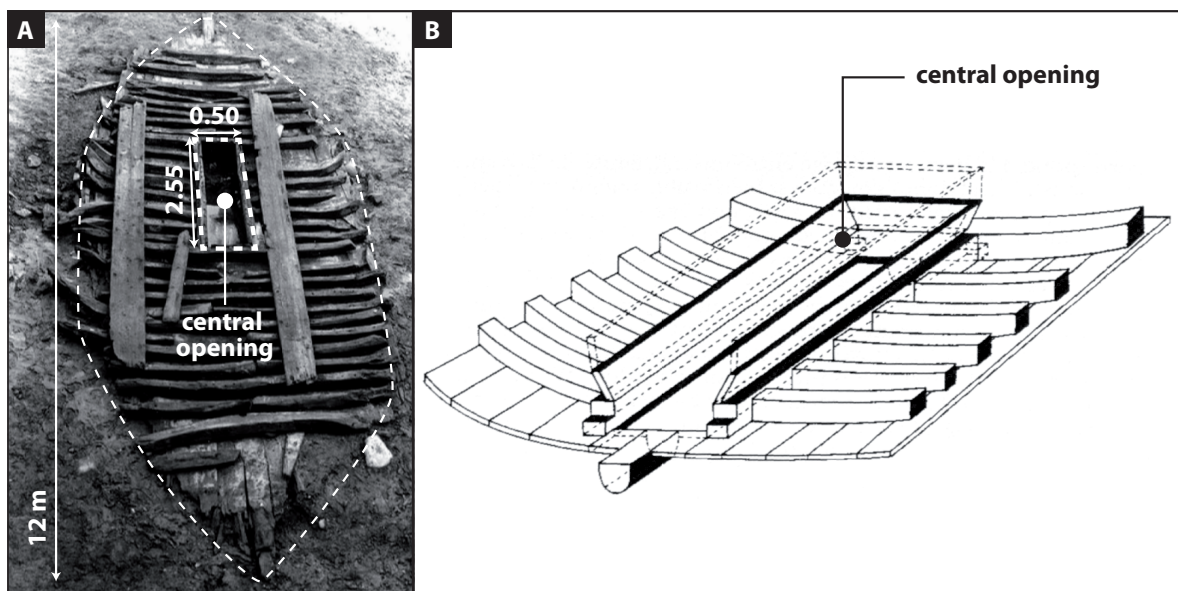
Figure 1.3: Roman dredging vessel. (A) Photograph of shipwreck Jules Verne 3 excavated in the ancient harbour of Marseille. The wreck dates to the 1 st to 2 nd century AD and is characterised by a rectangle-formed structure in the centre, opening the hull towards the sea. (B) Reconstruction of a Roman dredging vessel based on shipwreck Jules Verne 5, including fragments of planks that originally formed an inner casing around the central opening of the hull (adapted and modified after POMEY 1995).
