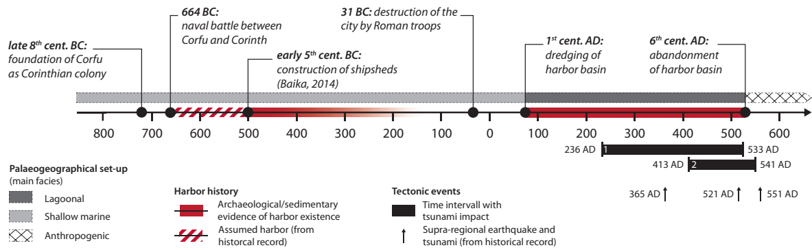
Figure 2.10: Schematic timeline with the main historical events concerning ancient Corfu and major geoarchaeological findings from this study. The pre-Roman Alkinoos Harbour naval installations were built on a sandy seashore. The Roman Alkinoos Harbour, a sheltered and quiescent basin, was used between the late 1 st and early 6 th cent. AD. It experienced two high-energy events related to tsunami landfall between the late 3 rd and the early 6 th cent. AD, most probably associated to the supra-regional 365 AD and 521/551 AD events, respectively.
