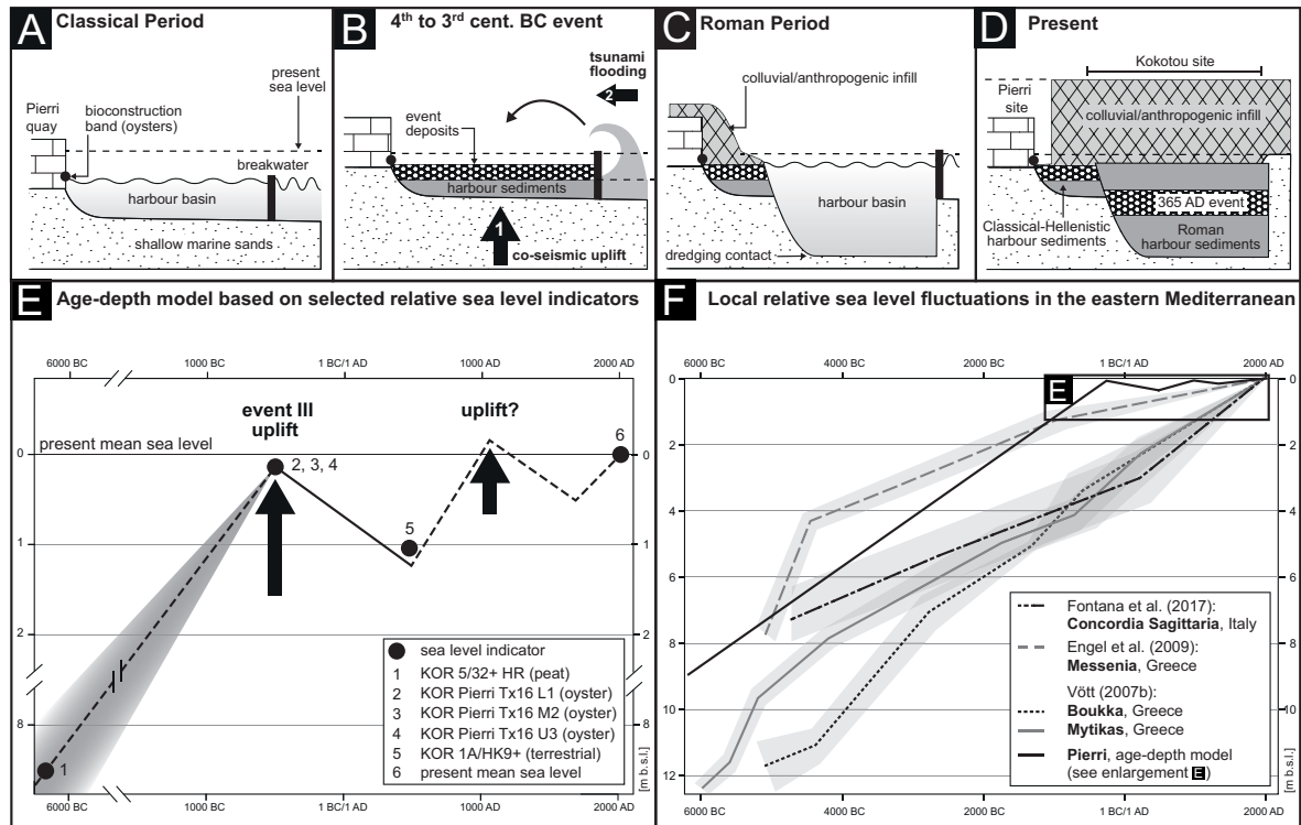
Figure 3.12: Schematic palaeoenvironmental development of the Pierri harbour site. (A) The harbour of the Classical period developed from shallow marine conditions by protective harbour infrastructure, possibly breakwaters. Oyster colonisation marked the approximate relative sea level at that time, resulting in a water depth of c. 1.2 m. (B) Between the 4 th and 3 rd cent. BC, the site experienced (i) co-seismic uplift causing decreasing water depths in the harbour, and, shortly afterwards, (ii) associated tsunami inundation. Due to co-seismic uplift and input of event deposits, the Classical-Hellenistic harbour was not navigable anymore. (C) During the Roman period, considerable parts of the buried Classical basin were deeply excavated, dredged and re-used, forming a more than 2 m deep harbour basin to the west of the Pierri site (FINKLER et al. 2017a). Comparing depths of the Classical and Roman harbour basins clearly reveals co-seismic uplift. (D) Today, harbour sediments of the Pierri site are covered by colluvial and anthropogenic material. Classical harbour infrastructure in form of a quay wall was found during archaeological excavations. (E) Age-depth model of selected relative sea level indicators from the Pierri site. Marine oysters dating to 335-183 cal BC were found on higher elevations than younger terrestrial material which causes a clear shift within the age-depth model. This break documents the co-seismic uplift of the Pierri site related to tsunami inundation of event III that occurred during Classical to Hellenistic times. It may be speculated that the time of dieback of oysters that took place between 335-183 cal BC represents the best-fit age estimate for this event. (F) Local relative sea level curves from different study sites in the eastern Mediterranean compared to relative sea level indicators encountered at the Pierri site.
