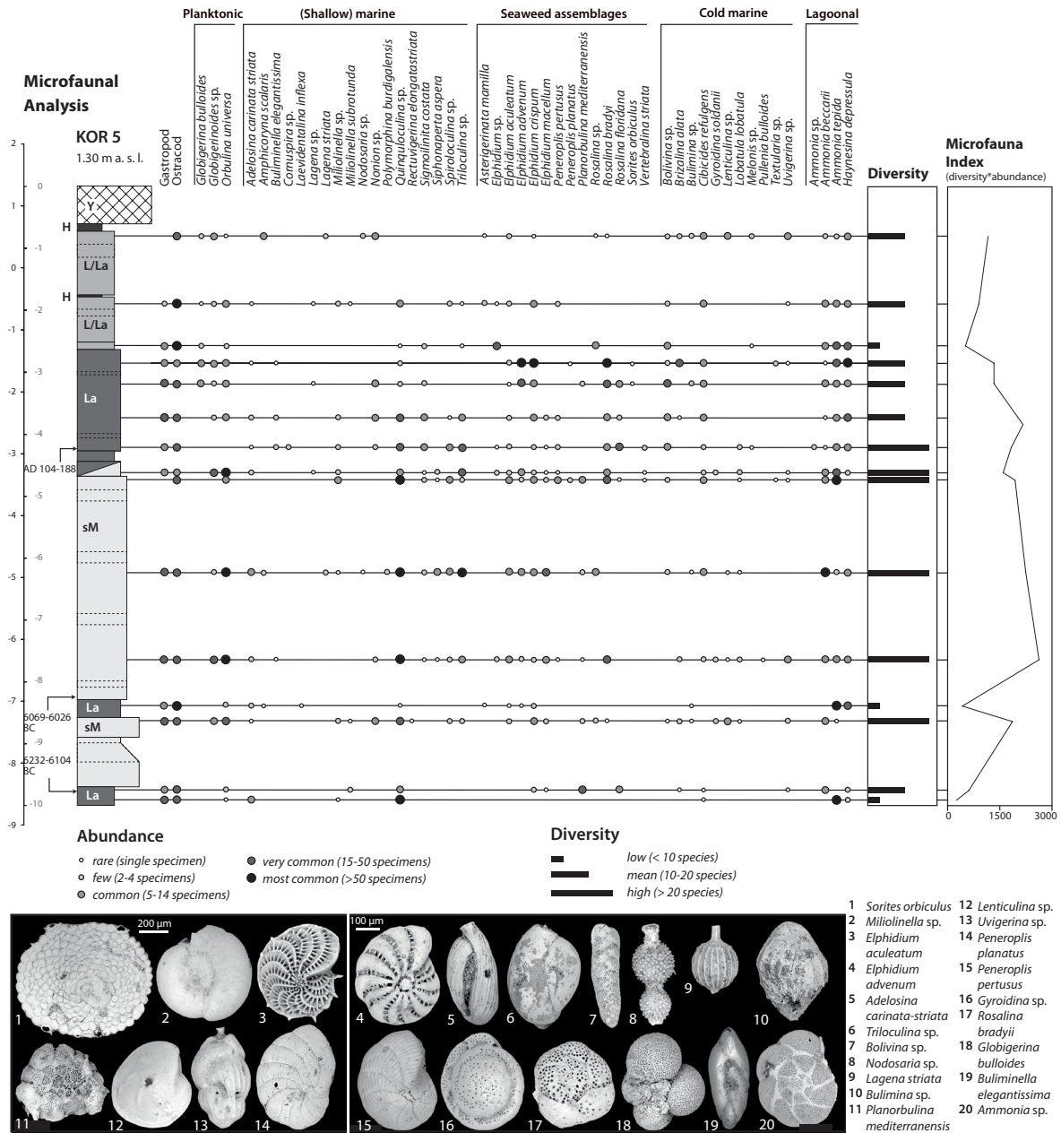
Figure 2.8: Results of microfaunal studies of selected samples from vibracore KOR 5. For location of vibracoring site see Figure 2.1; for explanations see text; legend according to Figure 2.2. Photos of selected samples were taken using a scanning electron microscope (SEM). Foraminifera species were determined after LOEBLICH & TAPPAN (1988) and CIMERMAN & LANGER (1991) and are classified according to their ecological preferences after MURRAY (2006) and SEN GUPTA (1999). Note the different foraminiferal fingerprint of the upper lagoonal unit (high diversity, high abundance) compared to the lower lagoonal deposits which are characterized by a distinct lower abundance and diversity.
