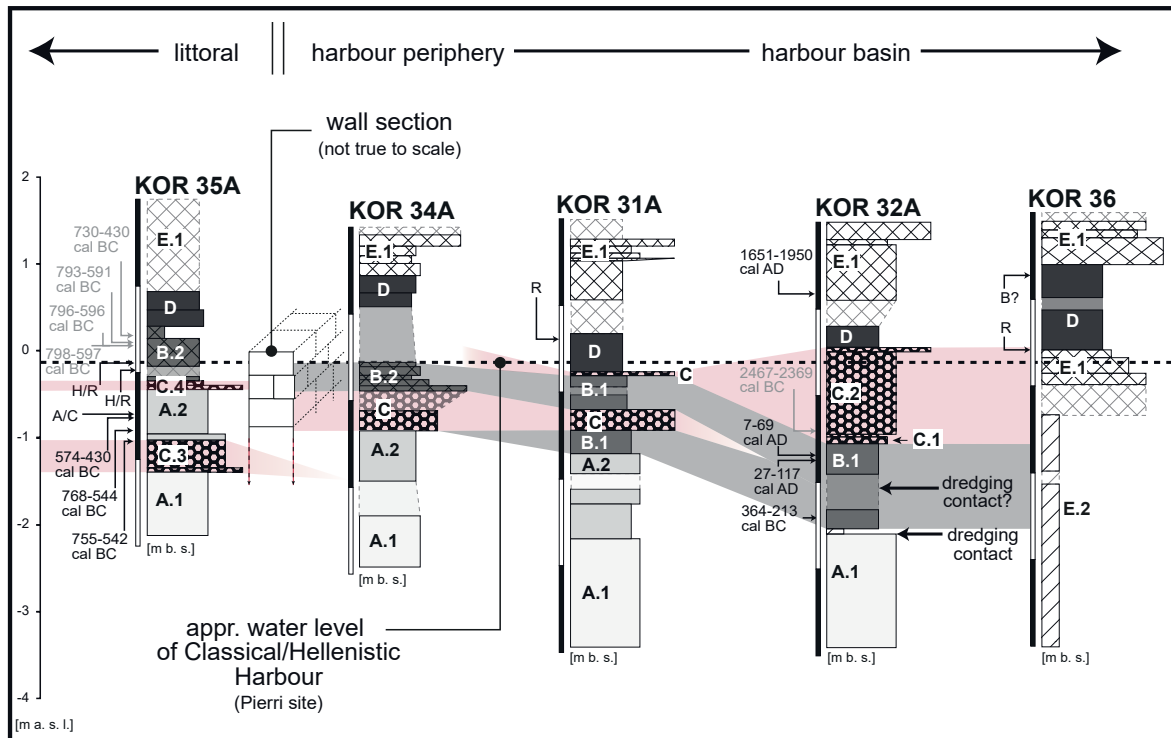
Figure 4.13: Cross-section of vibracores drilled at the Desylla site with simplified facies pattern and radiocarbon ages. Ages not considered for interpretation are depicted in grey (see section 4.5.3 for further explanations). Legend according to Figure 4.4. Sea level reconstruction for Pierri Harbour based on radiocarbon dating of sea level indicators (see section 5.3 and FINKLER ET AL. 2017b). A thick wall excavated between vibracoring sites KOR 34A and KOR 35A marks the western delimitation of the harbour basin which was found c. 2 m deep at site KOR 32A. Shallow marine conditions prevailed at site KOR 35A beyond the wall. Event layers of Pre-Archaic, Classical/Hellenistic and Roman age are included in the Desylla record.
