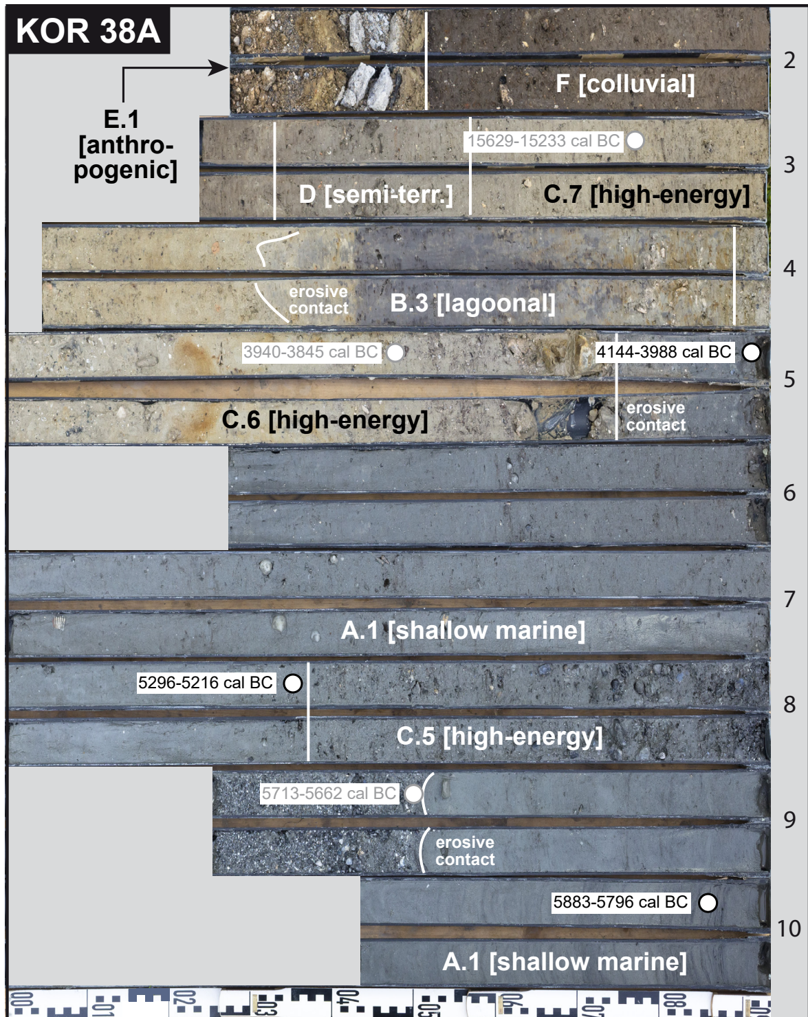
Figure 4.7: Sedimentary record and main stratigraphic units of vibracore KOR 38A, drilled at the western shore of the Analipsis Peninsula. Radiocarbon samples and associated ages (1 \sigma confidential interval) are marked by white dots. Ages not considered for interpretation are depicted in grey (see section 4.5.3 for further explanations). The vibracore is dominated by homogenous shallow marine sands followed by first lagoonal and semi-terrestrial but later colluvial deposits. Following sharp erosional contacts, high-energy sediments were deposited associated with extreme wave impact and extraordinarily high flow velocities mirrored by significant coarse grain size (C.5, C.6) and a mixing of autochthonous lagoonal mud with allochthonous marine sands (C.7).
