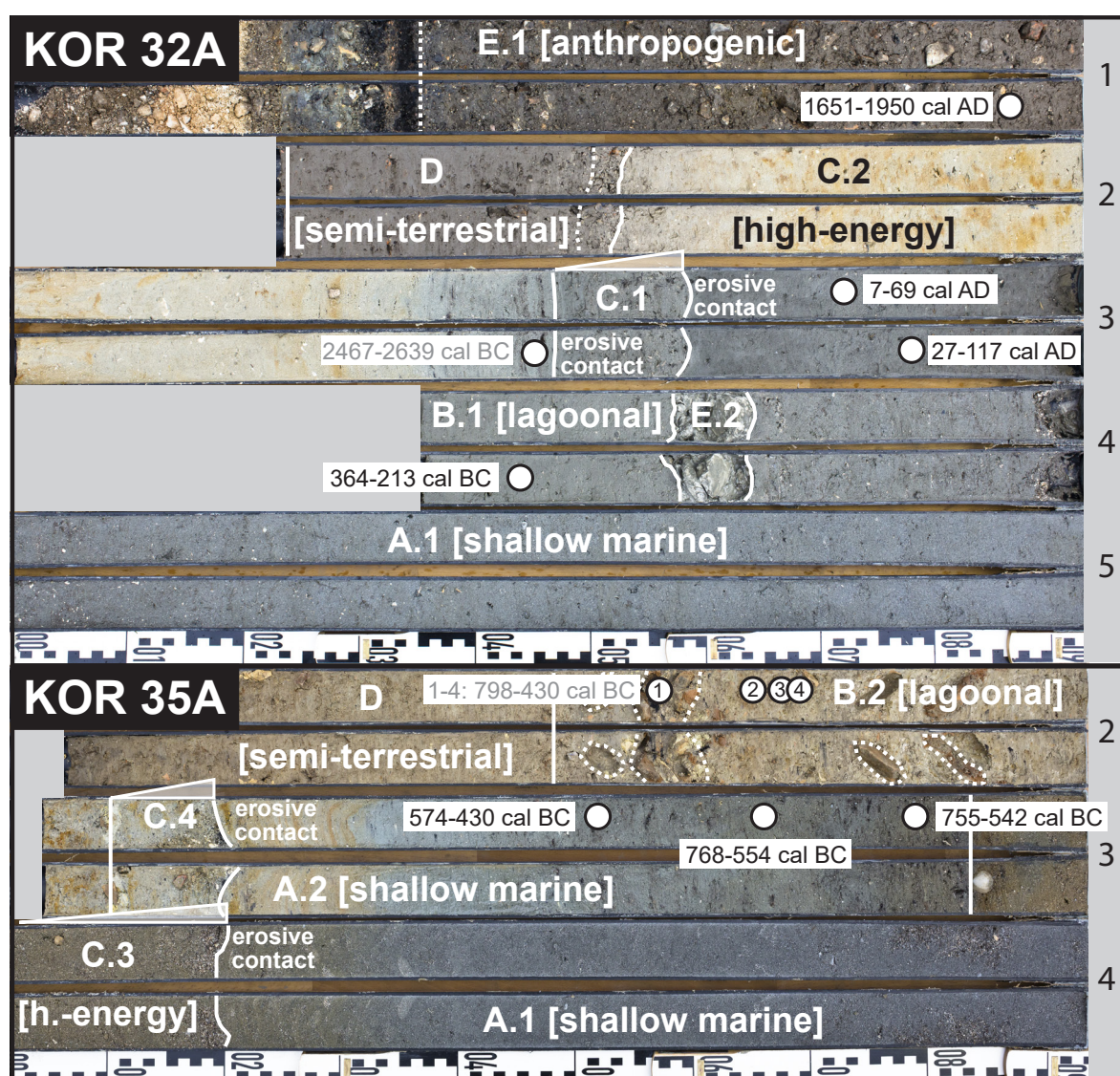
Figure 4.3: Sedimentary records and main stratigraphic units of vibracores KOR 32A and KOR 35A, drilled in the area of the former Desylla rope factory. Radiocarbon samples and associated ages ( 1\sigma confidential interval) are marked by white dots. Unreliable dates (see section 4.5.3 for further explanations) are depicted in grey. Both vibracores are characterised by first shallow marine and later lagoonall deposits and include several high-energy layers related to extreme wave events. In the upper part of both profiles silting processes are represented by semi-terrestrial deposits, which are buried under anthropogenic infill in vibracore KOR 32A.
