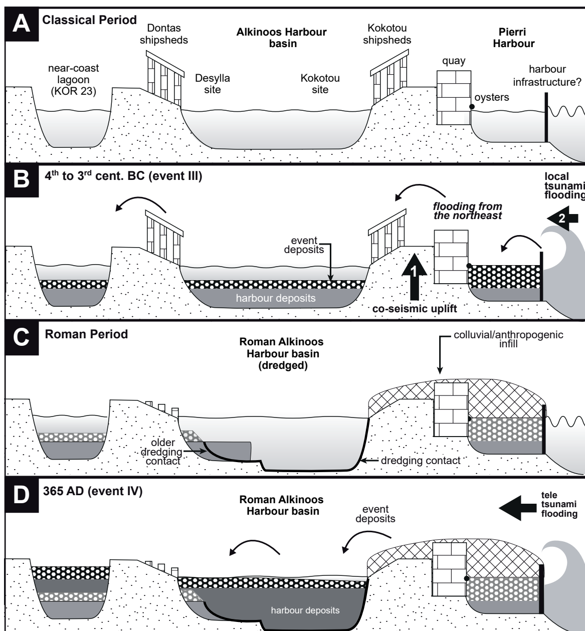
Figure 4.15: Schematic palaeoenvironmental development of ancient Corcyra and its harbours. (A) During the Classical period the Alkinoos Harbour extended from the Desylla site in the northwest towards the Kokotou shipsheds in the southeast and the Pierri quay towards the present coastline. (B) Triggered by a local earthquake, co-seismic uplift occurred between the 4 th and 3 rd cent. BC (event III) leading to decreased water depth within the harbour basins and natural lagoons. A subsequent tsunami hit the Bay of Garitsa filling the harbour basins with event deposits and breaching the barrier system at vibracoring site KOR 23. (C) During Roman times, a part of the former Alkinoos Harbour was dredged and re-used, while the Pierri site was buried under colluvial and anthropogenic infill. (D) Between the 3 rd and early 6 th cent. AD, most probably in 365 AD, a supraregional teletsunami hit Corcyra (event IV), leaving thick event deposits in the Roman harbours and lagoons (FINKLER et al. 2016a).
