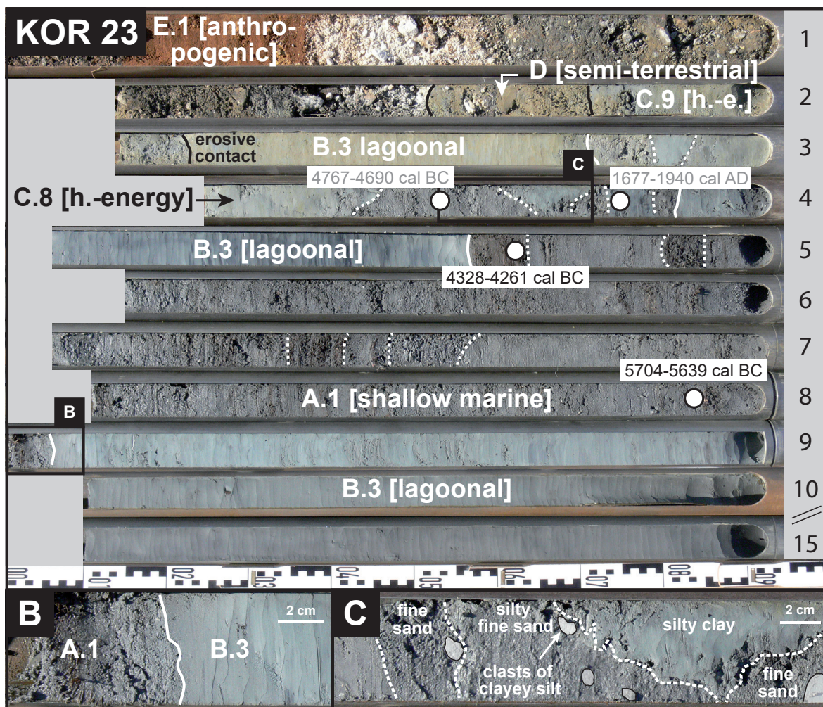
Figure 4.10: Stratigraphical record and simplified facies profile of vibracore KOR 23 retrieved at the narrow isthmus between the modern city of Corfu and the Analipsis Peninsula. Please note that the profile was shortened. The profile meters not depicted do not differ from profile meter ten. Radiocarbon samples and associated ages (1 \sigma confidential interval) are marked by white dots. Unreliable dates (see section 4.5.3 for further explanations) are depicted in grey.
