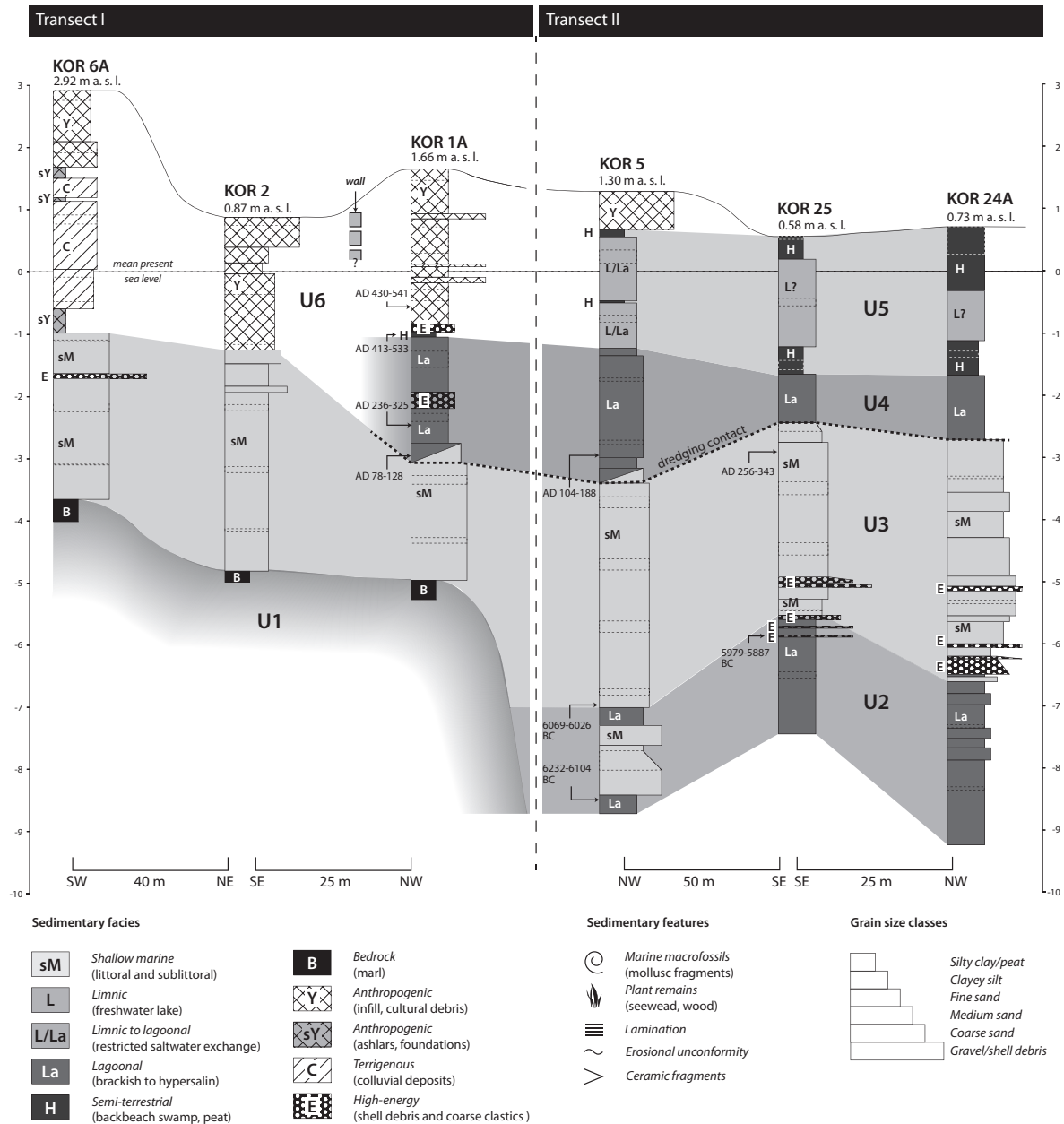
Figure 2.2: Simplified facies patterns found for vibracore Transect I (left) and II (right). For location of vibracoring sites see Figure 1. All radiocarbon ages are calibrated at 1 \sigma (see Table 2.1).
