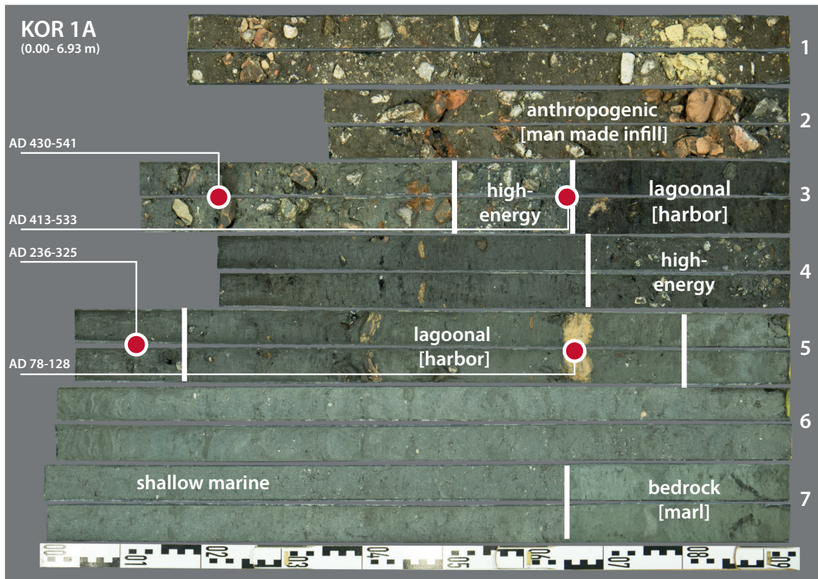
Figure 2.3: Photo of vibracore KOR 1A with the main stratigraphic units and radiocarbon ages (red circles; ages are 1\sigma values calibrated with Calib 7.0, see Table 2.1). For location of vibracoring site see Figure 2.1. Note the fine-grained, organic-rich lagoonal deposits, representing a harbour lagoon, which are interrupted and followed by coarse-grained high-energy layers.
