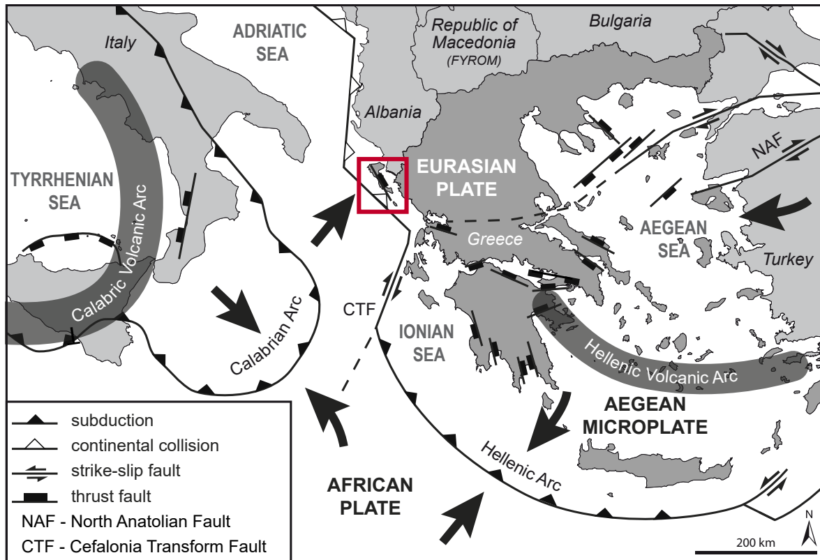
Figure 4.1: Simplified geotectonic setting of the eastern Mediterranean, including the Ionian, Adriatic and Aegean Seas. Corfu Island (red box) is located within a seismic stress field between the subduction zones of the Hellenic and Calabrian Arcs, the Adriatic collision belt and the Cefalonia Transform Fault. On Corfu, the Corfu thrust mirrors strong compressional tectonics. Main tectonic structures were simplified after Doutsos & Kokkalas (2001) and Billi et al. (2007).
