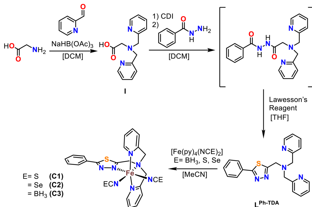
Fig. 1 Multi step synthetic scheme for synthesis of 1-(5-phenyl-1,3,4-thiadiazol-2-yl)- N,N -bis(pyridine-2-ylmethyl)methanamine ( \text{L}^{\text{Ph-TDA}} ).
