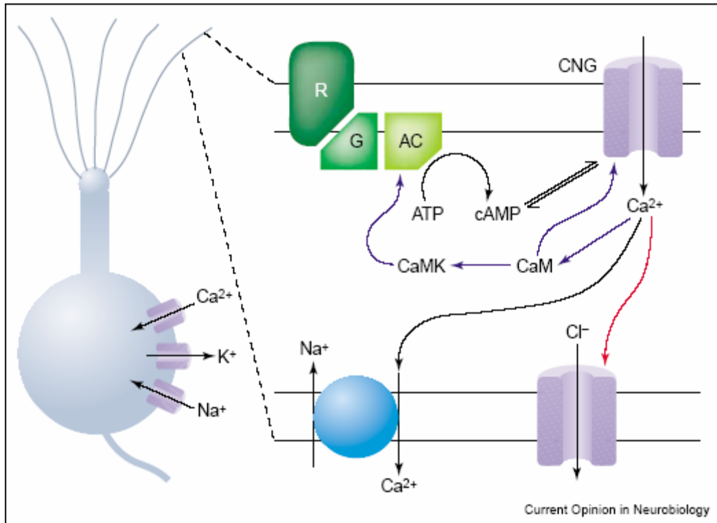
Figure 2.7 A schematic diagram that illustrates the olfactory transduction. 39 Blue and red arrows indicate the inhibitory and excitatory actions of \text{Ca}^{2+} respectively.
