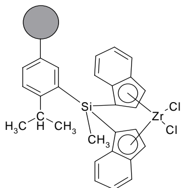
support 4
