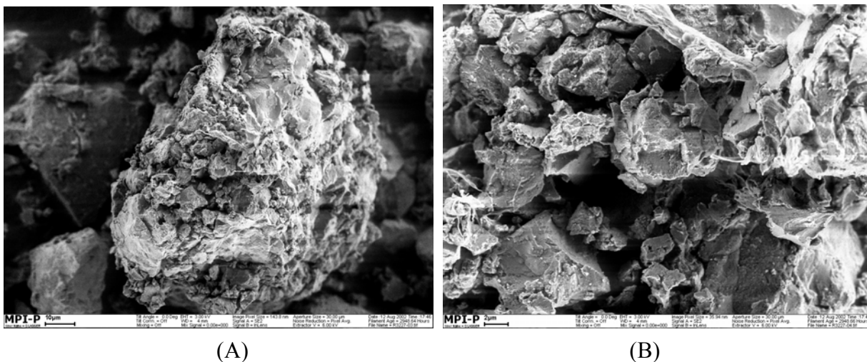
Figure 3-5. SEM images of the supported catalyst on the nanosized PS beads (NPS2-2) functionalized with PEO: scale bar – (A) 10 \mu\text{m} and (B) 2 \mu\text{m}
