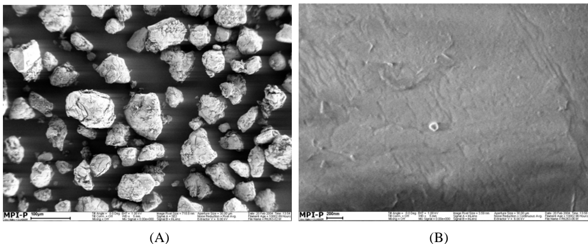
Figure 4-8. SEM images of the catalyst supported on the dendrimer (DEN 2): scale bar – (A) 100 \mu\text{m} and (B) 200 nm
