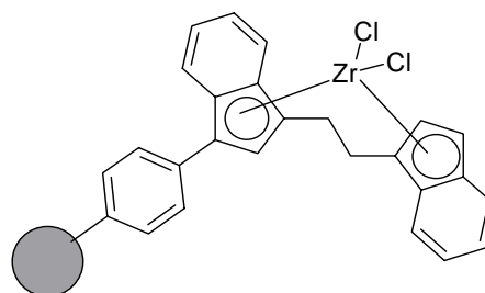
support 5
