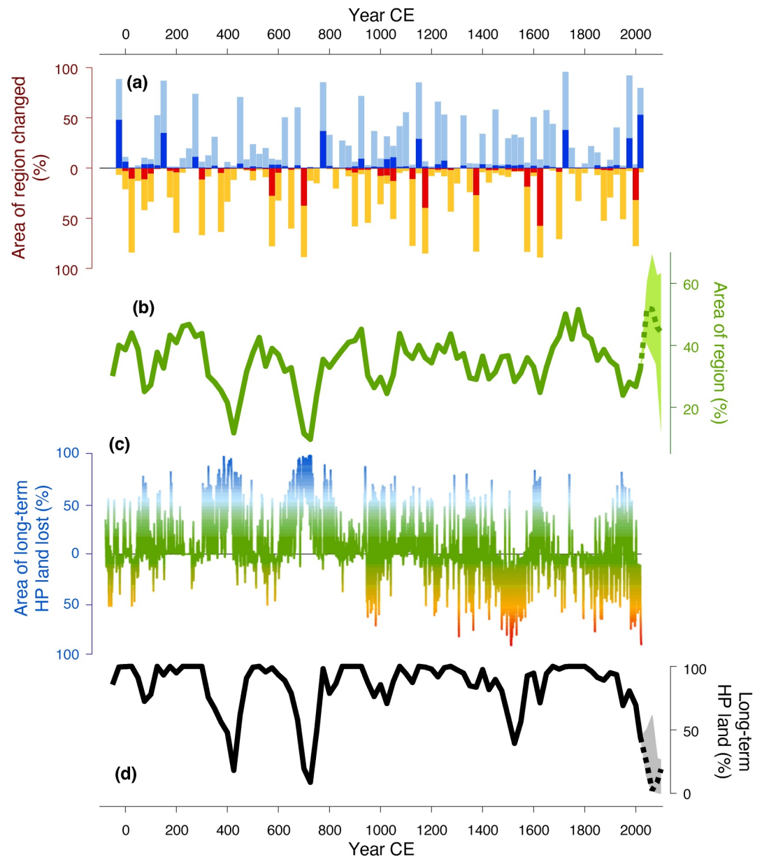
Figure 3. Changes over time in area agroclimatic zone. (a) Percentage of the study region for which the 25-year mode changed by one (light colors) and two (dark colors) zones compared to the previous 25-year period, and the direction of change (yellow/red toward drier and warmer zones; blue toward cooler). (b) Percentage of the study region that is classified as highly productive-humid (HPh) or dry (HPd). Light green spread indicates the range of changes for the six CMIP6 models considering SSP2-4.5, with the dotted line representing the mean of projected change. (c) Annual changes to the area of long-term HP land, with direction of change. (d) Percentage of long-term HP land that is classified as such for the 25-year periods over the full study period (75 BCE to 2099 CE). Gray spread indicates the range of the models, dotted line the mean.
