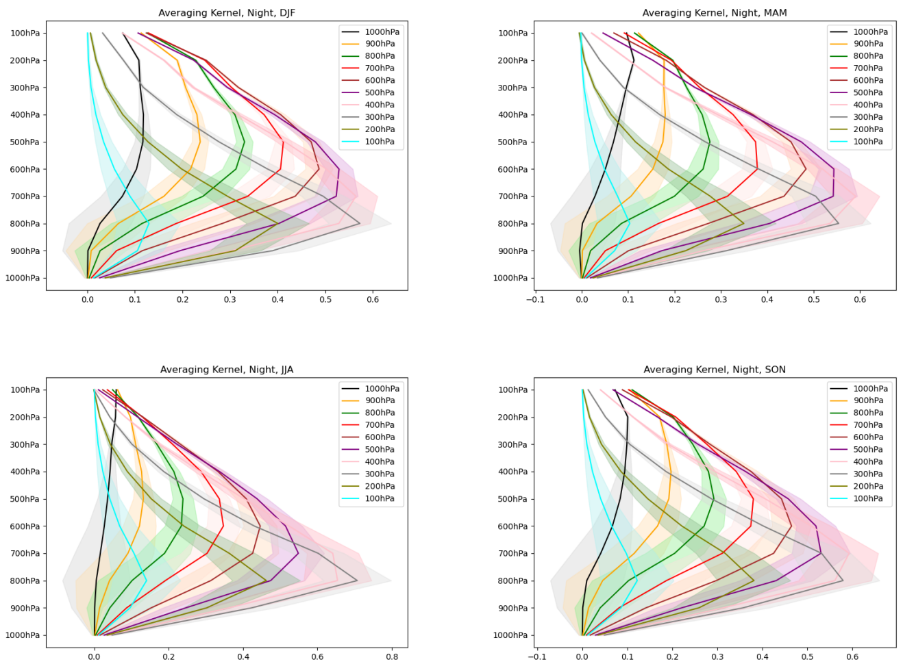
Figure 2: Nighttime averaging Kernels average over the study region (see Fig. 3 in the manuscript) and averaged over the study period (2000-2019). Shaded areas show the standard deviation for each vertical layer.
