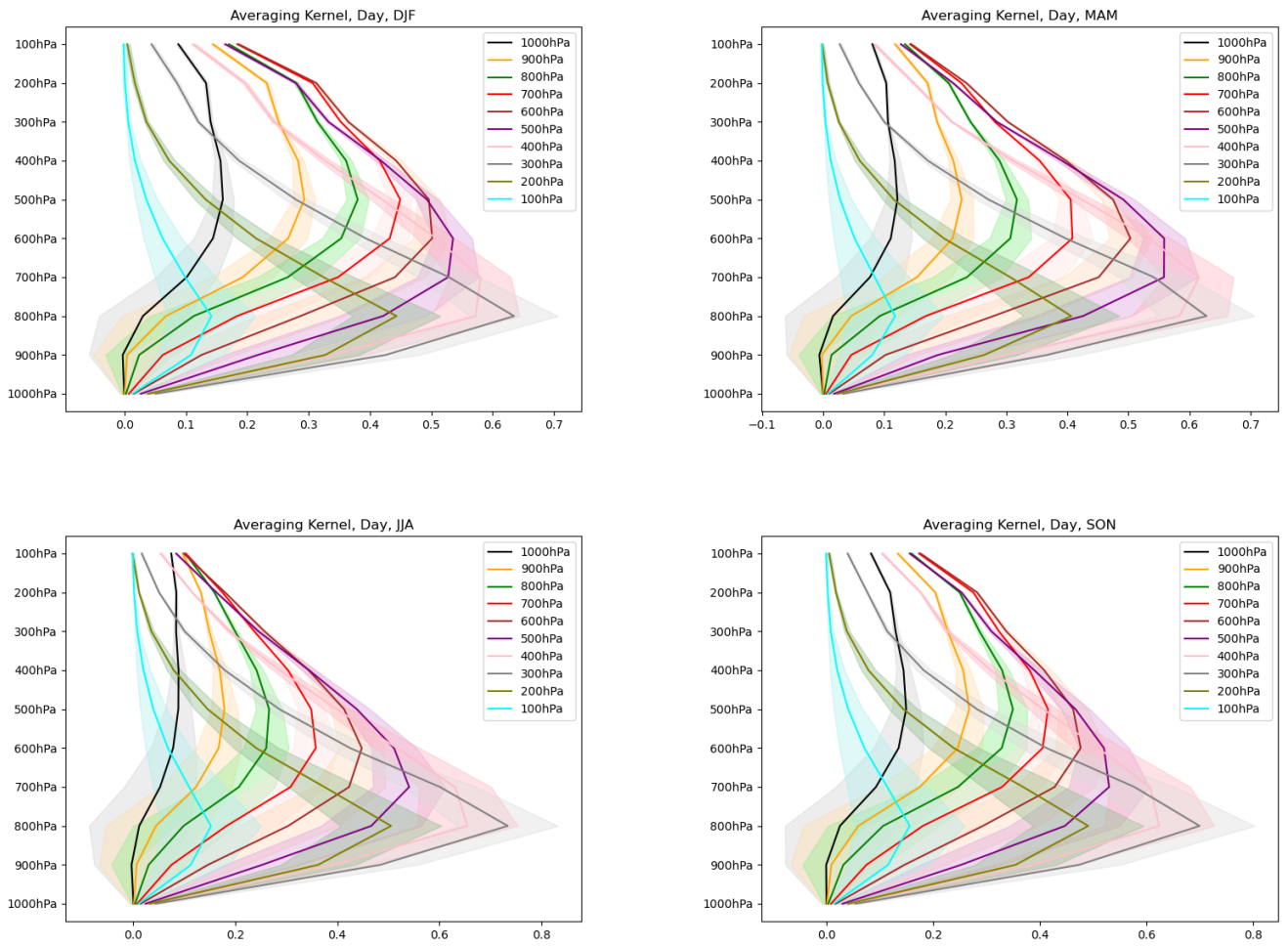
Figure 1: Daytime averaging Kernels average over the study region (see Fig. 3 in the manuscript) and averaged over the study period (2000-2019). Shaded areas show the standard deviation for each vertical layer.
