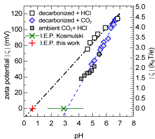
Fig. 6 Estimating the I.E.P. of fused silica surfaces. Magnitudes of \zeta -potentials in dependence on suspension \text{pH} for three different cases indicated in the key. The dashed line is an extrapolation towards vanishing \zeta -potential corresponding to the isoelectric point yielding \text{pH}_{\text{I.E.P.}} \approx 3.1 \pm 0.1 . Green Symbols are data as reviewed by Kosmulski. 86 The green cross denotes the median of a sub-sample as collected by Parks, 85 while the green bar denotes the spread of literature values for silica not included therein. The open symbols denote the potentials upon addition of acid to a system in the strictly \text{CO}_2 -free state. The dash-dotted line is a linear extrapolation towards the I.E.P. under decarbonized conditions (red cross) yielding \text{pH}_{\text{I.E.P.}} \approx 0.6 \pm 0.3 .
