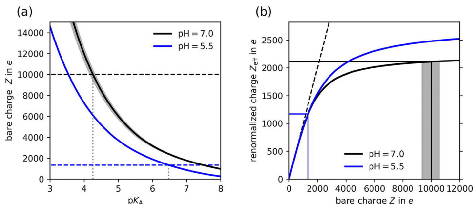
Fig. 5 Results from cell-model calculations. Comparison of data obtained using the Poisson–Boltzmann cell-model for the salt and \text{CO}_2 -free state at \text{pH}_{\text{bulk}} = 7 (black) and the \text{CO}_2 -equilibrated state at \text{pH}_{\text{bulk}} = 5.5 (blue). (a) Bare colloidal charges calculated for different surface group \text{pK}_\text{a} -values (solid lines). For \text{pH} = 7 the grey shaded regions indicate the variation of Z_{\text{bare}} due to its dependence on n . The variations are even less significant at \text{pH} = 5 , in fact so small that the shaded region is hidden by the line thickness. The experimentally observed bare charges are shown as dashed horizontal lines; crossing points with the curves obtained from the PBC allow to estimate effective surface \text{pK}_\text{a} -values of 4.26 and 6.5, respectively. (b) Renormalized charge as a function of the corresponding bare charge. The hypothetical case without charge renormalization ( Z_{\text{PBC}} = Z ) is shown as a black dashed line.
