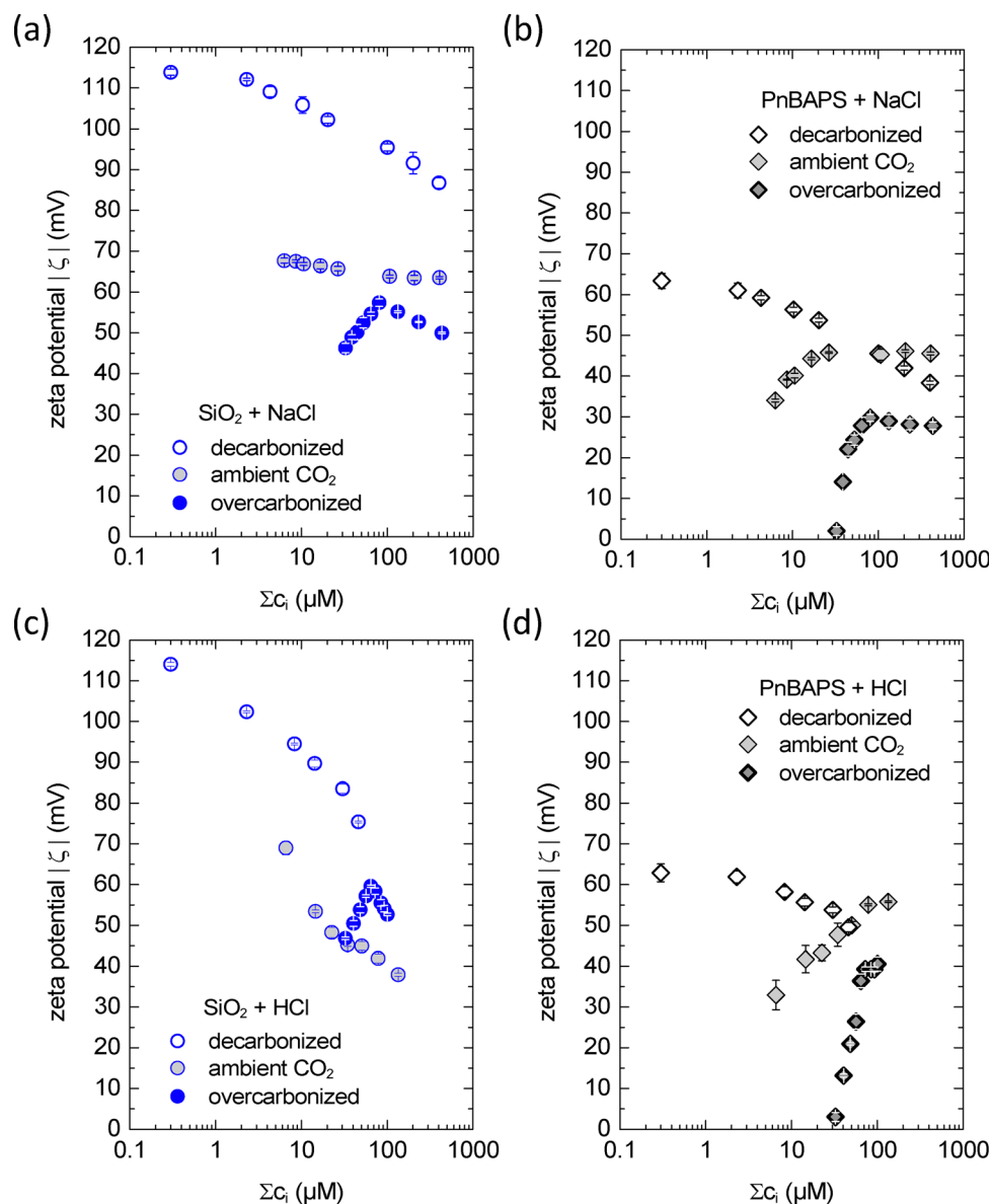
Fig. 7 Interplay of decharging and recharging processes in dependence on CO 2 content. Semi-logarithmic plots of the magnitudes of \zeta -potentials in dependence on total micro-ion concentration for SiO 2 (blue) and PnBAPS (black). The error bars correspond to the standard error at a confidence level of 0.95 of the fits to the Doppler-spectra. (a) Data taken for the silica surface upon the addition of NaCl starting from different state as indicated in the key. (b) The same, but for PnBAPS. (c) Data taken upon addition of HCl starting from different state as indicated in the key. (d) The same, but for PnBAPS. Data were recomputed from ref. 82 and 83.
