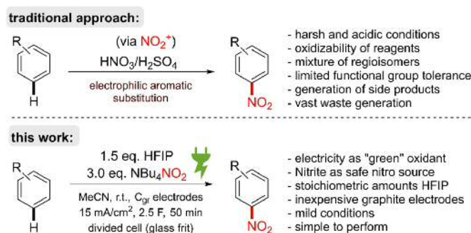
Scheme 2. Traditional approach (electrophilic aromatic substitution) in comparison to the electrochemical nitration with nitrite (this work); \text{C}_{gr} = graphite.
