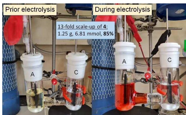
Figure 1. 13-Fold scale-up reaction of 4 in an H-type divided cell with a glass frit; left: cell setup prior electrolysis; right: cell setup during electrolysis (after passing ca. 1 F); A = anodic compartment; C = cathodic compartment.
