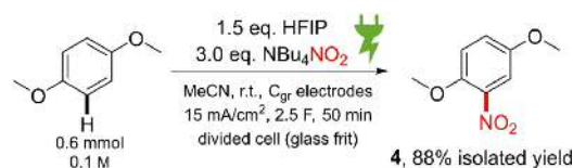
Scheme 3. Test reaction of 1,4-dimethoxybenzene with optimized reaction conditions (compare Table 1, entry 9).
