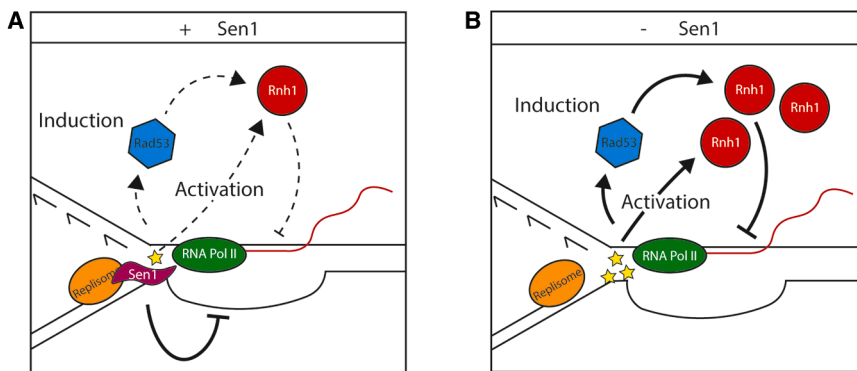
Figure 6. Interplay of Sen1 and Rnh1 during TRCs
