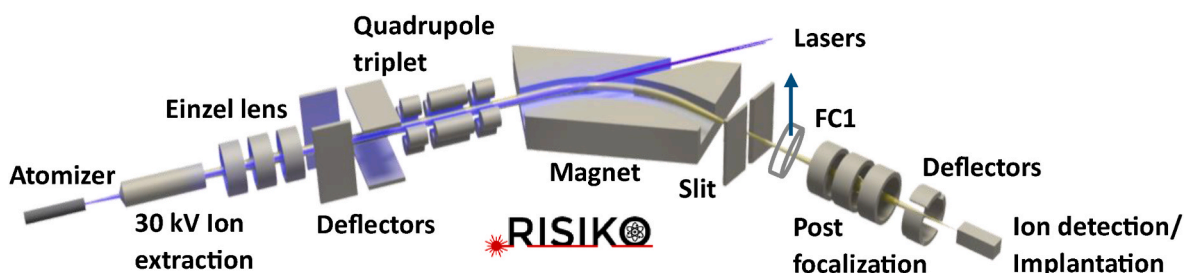
Fig. 1. Schematics of the RISIKO mass separator. Faraday-cup 1 (FC1) can be retracted during implantation. For a detailed description see text.
