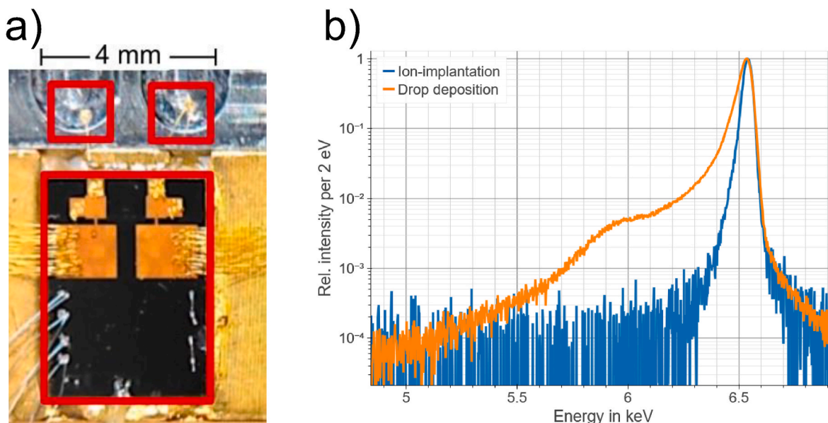
Fig. 10. Left) Photo of implanted absorbers (top red squares) thermally coupled by bond wires to the MMC chip (bottom red square). Right) Decay energy spectrum of the EC of ^{55}\text{Fe} . The spectra are normalized to the maximum intensity of the K binding energy of Manganese. The spectrum plotted in orange corresponds to a drop-deposited source while the blue one corresponds to an ion-implanted source. In both cases no background is subtracted. (For interpretation of the references to colour in this figure legend, the reader is referred to the Web version of this article.)
