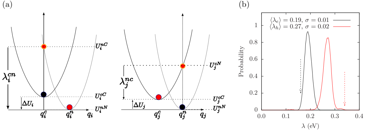
Figure 2.10. (a) Intramolecular reorganization energy: Potential energy surfaces of donor(left) and acceptor(right) in charged and neutral states. After the change of the charge state (black to orange circle) both molecules relax their nuclear coordinates (orange to red). If all vibrational modes are treated classically, the total internal reorganization energy and the internal energy difference of the charge transfer reaction are \lambda_{ij}^{\text{int}} = \lambda_i^{\text{cn}} + \lambda_j^{\text{nc}} and \Delta E_{ij}^{\text{int}} = \Delta U_i - \Delta U_j , respectively. (b) Histogram of intramolecular reorganization energy \lambda_{ij} for electrons and holes from an amorphous phase of 512 BTDF molecules taking into account different conformations that arise in the bulk. If the molecules could fully relax \lambda_{e(h)}^{\text{free}} = 0.16(0.34) eV as indicated by the arrows which deviates from the mean of the distribution in the bulk.
