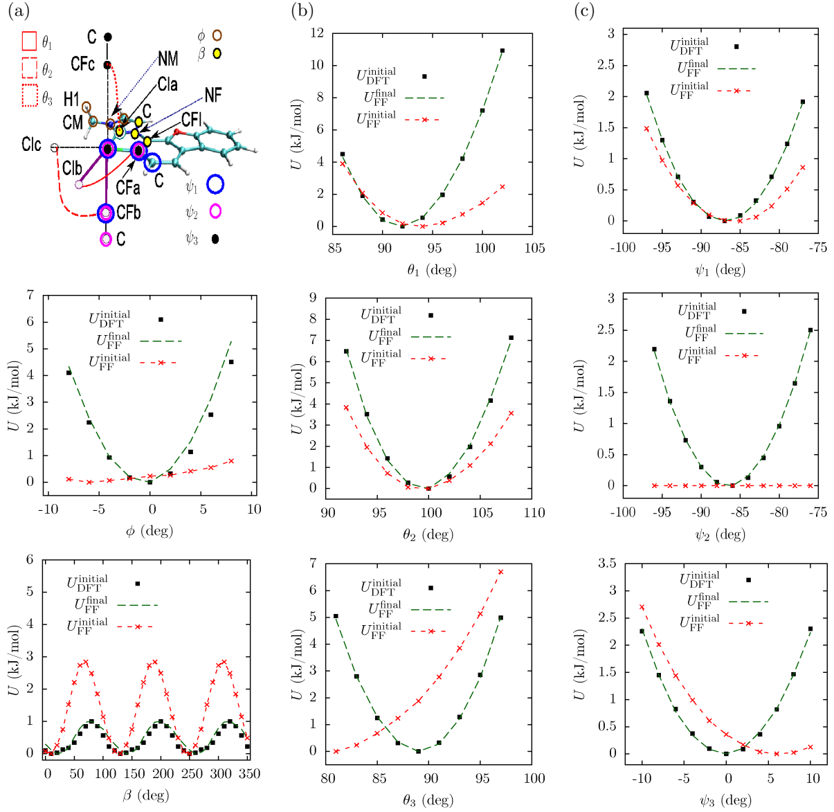
Figure 3.7. Force-field scans for the unknown degrees of freedom in the emitter. First-principles scans, U_{\text{DFT}} , and final and initial force field scans, U_{\text{FF}} , are shown. Column (a) Shows labeling with atoms Cl(a,b,c) connected to the imidazole unit of ligands a,b,c and CF(a,b,c) connected to dibenzofuran unit. Below is the scan for the improper dihedral \phi keeping the imidazole and dibenzofuran units of one ligand in the same plane. Below that is the scan for the rotational angle of the methyl group \beta . Column (b) shows scans for angles \theta between the three ligands. Column (c) shows scans for rotations of the ligands with respect to each other defined by the proper dihedral \psi . Resulting force-field parameters are given in tab. 3.4.
