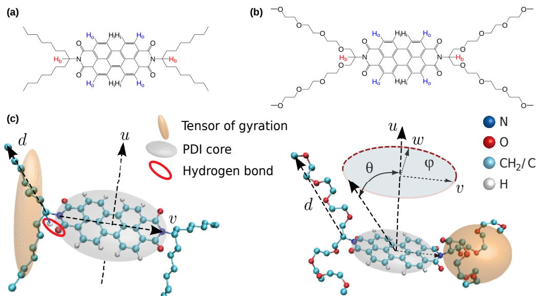
Figure 4.1. Chemical structure of (a) C 8,7 -PDI with the alkyl side chain and (b) TEG-PDI with the tri-ethylene-glycol (TEG) side chain. (c) Sketch of the two PDI derivatives: side chains are displayed using united atom representation except for the branching C-atom. The orientation of the conjugated core defines the coordinate systems given by vectors \mathbf{v} (connects the two N-atoms in the molecular plane), \mathbf{u} (normal to the molecular plane), and \mathbf{w} = \mathbf{u} \times \mathbf{v} . Angles \theta and \phi are polar and azimuthal angles of the end-to-end vector \mathbf{d} in this coordinate system. Ellipsoids depict tensors of gyration for each pair of side chains. Labels for different H atoms (left) are used for dynamical order parameters in Table 4.1.
