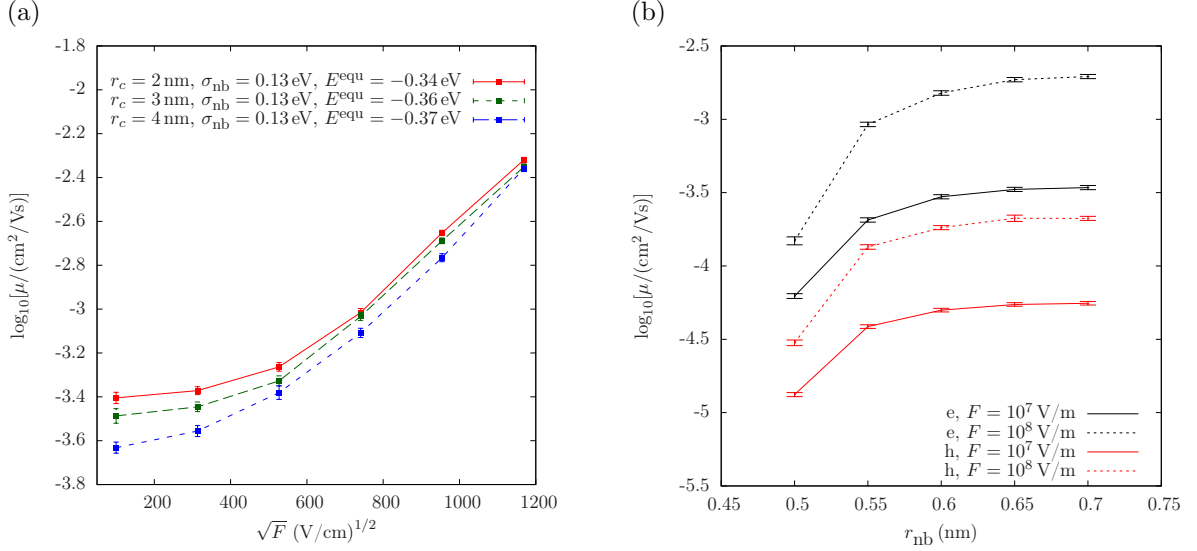
Figure 2.15. Convergence of mobility in system of 4096 BTDF molecules. (a) Poole-Frenkel plots for electron transport for different r_{\text{el}} used for polarized site-energy calculations show that although site-energy differences ( \sigma_{\text{nb}} ) are converged at r_{\text{el}} = 2 \text{ nm} , unconverged transport energy E^{\text{equ}} leads to slight overestimation of mobility for small electric fields. (b) A neighborlist cutoff of r_{\text{nb}} = 0.7 \text{ nm} between centers of mass of rigid fragments yielding 30.000 pairs is sufficient to converge mobilities. All mobilities in a and b are averaged over ten KMC runs with different injection points and six directions of the field. In case of b, averages are obtained from two independent MD snapshots while only one snapshot is used for a. Errors for the mean of the mobility are taken from a bootstrap analysis with 10.000 data sets. Conformational disorder has been neglected in a and b.
