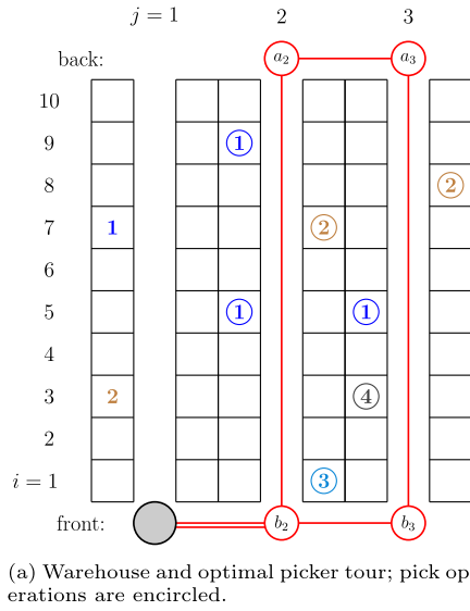
Fig. 2. An instance of the SPRP-SS. The pick list contains four articles S = \{1, 2, 3, 4\} with unit supply and demands q_1 = 3, q_2 = 2 , and q_3 = q_4 = 1 .
