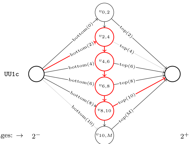
(b) Subnetwork EG for aisle j = 2 and the state of type UU1c. The highlighted path (red/bold) corresponds to gap(2,10) in Figure 3a. Gray edges can be omitted from the subnetwork by dominance considerations.
