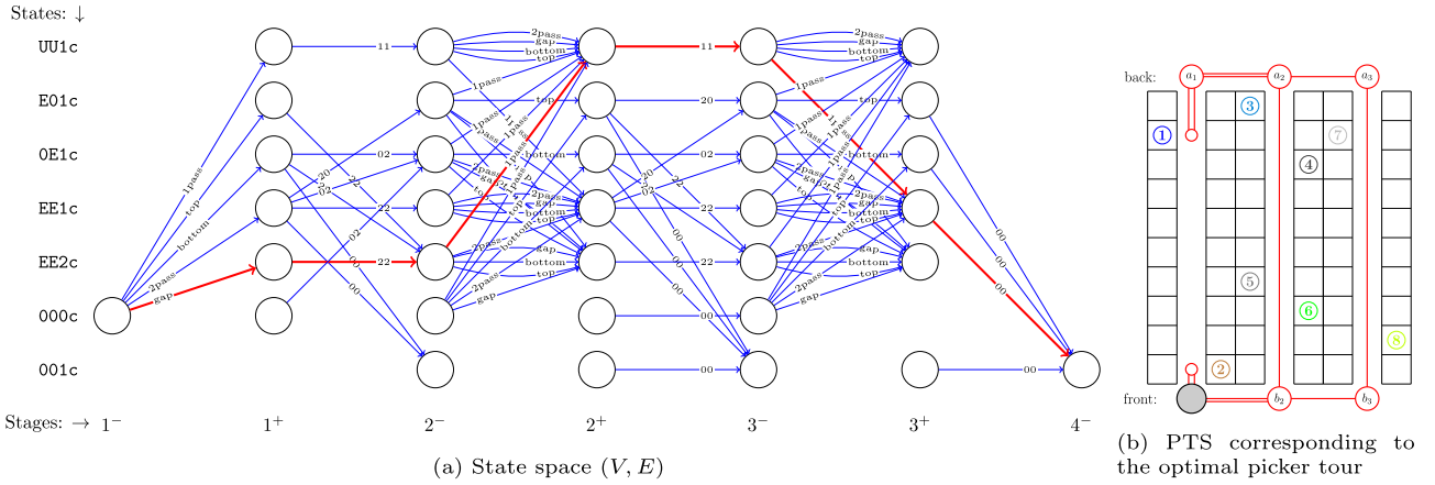
Fig. 1. State space and PTS for a warehouse with aisles J = \{1, 2, 3\} and articles S = \{1, 2, \dots, 8\} (unit demand). The highlighted path (red/bold) in the state space represents the optimal picker tour. (For interpretation of the references to colour in this figure legend, the reader is referred to the web version of this article.)
