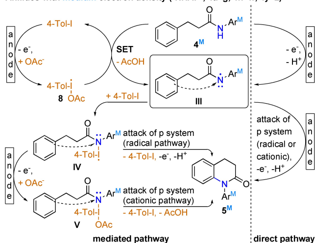
Scheme 4. Grouping of the substrates according to their oxidation potential (top) and proposed mechanisms for each group (center, bottom). SET = single electron transfer.
