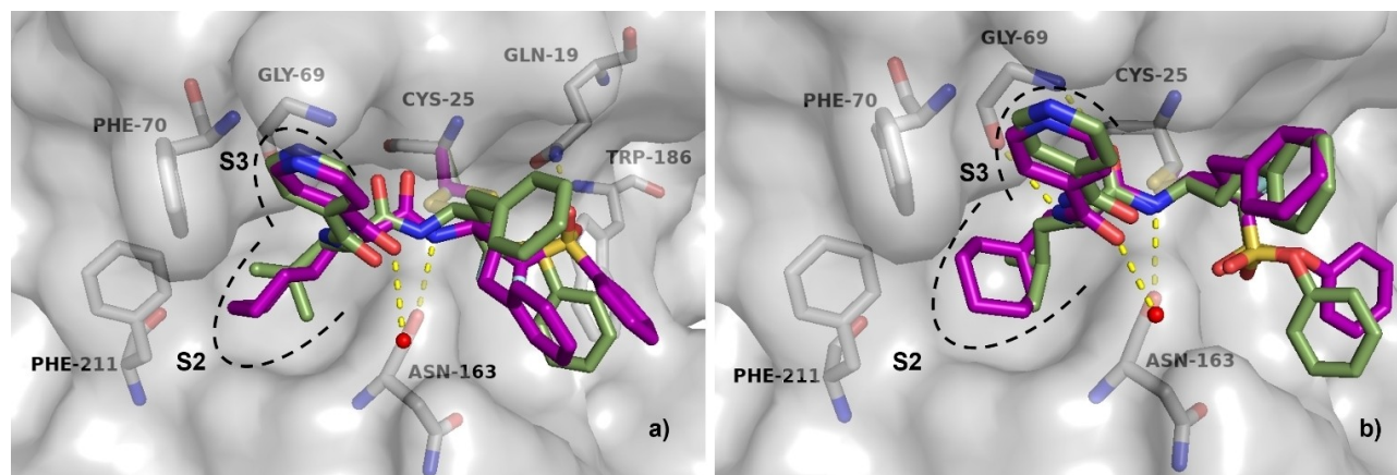
Figure 8. Predicted binding modes and non-covalent interactions (yellow dashed lines) of different inhibitors inside the CatS binding pocket (pdb: 1NPZ). (A) Superposition of the covalent docking poses of 4a (purple carbon-atoms) & 4b (smudge green carbon atoms). (B) Superposition of the covalent docking poses of 5a (purple carbon-atoms) & 5b (smudge green carbon atoms).
