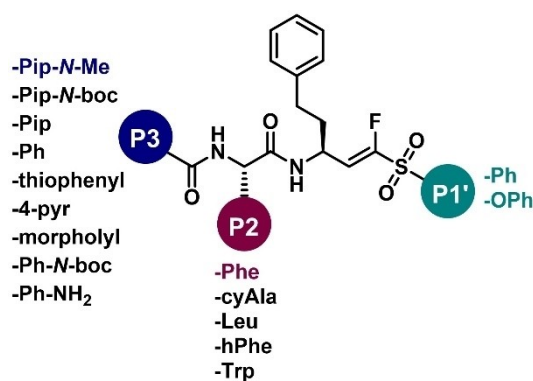
Figure 3. SAR variations for compounds 1a ( P1' = \text{Ph} ) and 1b ( P1' = \text{OPh} ). Residues of initial leads are highlighted.
