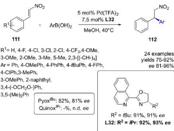
Scheme 53. Asymmetric synthesis of \beta,\beta -diaryl substituted nitroalkanes 112 through Pd(II)-catalyzed reactions.
