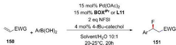
Scheme 74. 1,1-Difunctionalization of activated alkenes 150 by using Pd(II)-catalyst and BOX or Pyox ligand in function of the substrate.
