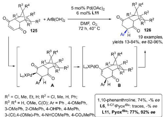
Scheme 60. Pd-catalyzed addition to polycyclic cyclohexenediones 125 , affording up to five stereocenters in 126 .
