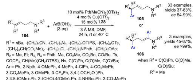
Scheme 50. Divergent reactivity of amides 104 in function of the –R 3 and –R 4 substituents, yielding allylic 105 or diarylated ene-products 106 .
