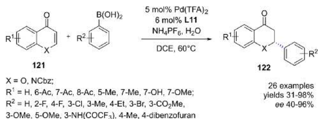
Scheme 58. Asymmetric conjugate addition to chromones and 4-quinolones 121 .
