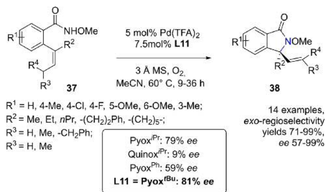
Scheme 18. Asymmetric aza-Wacker type intramolecular cyclization of N -methoxy-2-vinylbenzamides 37 .
