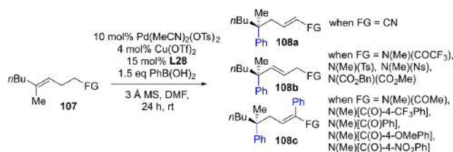
Scheme 51. Summary of the different outcomes investigated in function of the FG located at (–CH 2 –) distance from the olefin.
