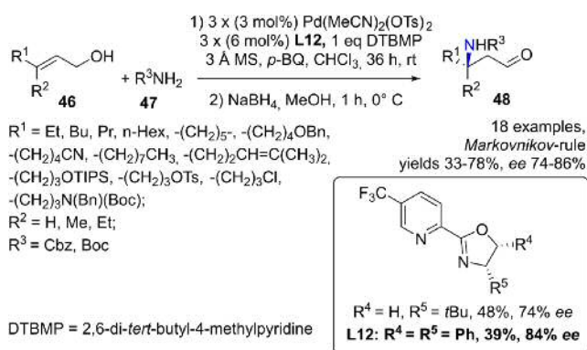
Scheme 22. Asymmetric redox-relay strategy for the synthesis of \beta -amino aldehydes 48 .
