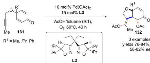
Scheme 64. Intramolecular asymmetric cyclization of alkynyl cyclohexadienones 131 in the presence of L3 and subsequent enantioselective acetylation.
