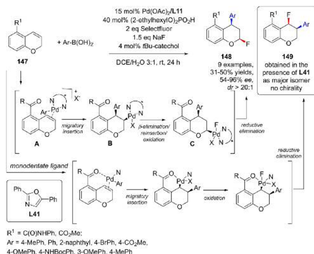
Scheme 73. Ligand effect on the regioselective carbonylation of chromenes 147 .
