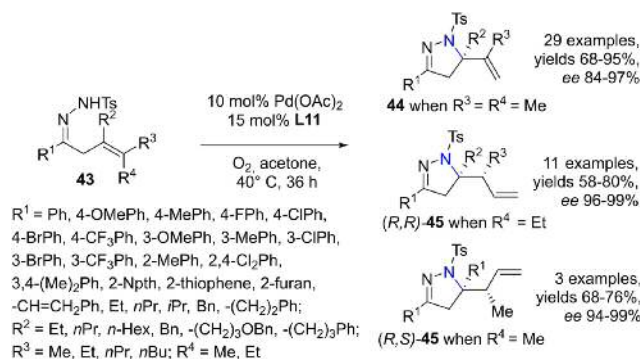
Scheme 21. Formation of two vicinal stereocenters by means of Pd(II)-catalyzed reactions on N -Ts hydrazine-tethered tetrasubstituted olefins 43 .
