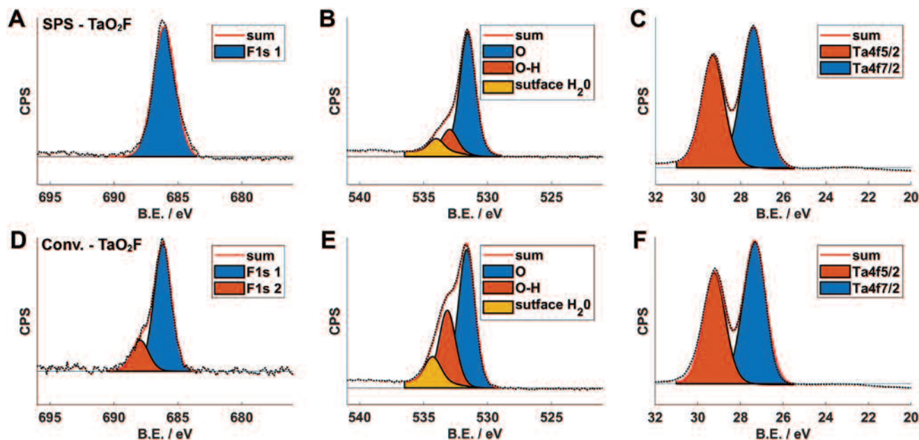
Figure 5. Electronic and surface structure of \text{Ta}_3\text{O}_7\text{F} and \text{TaO}_2\text{F} prepared by SPS and conventional solid-state chemistry. A–F) XPS spectra (with F, O, and Ta subspectra in (A,D), (B,E), and (C,F)) of \text{TaO}_2\text{F} , prepared by SPS (A–C) and conventional ampoule chemistry (D–F) with fitted signals for the respective environments.
