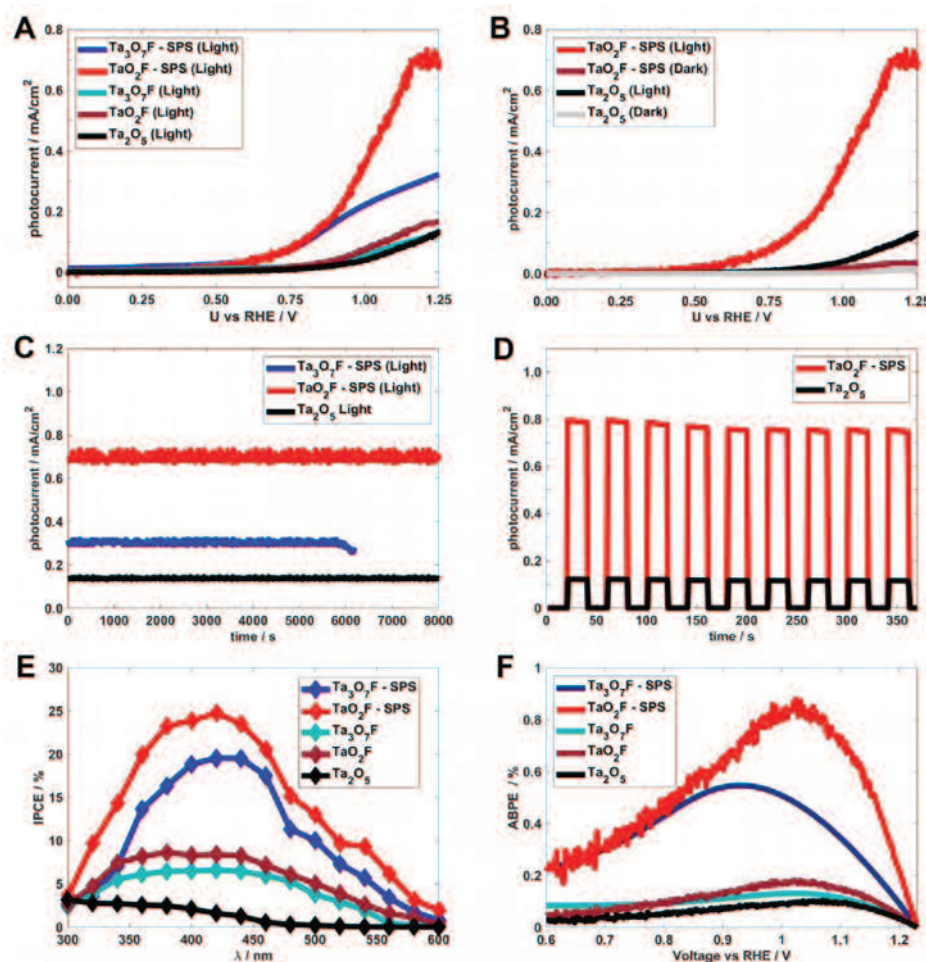
Figure 7. PEC measurements for Ta 2 O 5 and the tantalum oxyfluorides, prepared by SPS and conventional ampoules chemistry. A,B) Linear sweep voltammograms under light and dark conditions, C) I – t photostability curve under continuous luminescence at 1.23 V versus RHE, and D) amperometric I – t curves at an applied potential of 1.23 V versus RHE with 20 s ON/OFF cycle. E) Incident photon-to-current efficiencies, IPCE (%) and F) applied bias to photoconversion ABPE (%) for Ta 2 O 5 , Ta 3 O 7 F (SPS-prepared and conventional synthesis) and TaO 2 F (SPS-prepared and conventional synthesis).
