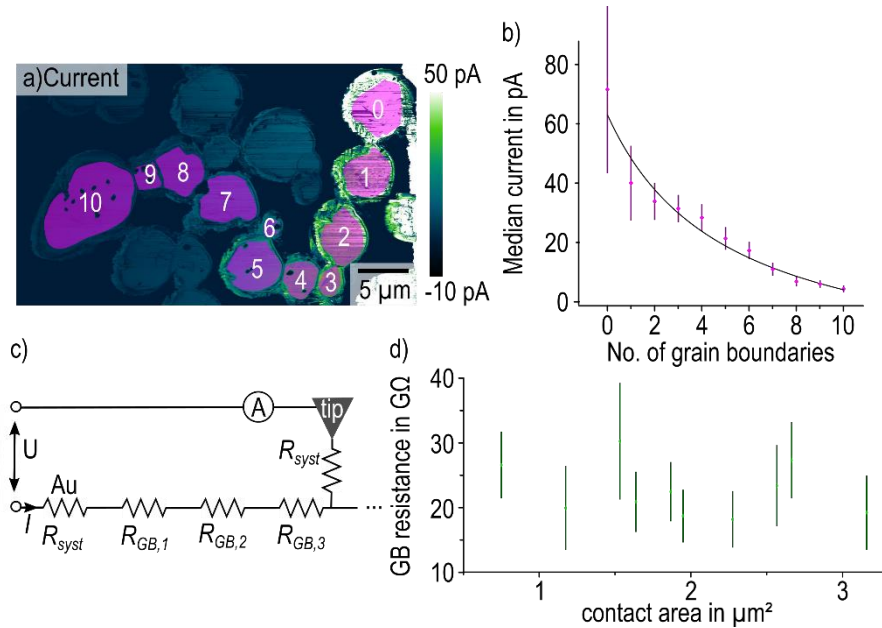
Figure 4.4: a) Enlarged image detail of an interconnected MAPbI 3 grain cluster extracted from current image in Figure 4.2b. Pink shaded areas represent the areas used to determine the average current of each grain excluding nonconductive dirt particles and grain edges. Numbers visualize the amount of grain boundaries the charge carriers have to pass from the electrode to the respective grain, starting with 0 for the grain in direct contact with the electrode. b) The median current I versus the amount of grain boundaries n with the standard deviation as error bars. The current decay was fitted via Equation 4.1. c) Schematic of electric circuit model used for Equation 4.1. d) Grain boundary resistance R_{GB} , calculated via Equation 4.2, vs. contact area, determined via topography cross sections across each grain boundary.
