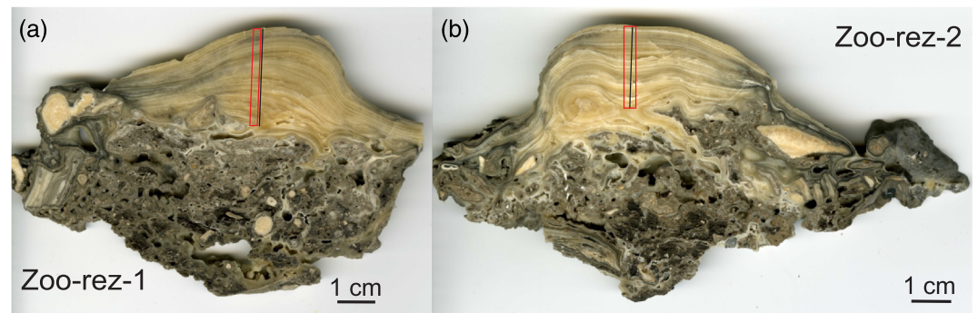
Figure 2. Pictures of the sampled slices of (a) Zoo-rez-1 and (b) Zoo-rez-2. The laser ablation tracks are indicated by black lines, and the milling tracks for the carbon and oxygen isotope samples are indicated by the red rectangles. The sampling tracks in Zoo-rez-1 are a little to the left from the growth axis (5 mm), due to the milling of the ^{14}\text{C} samples for the bomb peak detection (see Fig. 2a in Riechelmann et al., 2019). However, Zoo-rez-1 has an asymmetric growth, which gives the impression that the growth axis is located much more to the right. Zoo-rez-1 and -2 were sampled as a block from the cave. The two slices were cut from this block and by visual inspection of the cut slices and the other pieces of the block, we could identify the growth axes of the two stalagmites. The asymmetric growth of Zoo-rez-1 is probably due to the uneven basement.
