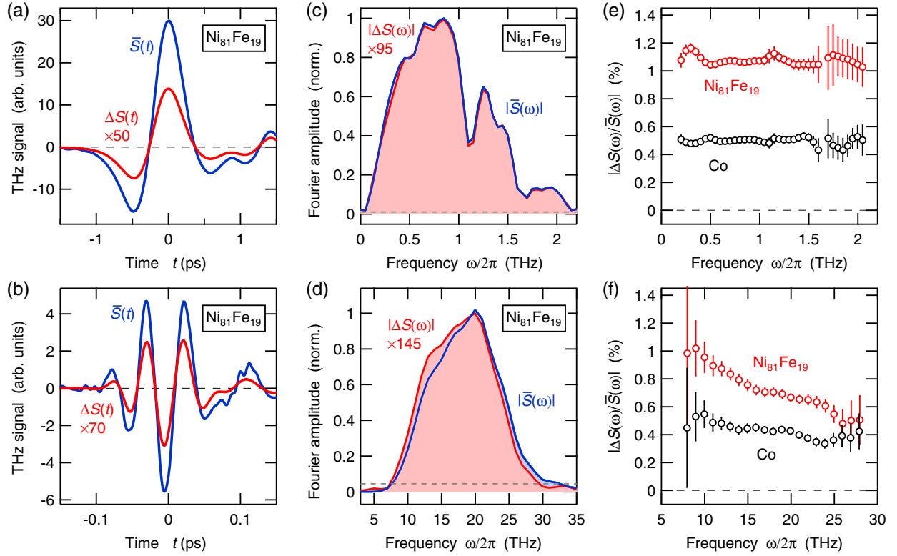
FIG. 2. THz AMR probes of \text{Ni}_{81}\text{Fe}_{19} and Co. (a) THz signal waveforms \Delta S(t) = S(t, 0^\circ) - S(t, 90^\circ) (red line) and \bar{S}(t) = [S(t, 0^\circ) + S(t, 90^\circ)]/2 (blue line) of a THz pulse from a source-detector combination with a bandwidth 0.2–2 THz after having traversed the \text{Ni}_{81}\text{Fe}_{19} thin film. The difference waveform \Delta S(t) reports on the change in the sample transmission when the magnetization is rotated from \alpha = 90^\circ to 0^\circ [see Fig. 1(b)]. It is a signature of the AMR. (b) Same as panel (a), but for measurements with bandwidth 8–28 THz. (c,d) Fourier amplitude spectra |\Delta S(\omega)| and |\bar{S}(\omega)| of the traces of panels (a) and (b), respectively. Signals are normalized to their respective maximum. The mean noise level of |\Delta S(\omega)| is indicated by the grey dashed lines and amounts to 0.01 and 0.04, respectively. (e,f) Relative spectral amplitude changes |\Delta S(\omega)/\bar{S}(\omega)| as derived from panels (c) and (d), respectively (red circles). Results for Co are also shown (black circles). Note that |\Delta S(\omega)/\bar{S}(\omega)| is closely related to the AMR contrast through Eq. (6). The error bars indicate the precision of the measurements as estimated from the noise level in panels (c) and (d). Data in all panels are scaled by the indicated factors for clarity.
