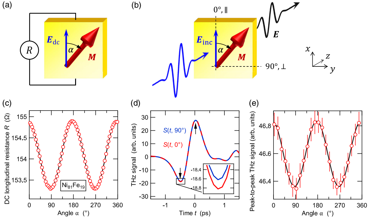
FIG. 1. Measuring dc and THz AMR. (a) Schematic of a dc electrical AMR measurement. The resistance R of a magnetic thin film with magnetization \mathbf{M} (red arrow) is measured along the applied dc electric field \mathbf{E}_{dc} (blue arrow) for different rotation angles \alpha of \mathbf{M} . (b) Schematic of the THz AMR measurement. An x -polarized THz pulse with transient electric field \mathbf{E}_{inc}(t) (blue arrow) is incident on the magnetic thin film. After traversal of the sample, we detect the x component of the THz electric field \mathbf{E} , that is, \mathbf{E} projected onto the fixed direction of \mathbf{E}_{inc} , as a function of the magnetization angle \alpha . (c) dc longitudinal resistance of \text{Ni}_{81}\text{Fe}_{19} vs \alpha (red open circles) with a fit by R_{\perp} + \Delta R \cos^2 \alpha (black solid line). (d) THz waveforms S(t, \alpha) for \alpha = 90^\circ (blue solid line) and 0^\circ (red dashed line) vs time t for the emitter-detector configuration covering the frequency range 0.2–2 THz. The inset shows a magnified version of the signal around its minimum, indicating a signal change of about 1%. (e) Peak-to-peak amplitude of the THz signal waveform S(t, \alpha) as a function of \alpha (open circles) with a fit as in panel (c). The signal extrema used for the evaluation are indicated by the black arrows in panel (d).
