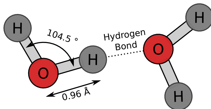
Figure 1.1: Model of two hydrogen-bonded water molecules.
