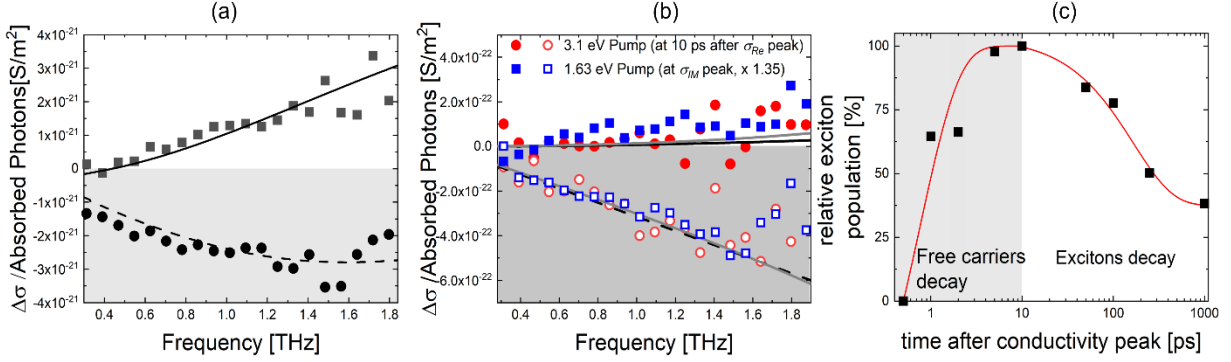
Figure 4: (a) The complex frequency-dependent conductivity measured at 0.5 ps, at the peak of the photoconductivity by 3.1 eV pump. The conductivity is scaled to the density N of absorbed photons; the solid line represent the Drude-Smith fitting described in the SI; (b) The complex frequency-dependent conductivity comparison between the one measured at 10 ps after photoexcitation with 3.1 eV pump (read), and that at the peak of the imaginary conductivity with 1.63 eV pump (blue, rescale with a factor of 1.35 for comparison). The data are fitted by Lorentzian model described in the main text. Two fitting examples are given here with the center frequency for the black one 25 THz, and the grey one 6 THz. (c) Tracking of exciton formation and recombination dynamics in GNRs, inferred from the fitting described in the main text. The red solid line is a fitting combined an exponential ingrowth and a followed decay, from which the exciton formation and decay time are obtained.
