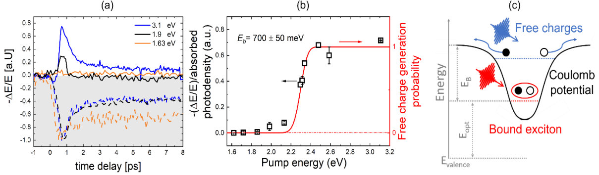
Figure 2: (a) The sub-picosecond time evolution of both the real and imaginary frequency-integrated photoconductivity as a function of the pump-probe delay and the pump wavelength. The used fluences were 200 \mu\text{J}/\text{cm}^2 , 246 \mu\text{J}/\text{cm}^2 and 227 \mu\text{J}/\text{cm}^2 for 1.63, 1.9 and 3.1 eV respectively; (b) The maximum of the real part of the one-dimensional conductivity normalized to the absorbed photon density. The red line is a best fit to a model described in the main text to account for the free carrier generation probability with increasing the pump energy. The model and the corresponding fitting yield an excitonic binding energy of 700 \pm 50 \text{ meV} ; (c) Illustrates the model used here to simulate the probability of exciton dissociation from the deep Coulomb potential into free charges at the band edge by thermal excitation.
