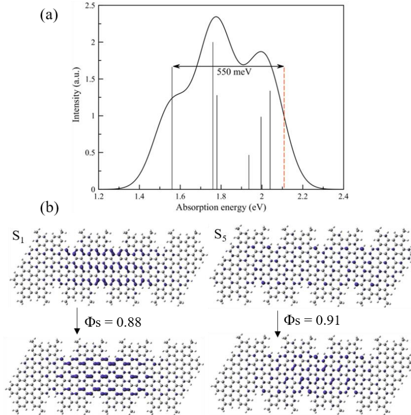
Figure 3. (a) Computed absorption spectrum for the GNR-AHM tetramer; black vertical bars represent the oscillator strength for the transitions, the red dashed line the band edge. The binding energy is indicated with a black arrow; (b) detachment/attachment density for the two excited states of interest, S1 and S5, together with their spatial overlap.
