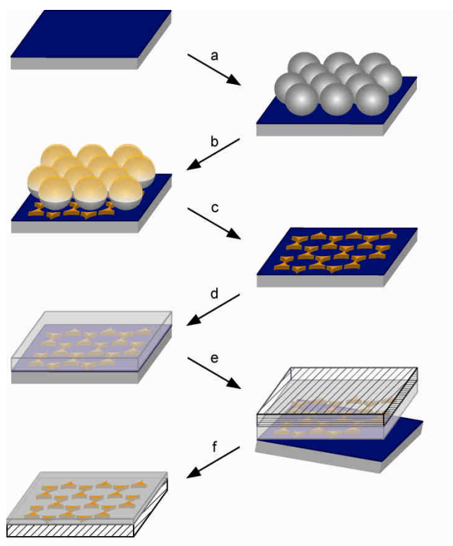
Figure 5.3.26 Flow process for the construction of embedded nanoparticles arrays: A hexamethyldisilazane-modified wafer is used as template material. a) Colloidal monolayer assembly. b) Thermal evaporation of gold (50 nm) and chromium (< 2 nm). c) Removal of the colloidal monolayer. d) Thermal evaporation of silicon dioxide (100 nm). e) Gluing of the interface to a glass slide and mechanical separation. e) Template-stripped surface with gold nanoparticles embedded in a silicon dioxide matrix.
