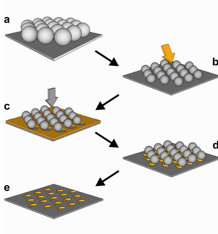
Figure 5.3.8. Fabrication of the nanostructure arrays: (a) monolayer formation, (b) size reduction and metal deposition, (c,d) ion etching, (e) mask removal.
