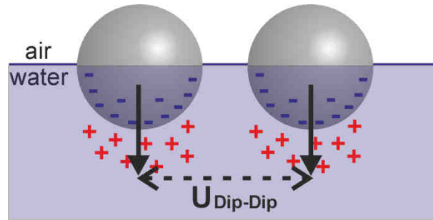
Figure 3.2.4. Two colloidal particles at the air/water interface. The asymmetry of the counter-ion clouds induces repulsive dipole moments normal to the interface.
