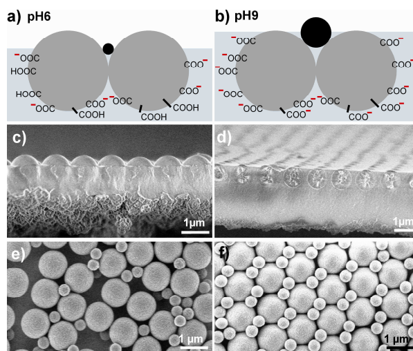
Figure 5.2.23. Effect of the \text{pH} value on the position of the monolayer at the interface and consequences for the crystallization of a binary system composed of 1063 \text{ nm} and 422 \text{ nm} colloids (size ratio RS = 0.40 ). a,b) Schematic illustration of one small- between two large colloids at the air/water interface at \text{pH} = 6 (a) and \text{pH} = 9 (b). The black sphere illustrates the maximum size of a small colloid that fit into the interstitial site at the interface without disturbing the crystal structure of the large sphere monolayer; c,d) SEM images of a monolayer embedded in a poly-(butyl cyanacrylate) matrix that was polymerized at the interface to visualize the colloid positions at \text{pH} 6 (c) and \text{pH} 9 (d); e,f) binary monolayers with a size ratio of 0.40 produced at \text{pH}6 (e) and \text{pH}9 (f).
