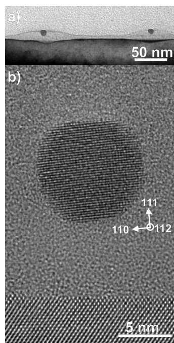
Figure 5.3.7. The top TEM image shows two FePt NPs embedded in a lens-shaped silicon oxide layer on a silicon substrate. Silicon oxide is growing faster under and around the particles compared to naked substrate due to the catalytic effect of Pt. The HRTEM image clearly demonstrates the crystalline structure of the FePt NPs. By analysis of in total 13 NPs an average lattice fringe spacing of (0.2225 \pm 0.0058) nm is determined as expected for (111) lattice planes of fcc FePt. Experiments performed and images provided by Ute Kaiser; University of Ulm.
