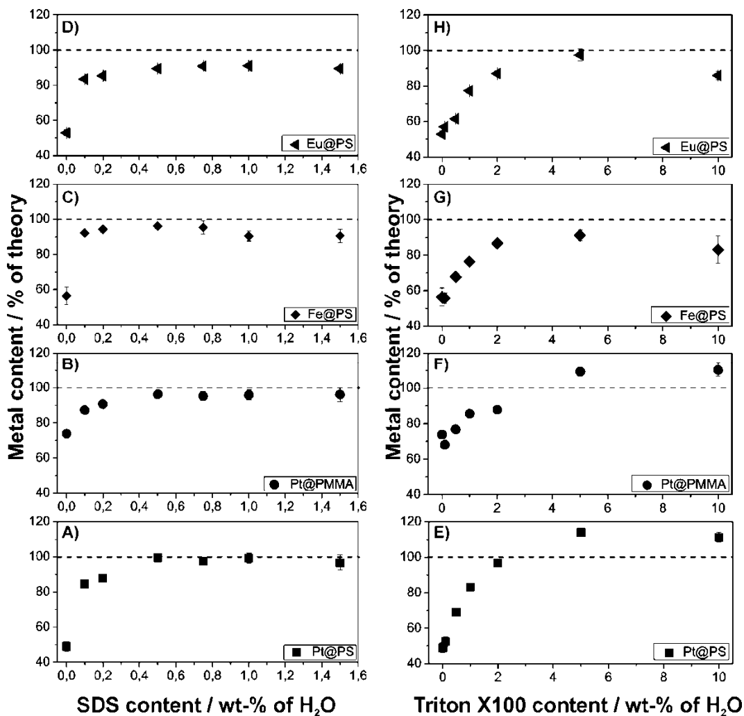
Figure 5.1.4. Effect of surfactant addition on metal content measured by ICP-OES. Left side (A-D): measured metal contents after addition of SDS to 0.1 wt.-% colloidal dispersions; right side (E-H): measured metal contents after addition of Triton X100 to 0.1 wt.-% colloidal dispersions. The dotted line represents the theoretical metal content.
