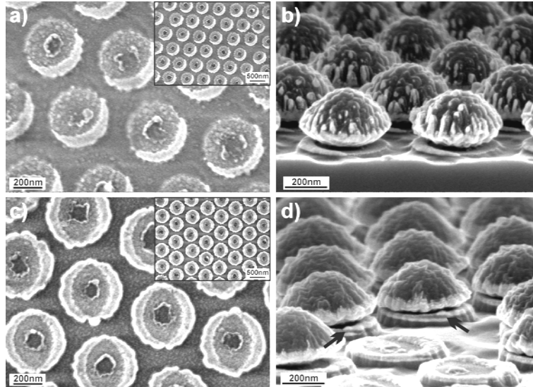
Figure 5.3.11. Scanning electron microscopy (SEM) images of the stacked nano-crescents arrays. Top row: single crescents arrays representing the first layer in the stacked crescent configuration. a) top view; b) side view. Bottom row: stacked crescents arrays. c) top view; d) side view. The black arrows highlight the separation layer between the two crescents. For a better illustration of the preparation method, the side-view images were taken on a sample where the colloidal monolayer used as mask was not removed.
