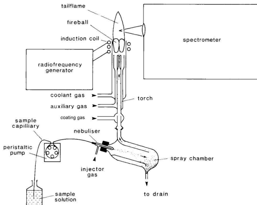
Figure 4.2.1. Schematic illustration of an inductively coupled plasma optical emission spectrometer.
