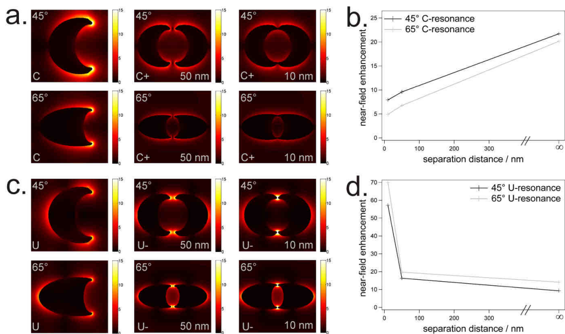
Figure 5.3.25. a) Simulations of the electrical near-fields in c-polarization of single crescents and opposing double crescents for 50 nm and 10 nm tip separation distance (upper row: 45° etching angle, lower row: 65° etching angle). b) Corresponding maximum near-field enhancements in c-polarization of double crescents versus the separation distance. c) Simulations of the electrical near-fields in u-polarization of single crescents and opposing double crescents 50 nm and 10 nm tip separation distance (upper row: 45° etching angle, lower row: 65° etching angle). d) Corresponding maximum near-field enhancements in u-polarization of double crescents versus the separation distance.
