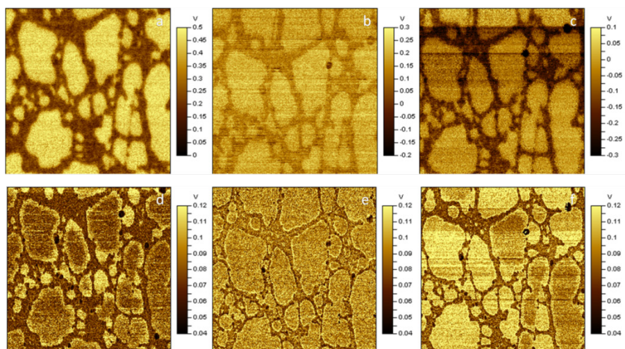
Figure A11. Surface potential (a, b, and c) and dielectric images (d, e, and f) of annealed thin PPy:PSS film at different RH: a) and d) the 1 st dry state, RH = 7%; b) and e) the 1 st swollen state, RH = 90%; c) the 2 nd dry state, RH = 5%.
