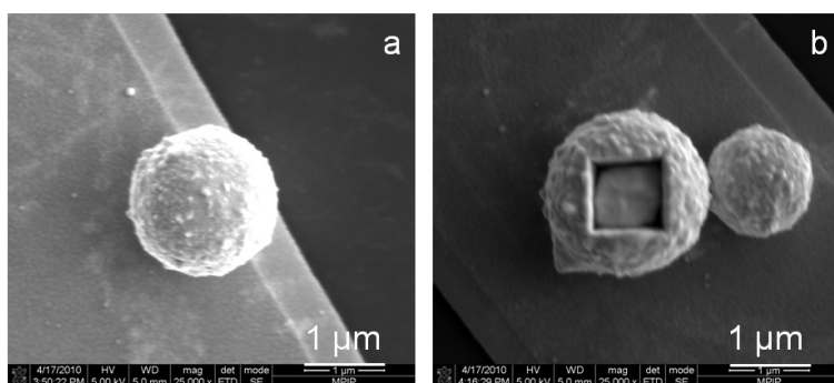
Figure 2.3. SEM images of Au bulk particles before (a) and after (b) FIB etching.
