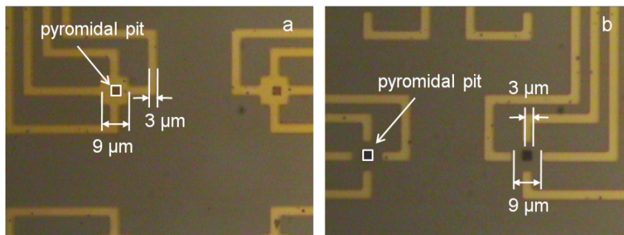
Figure 2.5. Optical microscopy images of two geometries of the electrode array: a) bottom contact; b) top contact. The magnification is 50 x.
