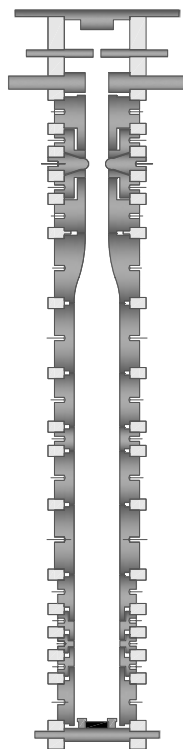
Figure 4. Sketch of the double trap for (anti)proton g factor determination.
