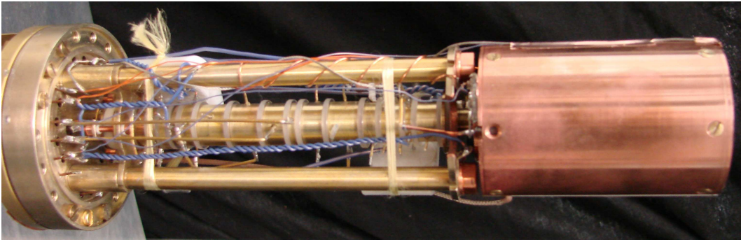
Figure 4.12: Completely assembled trap tower with the cyclotron resonator on the right.
