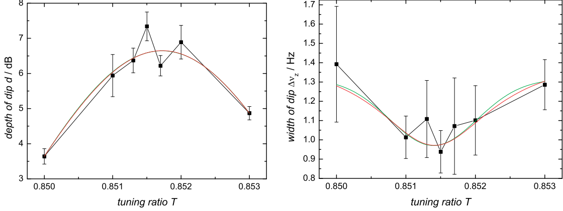
Figure 6.2: The two parameters depth d and the width \Delta\nu_z of single particle dips are plotted for different tuning ratios T to determine the tuning ratio for which the trap is optimized.
