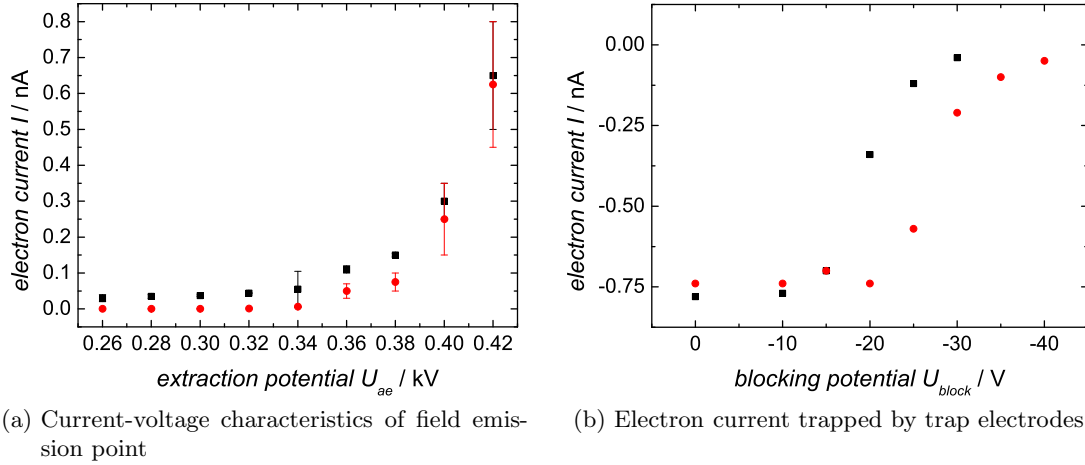
Figure 4.7: (a) Current-voltage curve of field emission of the FEP implemented inside the bore vacuum in the magnetic field at room temperature. The high voltage U_{\text{ae}} is applied to the acceleration electrode. The black squares denote the current measured at the FEP, the red circles that measured at the target at the other side of the trap tower. (b) Electron current as a function of the blocking voltage U_{\text{block}} applied to two different transport electrodes (black squares and red circles).
