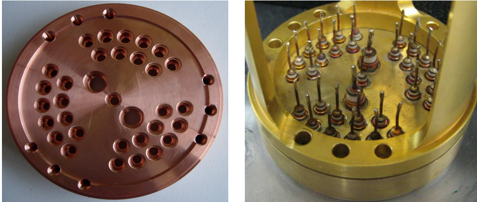
Figure 4.14: Mounting flange of the UHV trap chamber. The machined piece is shown on the left, the gold-plated and with 33 electric feedthroughs equipped mounting flange with the adjacent workpiece on the right side.
