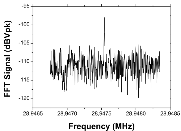
Figure 5. Fourier-transform of the noise in the radial detection circuit showing a maximum at the perturbed cyclotron frequency induced by a single trapped proton.
