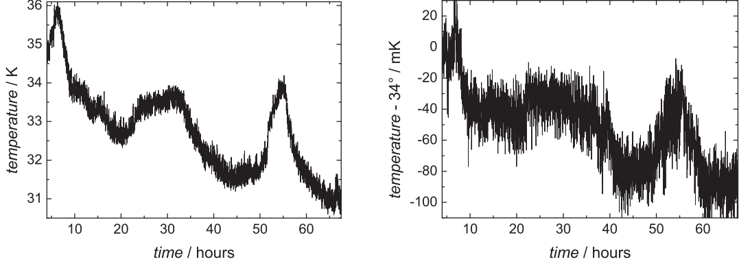
Figure 4.9: Temperature development during the measurement of the voltage stability. On the left, the development of the ambient laboratory air is plotted, on the right, the corresponding one of the copper housing of the voltage source.
