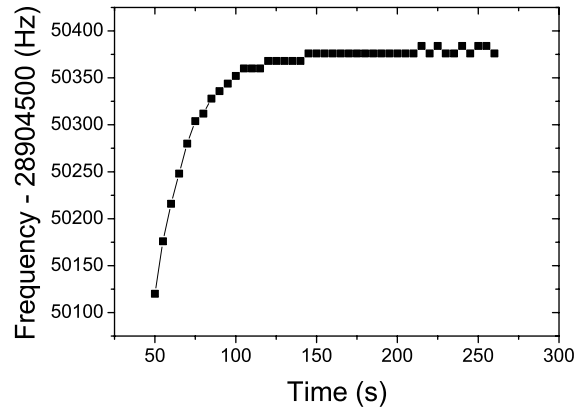
Figure 6. Change of the cyclotron frequency of a single proton in the analysis trap by resistive cooling.
