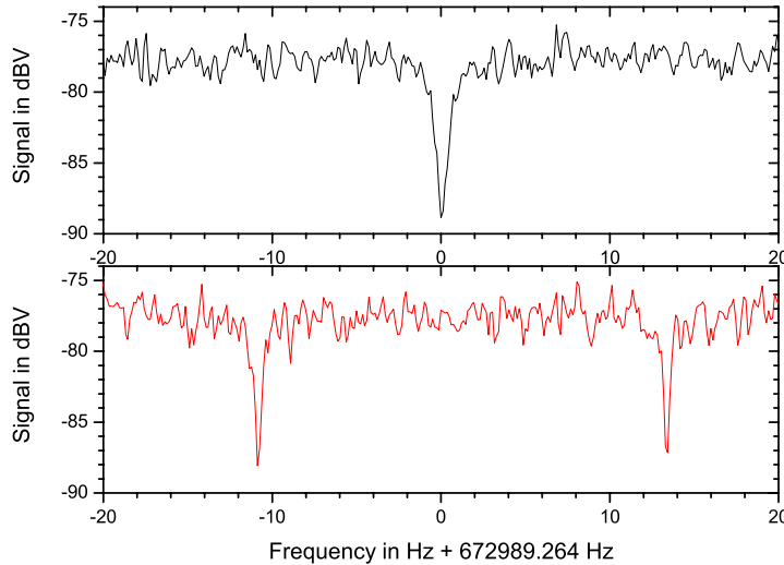
Figure 3. a(upper trace): Axial signal from a single \text{Si}^{12+} ion resistively cooled to 4K. b(lower trace): Split of the axial resonance into two components when axial and cyclotron oscillations are coupled by an additional rf field at their frequency difference.
