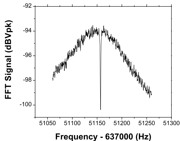
Figure 7. Axial resonance of a single proton in thermal equilibrium with a circuit at 4 K.
