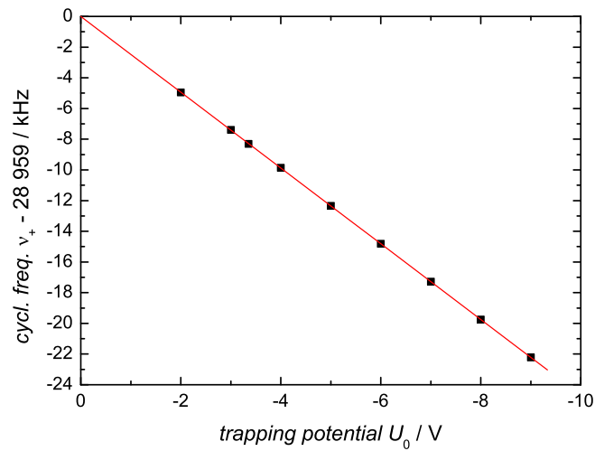
Figure 5.10: Cyclotron frequency \nu_+ as a function of the voltage applied to the ring electrode U_0 . The red curve denotes a linear extrapolation fitted to the data, where the intercept at the y -axis defines the zero in frequency.
