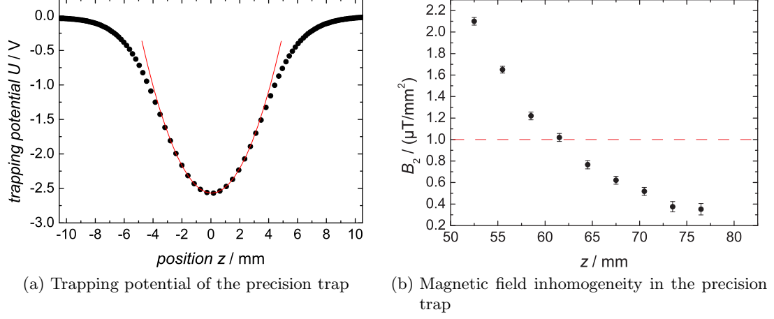
Figure 2.5: (a) The trapping potential of the precision trap is shown as a result of a simulation with SIMION. At the ring electrode, a voltage of U_0 = -3.3 V is applied, the correction electrodes are provided with a voltage of T_{\text{id}}^{\text{pt}} \cdot U_0 , and the end caps are grounded. A harmonic potential (red curve) is fitted within \pm 2 mm around the center, however, the curve is drawn for a wider interval. (b) The magnetic field inhomogeneity in the vicinity of the center of the precision trap introduced by the ferromagnetic ring of the analysis trap. The required distance between the two trap centers to meet the condition B_2 \leq 1 \mu\text{T} / \text{mm}^2 is 72 mm.
