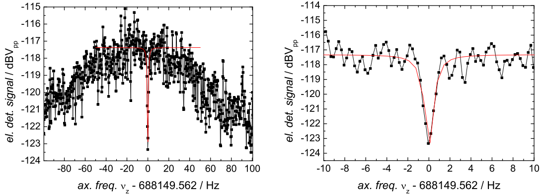
(a) Single particle dip in the noise spectrum of the axial detection circuit. (b) Zoom into the noise spectrum with \pm 10 Hz around the dip center.
