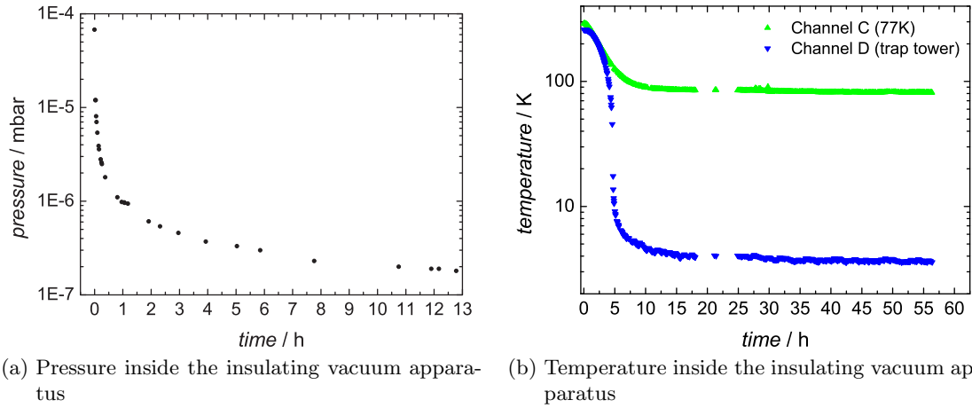
Figure 4.5: The pressure development inside the bore vacuum at room temperature is shown on the left and the temperature development of the two cooling stages inside the bore vacuum on the right.
