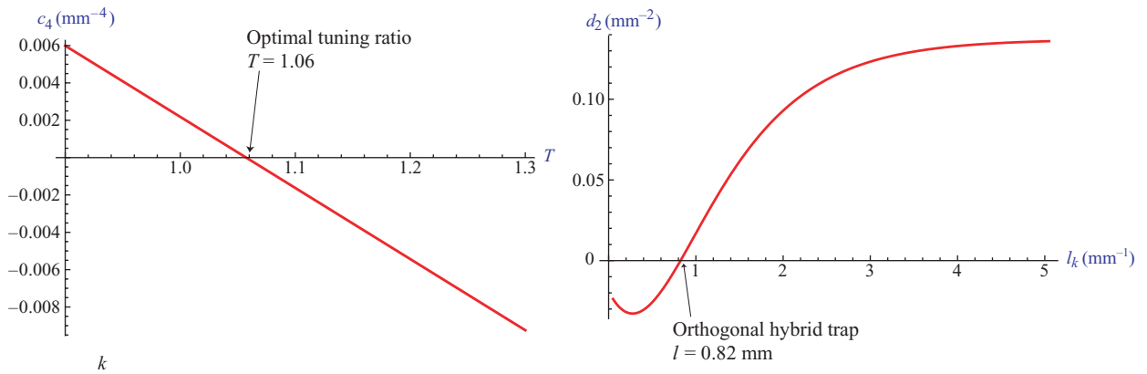
Figure 8. Left: the c_4 term can be canceled by applying the optimal tuning ratio. Right: a specific l_k makes d_2 = 0 and the trap becomes orthogonal.
