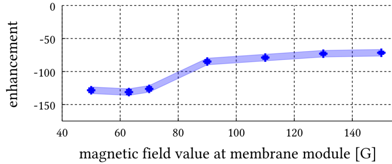
(a) ortho
