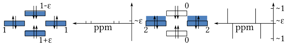
(a) Thermal equilibrium polarization: All energy levels are populated. The NMR signal arises from the small population differences described by the Boltzmann factor. (b) Hyperpolarized: The spin system is out of thermal equilibrium, only antiparallel levels are populated.
