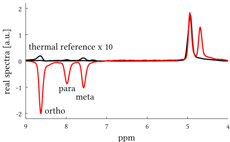
Figure 5.2: Spectrum of hyperpolarized pyridine (red) and corresponding thermal reference (black). Pyridine peaks are located between 7 to 9 ppm, residual water of the solvent ( D_2O ) at 4.9 ppm, and orthohydrogen at 4.7 ppm. The hyperpolarization was generated at a field of 70 Gauss outside the spectrometer and detected inside at 4.7 Tesla.
