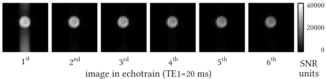
Figure 3.23: Images generated within a echo train with hyperpolarized 2-hydroxyethylpropionate. A fixed set of TE_1 = 20 ms and TE_2 = 3.5 ms was used. The magnetization during the first image was not stable leading to artifacts, later images show almost no artifacts (see 3.24 on the next page for proper scaling). Imaging was performed using a centric reordered deFSE sequence, flip angle: 45^\circ , time per image: 126 ms, echo time 1: 20 ms, echo time 2: 3.5 ms, bandwidth: 1375 Hz/pixel, matrix size: 36 \times 36 (presented: 30 \times 20 ), phase encoding: up-down, resolution: 1.36 mm/pixel, crusher gradients: 40\pi /voxel and slice thickness 10 mm.
