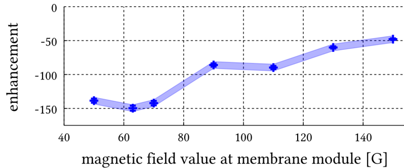
(c) meta
