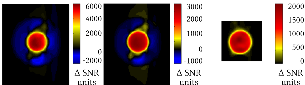
(a) Hyperpolarized 1-Hexene and (b) Hyperpolarized 2-hydroxy-ethylpropionate and thermally polarized water: Image at echo time 15 ms subtracted from polarized water: Image at echo time 10 ms (images at figure 3.11 on page 37). (c) Hyperpolarized 2-hydroxy-ethylpropionate and thermally polarized solvent at the same image at echo time 15.1 ms subtracted from image at echo time 11.5 (images at figure 3.18 on page 43).
