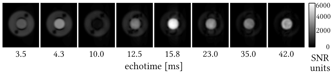
Figure 3.11: MR-images of hyperpolarized PHIP substance (1-Hexene) surrounded by thermally polarized water acquired at different echo times ( TE_{\min} + tw = 3.5 \text{ ms} + tw ) by individual experiments. The typical signal decay within the thermally polarized area can be observed. The intensity evolution of the hyperpolarized area, however, is generated by the hyperpolarized protons. Imaging was performed by using a slice selective gradient echo sequence with centric reordering, flip angle: 10^\circ , repetition time: 45 ms, bandwidth: 600 Hz, FOV: 60 \text{ mm}^2 , acquisition matrix: 88 \times 88 , resolution: 0.7 \text{ mm}/\text{pixel} and slice thickness 10 mm.
