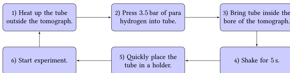
Figure 3.7: Measurement protocol for hyperpolarization experiments.
