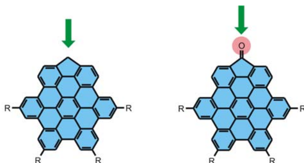
Figure 6-3: Direct functionalization of the aromatic core in CPHBC(C 12 ) 4 5-80 and CPHBCCO(C 12 ) 4 5-81.
