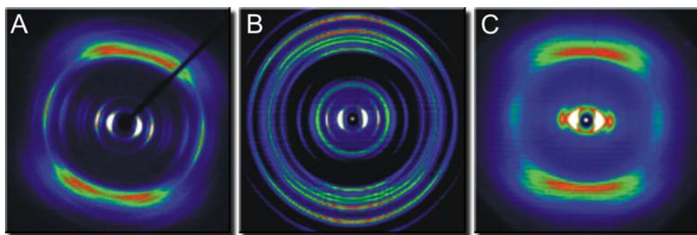
Figure 5-53: Temperature 2D-WAXS patterns of derivatives with a symmetrical architecture as (A) \text{HBC-C}_{12} 3-3a , (B) p\text{DBPO}(\text{C}_{12})_2 5-42 and (C) \text{DPO}(\text{C}_{12})_6 5-57 .
