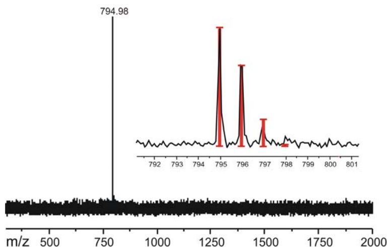
Figure 5-27: MALDI-TOF spectrum of pDBPO(tBu) 4 5-37 , solid-state prepared sample using TCNQ as matrix substance.
