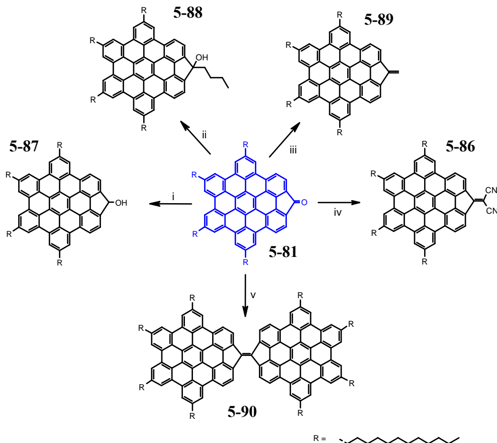
Scheme 5-23: Tested reactions for the functionalization of CPHBCCO(C 12 ) 4 5-81 : i) Reduction with LiAlH 4 ; ii) reaction with n -BuLi; iii) WITTIG reaction; iv) KNOEVENAGEL with malonitrile; v) MCMURRAY reaction.
