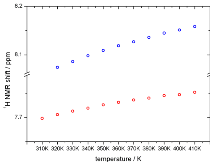
Figure 5-83: Temperature dependent 1 H NMR shifts of the aromatic ring protons of 5-115 , recorded in tetrachloroethane- d 2 .
