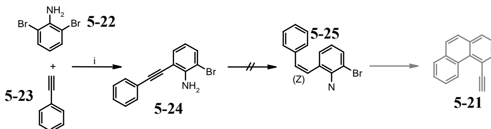
Scheme 5-7: i) Cl 2 Pd(PPh 3 ) 2 , 42%.
