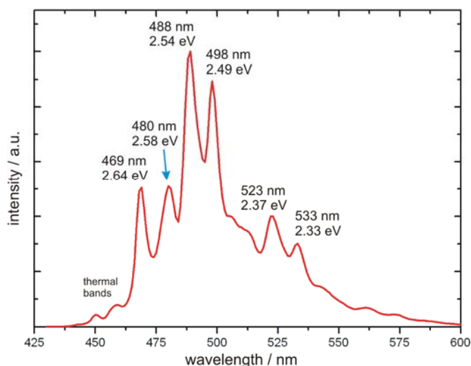
Figure 5-9: PL spectrum of HBC-C 12 3-3a ( \lambda_{\text{ex}} = 362 \text{ nm} , in oDCB).
