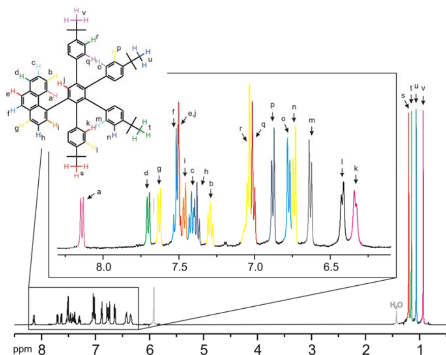
Figure 5-15: ^1\text{H} NMR spectrum of 5-13b , recorded in 1,1,2,2-tetrachloroethane- d^2 at 80 °C (500 MHz).
