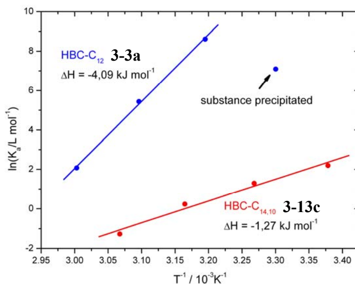
Figure 3-10: van't Hoff plot of self-association constants K_a for HBC- C_{14,10} 3-13c and HBC- C_{12} 3-3a .
