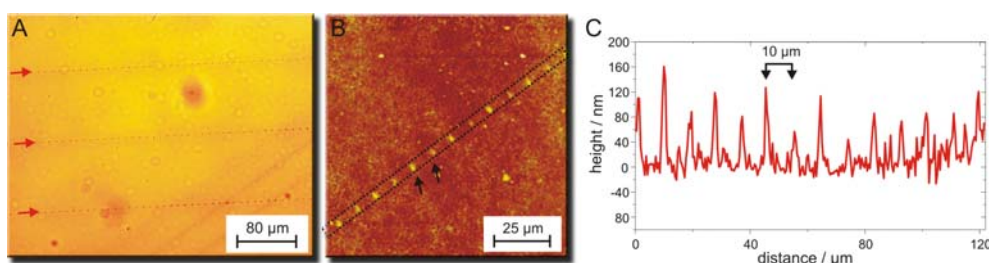
Figure 4-30: Analysis of the nanostructured HBC- C_5 -acrylate 4-18 (A) optical microscopy image, red arrows mark the written point-lines (B) AFM topography image, dotted box indicates the written “columns”, black arrows point onto two “columns” and (C) height profile of the dotted box in (B), written “columns” are separated by \sim 10 \mu\text{m} .
