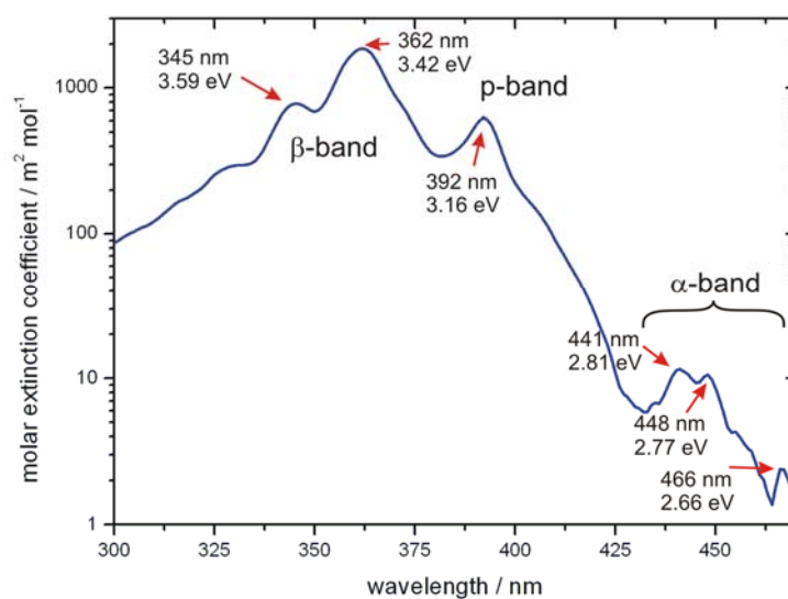
Figure 5-8: Logarithmically plotted UV/vis absorption spectrum of HBC- C_{12} 3-3a (oDCB).
