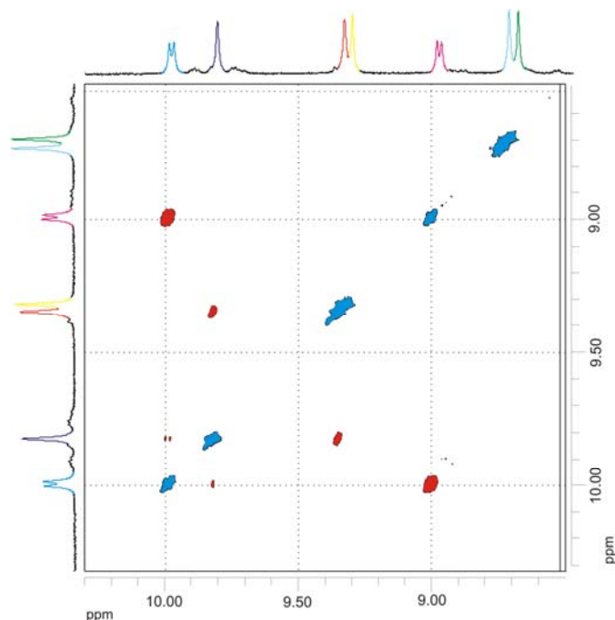
Figure 5-26: H,H COSY of pDBPO(tBu) 4 5-37 , recorded in THF-d 8 at 57 °C (700 MHz).
