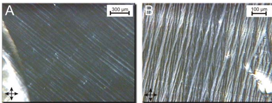
Figure 4-31: POM images of zone-cast HBC-C 5 -acrylate 4-18 films, different magnifications.
