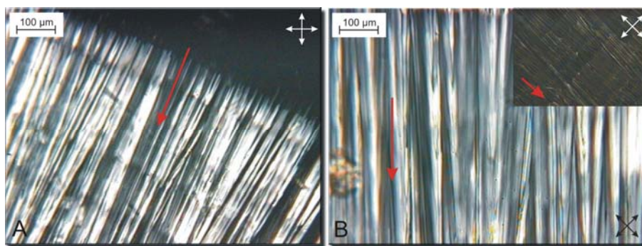
Figure 3-22: A: POM of the nucleation site, at which the structures begin to grow in the moving direction of the support; B: POM of the interior of the film revealing a uniaxial orientation of the microfibers.
