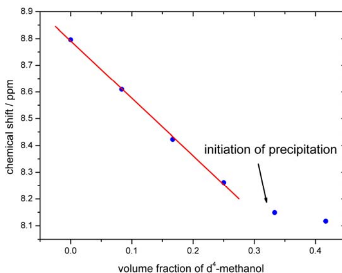
Figure 3-8: Chemical shift dependence of HBC- C_{14,10} 3-13c in a mixture of methanol- d^4 and 1,1,2,2-tetrachloroethane- d^2 with different compositions (concentration: 4.75 \times 10^{-3} M).
