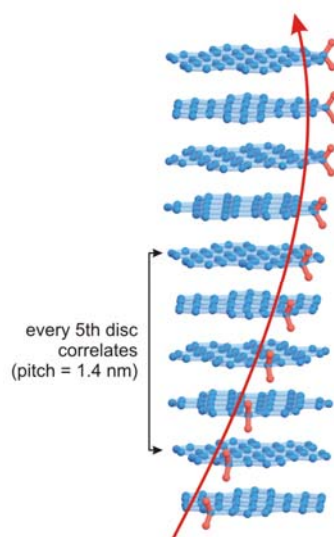
Figure 5-73: Suggested helical superstructure in the crystalline phase of CPHBC(C 12 ) 4 5-80 with a helical pitch of 1.4 nm (5 discs); alkyl chains are omitted for clarity.
