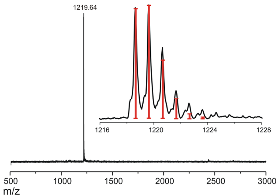
Figure 5-14: MALDI-TOF spectrum of \text{TBO}(\text{C}_{12})_4 5-16c , solid-state prepared sample using TCNQ as the matrix substance.
