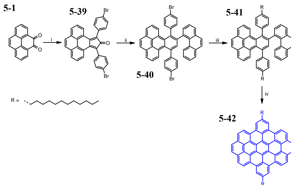
Scheme 5-12: i) 1,3-bis-(4-bromo-phenyl)-propan-2-one, KOH, 47%; ii) 4-ethynylphenanthrene, 75%; iii) RMgBr, Pd(dppf)Cl 2 , 91%; iv) FeCl 3 , 90%
