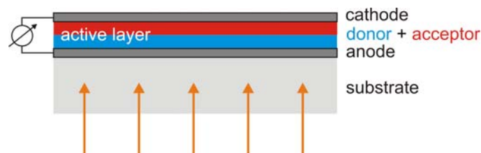
Figure 1-16: Schematic presentation of the setup of a heterojunction photovoltaic device.
