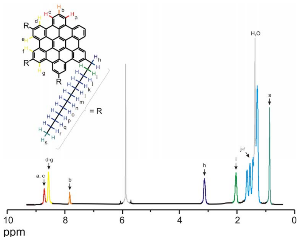
Figure 5-52: ^1H NMR of HBC( C_{12} ) _4 5-74 , recorded in THF-d^8 at 57 °C.
