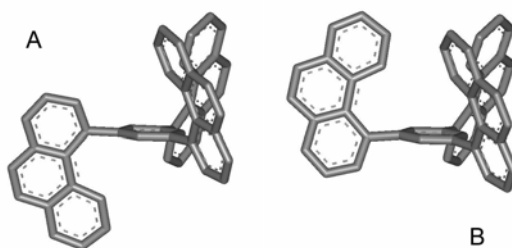
Figure 5-34: Simulated atropisomers of 5-44A and 5-44B (molecular mechanic force field, MMF).
