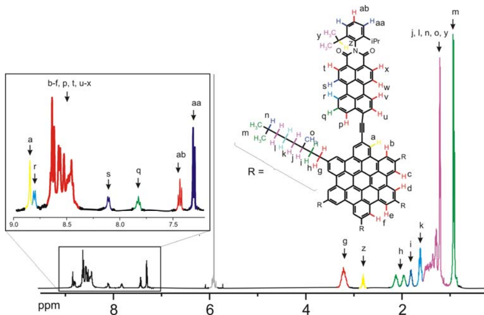
Figure 4-3: ^1\text{H} NMR spectrum of HBC-PMI 4-4 , recorded in 1,1,2,2-tetrachloroethane- d^2 at 127 °C, solvent peak was colored in grey.
