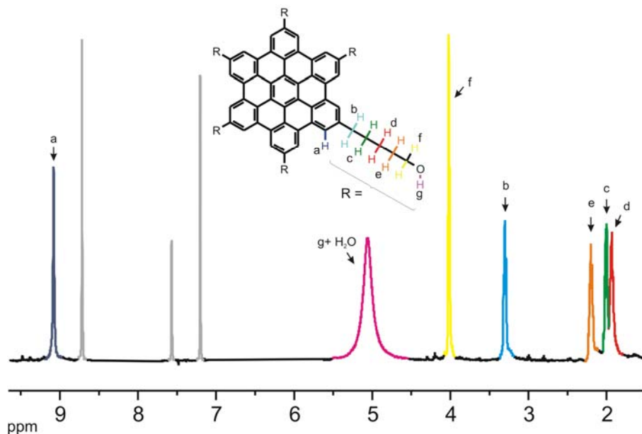
Figure 4-10: ^1H NMR spectrum of HBC- C_5OH 4-12 , recorded in pyridine- d^5 (500 MHz), solvent signals are colorized in grey.
