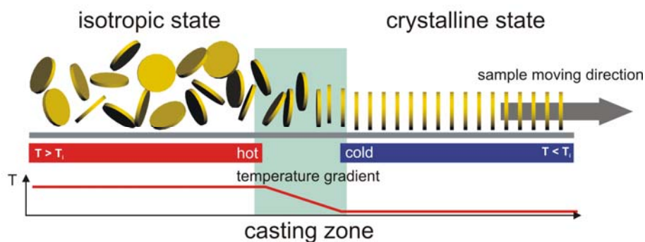
Figure 3-40: Schematic presentation of zone-crystallization processing.
