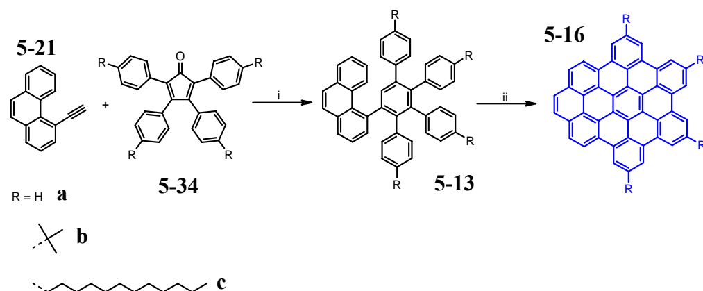
Scheme 5-9: Synthetic concept towards TBO derivatives using 4-ethynylphenanthrene as building block. i) 84-95%; ii) \text{FeCl}_3 , 79-83%.
