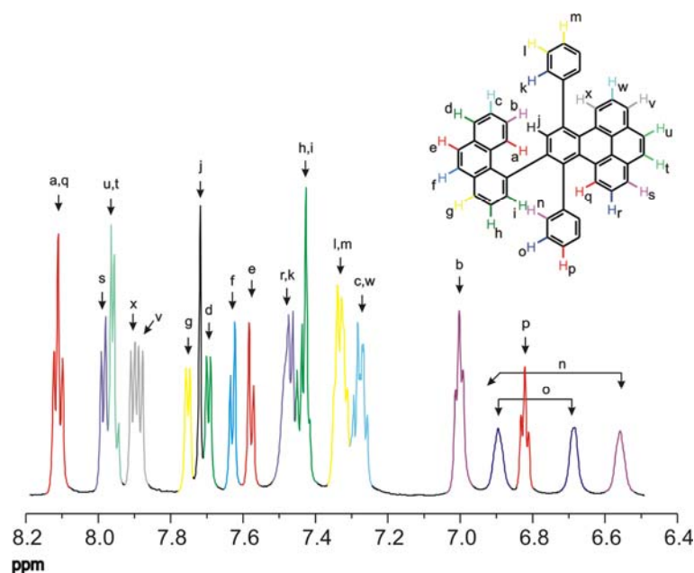
Figure 5-21: ^1\text{H} NMR of 5-35 , recorded in \text{THF-d}^8 at 70\text{ }^\circ\text{C} (700 MHz).
