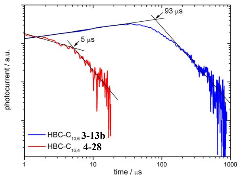
Figure 3-67: Comparison of the hole current transients for thick samples ( 44 \mu\text{m} ) of HBC- C_{10,6} 3-13b and HBC- C_{16,4} 4-28 , both recorded at 40^\circ\text{C} in their mesophase with an electric field of 1.36 \times 10^4 \text{ V/cm} .
