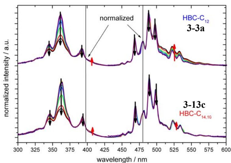
Figure 3-11: PL and PLE spectra of HBC-C 14,10 3-13c and HBC-C 12 3-3a in CHCl 3 at concentrations between 1x10 -4 to 1x10 -7 M (black to blue); normalized at 480 nm and 398 nm, respectively. Arrows point into the direction of the highest concentration.
