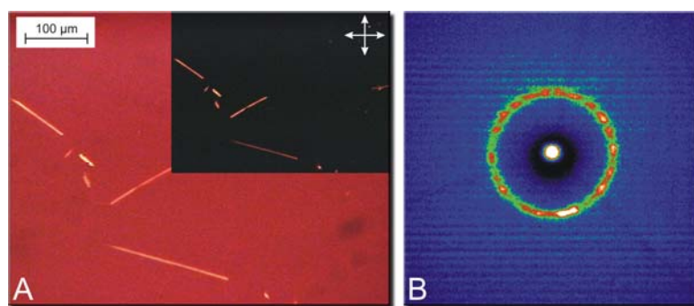
Figure 3-57: Example for a homeotropically aligned sample based on the mixture of HBC- C_{10,6} ( 3-13b ) and PDI- C_{8,7} ( 3-19 ) of a molar ratio of 2:1 a) image from the optical microscopy (inset in cross-polarizers) and b) characteristic 2D-WAXS pattern of the film with homeotropic order (identical hexagonal lattice in different small domains led to the multiple appearance of reflections).
