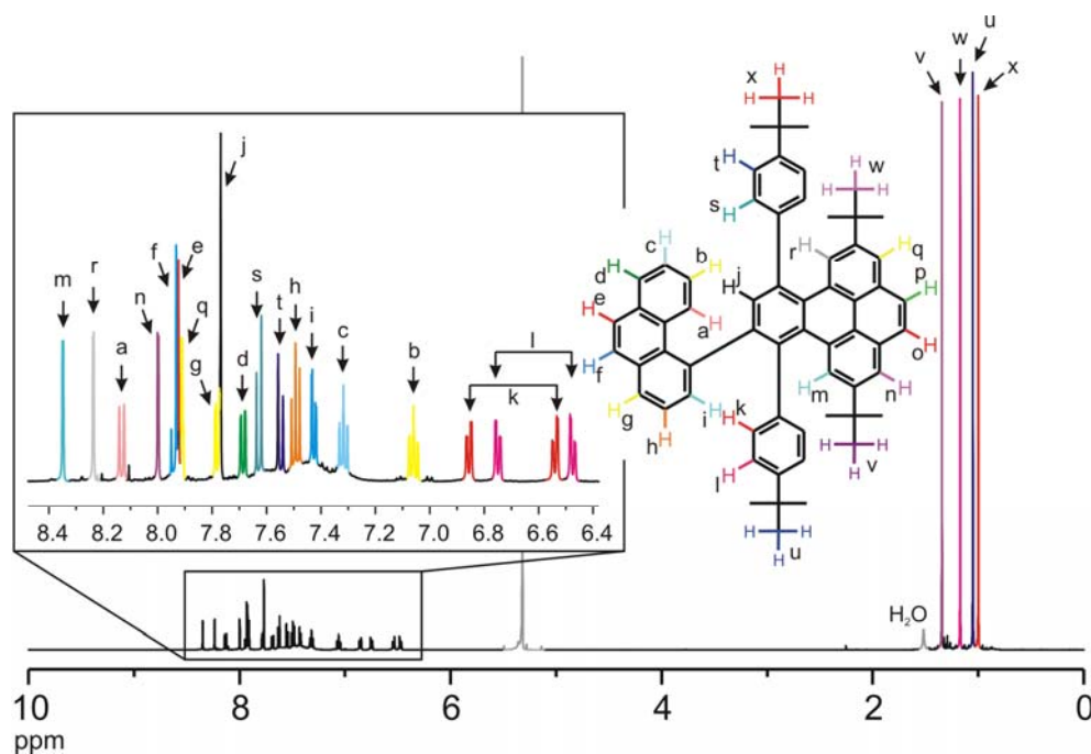
Figure 5-23: ^1H NMR of 5-37 , recorded in dichloromethane- d^2 at 25 °C (500 MHz).
