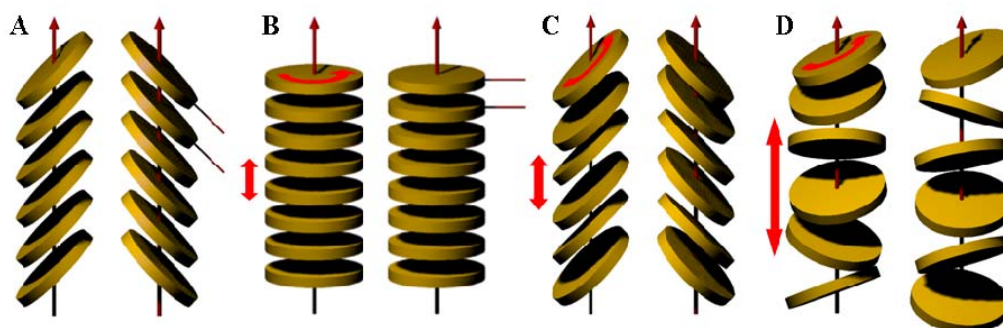
Figure 3-47: Schematic illustration of the arrangement of the aromatic core in (A) the herringbone order, (B) the planar arrangement which is characteristic mesophase-organization for HBCs substituted by alkyl chains with a low steric demand, (C) the disordered columnar arrangement of the HBC- C_{6,2} 3-13a and (D) of the HBC- C_{10,6} 3-13b discs in the mesophase. Thereby, the discs possess a rapid rotation around the columnar axes, whereby the longitudinal fluctuations increase with longer side chains.
