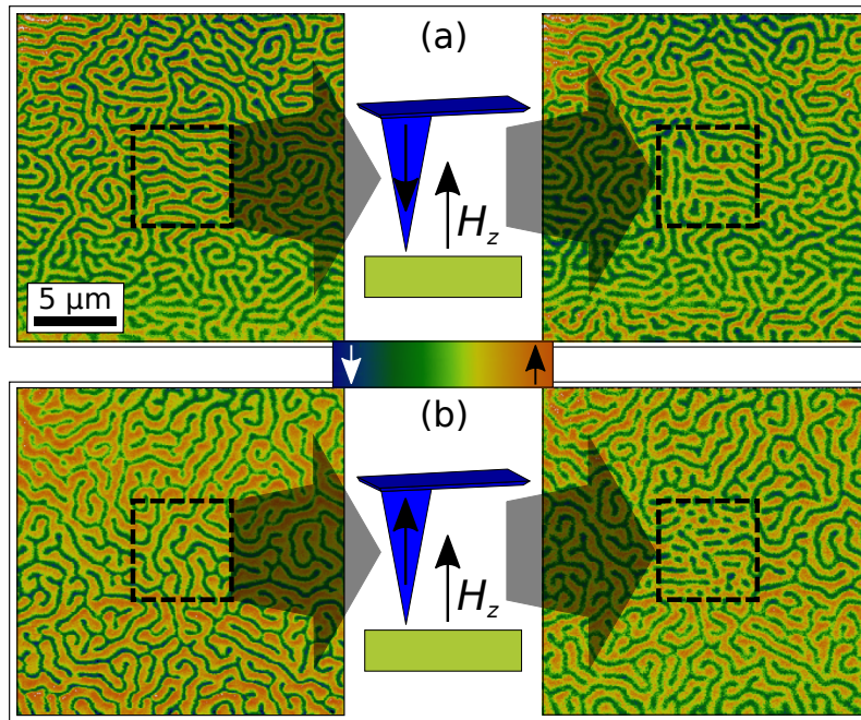
Figure 7. MFM probe-cutting of labyrinth domains into individual skyrmions. Single pass MFM images of W/CoFeB/MgO multilayer under an applied field of \sim 10 mT before (left) and after (right) a topography scan of the central area (not show) with the tip magnetised against (a) or along (b) the external field. The topography scan was performed with the slow scan axis from bottom to top. The color scale bar indicates the direction of the magnetisation in the sample.
