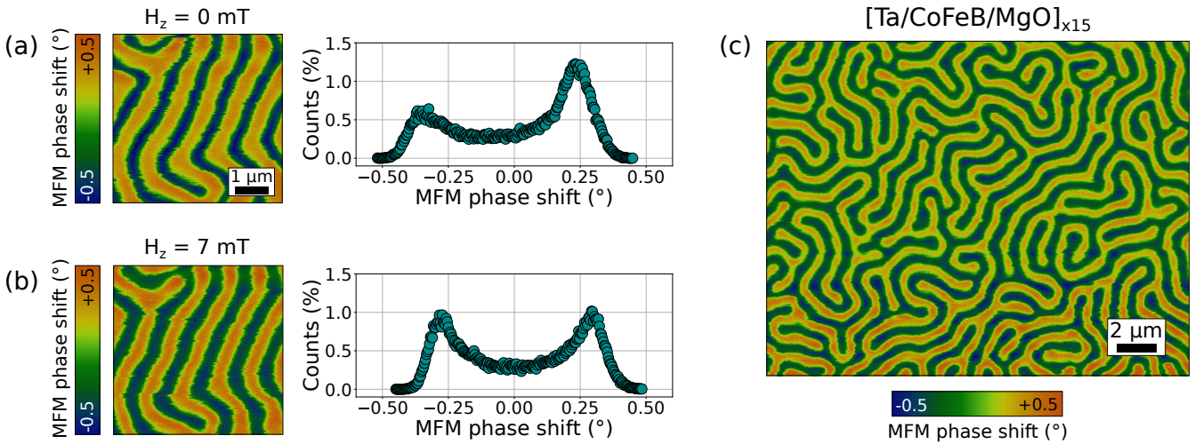
Figure 2. Procedure used to image the demagnetised configuration. MFM imaging of Ta/CoFeB/MgO multilayer at \Delta z = 145 nm without (a) and with (b) an external perpendicular bias field H_z \sim 7 mT, applied to compensate for the probe stray field. Image histograms are shown beside the corresponding MFM images. (c) Example of one of the MFM images for the Ta/CoFeB/MgO stack used to extract the DMI constant D . \Delta z and H_z are the same as in (b).
