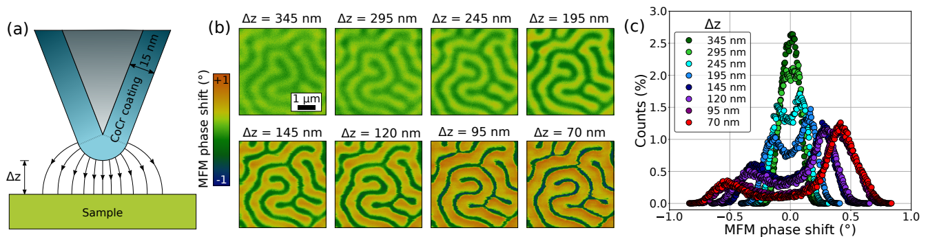
Figure 1. MFM image perturbations caused by probe-sample magnetic interaction. (a) Schematic illustration of the magnetic stray field generated by an MFM probe. All MFM imaging was performed using low moment tips (NT-MDT MFM-LM), with magnetic CoCr coating thickness of \sim 15 nm. \Delta z represents the tip lift height used to record the MFM phase signal. (b) MFM imaging of the demagnetised state of Ta/CoFeB/MgO multilayer at different \Delta z , with the corresponding image histograms shown in (c). The bin width is kept constant across all histograms.
