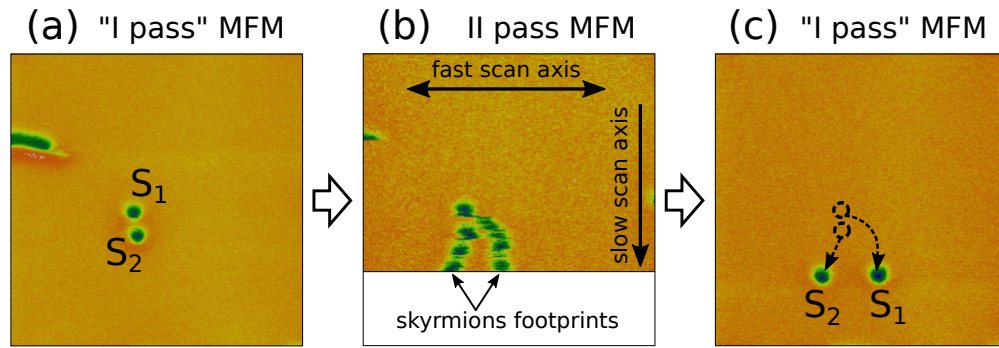
Figure 5. MFM imaging of the probe-driven interaction between two individual skyrmions. Sequence of MFM images illustrating the dynamics of probe-driven skyrmion interaction in Pt/CoFeB/MgO multilayer under an applied perpendicular field H_z = 71 mT. (a,c) Two individual skyrmions, marked by S_1 and S_2 , are imaged in single pass MFM mode at a lift height \Delta z = 145 nm, with the topography acquired separately at H_z = 50 mT. The dashed arrows are guides for the eye indicating the trajectories followed by the skyrmions during the probe-driven interaction. (b) Skyrmion S_1 is pushed against skyrmion S_2 by the probe stray field during the topography line scans of a standard two pass MFM scan (also with \Delta z = 145 nm). Skyrmion S_1 avoids the collision with skyrmion S_2 by jumping abruptly towards the right. The directions of fast and slow scan axes are marked by the arrows. The tip is magnetised along the external field direction, thus opposing the skyrmions core magnetisation.
