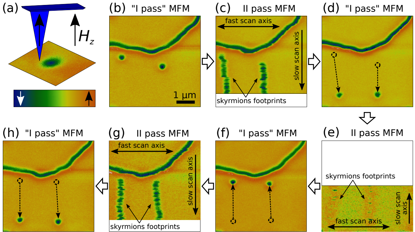
Figure 3. MFM imaging of individual skyrmions and manipulation by local field gradients. Sequence of MFM images illustrating individual skyrmion manipulation by MFM in Pt/CoFeB/MgO multilayer under an applied perpendicular field H_z = 71 mT. (b,d,f,h) Skyrmions are imaged in single pass MFM mode at a lift height \Delta z = 145 nm, with the topography acquired separately at H_z = 50 mT. The dashed arrows are guides for the eye indicating skyrmion motion between consecutive steps. (c,e,g) Skyrmions are moved by the probe stray field during the topography line scans of a standard two pass MFM scan (also with \Delta z = 145 nm), which reveal the trajectory followed by skyrmions in the form of actual skyrmion “footprints”. These scans were stopped before reaching the end only to prevent skyrmions from moving outside of the selected region. The directions of fast (with trace and retrace line scans) and slow MFM scan axes are marked in the individual images. The spacing between consecutive line scans along the slow scan axis is \delta \sim 20 nm. As indicated by the sketch in (a), the tip is magnetised along the external field direction for all MFM images, thus opposing the skyrmions core magnetisation.
