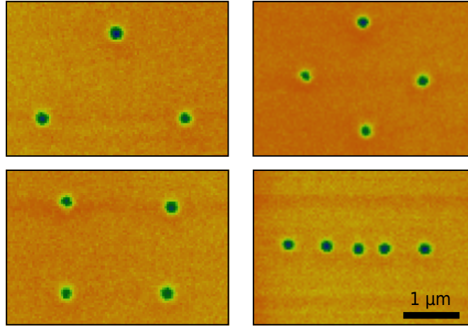
Figure 4. Drawing arbitrary patterns with individual skyrmions. Single pass MFM imaging of different geometrical skyrmion patterns in Pt/CoFeB/MgO multilayer obtained by manipulating the individual skyrmions through a series of two pass MFM scans (not shown) with \delta \sim 10\text{-}20 nm. All images are taken at a lift height \Delta z = 145 nm and under an applied perpendicular field H_z = 71 mT, with the topography acquired separately at H_z = 50 mT. The tip is magnetised along the external field direction, thus opposing the skyrmions core magnetisation.
