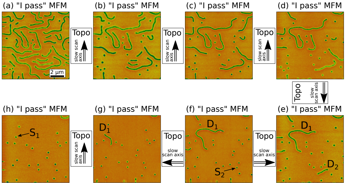
Figure 6. MFM probe-induced collapse of domains into individual skyrmions. Sequence of MFM images illustrating conversion of domains into skyrmions via MFM in Pt/CoFeB/MgO multilayer under an applied perpendicular field H_z = 57 mT. All images are acquired in single pass MFM mode at a lift height \Delta z = 145 nm. A topography scan with a line spacing \delta \sim 40 nm is performed between each image (not shown), with the slow scan axis direction as indicated by the arrows. Symbols D_1 and D_2 mark two stripe domains which convert into skyrmions S_1 and S_2 , respectively, upon successive topography scans, as explained in the text. In all images the tip is magnetised along the external field direction, thus opposing the skyrmions core magnetisation.
