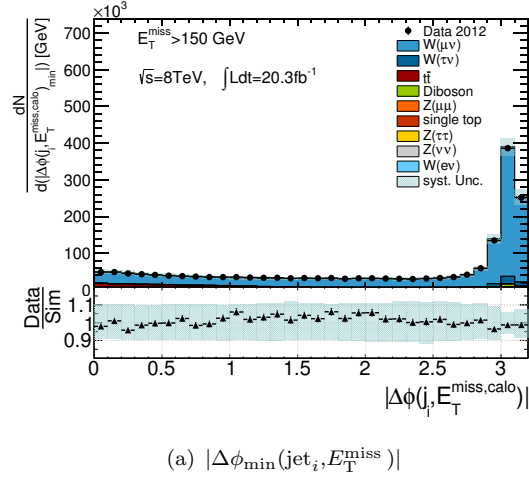
FIGURE 14.28: |\Delta\phi_{\min}(\text{jet}_i, E_T^{\text{miss}})| in the lowest W^\pm(\rightarrow \mu^\pm\nu)+\text{jets} control region.
