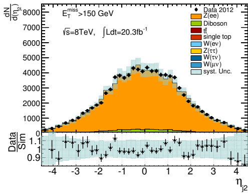
(a) Pseudo-rapidity
