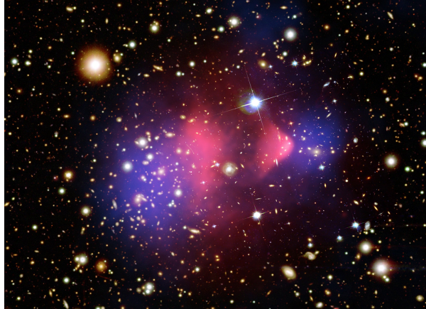
FIGURE 3.3: The “Bullet Cluster”: product of the collision of two galaxy clusters. The dark matter halo shown in blue is inferred from gravitational lensing effects. [51]
