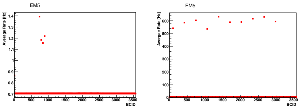
FIGURE 8.8: CTPMON rate histograms for EM5 from run 191381 and 191628. [205]
