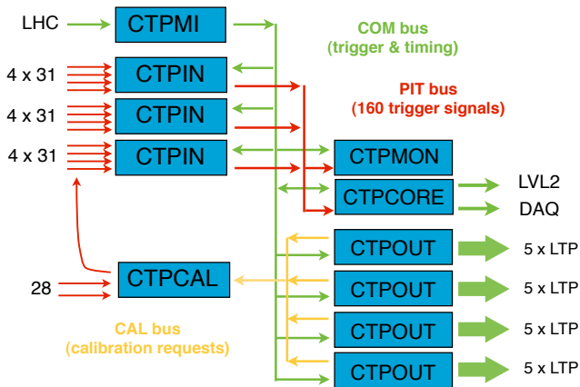
FIGURE 7.10: Schematic view of the central trigger system, its boards and the signal distribution. Adapted from figure 11 in reference [180].
