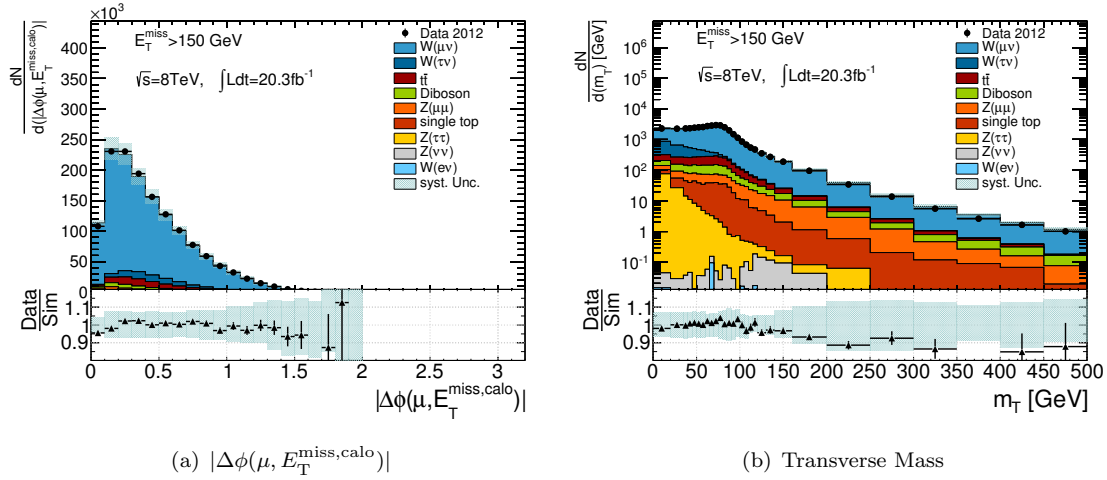
FIGURE 14.27: Azimuthal separation of muon and E_T^{\text{miss}} (a) and transverse mass distribution (b) in the lowest W^\pm(\rightarrow\mu^\pm\nu) +jets control region.
