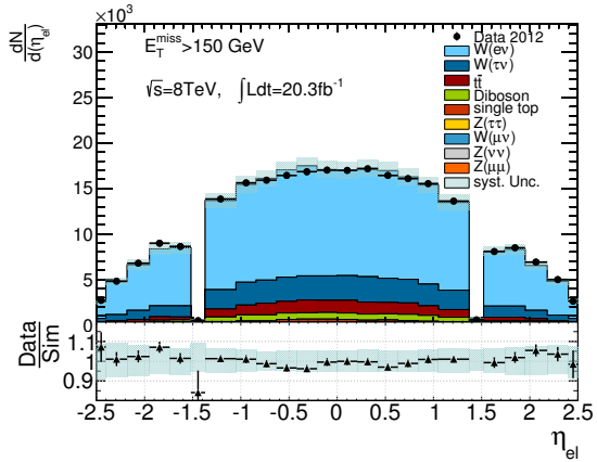
(a) Pseudo-rapidity
