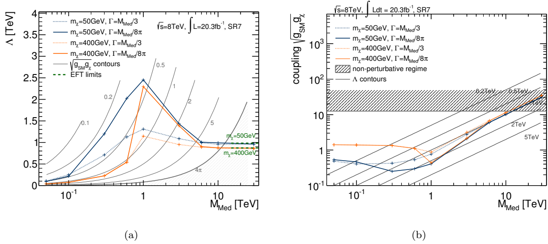
FIGURE 15.9: 95% CL observed lower limits from SR7 on the scale \Lambda (a) and upper limit on the coupling (b) in the simplified model as a function of the mediator mass M_{Med} . Blue lines are for m_\chi = 50 GeV, orange lines for m_\chi = 400 GeV. Limits for \Gamma = M_{Med}/3 are shown as dashed, limits for \Gamma = M_{Med}/(8\pi) as solid lines. Grey lines give the contours of constant \sqrt{g_\chi g_{SM}} (a) and constant \Lambda (b). The non-perturbative regime with couplings larger than 4\pi is indicated as a dark shaded area.
