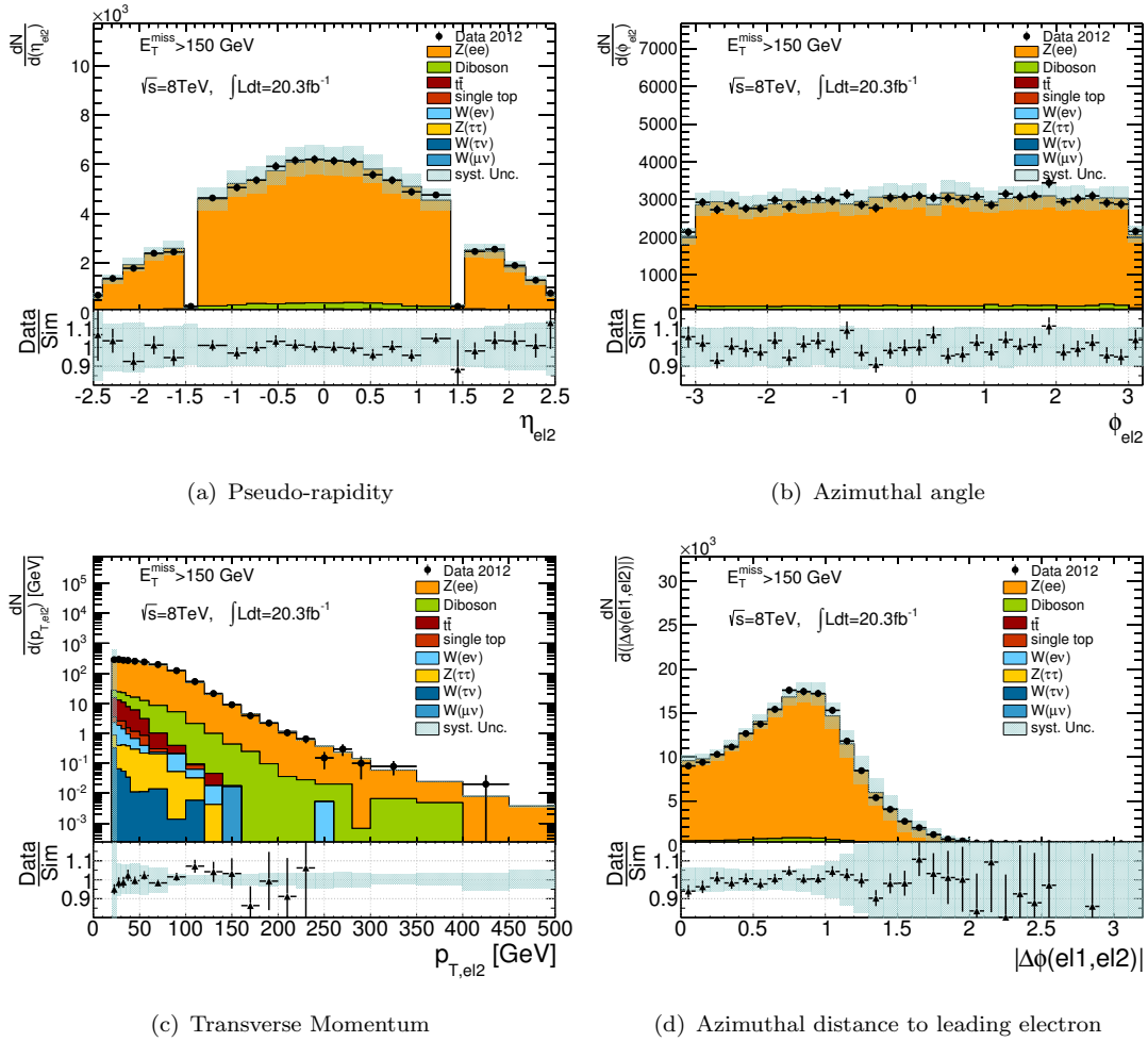
FIGURE 14.19: Kinematic variables of the sub-leading electron in the lowest Z(\rightarrow e^+e^-) +jets control region.
