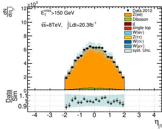
(a) Pseudo-rapidity
