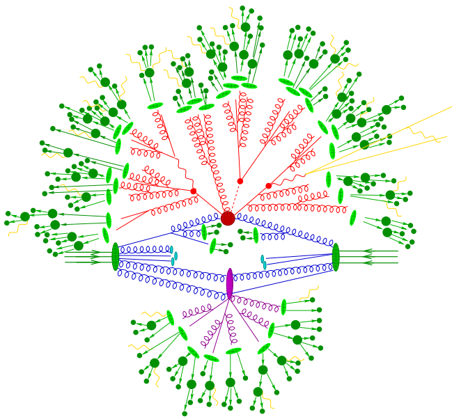
FIGURE 4.1: Illustration of a pp collision. Two partons from the incoming protons (large green ellipses) undergo initial state radiation and interact in the hard process (big red blob). A parton shower (red) emerges from the products of the hard interaction. The resulting partons hadronise into colourless states (light green blobs) that subsequently decay into stable particles (green circles). A secondary interaction between proton remnants is shown as a purple blob, again creating a parton shower (purple), which hadronises, followed by decays into stable particles. This is part of the underlying event, together with the beam remnants (light blue blobs). Electromagnetic radiation (yellow) can be emitted by charged particles at any stage. [101]
