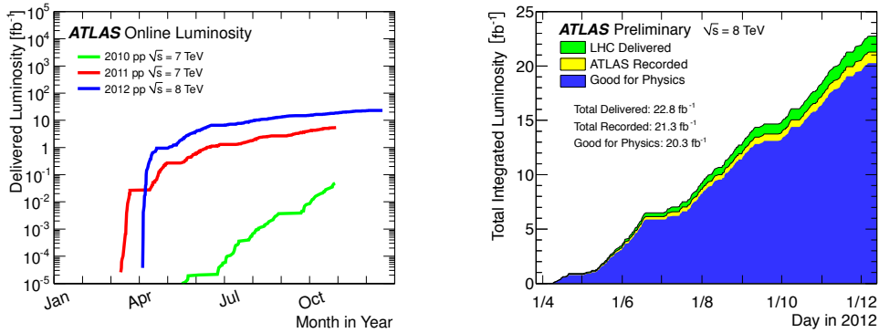
FIGURE 7.12: Left: Cumulative luminosity of pp collisions versus day delivered to ATLAS during stable beams for 2010 (green), 2011 (red) and 2012 (blue). Right: Accumulated luminosity as a function of day in 2012. Total delivered, recorded and deemed good for physics are shown in green, yellow and blue.[204]
