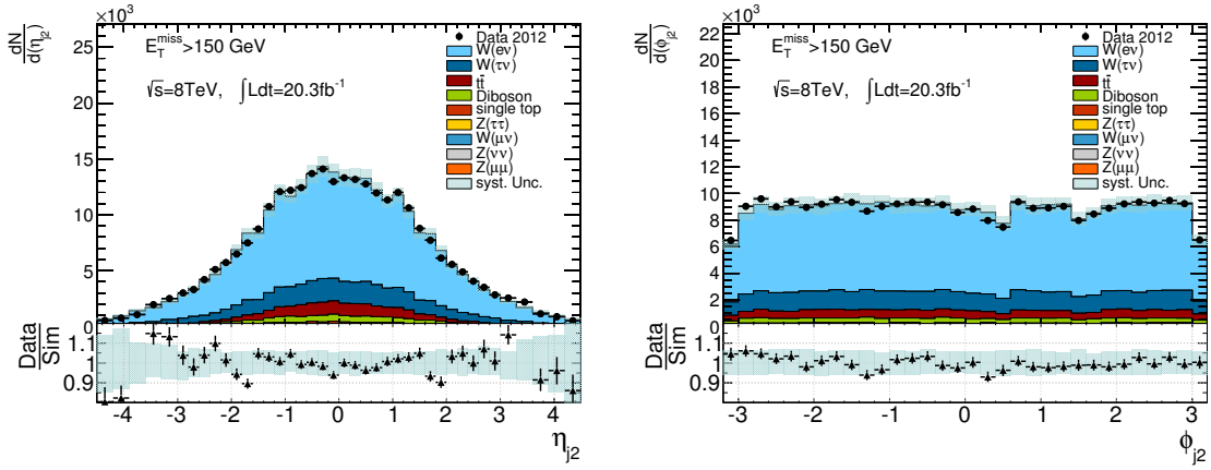
(a) Pseudo-rapidity
