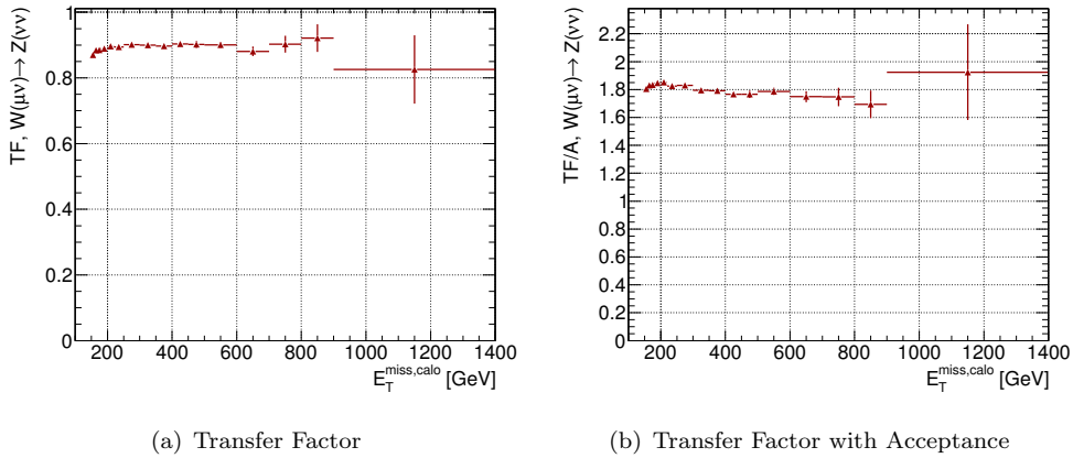
FIGURE 14.32: Transfer factors before and after applying the lepton selection in the W^\pm(\rightarrow\mu^\pm\nu^\pm)+\text{jets} control region.
