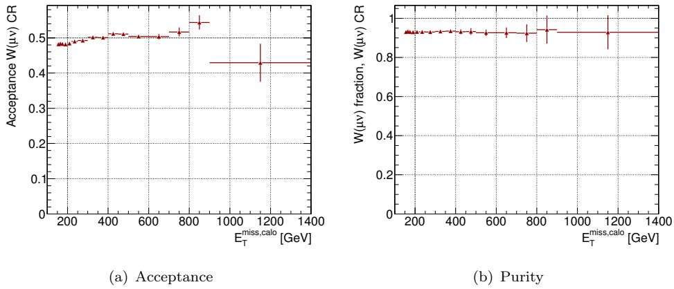
FIGURE 14.31: Acceptance and purity in the W^\pm(\rightarrow\mu^\pm\nu^\pm)+\text{jets} control regions as a function of E_T^{\text{miss}} . The error bars are statistical uncertainties only.
