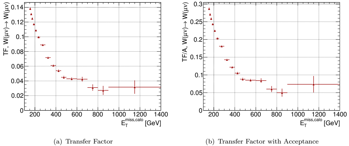
FIGURE 14.42: Transfer factors before and after applying the lepton selection in the W^\pm(\rightarrow \mu^\pm\nu)+\text{jets} control region.
