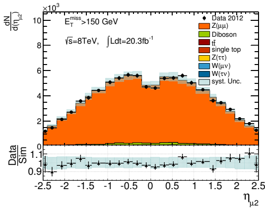
(b) Pseudo-rapidity
