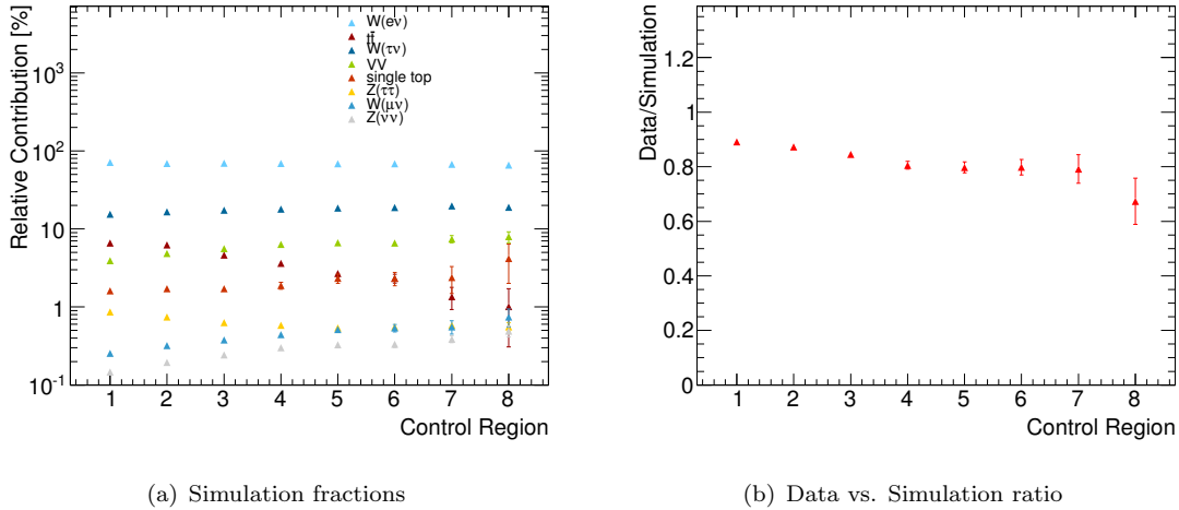
FIGURE 14.43: Relative simulation fractions (a) and ratio of data vs. simulation (b) in the W^\pm(\rightarrow e^\pm\nū)+\text{jets} control regions B. The error bars show statistical uncertainties only.
