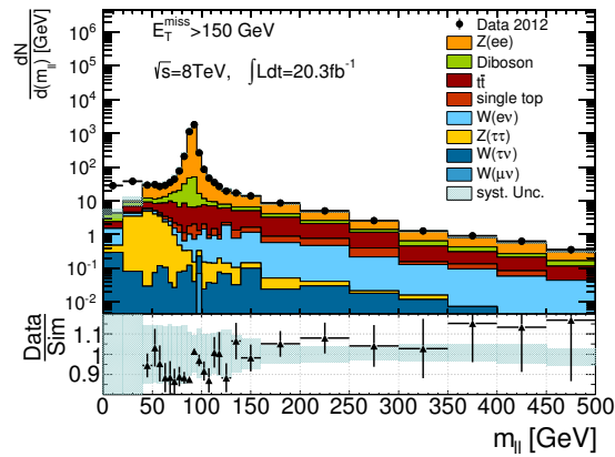
FIGURE 14.20: Di-lepton mass distribution in the lowest Z(\rightarrow e^+e^-) +jets control region.
