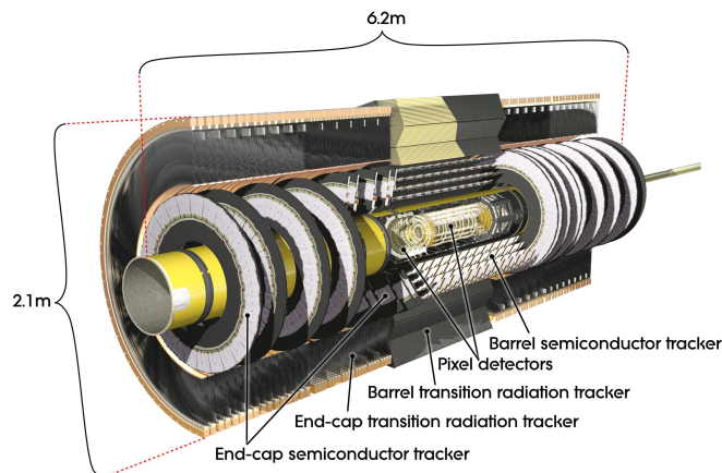
FIGURE 7.2: Schematic view of the ATLAS inner detector. [168]
