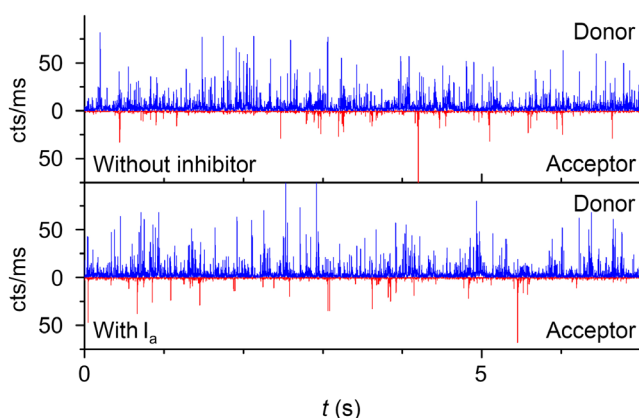
FIGURE 4 Section of the fluorescence intensity time trace of ATTO 488/ATTO 643 FRET pair labeled DENV protease with and without 200 \mu\text{M} of the allosteric inhibitor. The sample was excited with excitation pulses at 502 nm. The binning time was 1 ms. the donor channel is shown in blue, the acceptor channel is shown in red. DENV, dengue virus
