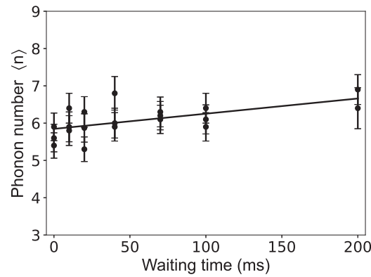
Figure 9. Heating rate of axial motional mode. The mean phonon number is measured for different waiting times after PGC. A linear fit reveals a heating rate of 4.1(8) phonons per second for a trap frequency of 2\pi \times 285 kHz.
