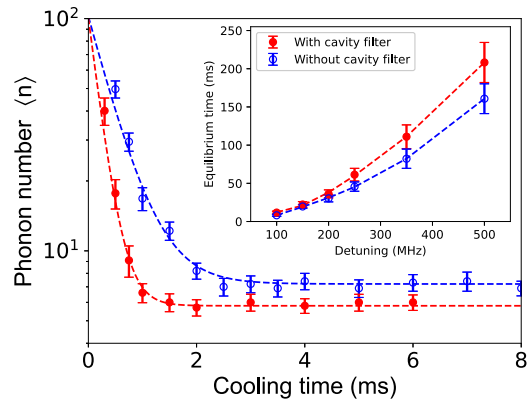
Figure 8. Cooling dynamics of PGC with (red solid circles) and without (blue hollow circles) cavity filter for fixed detuning of 2\pi \times 210 MHz and fixed intensity of the laser beams. The equilibrium cooling rate is improved by a factor of 2.1(2) when the cavity filter is used. Inset: pumping dynamics from one S_{1/2} Zeeman state to the equilibrium by the 393 nm light beams with (red solid circles) and without (blue hollow circles) cavity filter, respectively. The increased pumping rate without the cavity filter is caused by additional resonant scattering events due to the ASE background.
